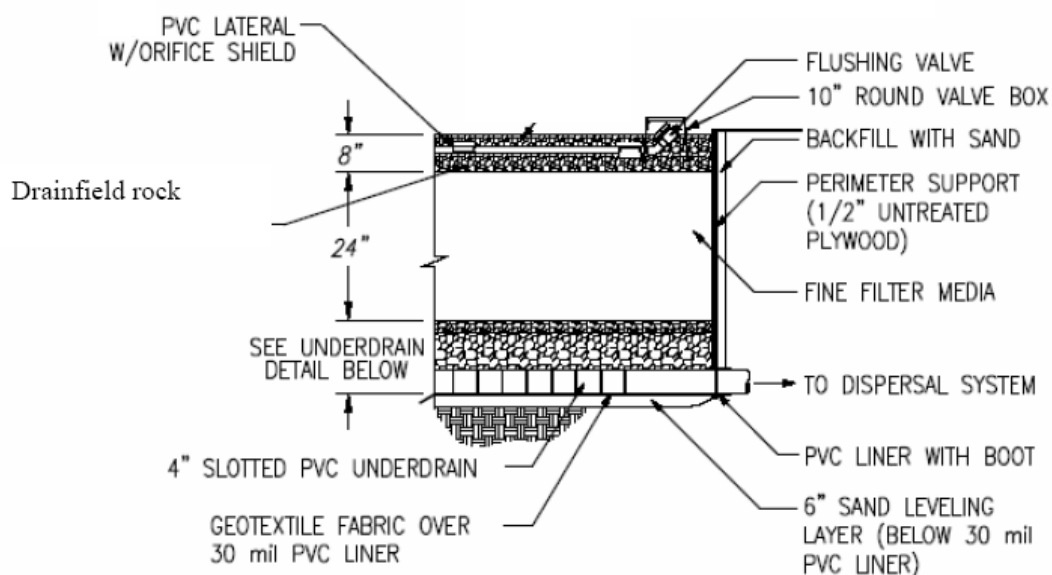
FILTER CROSS SECTION
