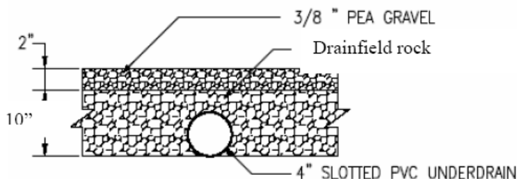
UNDERDRAIN DETAIL
