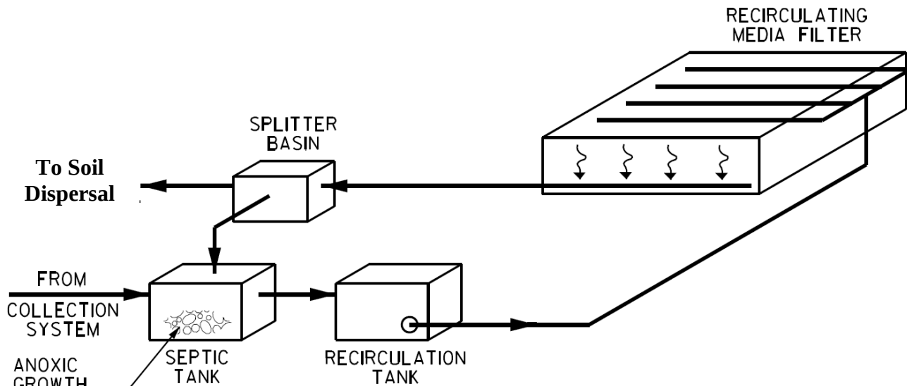
b) RECIRCULATING MEDIA FILTER MODIFIED FOR ENHANCED TOTAL NITROGEN REMOVAL
