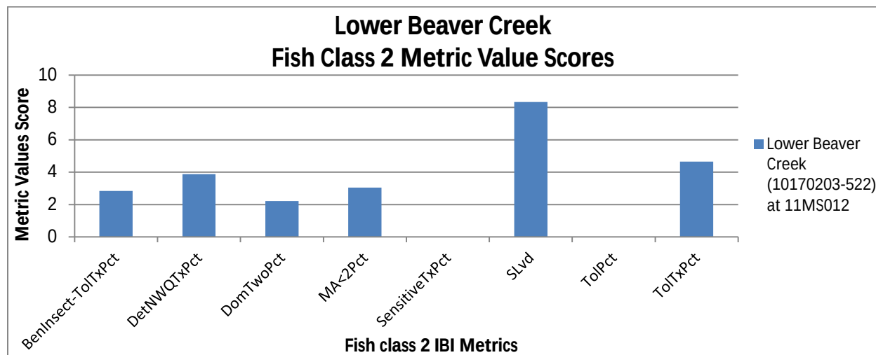
Figure 8: Fish class 2 IBI metric value scores along Lower Beaver Creek at site 11MS012
