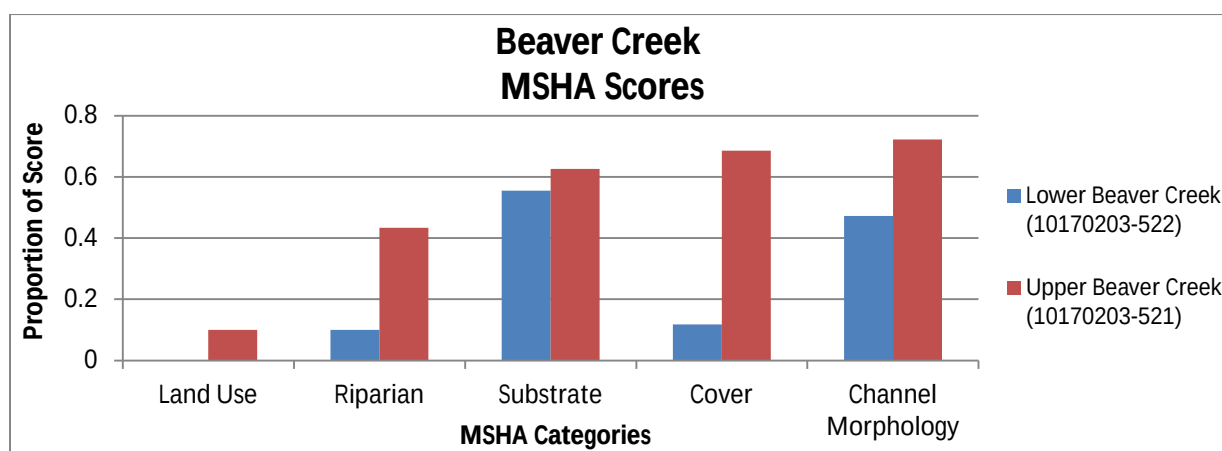
Figure 16: Proportion of scores of the MSHA categories along Upper and Lower Beaver Creek
