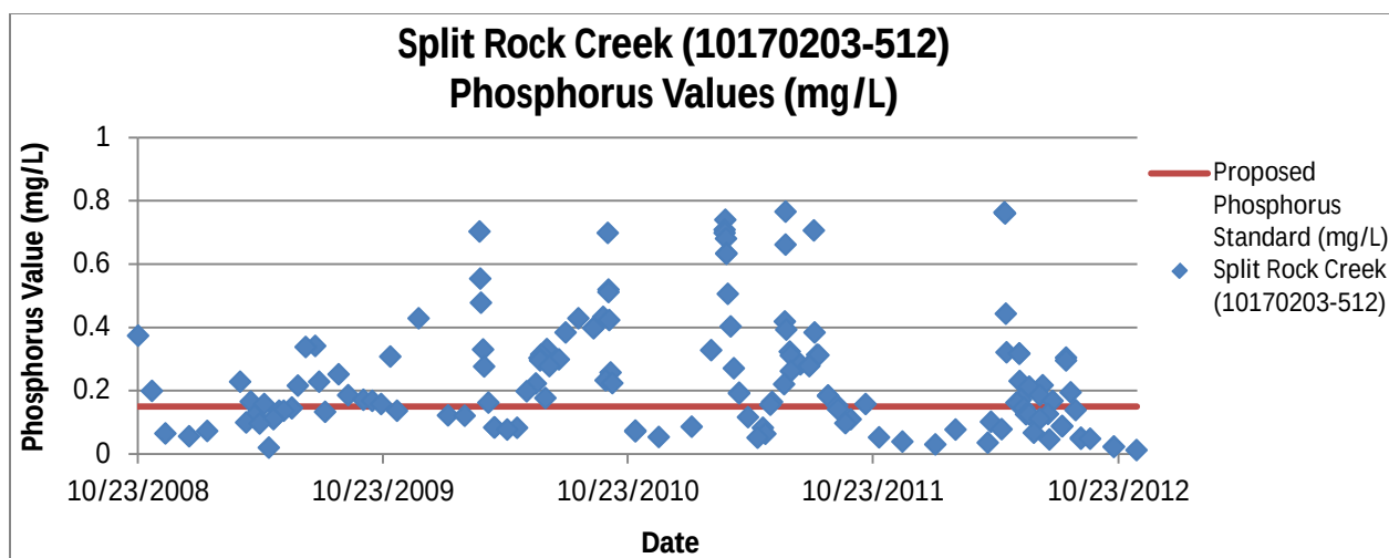
Figure 60: Phosphorus monitoring results from 2008-2012 along Split Rock Creek (10170203-512)
