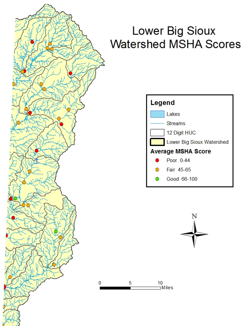
Figure 6: Average MSHA scores at biological sampling stations in the Lower Big Sioux River watershed
