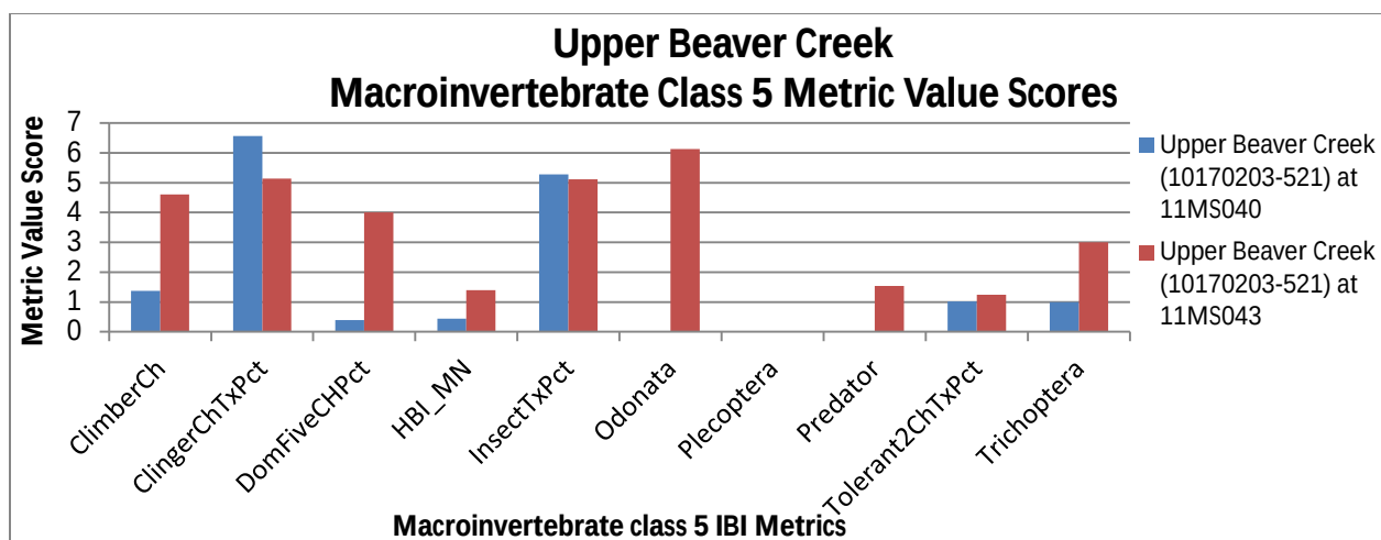
Figure 9: Macroinvertebrate class 5 metric value scores at the two sites in Upper Beaver Creek (10170203-521)
