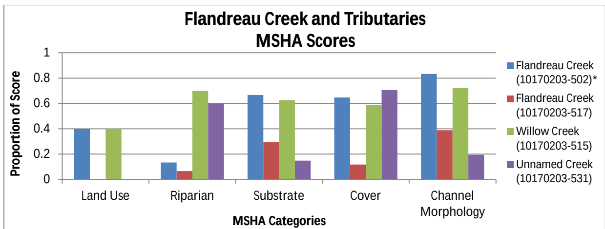
Figure 34: MSHA results from the biologically impaired reaches in the Flandreau Creek watershed *Average of two visits at 11MS005.
