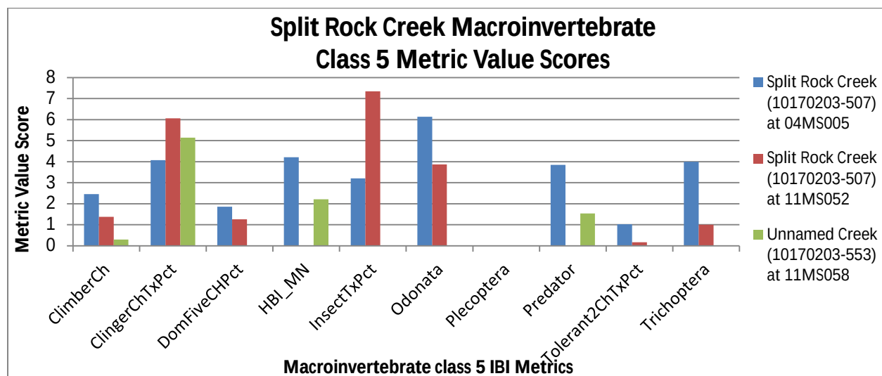
Figure 57: Macroinvertebrate class 5 metric value scores at three sites in the Split Rock Creek watershed
