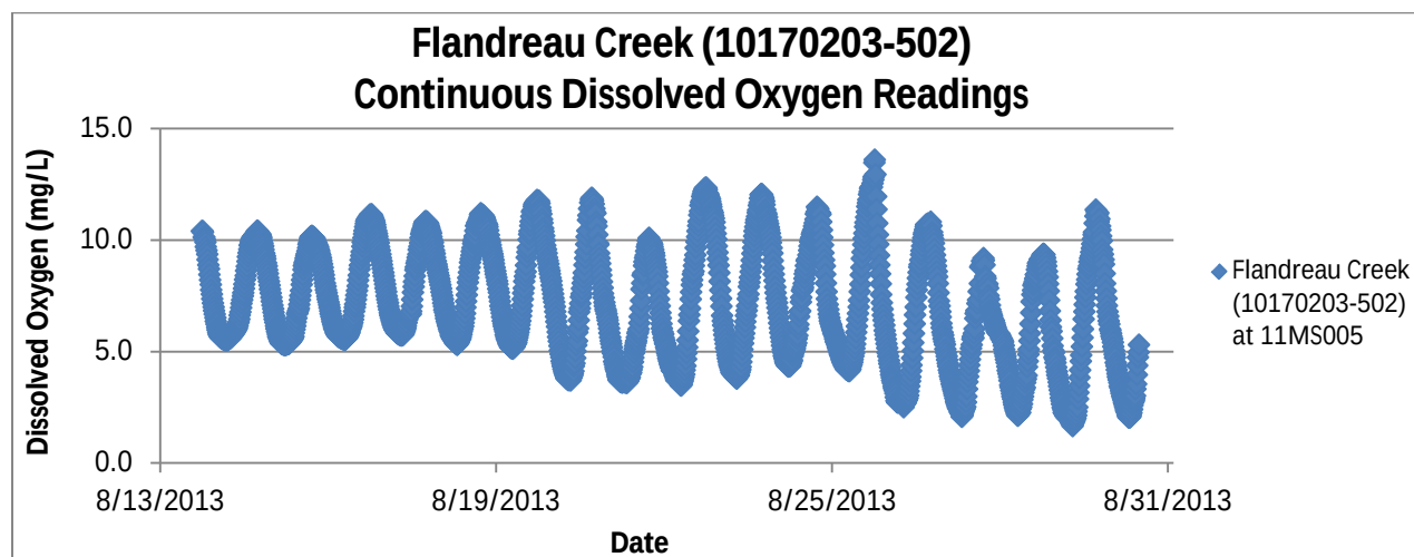
Figure 27: Continuous DO monitoring results from Flandreau Creek (10170203-502) at site 11MS005
