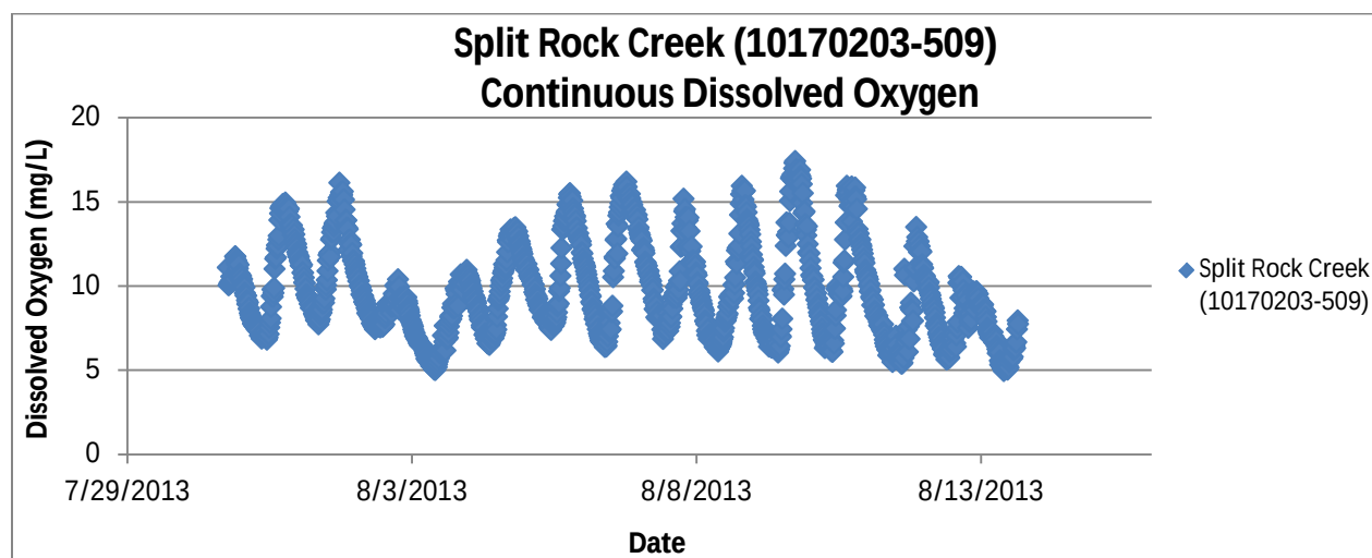
Figure 59: Continuous DO monitoring results at Split Rock Creek (10170203-509) in 2013
