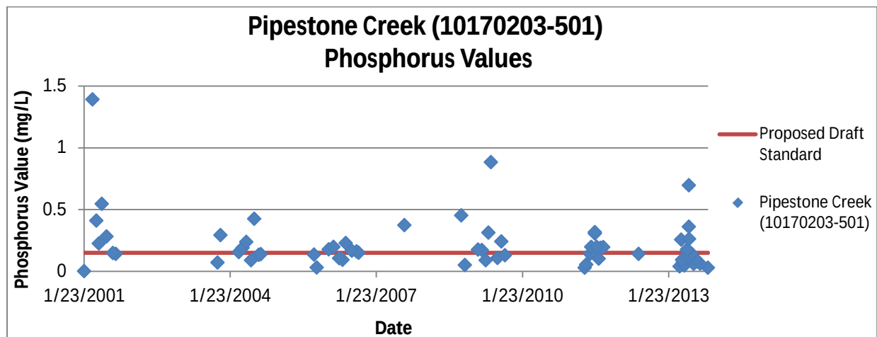
Figure 45: Pipestone Creek (10170203-501) phosphorus values from 2001-2013
