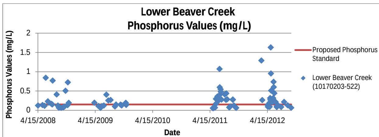
Figure 12: Phosphorus sample values from 2008-2012 along Lower Beaver Creek (10170203-522)
