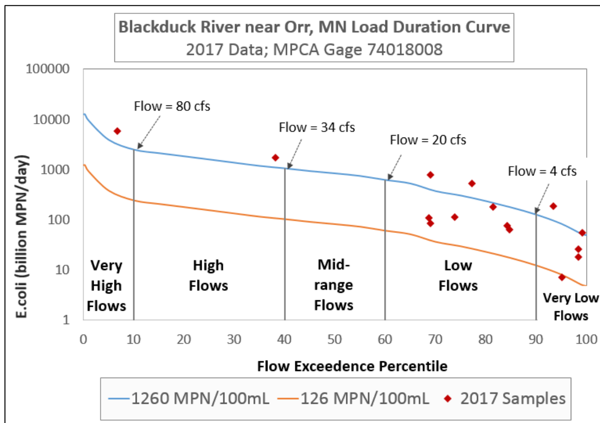
Figure 16. E.coli bacteria Load Duration Curve at the Blackduck River station B2c, year 2017. Target loads are shown for the two E.coli standards (individual and geometric mean). E.coli exceeds the target loads for all sampled flow regimes. No E.coli samples were collected for Mid-range flows.
