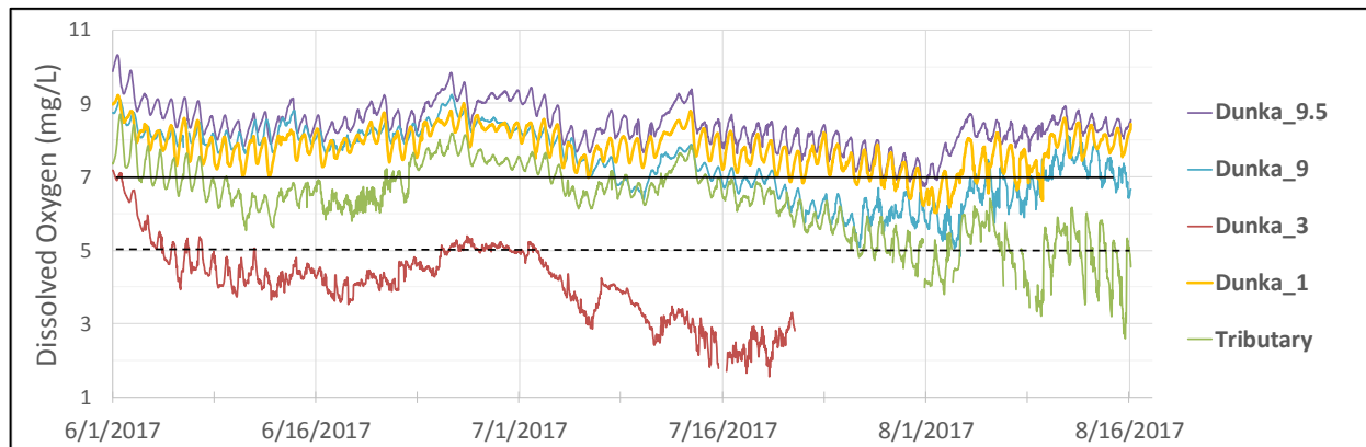
Figure 25. Continuous DO records collected in field season 2017 show the variability of DO in the Dunka River Watershed.
