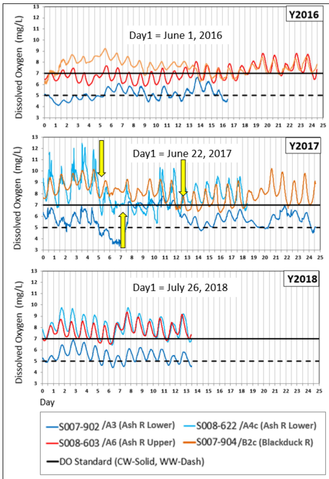
Figure 19. DO levels for reaches of the Ash River and Blackduck River, years 2016-2018.
