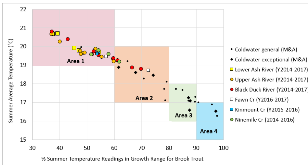
Figure 17. Plot of Summer Average Temperature vs. Percent of Summer Readings within the growth range for Brook Trout, a regionally native Coldwater trout species. Ash River Watershed stations are shown in colored markers, while all other Rainy River Headwater Watershed Coldwater stations collected during the Monitoring and Assessment (M&A) period are shown in black. Diamonds indicating streams with exceptional Coldwater communities.
