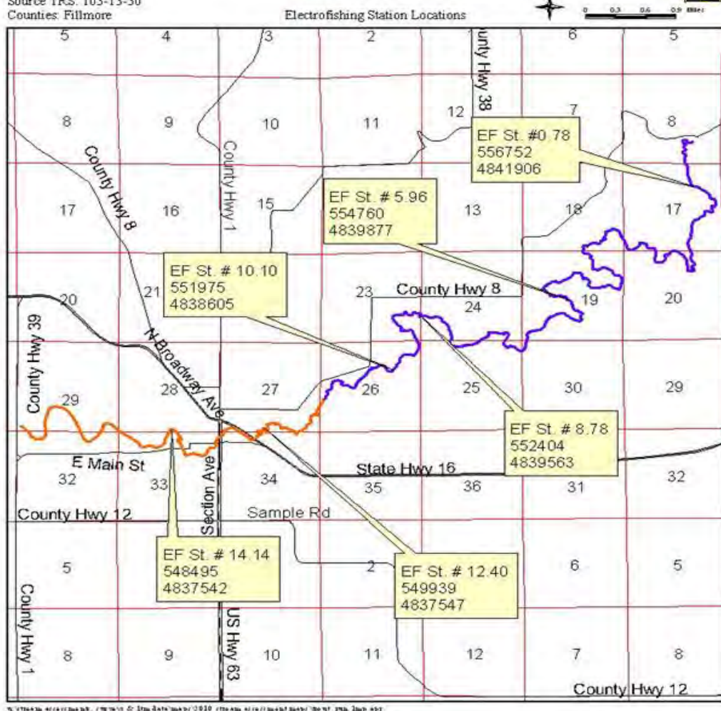
Figure 54. MDNR monitoring stations on Spring Valley Creek.
