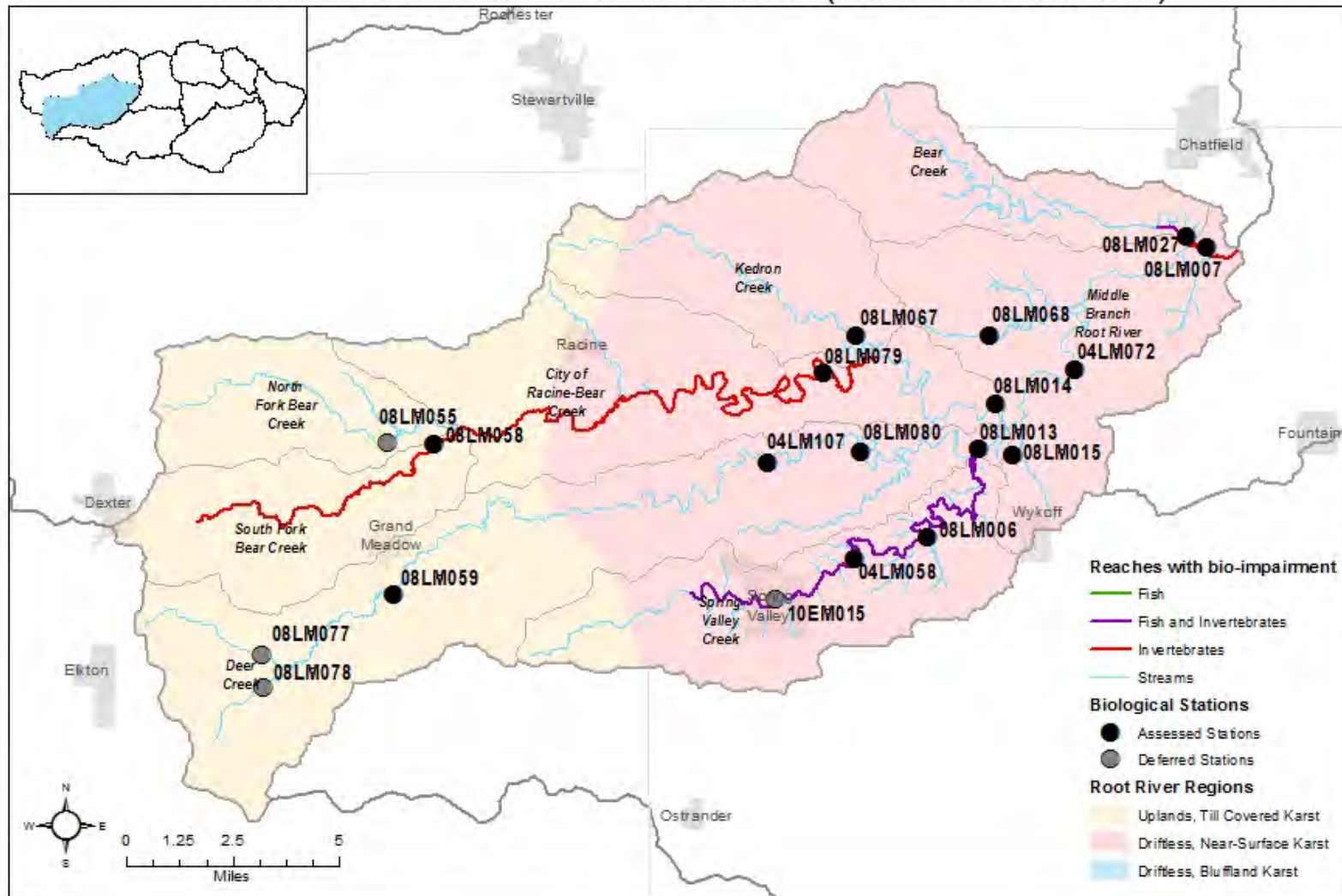
Figure 41. Map of the Middle Branch Root River watershed showing reaches of biological impairment and biological sampling locations
