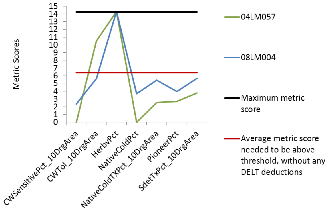
Figure 104. Metric scores for stations in Watson Creek of the Southern Coldwater fish IBI, with five point deduction for DELTs at Station 04LM057
