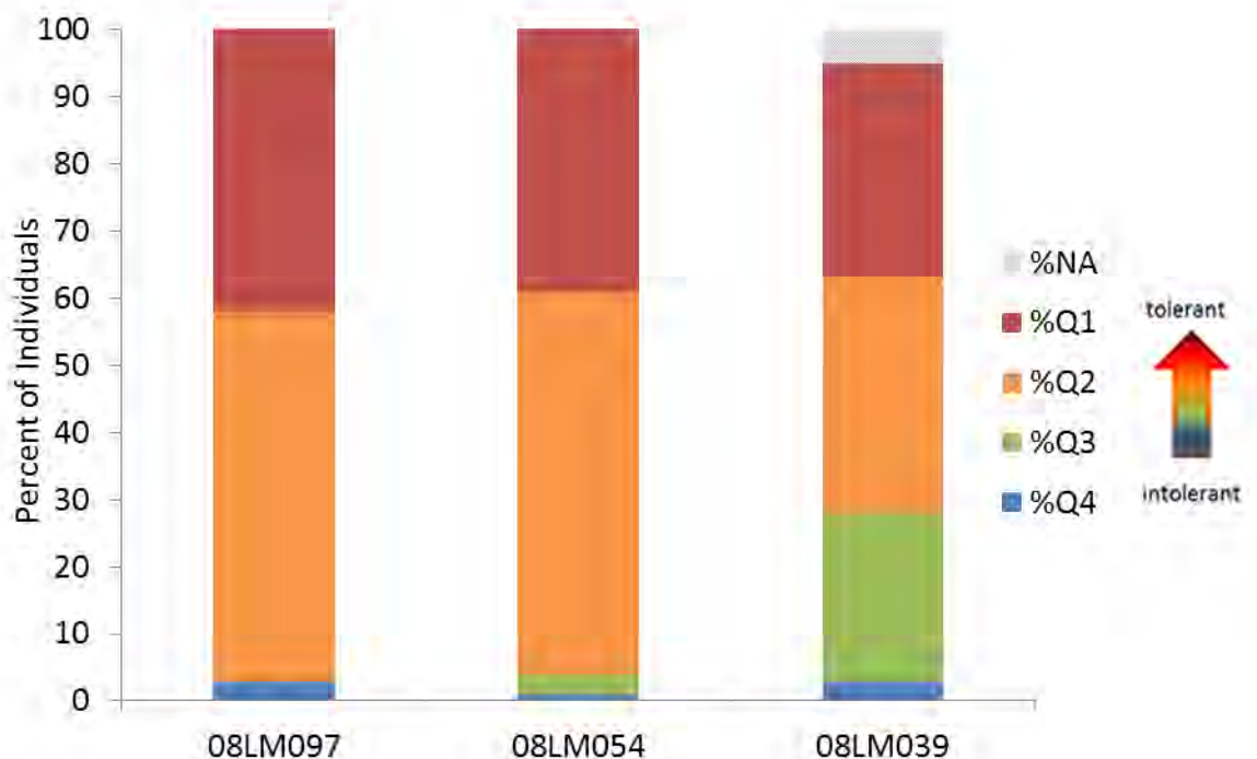
Figure 76. Fish DO TIV's for three biological stations on AUID 717.
