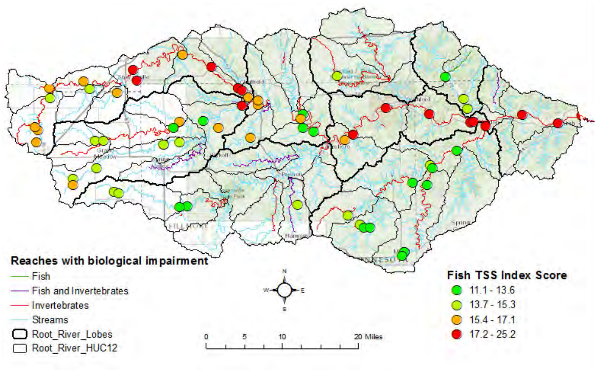
Figure 26. Station index scores for fish tolerance to TSS in the warmwater biological stations of the Root River Watershed; quartiled based on data shown. Note: This analysis is comparative among stations in the Root River only, and does directly translate to high TSS. This tool is used for understanding community composition, and species which are tolerant to high TSS, can also be responding to other stressors present.
