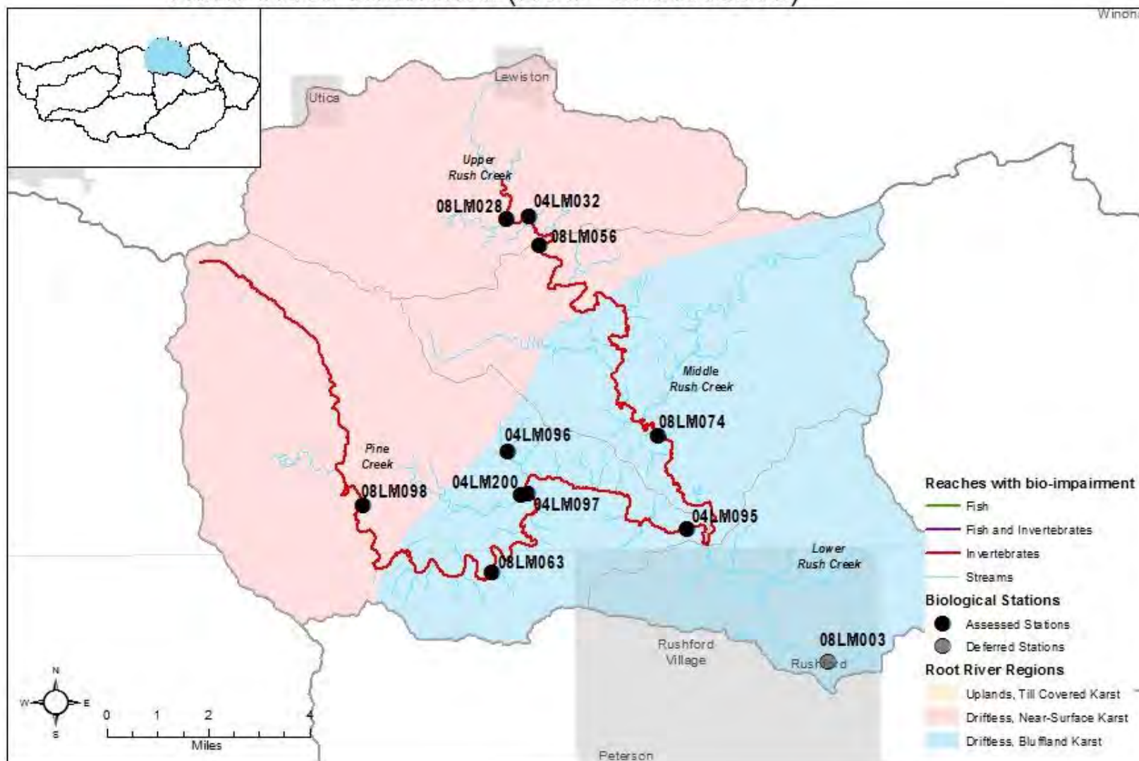
Figure 92. Rush Creek biological monitoring stations and aquatic life impairment
