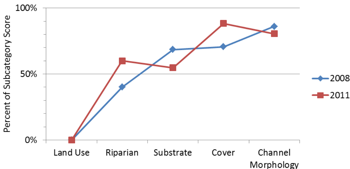
Figure 101. Percent of MSHA subcategory scores at Station 08LM026 in 2008 and 2011
