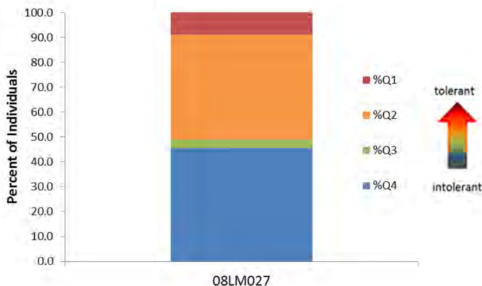
Figure 59. Fish DO TIV for Station 08LM027.
