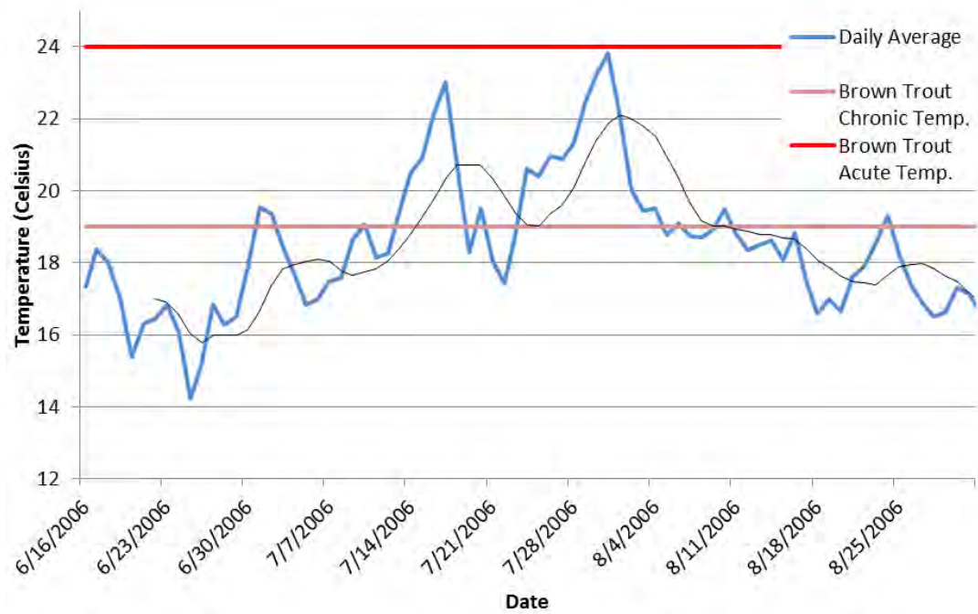
Figure 50. MDNR Station 5.95 (at 08LM006), daily average temperature with weekly average temperature.
