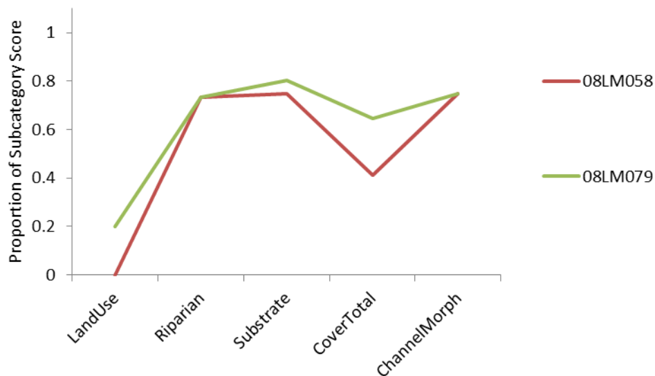
Figure 43. MSHA and subcategory scores for Bear Creek.
