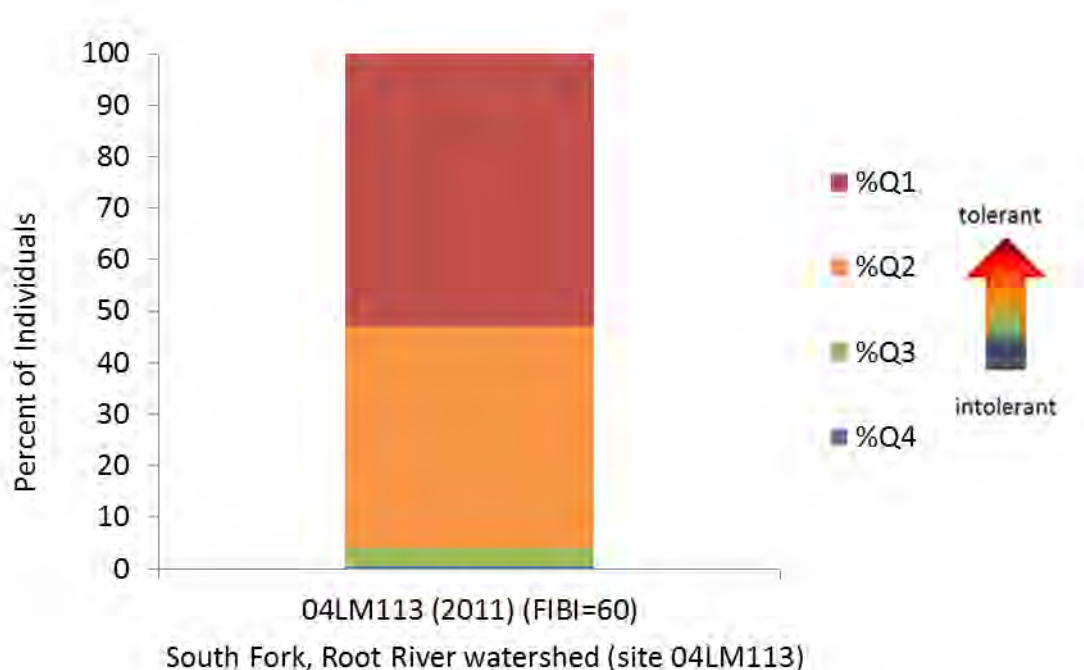
Figure 134. Dissolved oxygen tolerance indicator values for Station 04LM113 based on individuals present in fish community (2011).
