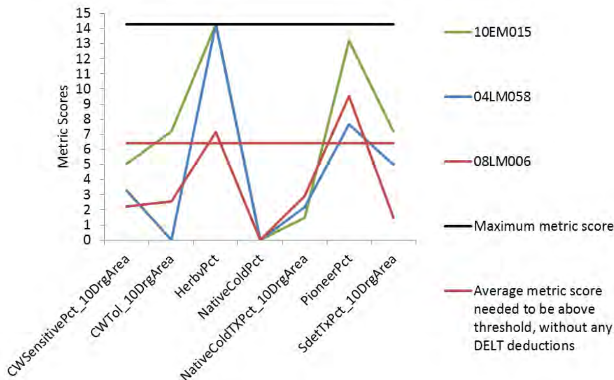
Figure 46. Fish IBI metric scores (Southern Coldwater IBI) for 3 stations in Spring Valley Creek.
