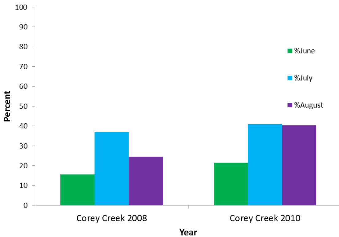
Figure 62. Corey Creek percent temperature measurements above 19°C, for Station 08LM018, 2008 and 2010.
