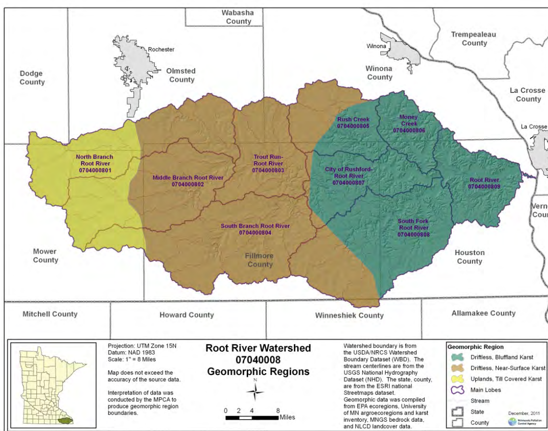
Figure 4. Three Root River Watershed Geomorphic Regions (GIS data used geomorphic data compiled by EPA ecoregions, the University of Minnesota agroecoregions, Minnesota Geological Survey (MGS) bedrock data, and NLCD land cover data).
