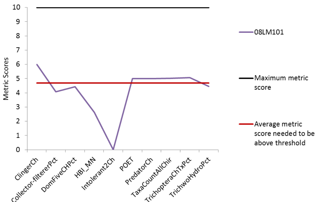
Figure 80. Metric scores for Station 08LM101 of the Southern Forest Streams GP macroinvertebrate IBI
