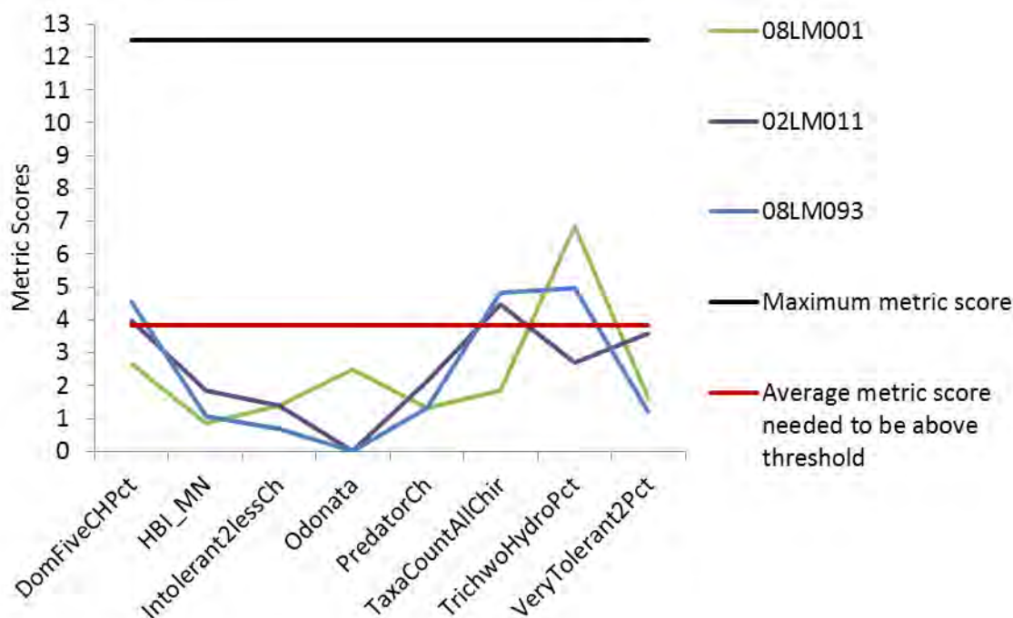
Figure 85. Metric scores for stations in Root River (AUID 501 and 502) of the Prairie Forest Rivers macroinvertebrate IBI
