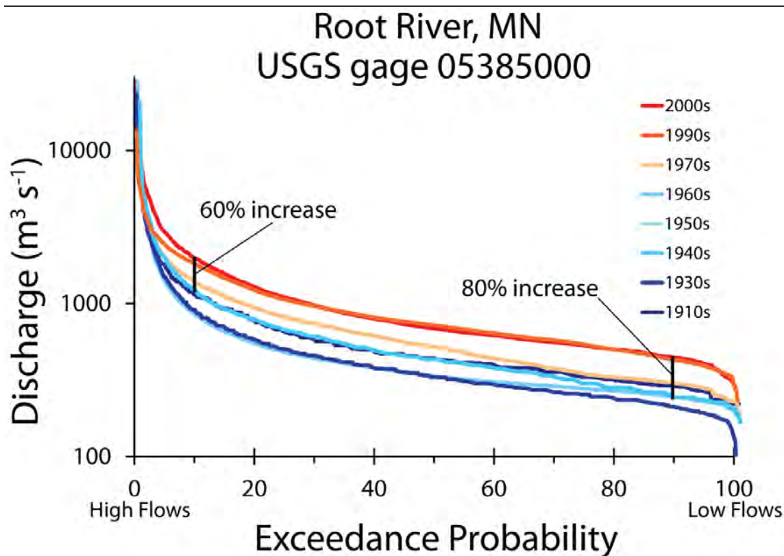
Figure 18. Discharge analysis from the Root River near Houston, (Belmont, 2011)
