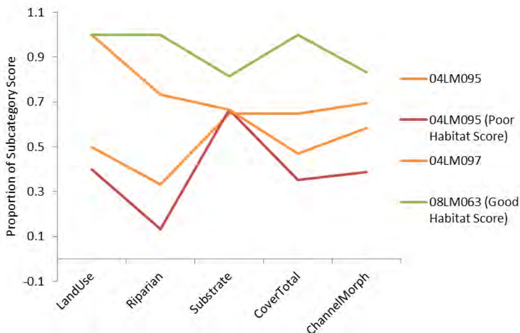
Figure 95. Pine Creek MSHA and subcategory scores.
