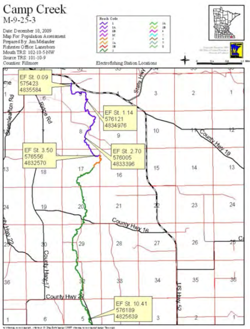
Figure 117. MDNR sectors of Camp Creek
