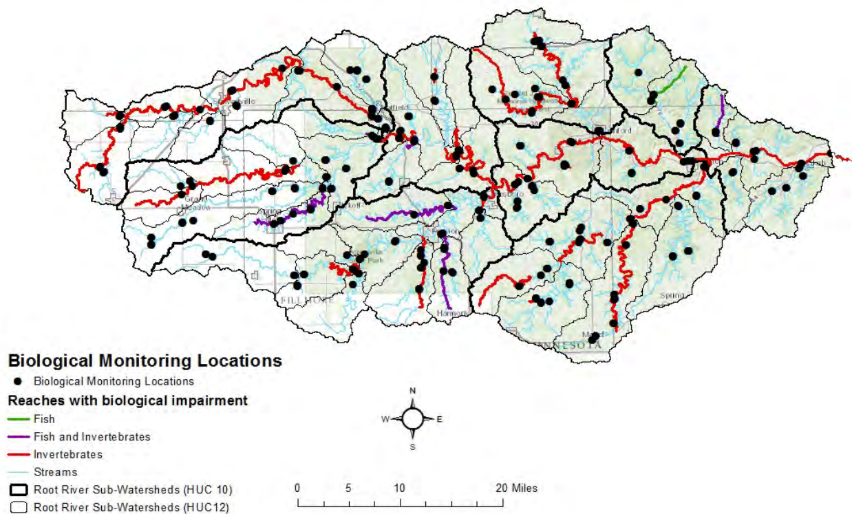
Figure 15. Biological monitoring locations and reaches with identified biological impairment in the Root River.
