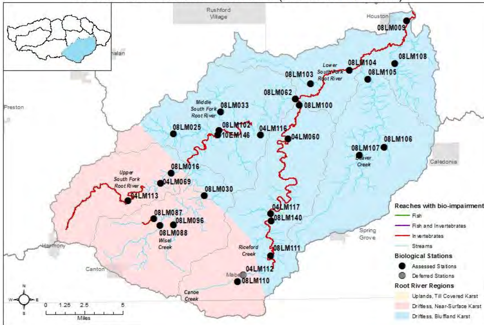
Figure 121. South Fork Root River biological monitoring stations and aquatic life impairments
