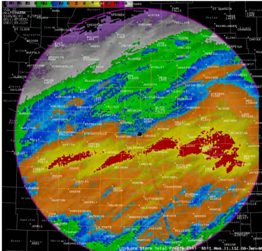
Figure 13. Two-day radar rainfall estimates from Saturday the 7th through Monday morning (the 9th), June 2008 National Weather Service (NWS).
