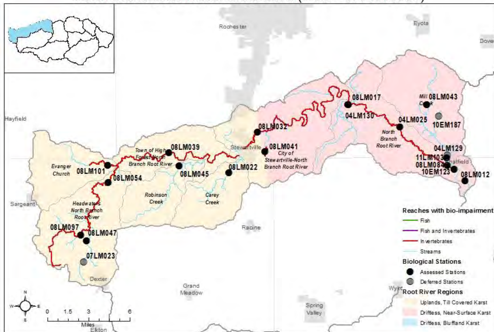
Figure 67. Map of the North Branch Root River Watershed showing reaches of biological impairment and biological sampling locations
