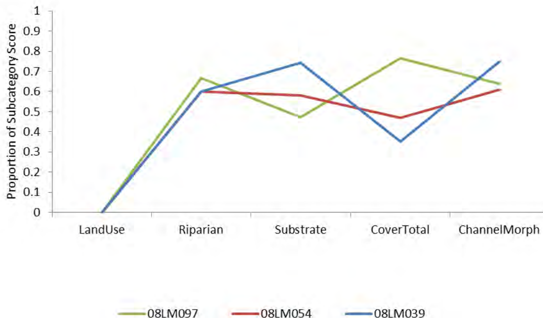
Figure 77. MSHA and subcategory scores for Stations in the North Branch Headwaters
