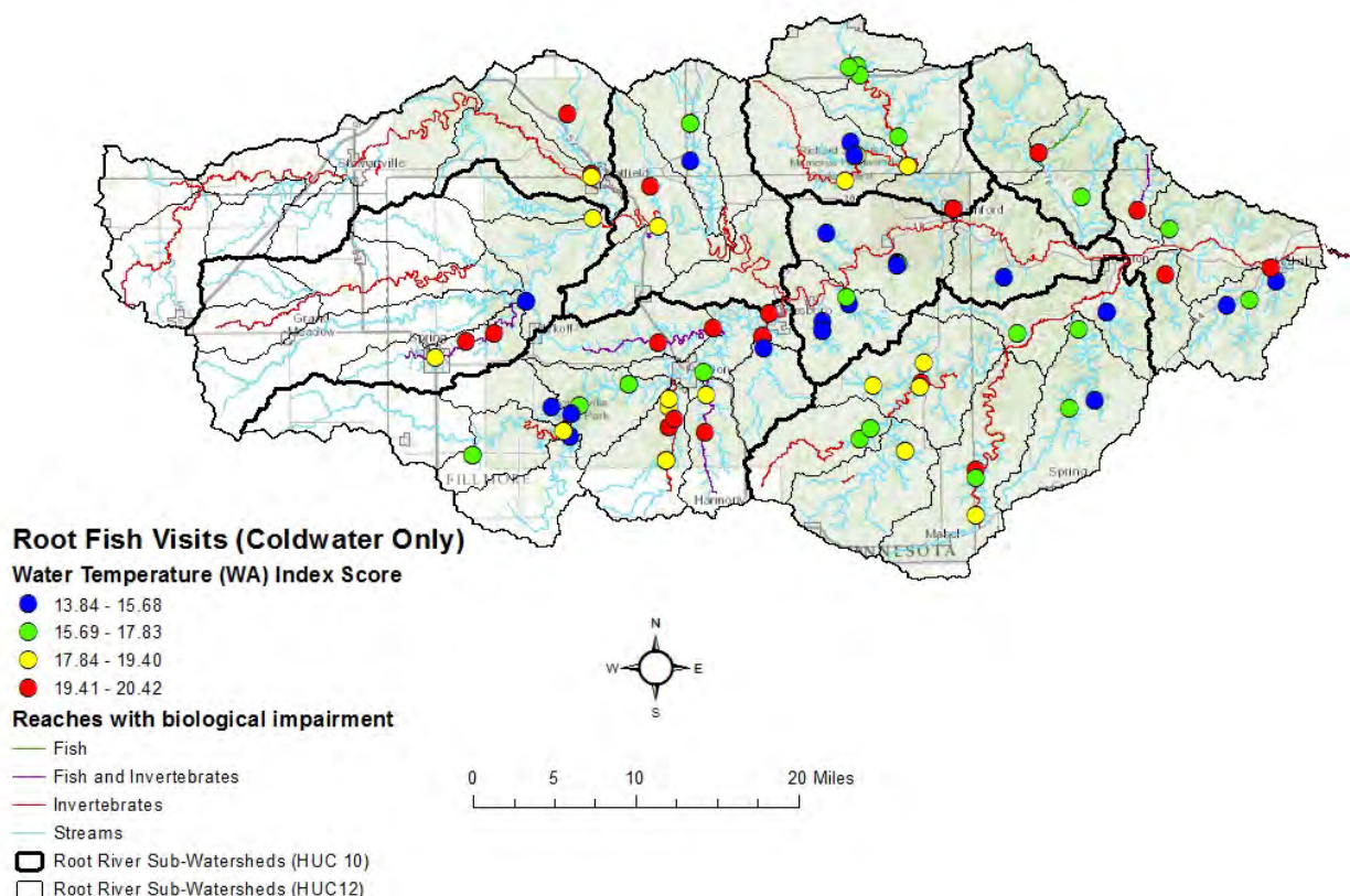
Figure 19. Water temperature index scores (WA-weighted averages) for Coldwater stations in the Root River quartiled based on data shown.
