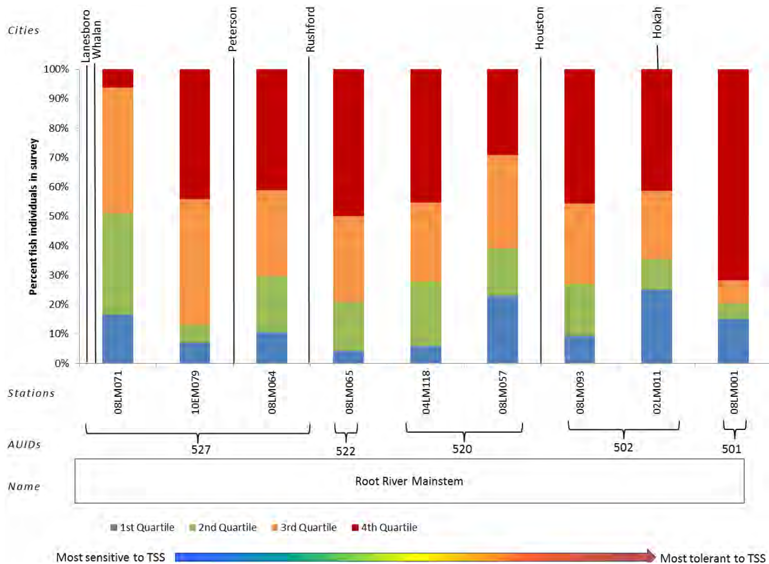
Figure 36. Root River mainstem fish TSS TIV's (tolerance indicator values) from Lanesboro to mouth, demonstrating fish community composition and overall tolerance to TSS.
