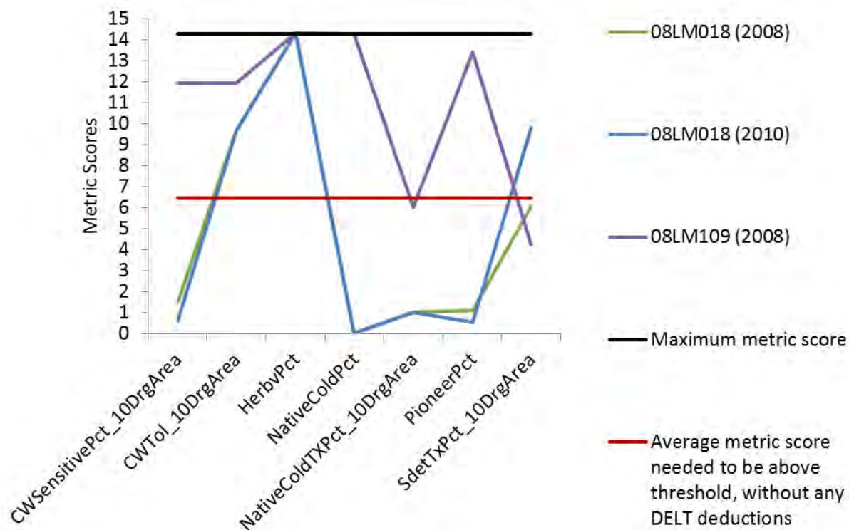
Figure 61. Metric scores for stations in Corey Creek and Campbell Creek of the southern coldwater fish IBI, with no deductions for DELTs Corey Creek
