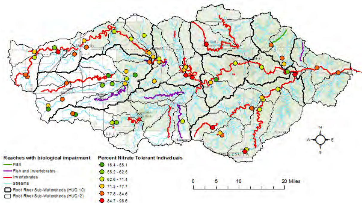
Figure 25. Map of the percent nitrate tolerant macroinvertebrate individuals in warmwater stations in the Root River Watershed
