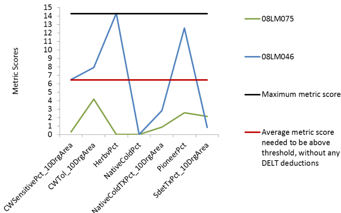
Figure 115. Metric scores for stations in Camp Creek of the Southern Coldwater fish IBI, with no deductions for DELTs
