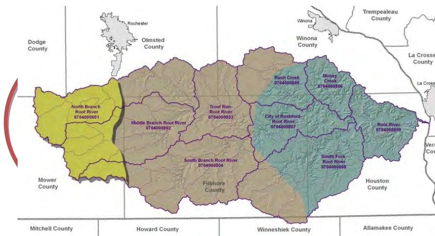
Figure 5. Upland zone highlighted
