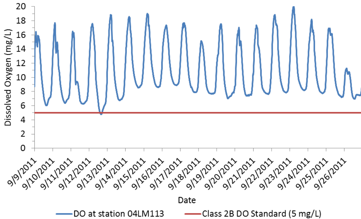
Figure 132. Diurnal DO data from Station 04LM113, September 9 - 26, 2011
