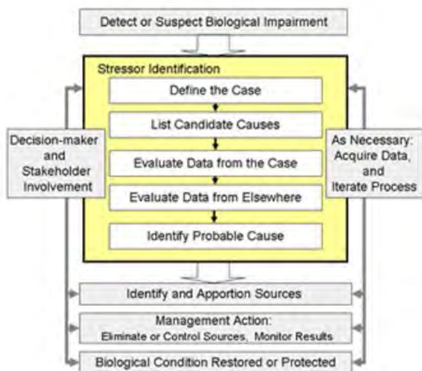
Figure 1. Conceptual model of Stressor Identification process (Cormier et al. 2000).
