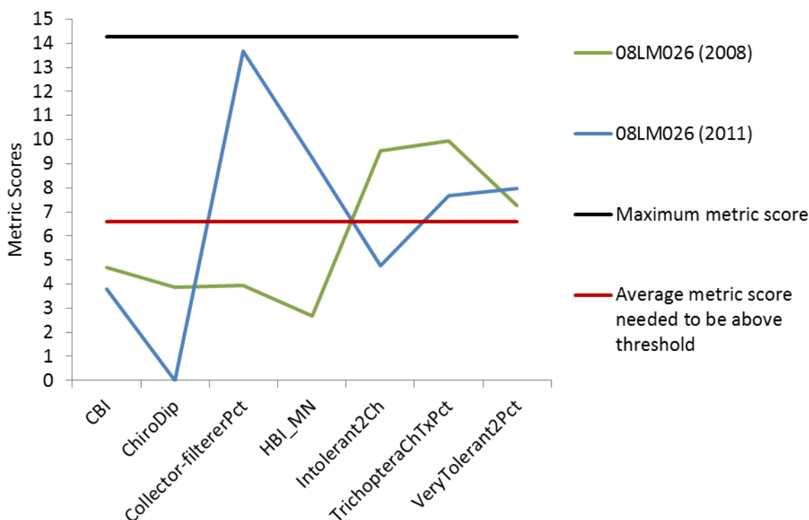
Figure 100. Metric scores for stations in Etna Creek of the Southern Coldwater macroinvertebrate IBI
