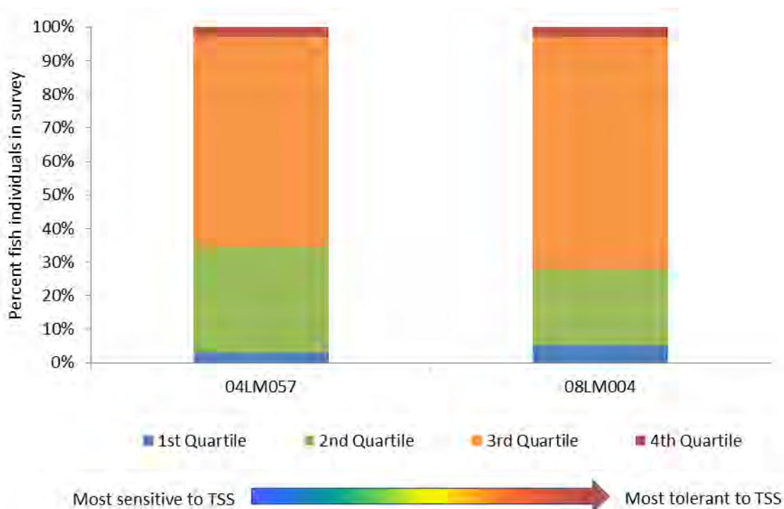
Figure 108. Watson Creek fish TSS TIV's (tolerance indicator values) at Stations 04LM057 and 08LM004
