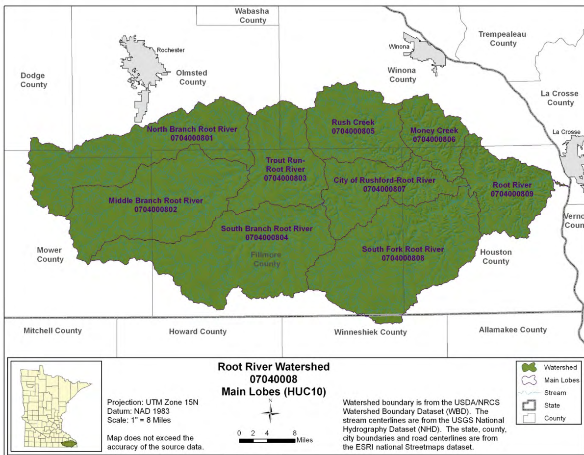
Figure 3. Root River Watershed 10 digit HUC subwatersheds.
