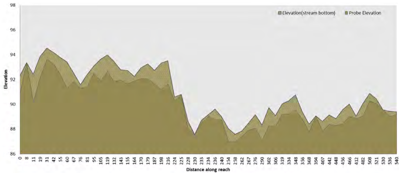
Figure 79 Station 08M054 longitudinal profile and sediment deposition
