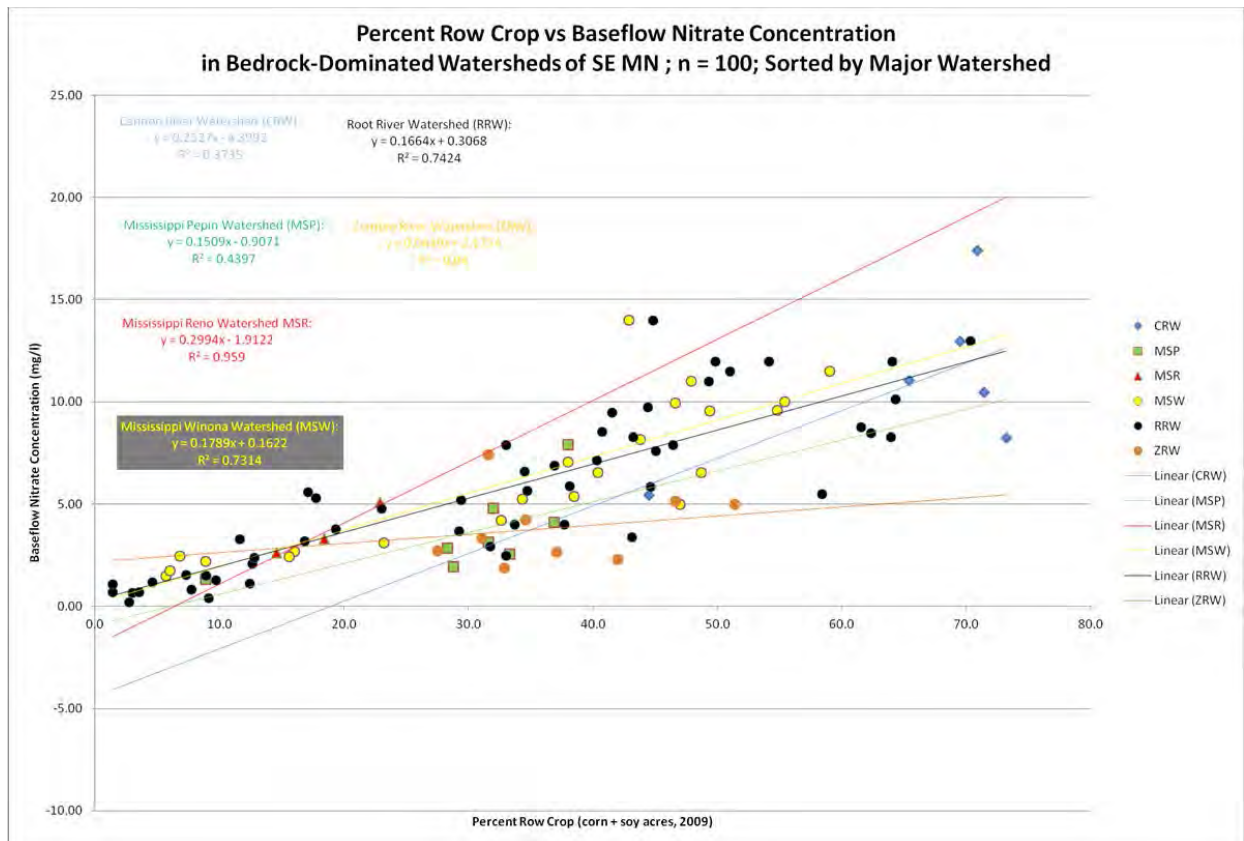
Figure 23. Nitrate concentration vs row crop percentage in southeastern Minnesota (Watkins et al.)
