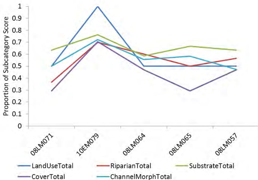
Figure 37: MSHA scores for sites by subcategory for biological stations on AUIDs 520, 522 and 527.
