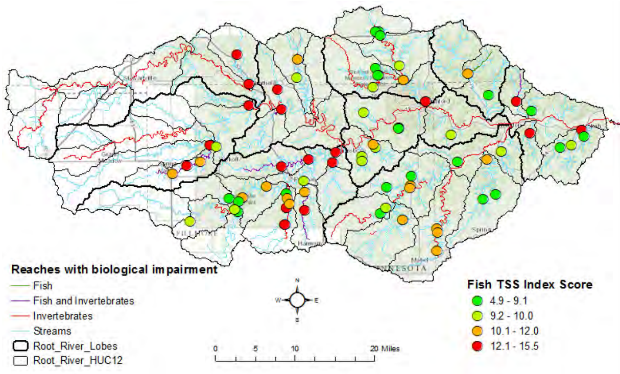
Figure 27. Station index scores for fish tolerance to TSS in the coldwater biological stations of the Root River Watershed; quartiled based on data shown. Note: This analysis is comparative among stations in the Root River only, and does directly translate to high TSS. This tool is used for understanding community composition, and species which are tolerant to high TSS, can also be responding to other stressors present.
