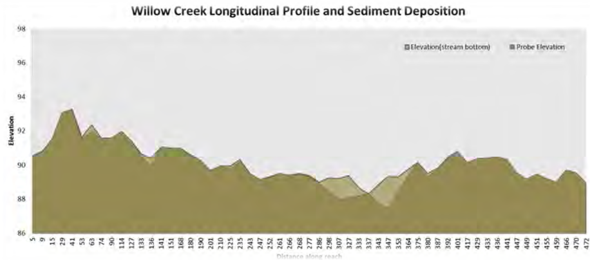
Figure 113. Sediment deposition (shown in light brown) in pools on longitudinal profile, Willow Creek-10EM143.
