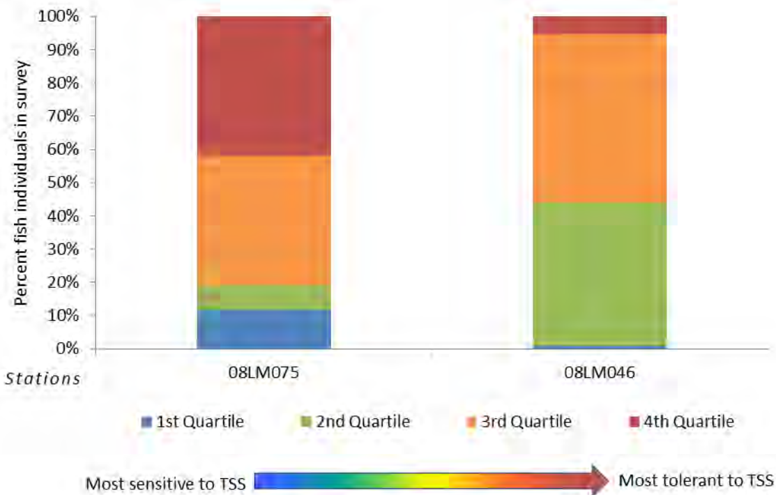
Figure 120. Camp Creek fish TIV's (tolerance indicator values)
