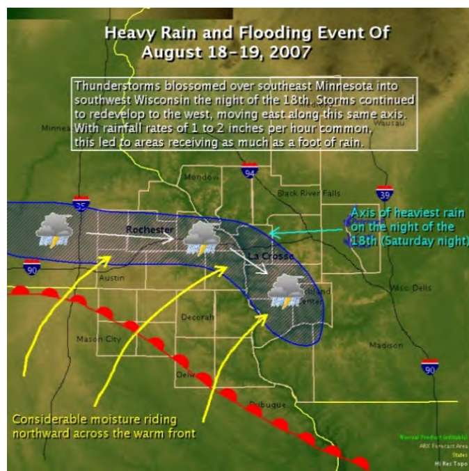
Figure 14. Location of heaviest rain from August 18, 2007 (NWS)
