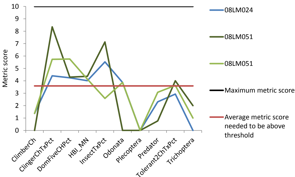
Figure 150. Metric scores for stations in Wadden Valley Creek and Money Creek of the Southern Streams RR macroinvertebrate IBI
