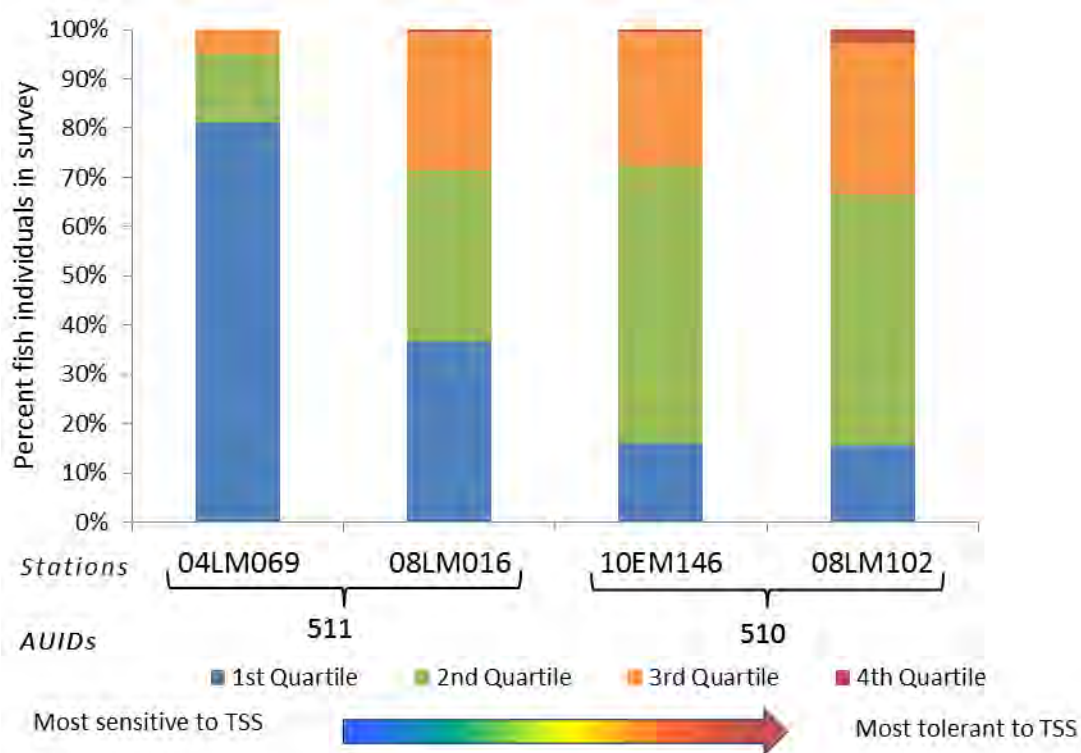
Figure 124: TSS TIV for Coldwater stations in the South Fork Root
