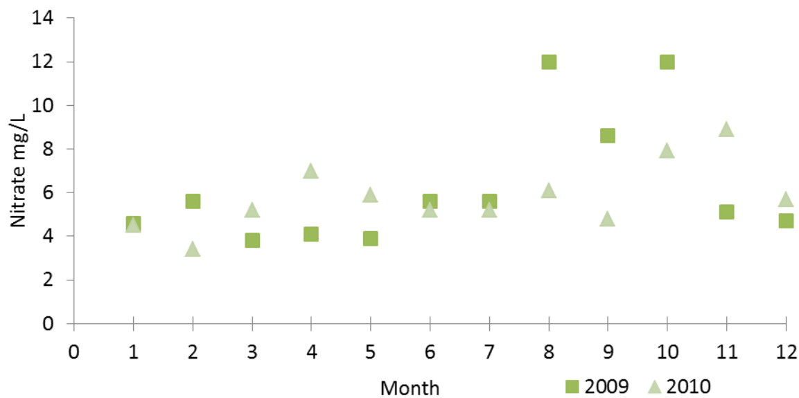
Figure 149. Nitrate concentration ranges from 2009 and 2010 at Station S004-842 (Pilot Mount monitoring station).
