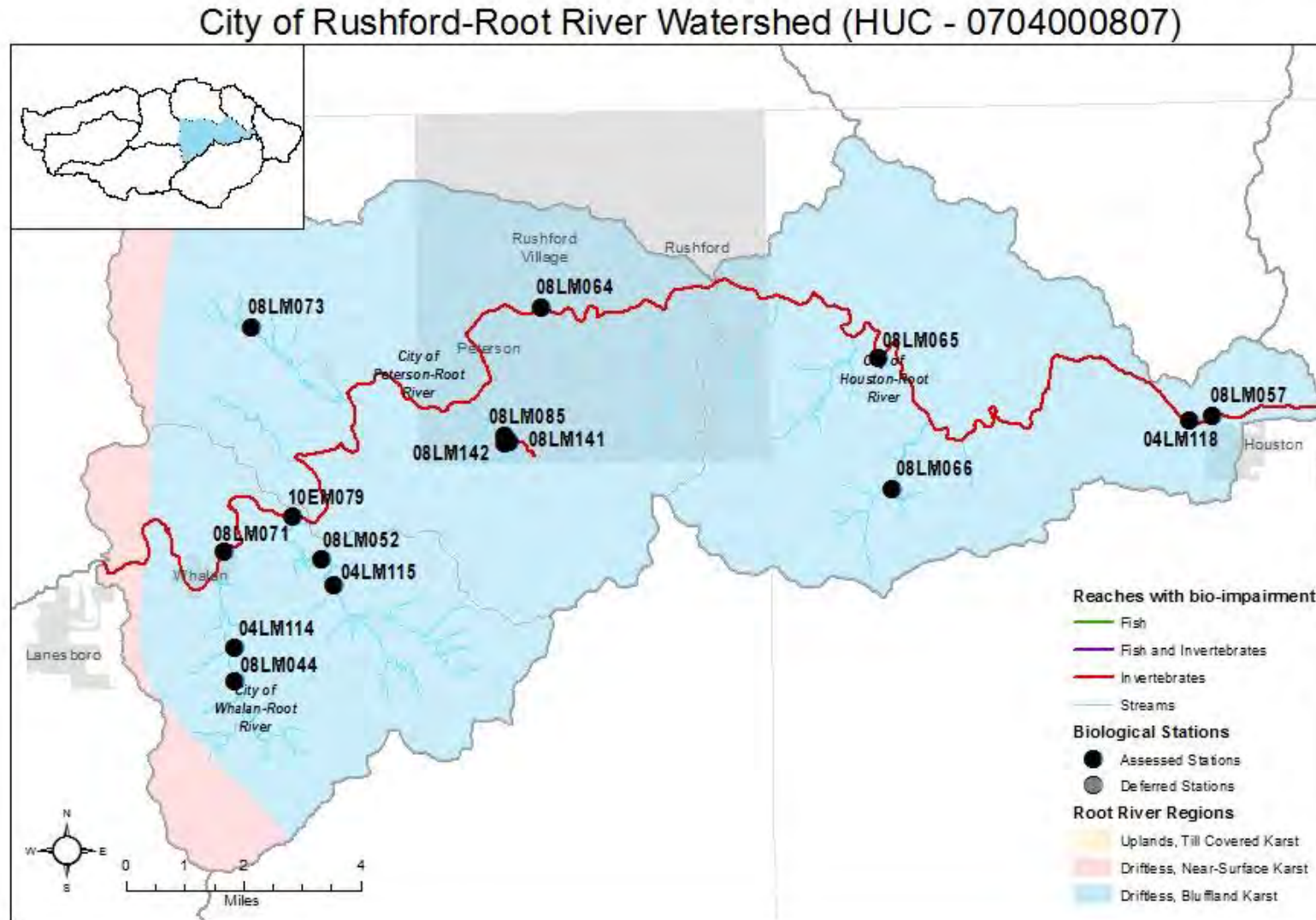
Figure 34. Map of City of Rushford-Root River watershed showing reaches of biological impairment and biological sampling locations
