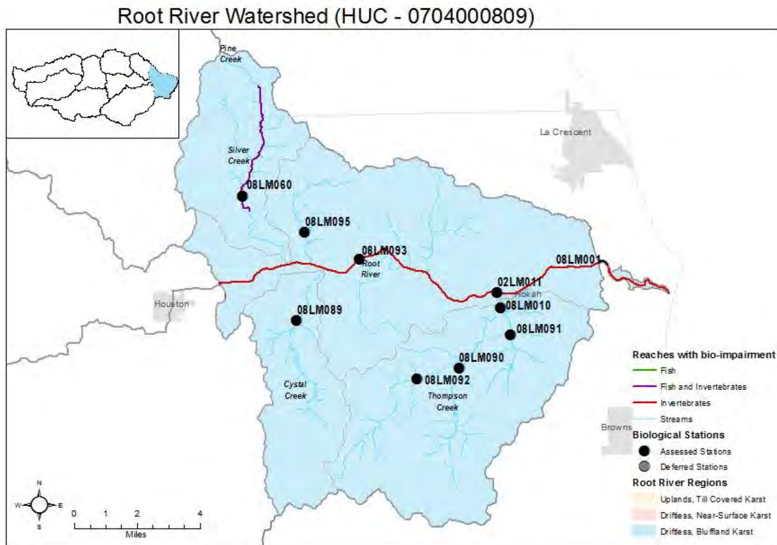
Figure 84. Map of Root River 10 HUC, showing reaches of biological impairment and biological sampling locations
