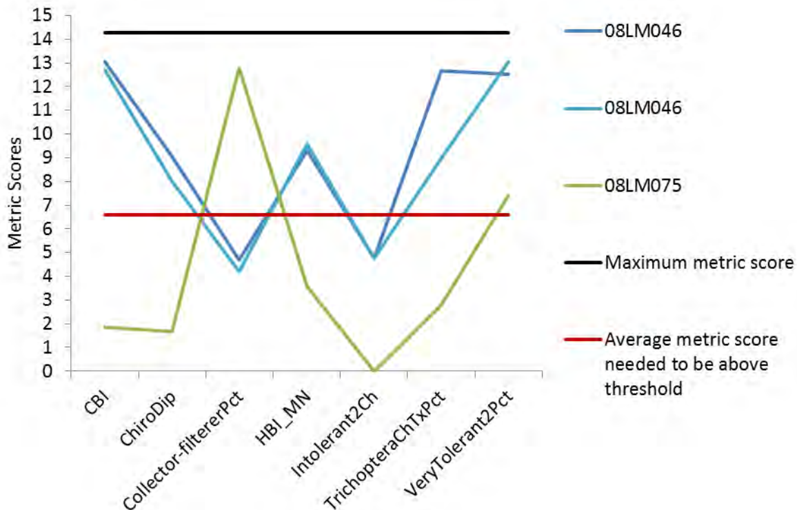
Figure 116. Metric scores for stations in Camp Creek of the Southern Coldwater macroinvertebrate IBI.
