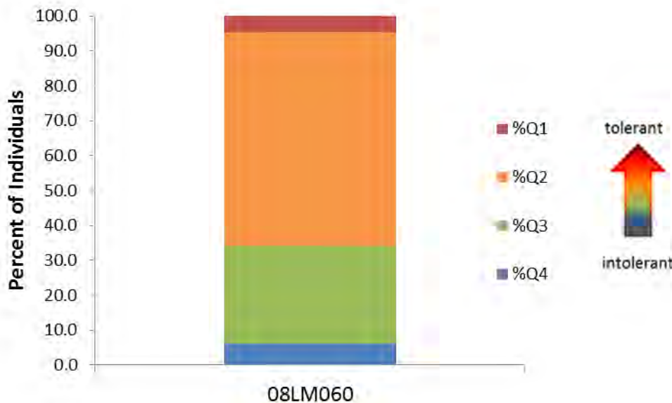
Figure 90: DO TIV for fish at Station 08LM060.
