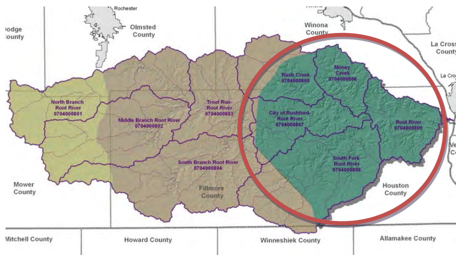
Figure 11. Driftless bluffland Karst zone
