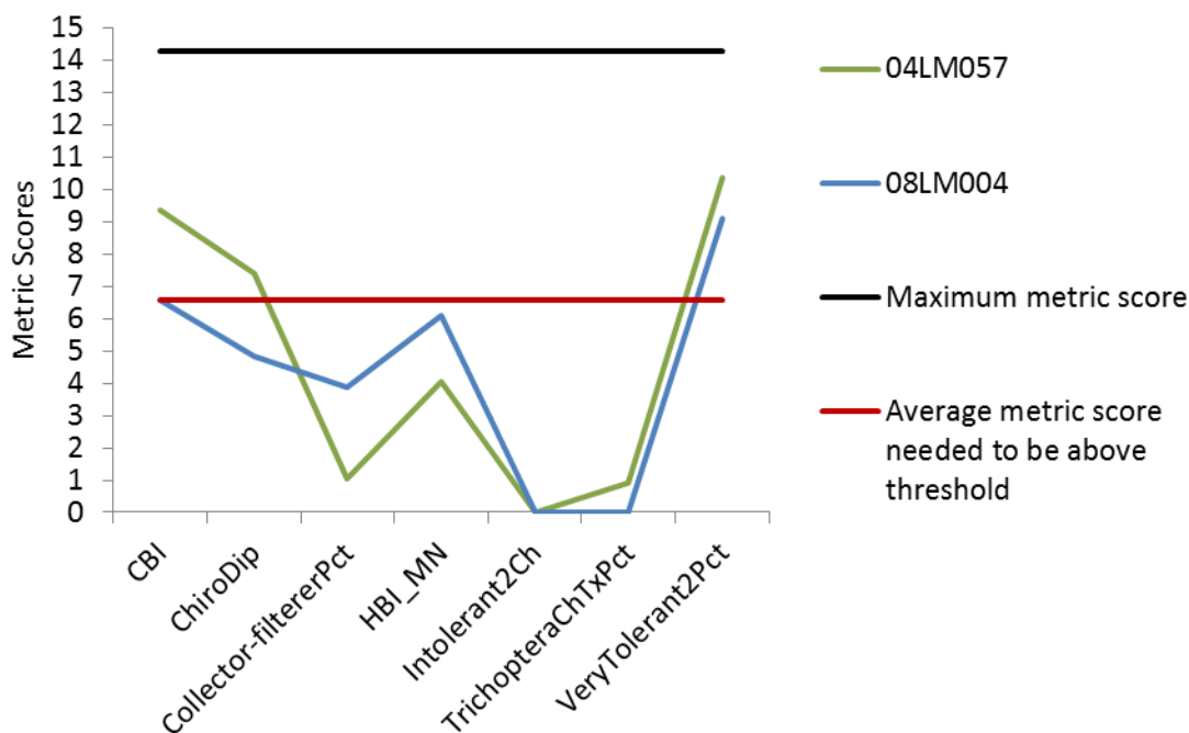
Figure 103. Metric scores for stations in Watson Creek of the Southern Coldwater macroinvertebrate IBI
