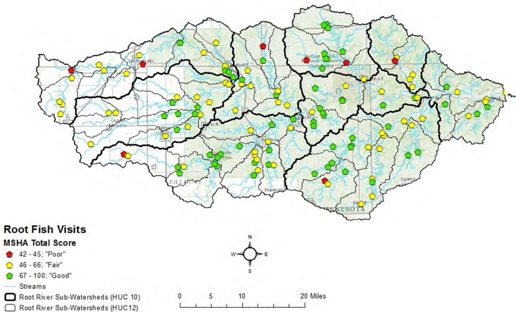
Figure 31. Root River MSHA scores for each biological station
