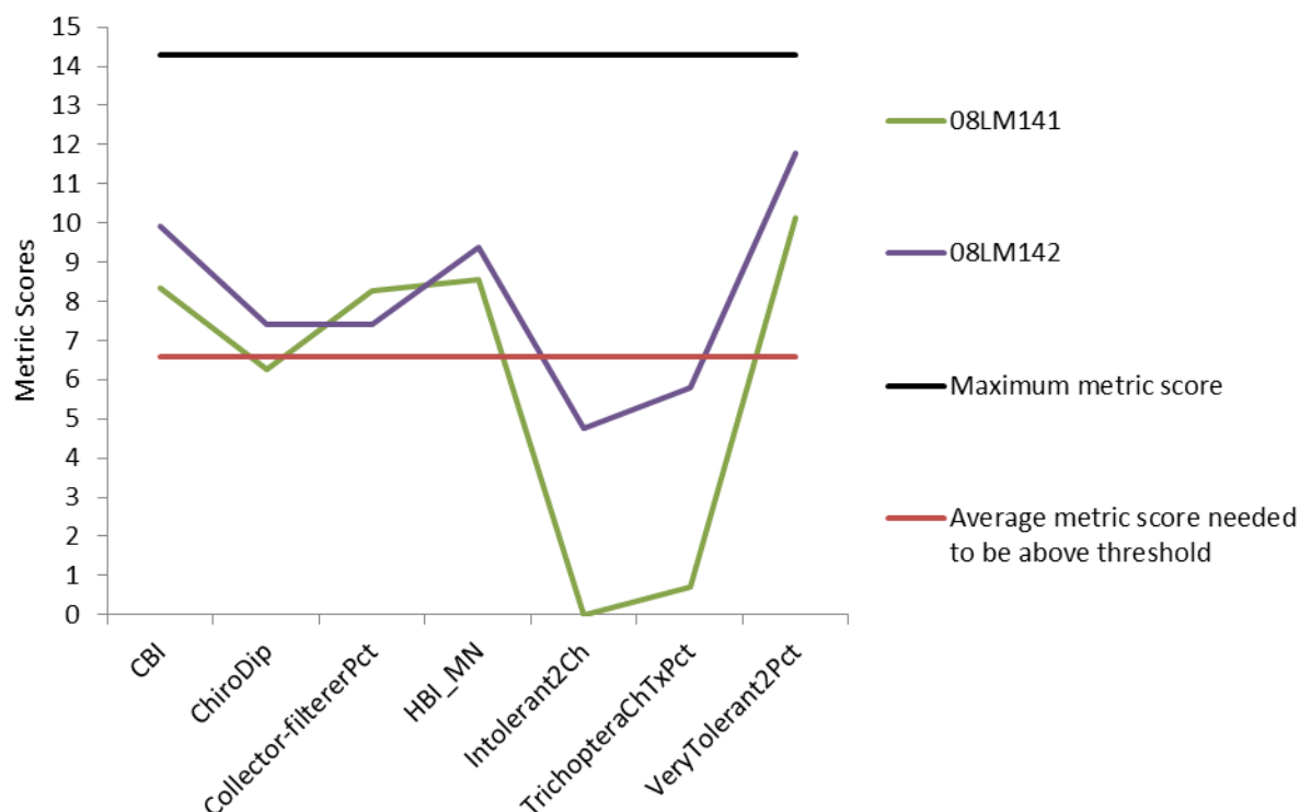
Figure 38. Metric scores for stations in the Camp Hayward Creek Watershed of the Southern Coldwater macroinvertebrate IBI
