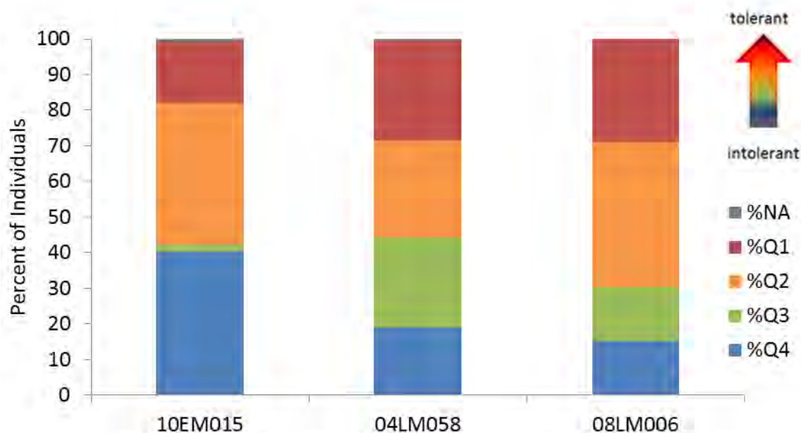
Figure 52. Fish community tolerance to low DO at three stations in Spring Valley Creek.
