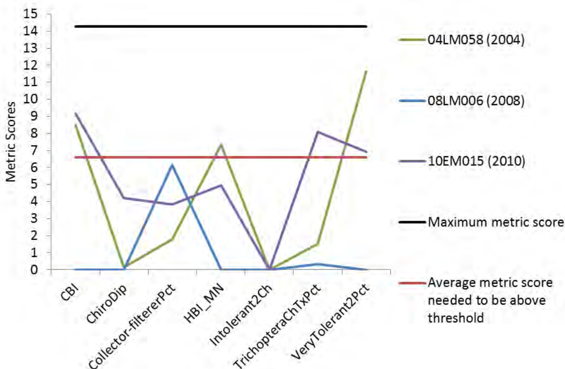
Figure 45. Metric scores for stations in Spring Valley Creek of the Southern Coldwater macroinvertebrate IBI.
