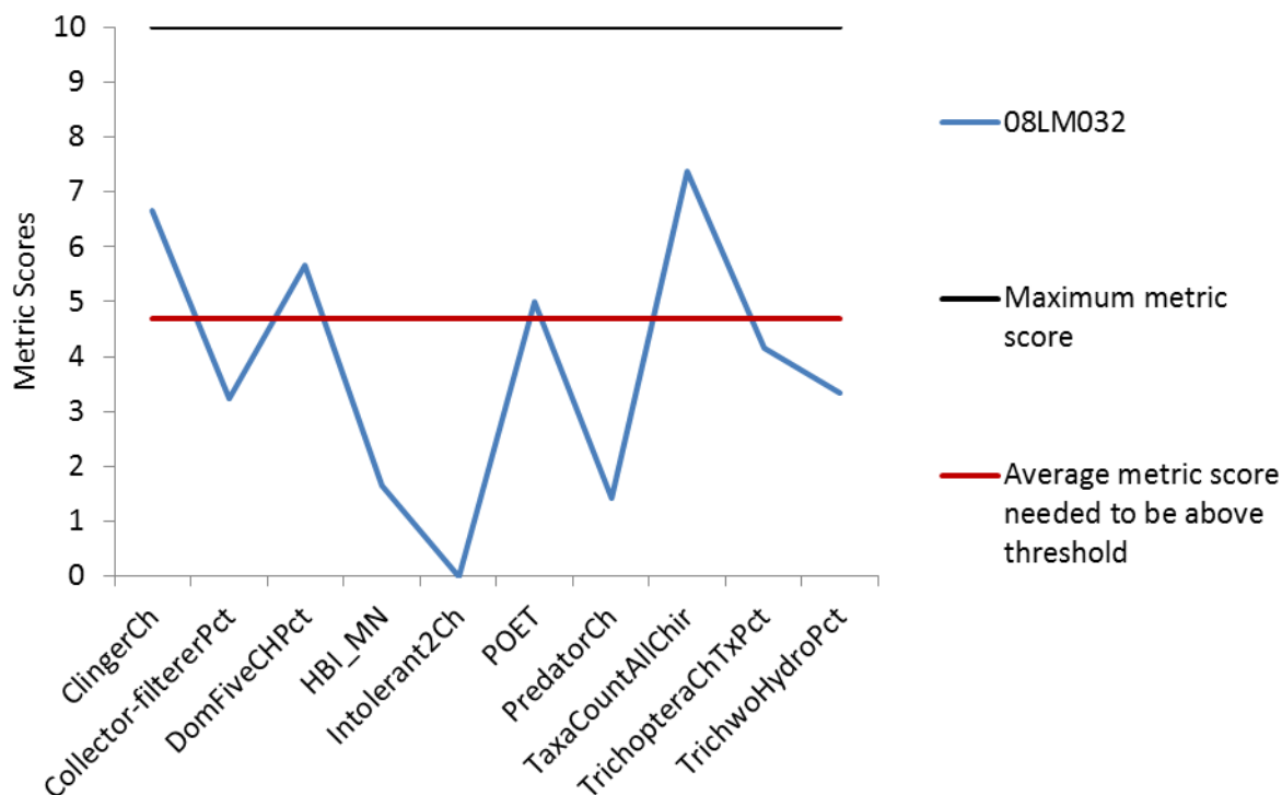
Figure 69. Metric scores for stations of MIBI Class 6, Southern Forest GP (716)
