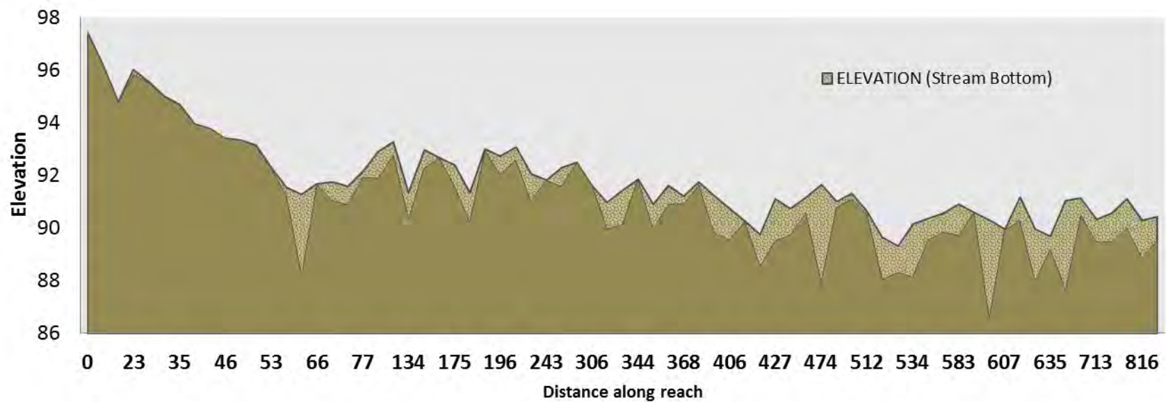
Figure 64. Graph of longitudinal profile geomorphology data demonstrating substrate embeddedness and sediment deposition in Corey Creek
