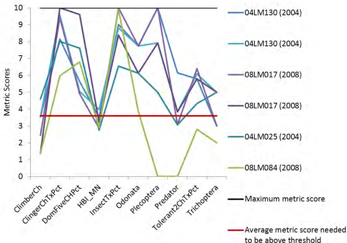
Figure 68. Metric scores for stations of MIBI Class 5, Southern Forest RR (716)
