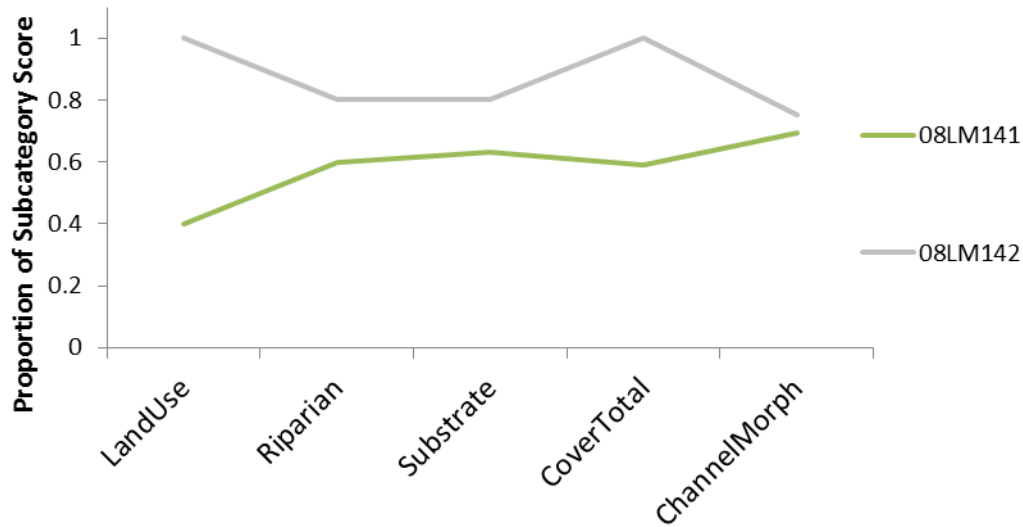
Figure 39. Components of the MSHA comparison for 08LM141 and 08LM142.
