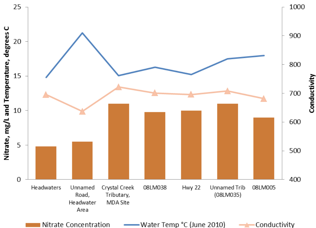
Figure 111. Willow Creek longitudinal nitrate concentration with conductivity and water temperature, June 9, 2010
