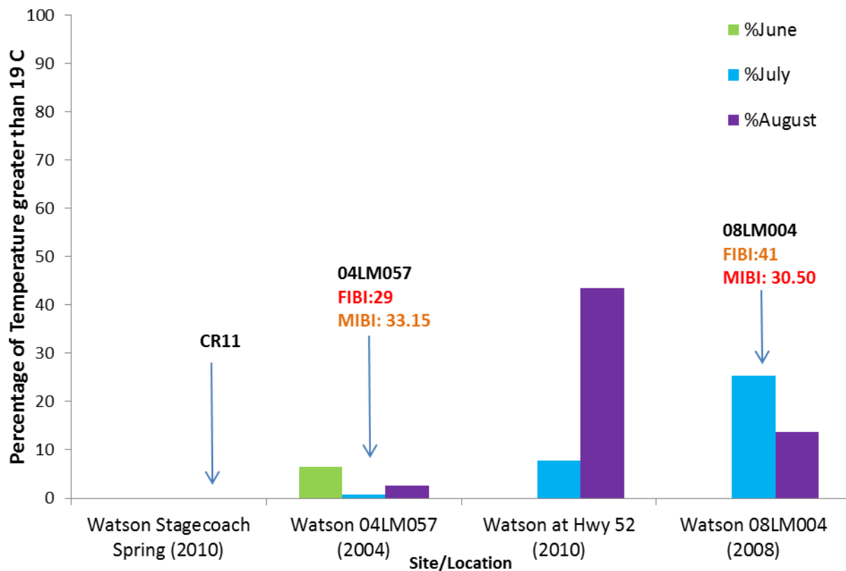
Figure 105. Watson Creek percentage of temperature measurements above 19°C, at 4 locations.
