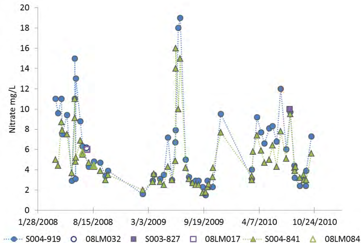
Figure 70. Range of nitrate concentrations from 2008-2010 on AUID 716.
