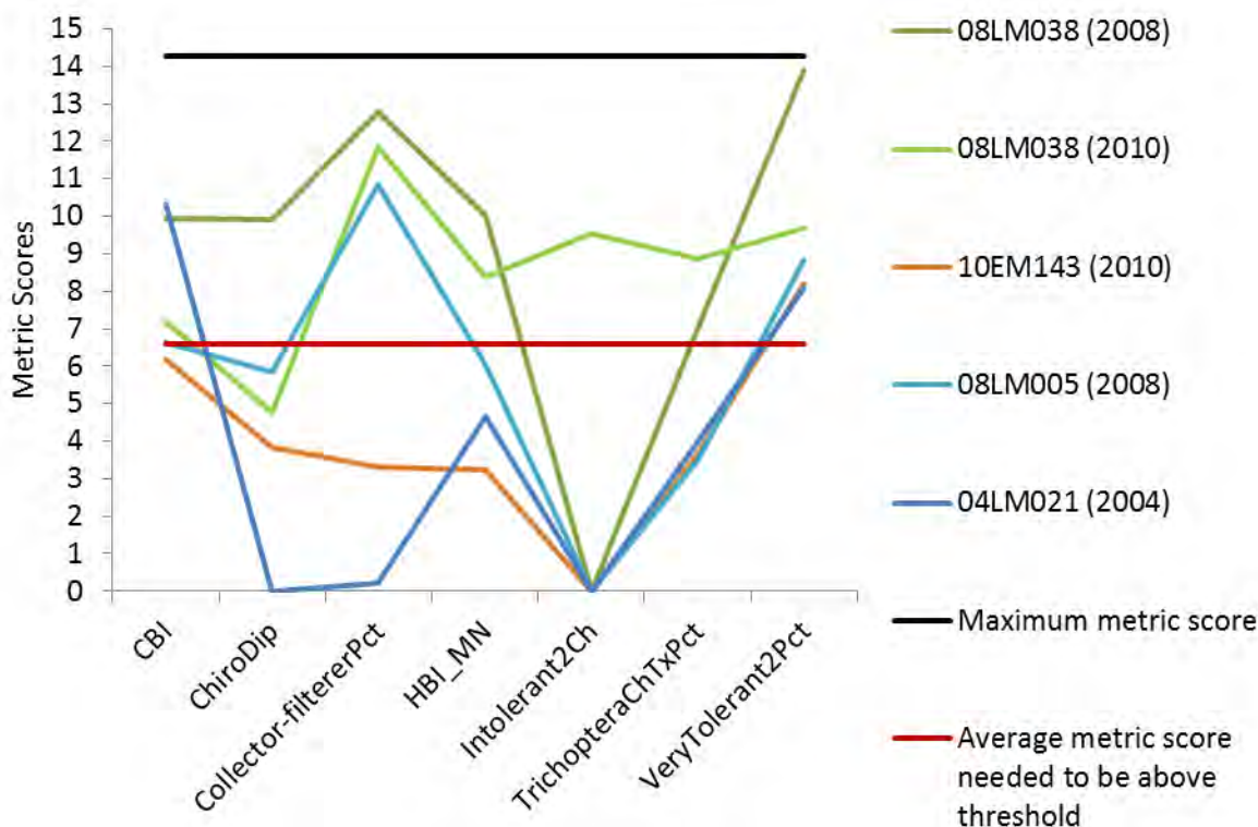
Figure 110. Metric scores for stations in Willow Creek, Southern Coldwater macroinvertebrate IBI
