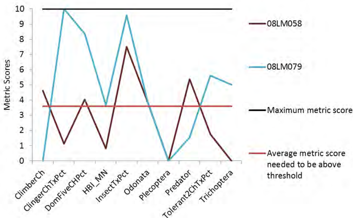
Figure 42. Metric scores for stations in Bear Creek of the Southern Streams RR macroinvertebrate IBI
