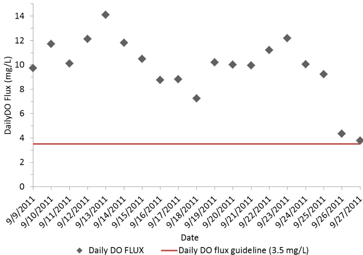
Figure 133. Daily dissolved oxygen flux at 04LM113, in September 2011.
