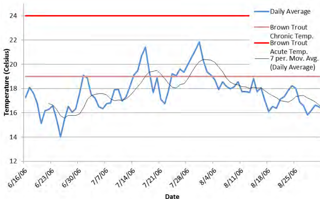
Figure 51. MDNR Station 8.78 (near 04LM058) daily average temperature and weekly average temperature.
