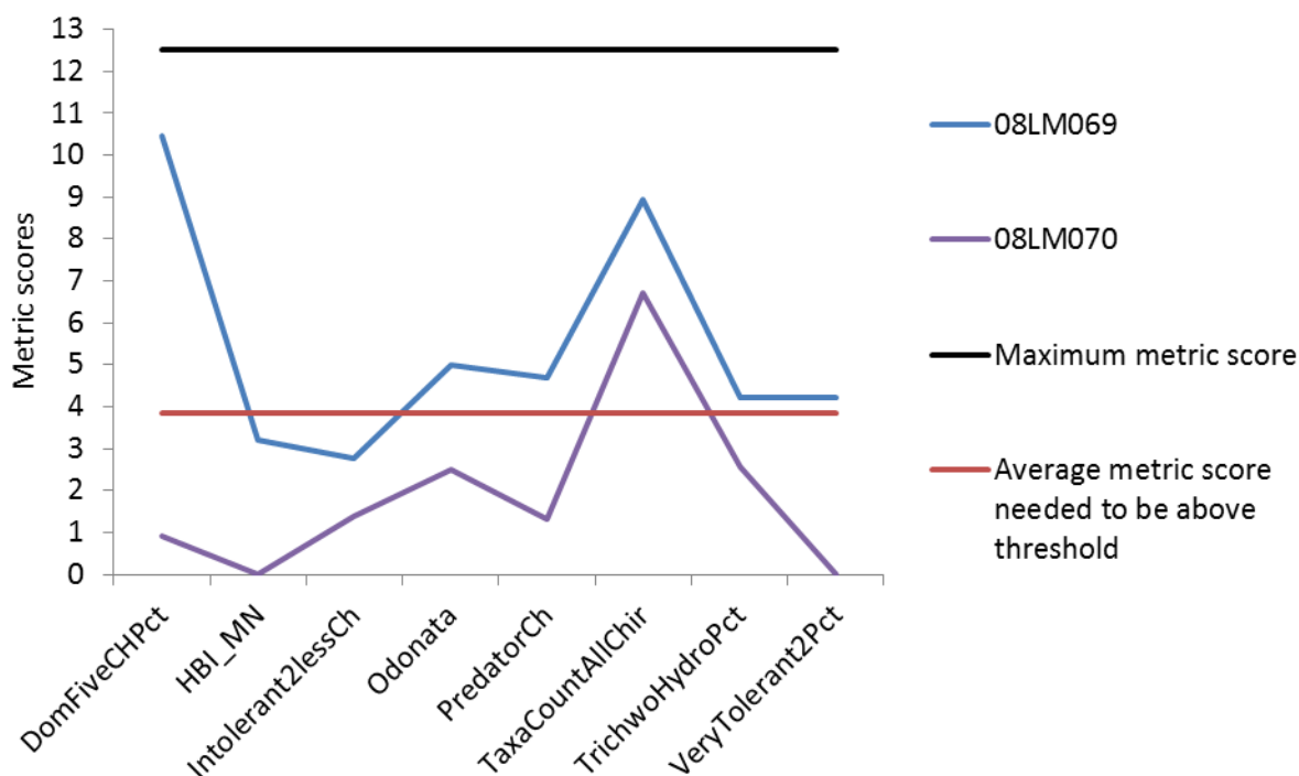
Figure 146. Metric scores for stations in Middle Branch Root River of the Prairie Forest Rivers macroinvertebrate IBI
