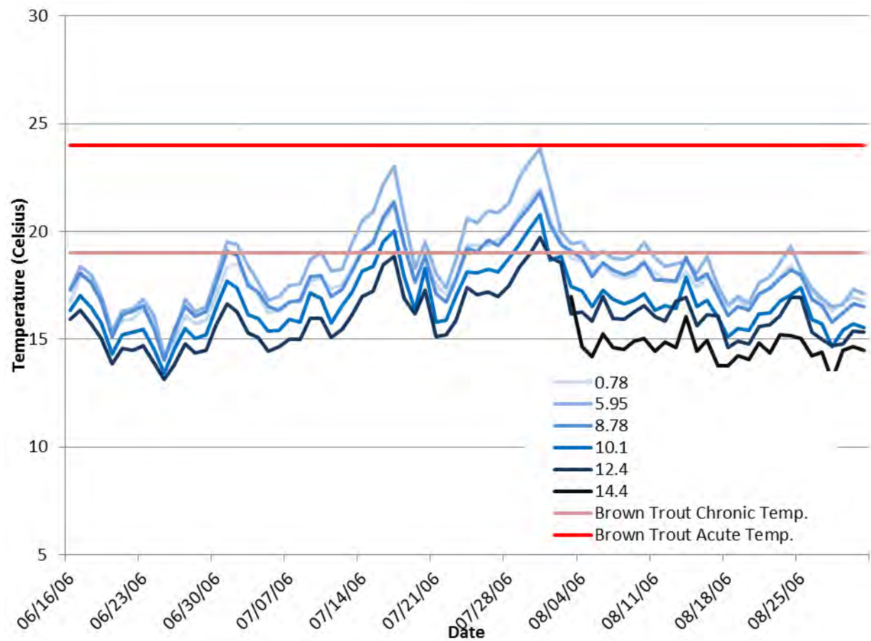
Figure 49. Spring Valley Creek continuous temperature measurements at multiple locations June-August 2006 (MDNR data).
