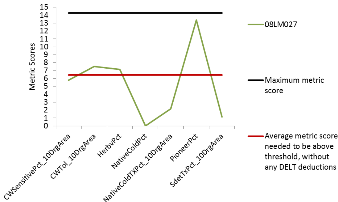
Figure 58. Fish metric scores for Station 08LM027 in Upper Bear Creek of the southern Fish Coldwater IBI.
