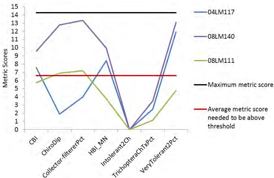
Figure 125. Metric scores for stations in Riceford Creek of the Southern Coldwater macroinvertebrate IBI
