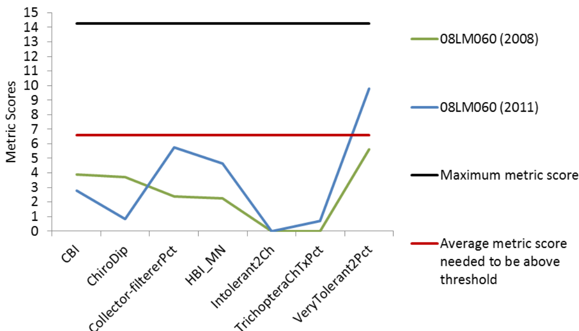
Figure 88. Metric scores for Station 08LM060 in Silver Creek of the Southern Coldwater Macroinvertebrate IBI
