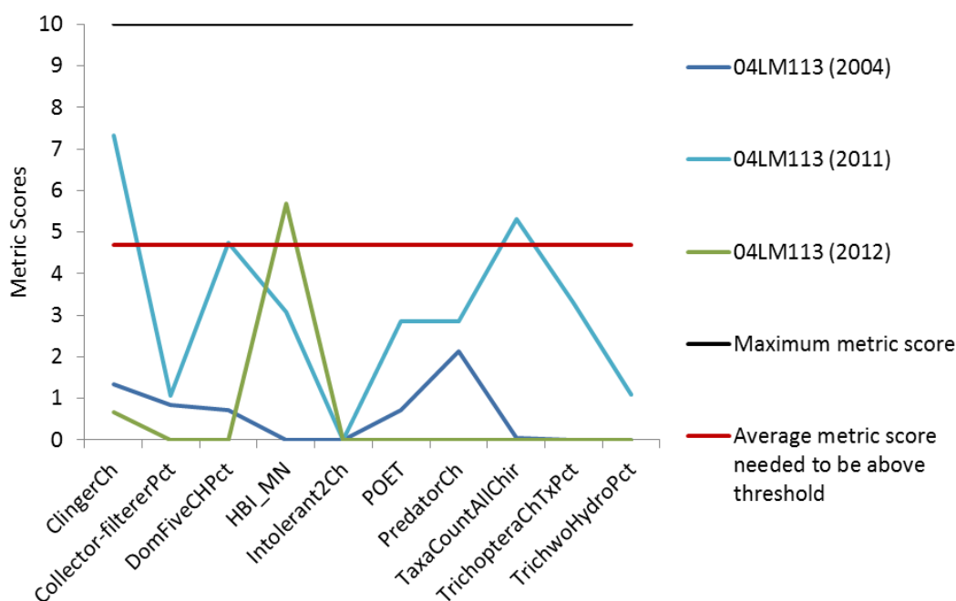
Figure 131. Metric scores for stations in the Upper South Fork Root River (04LM113) of the Southern Forest Streams GP macroinvertebrate IBI
