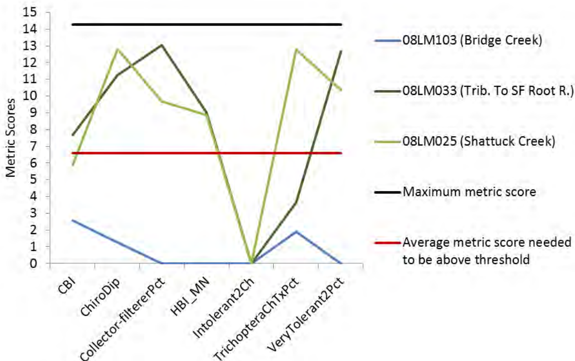
Figure 126. Metric scores for stations in Bridge Creek with comparison to Tributary to SF Root River and Shattuck Creek of the Southern Coldwater macroinvertebrate IBI
