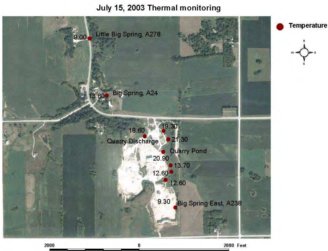
Figure 118. Temperature (degrees Celsius) monitoring results. MDNR study (2003).
