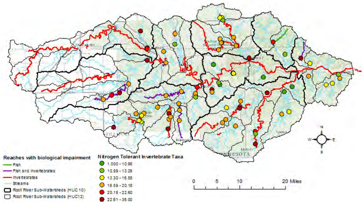
Figure 24. Map of the number of nitrate tolerant macroinvertebrate taxa in coldwater stations in the Root River Watershed
