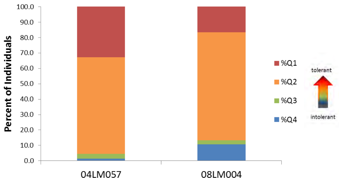
Figure 106. Dissolved oxygen, fish tolerance indicator values for Watson Creek at the two biological stations
