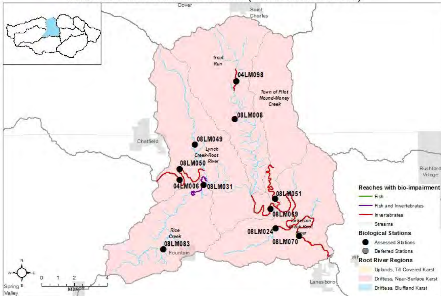
Figure 137. Trout Run-Root River biological monitoring stations and aquatic life impairments
