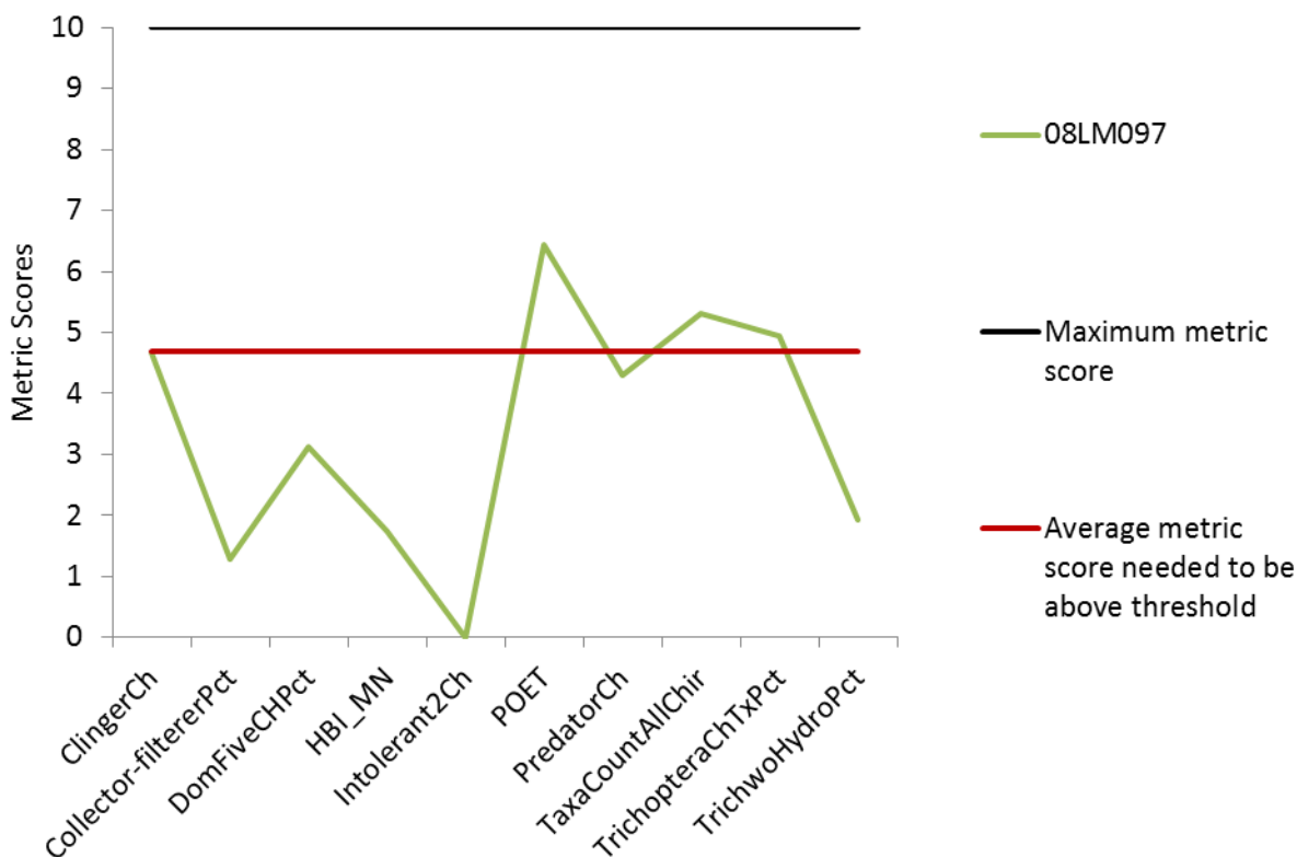
Figure 73. Metric scores for Stations (AUID 717) of the Southern Forest Streams GP macroinvertebrate IBI
