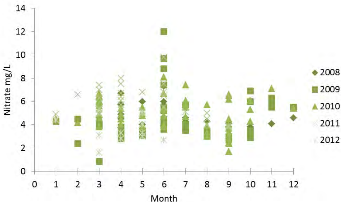
Figure 86. Nitrate concentrations for the mainstem Root River, Station S004-858 (Mound Prairie, 2008-2012)
