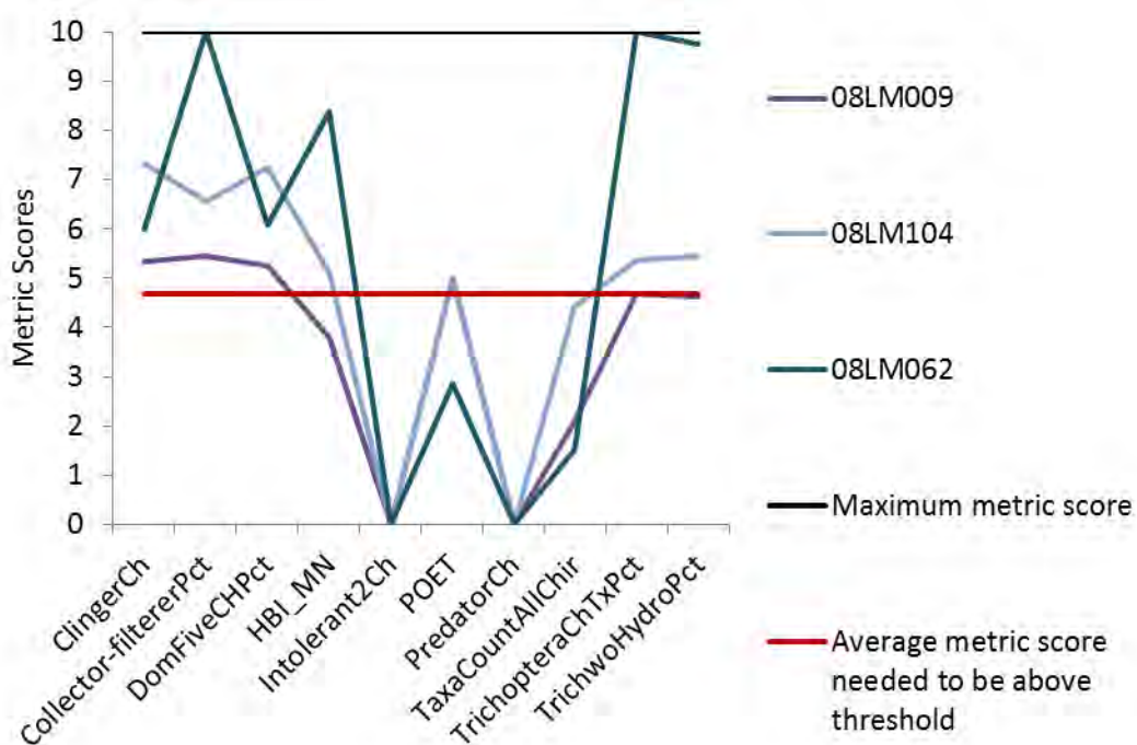
Figure 122. Metric scores for stations in the South Fork Root River of the Southern Forest Streams GP macroinvertebrate IBI
