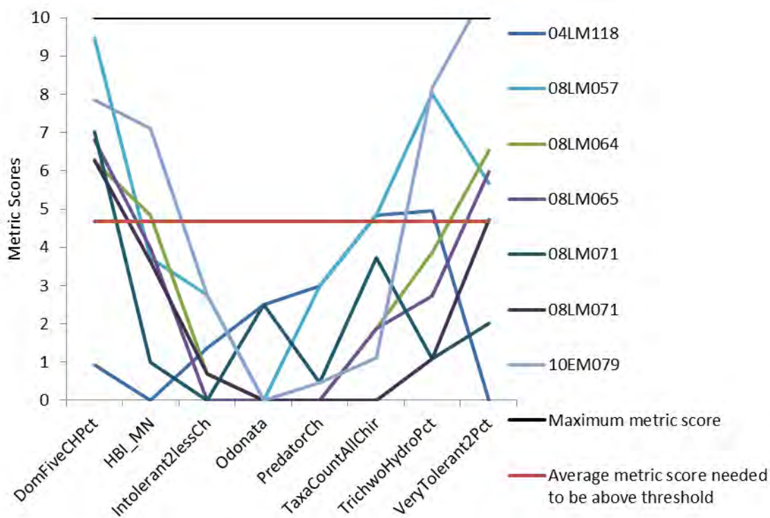
Figure 35. Macroinvertebrate IBI metrics for biological stations on AUIDs 520,522,527; Prairie Forest Rivers (Class 2).
