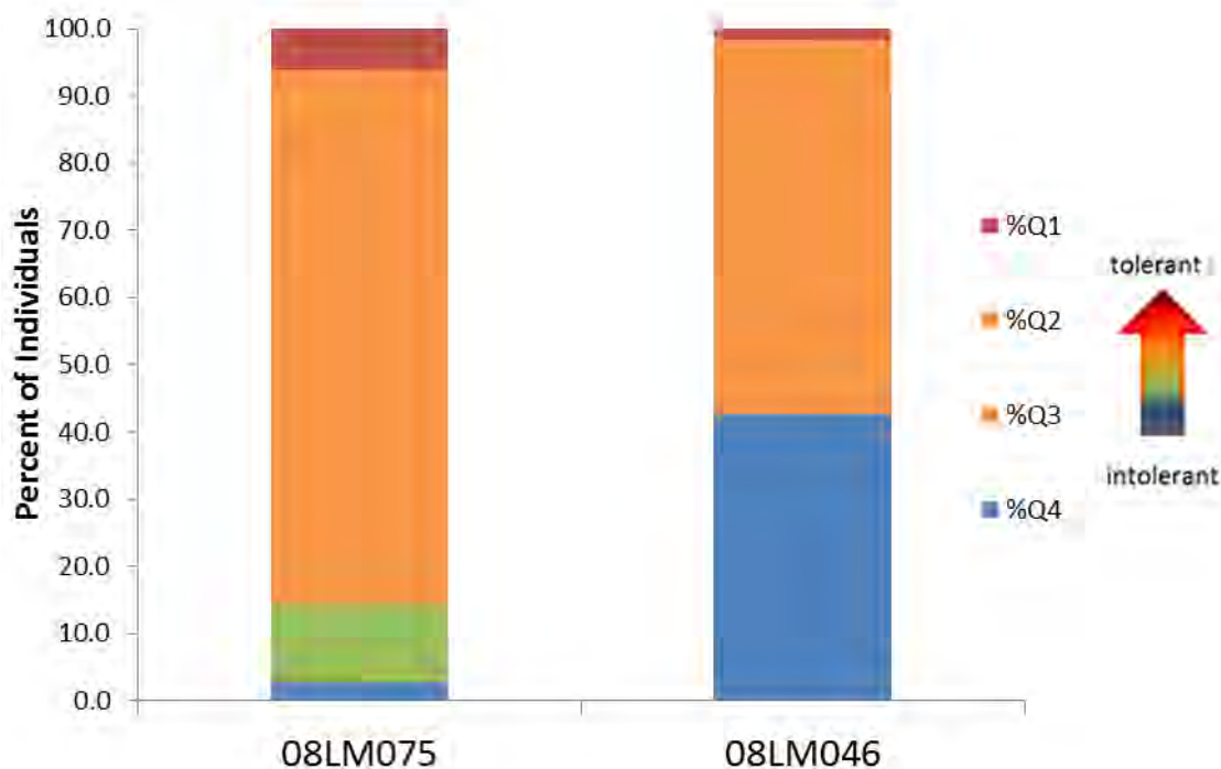
Figure 119. Dissolved Oxygen, fish tolerance indicator values for Camp Creek
