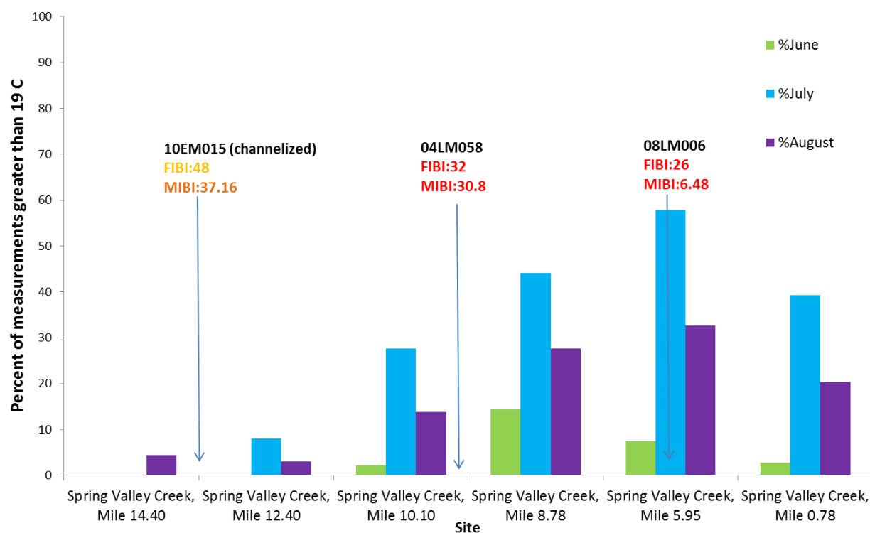
Figure 48. Spring Valley Creek percent temperature measurements above 19°C with biological information at multiple stations along the creek, for all summer months (MDNR continuous temperature data from 2006).
