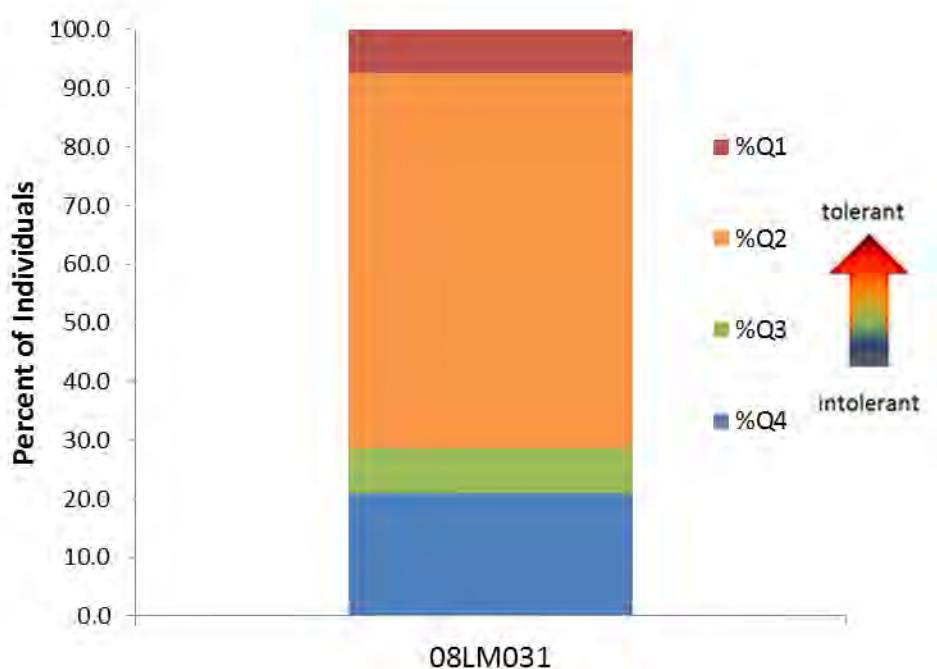
Figure 143: Dissolved Oxygen tolerance indicator values for 08LM031.
