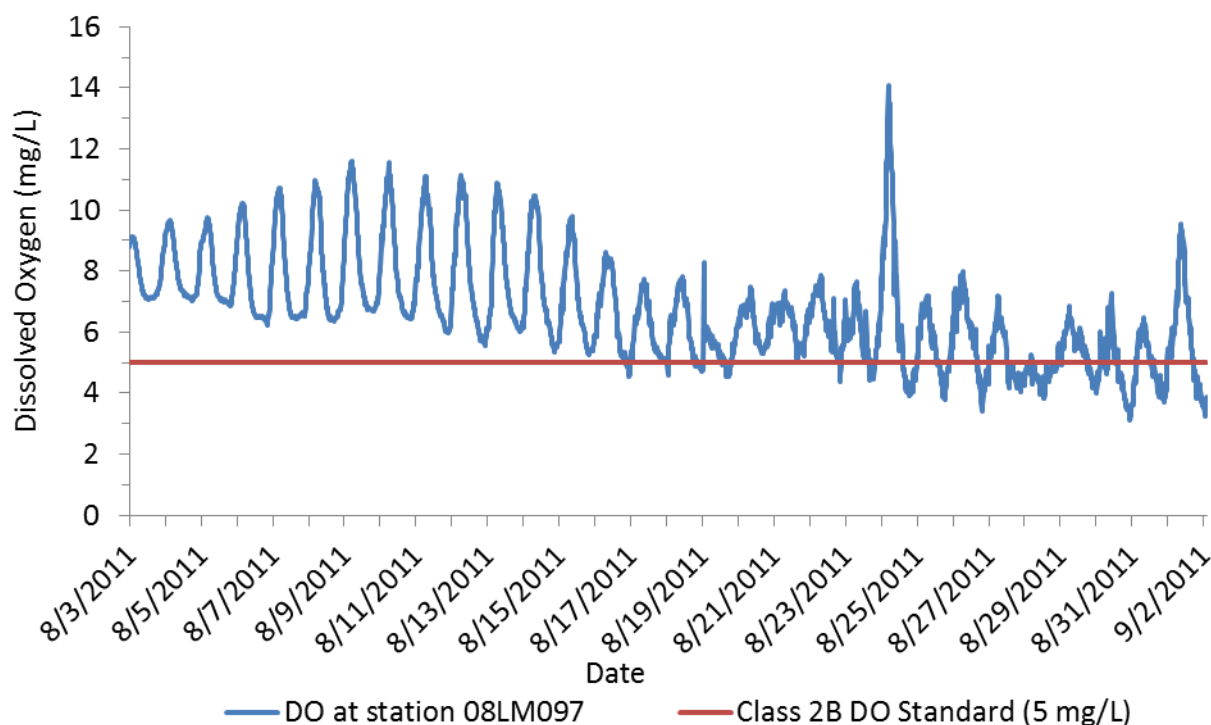
Figure 75. Dissolved oxygen data from 08LM097 from 8/3/2011-9/2/2011.
