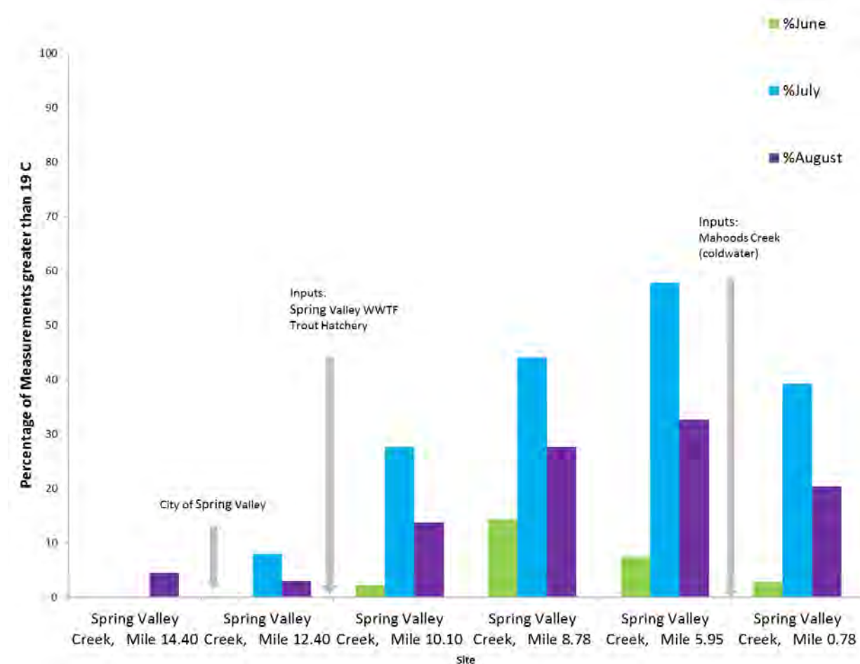
Figure 47. Spring Valley Creek percent temperature measurements above 19°C with geographical and input consideration (MDNR continuous temperature data from 2006).
