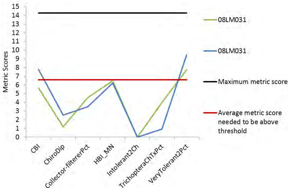
Figure 142. Metric scores for visits at Rice Creek, Station 08LM031, of the Southern Coldwater macroinvertebrate IBI
