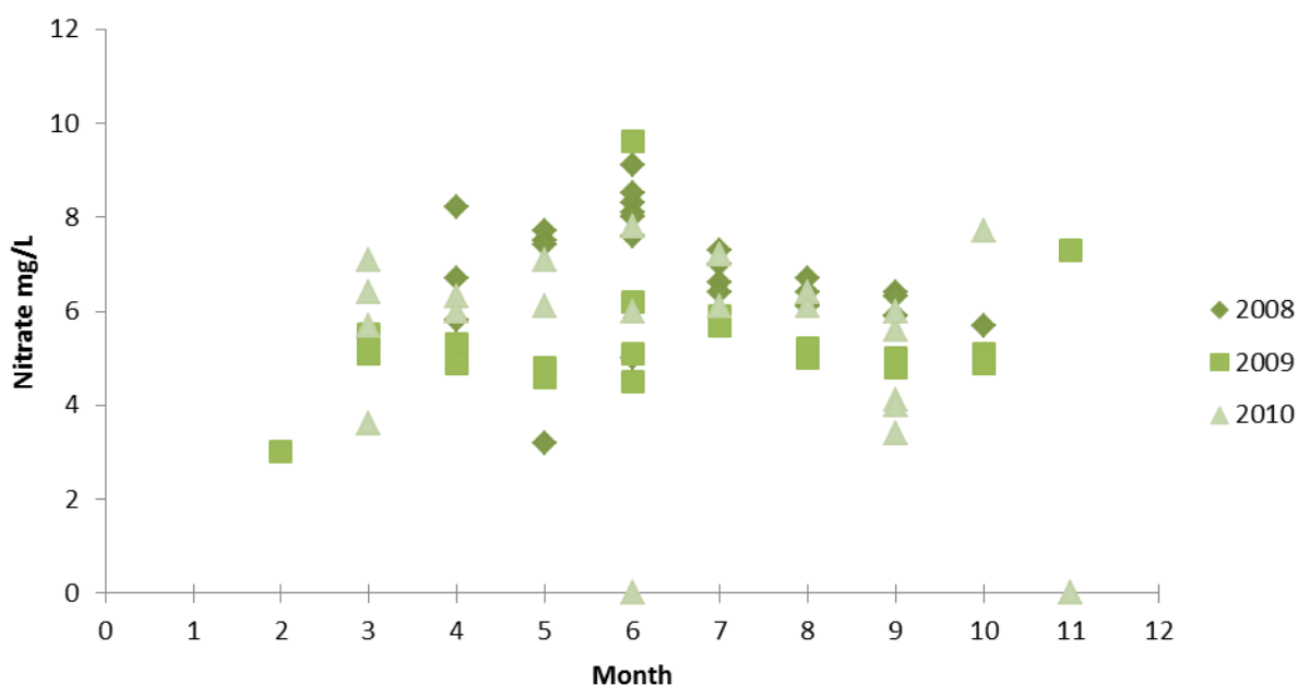
Figure 99. Grab sample nitrate concentration for South Branch Root River, at Lanesboro 2008-2010
