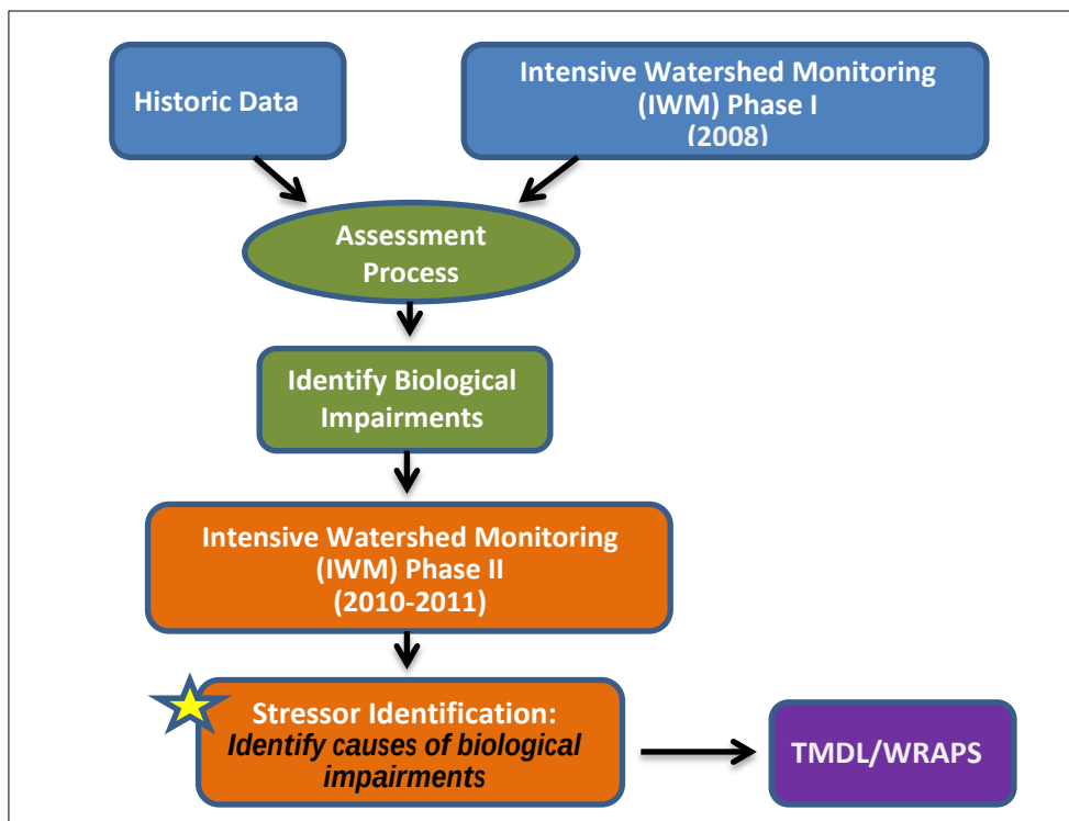
Figure 1. Process map of Intensive Watershed Monitoring, Assessment, Stressor Identification and TMDL processes.
