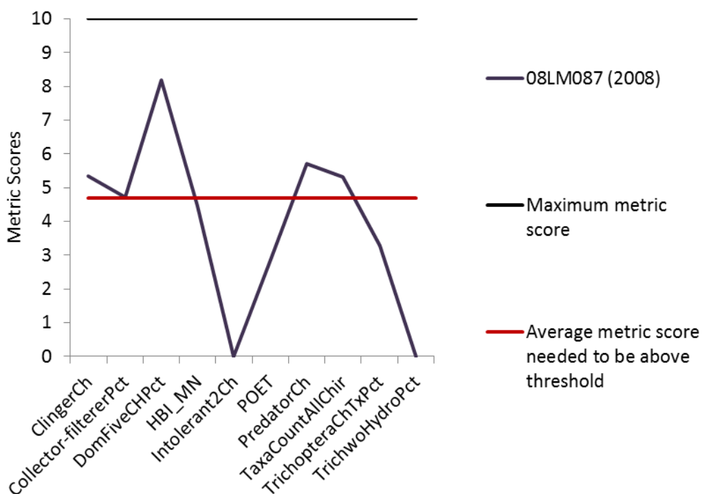
Figure 135. Metric scores for stations in the Upper South Fork River and Sorenson Creek (08LM087) of the Southern Forest Streams GP macroinvertebrate IBI
