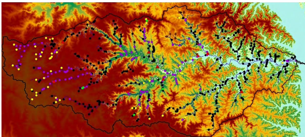
Figure 33. Culverts evaluated in the Root River, data and map provided by MDNR
