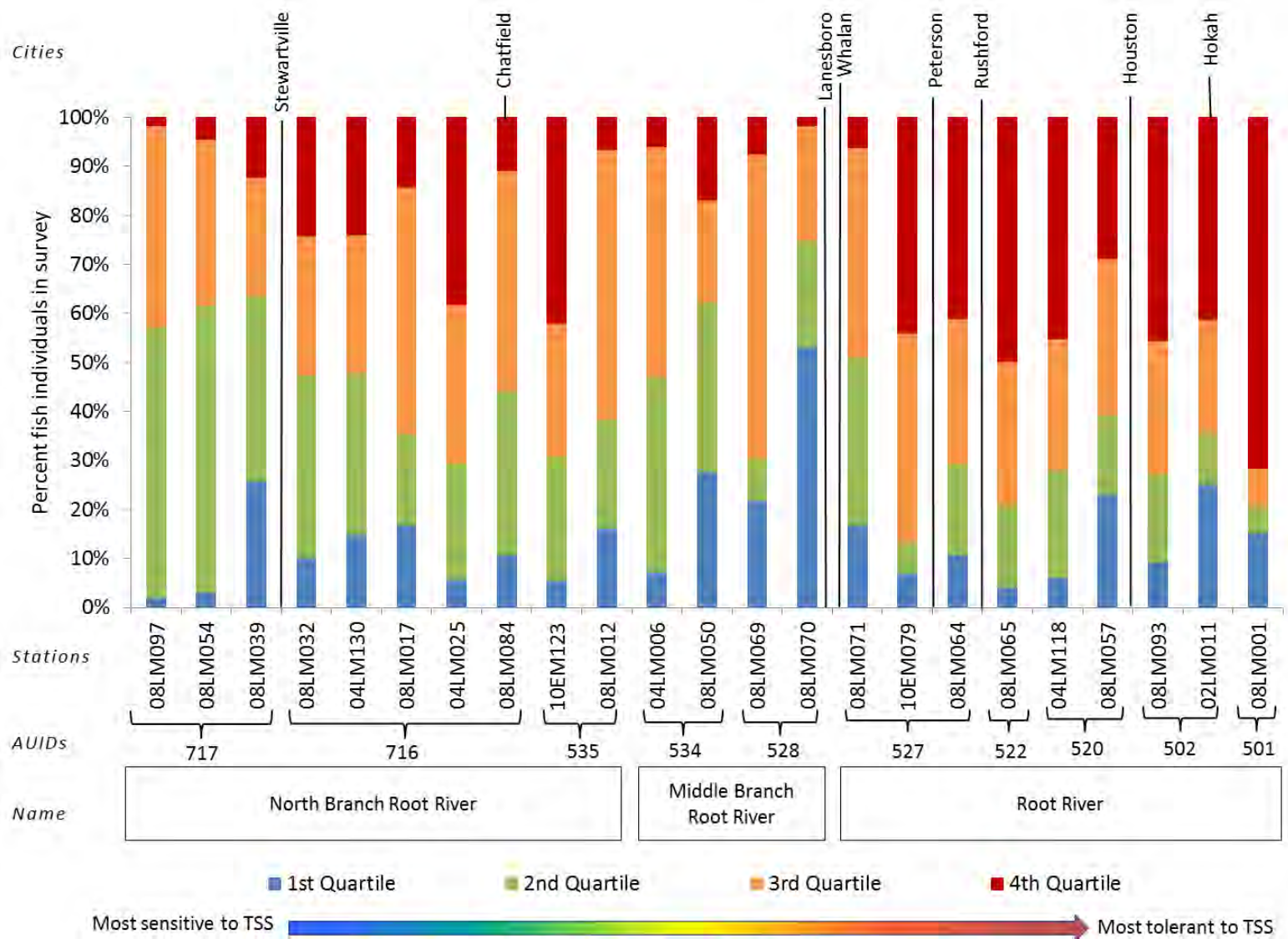
Figure 30. Percent fish individuals by biological station along the Root River, for each quartile based on total suspended sediment tolerance values for fish species, weighted on the warmwater species present in the Root River Watershed.
