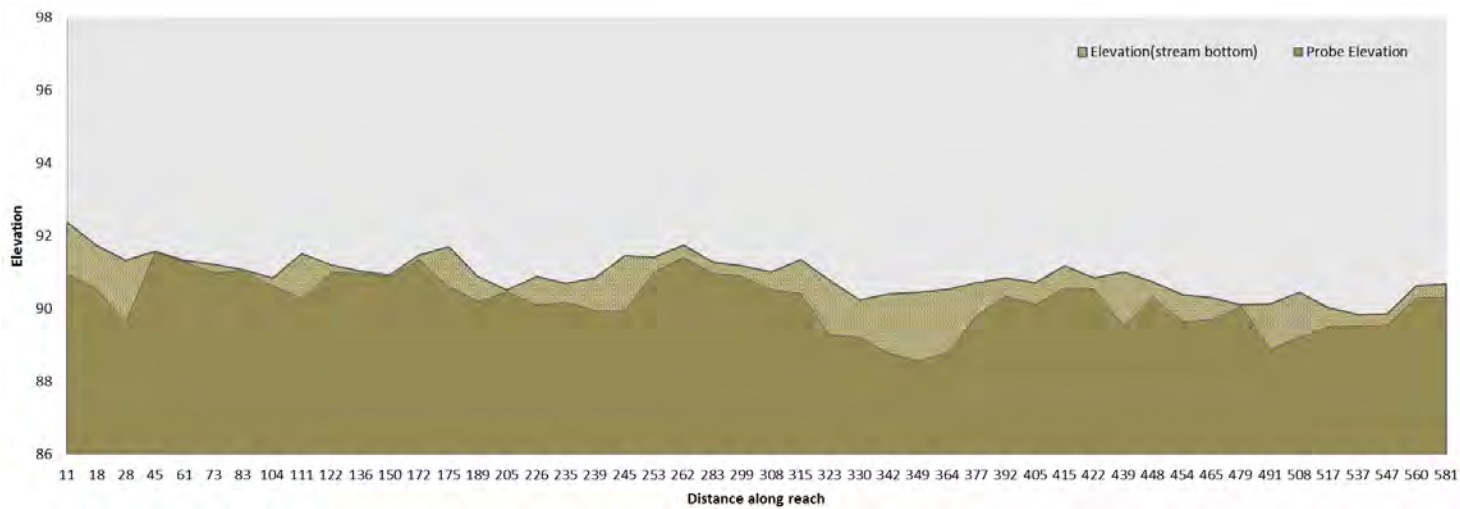
Figure 78. Station 08LM097 longitudinal profile and sediment deposition
