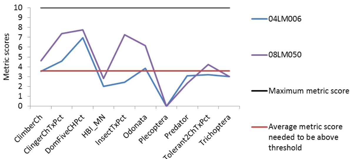
Figure 144. Metric scores for stations in Middle Branch Root River of the Southern Streams RR macroinvertebrate IBI
