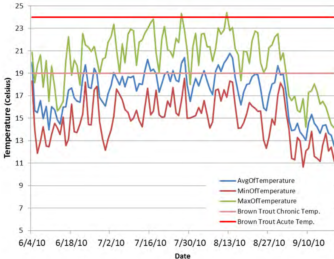
Figure 63: Corey Creek Daily average, maximum and minimum temperatures for 2010.
