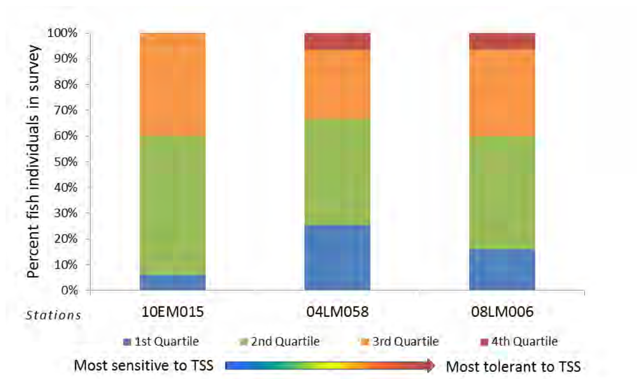
Figure 53. Fish TSS TIVs for three biological stations in Spring Valley Creek.
