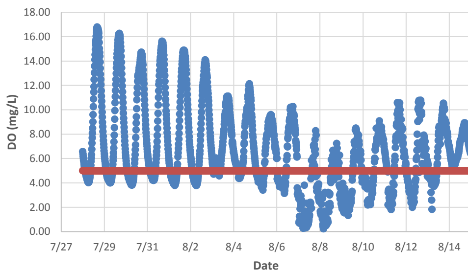
Figure 67. Continuous DO data at station 15MN056
