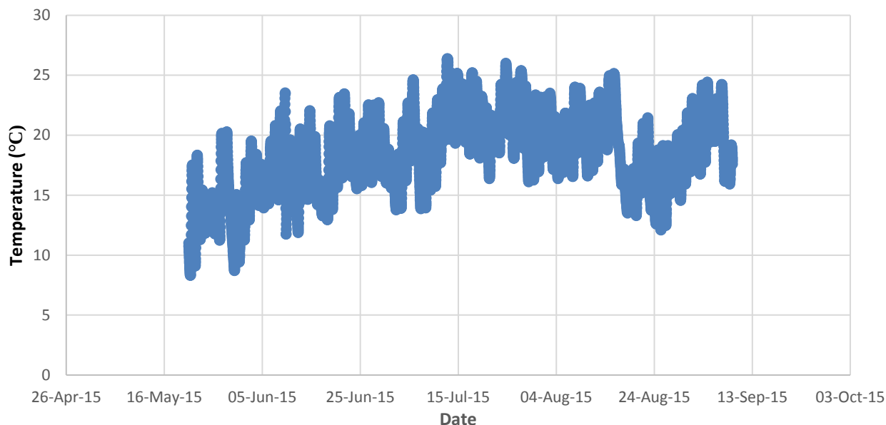
Figure 40. Continuous temperature data at station 09MN093
