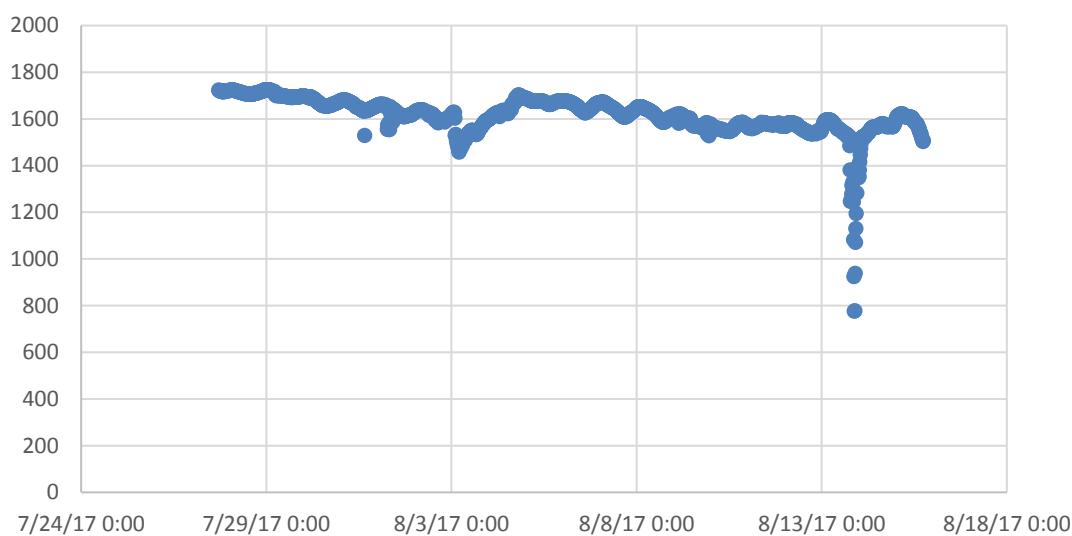
Figure 82. Continuous specific conductance values at site 15MN090
