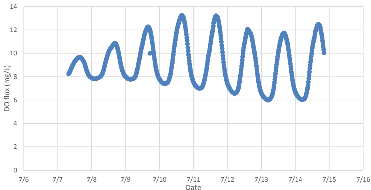
Figure 39. Continuous DO data at station 15MN049
