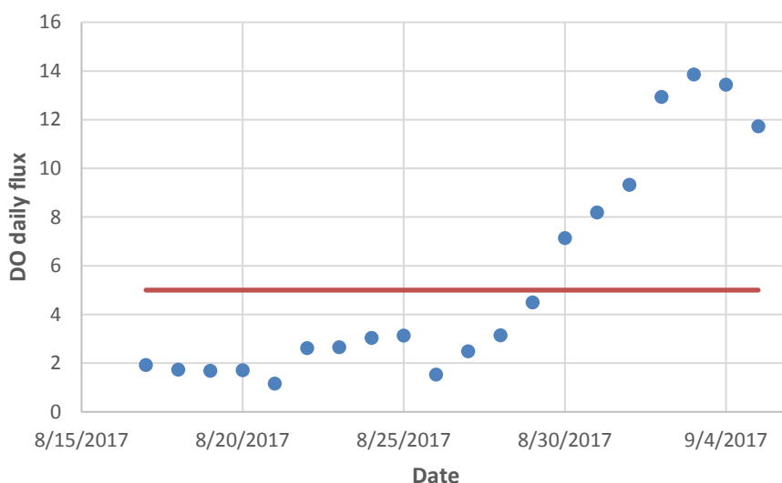
Figure 70. DO fluctuation at station 15MN050
