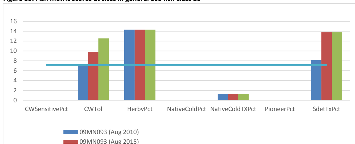
Figure 35. Fish metric scores at sites in general use fish class 10
