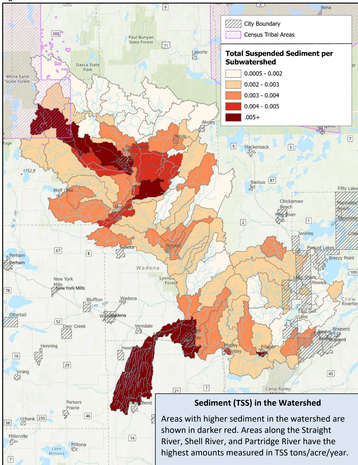
Figure 10. Modeled TSS in the watershed.
