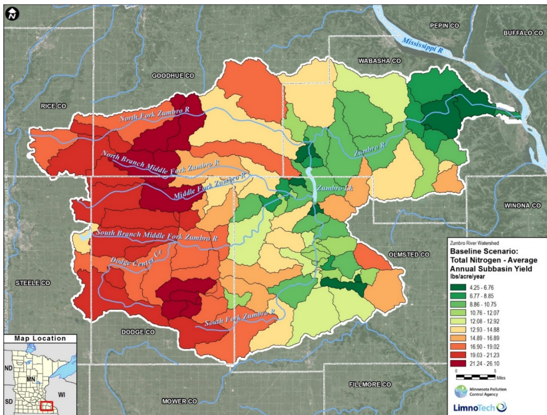
Figure 38. HSPFZRW model baseline simulation for TN.
