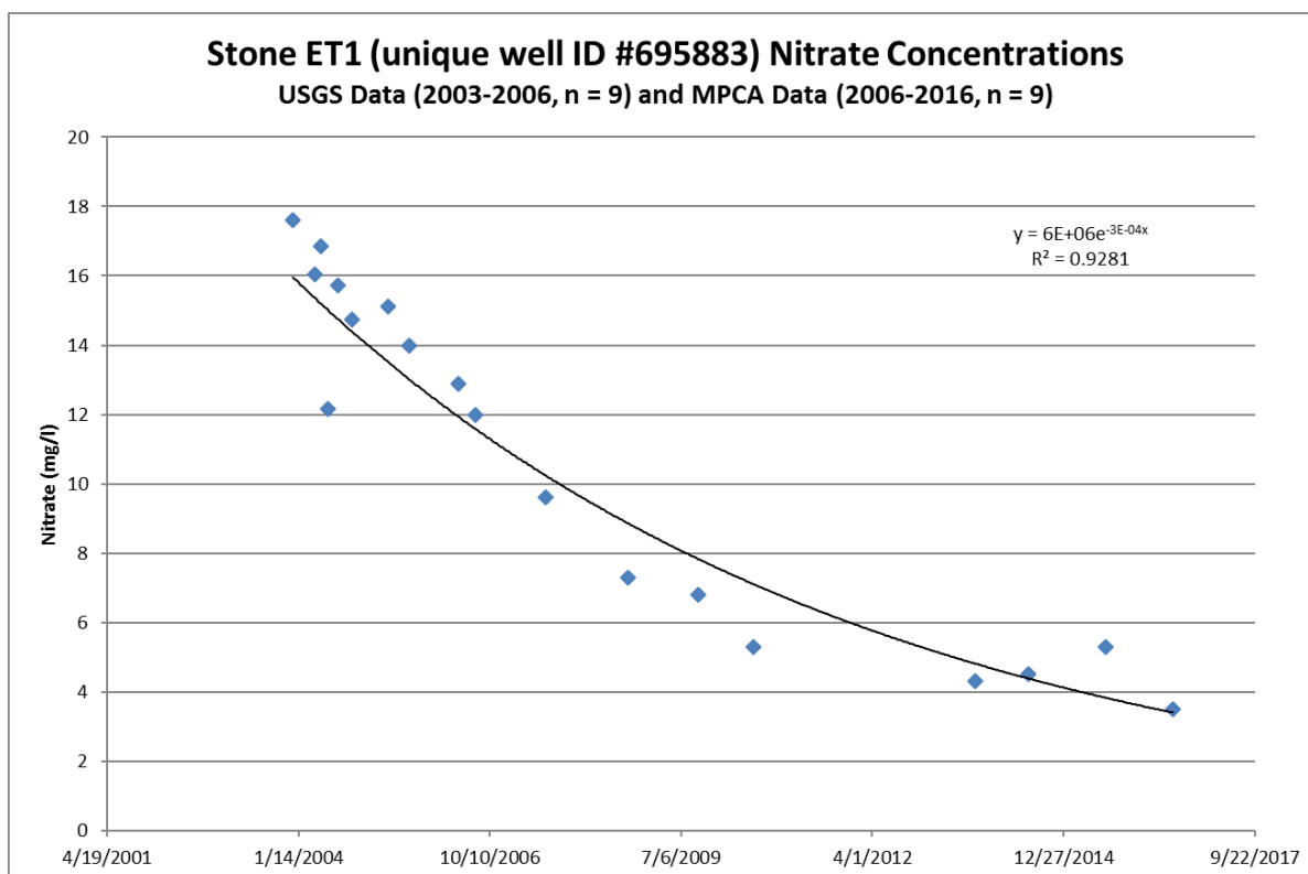
Figure 28. Stone ET1 well nitrate data.
