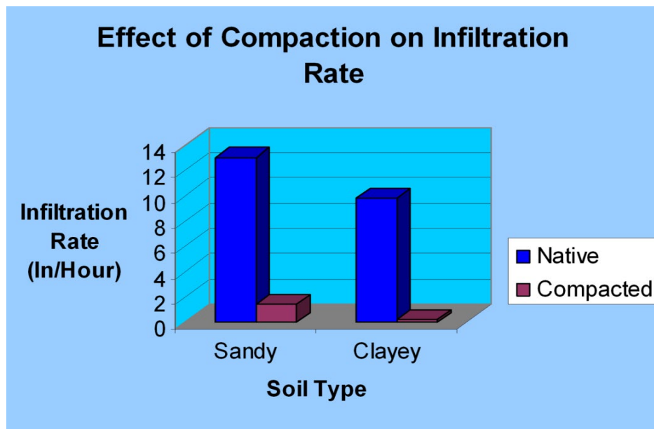
Figure 57. Infiltration rates by soil type and level of compaction. (Source: Minnesota Stormwater Manual)
