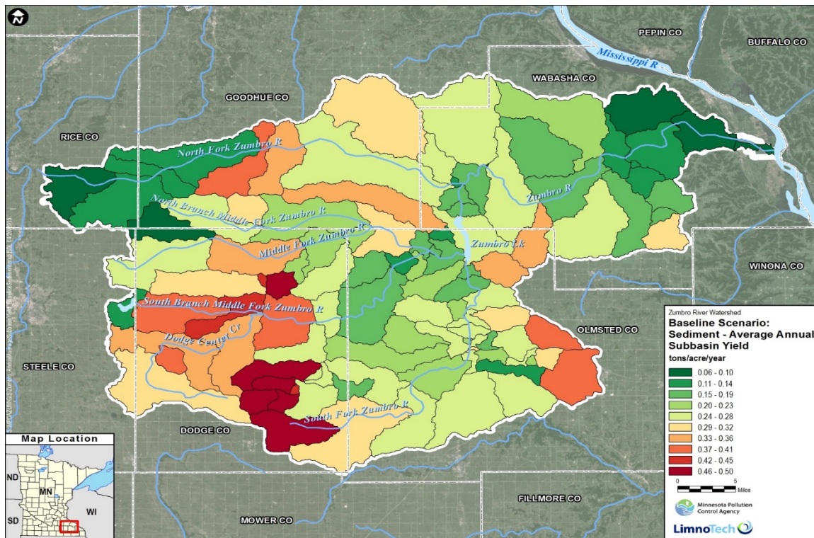
Figure 40. HSPFZRW model baseline simulation for TSS.
