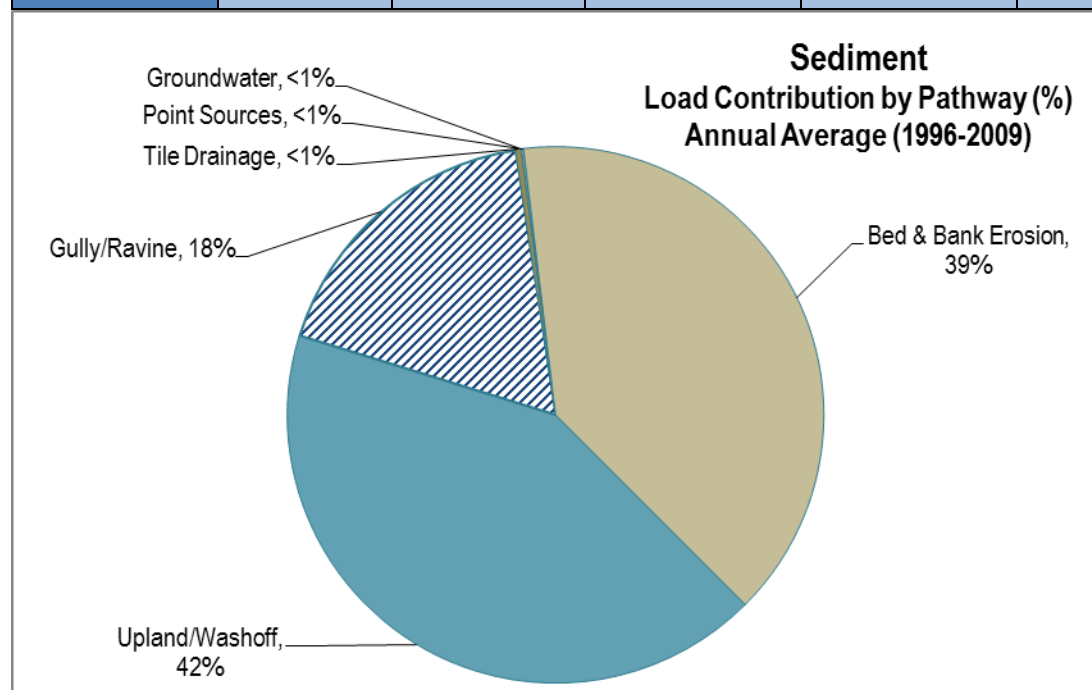
Figure 19. Breakdown of sediment sources for the ZRW HSPF model (1996 – 2009).
