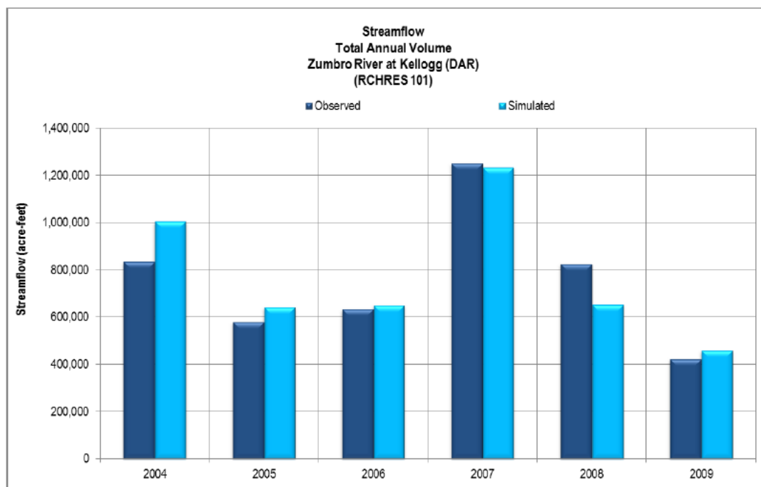
Figure 1: Observed annual streamflow volume (dark blue) and HSPF simulated volume (light blue) at the outlet of the Zumbro River. (Figure produced by LimnoTech.)
