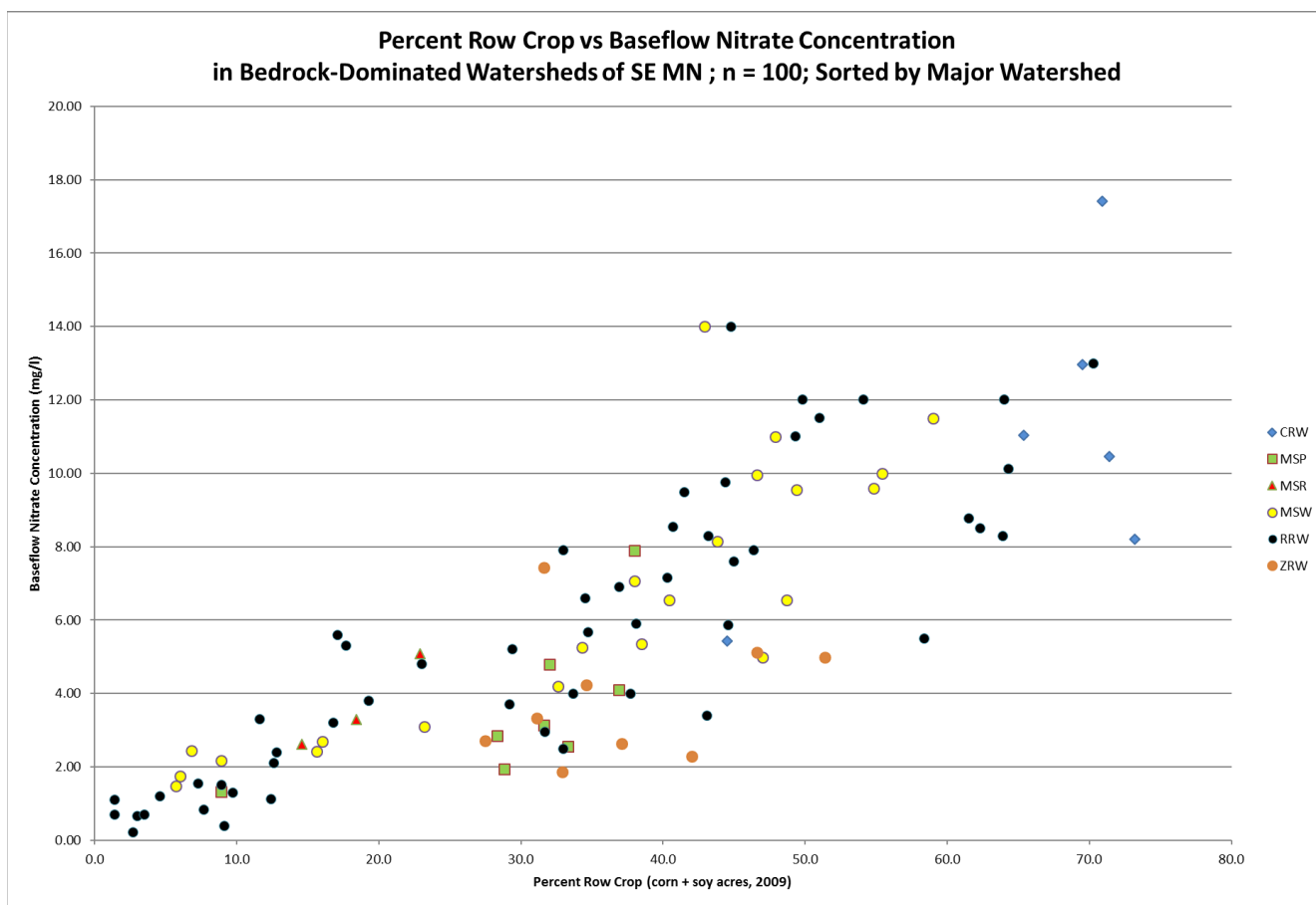
Figure 22. Baseflow nitrate and row crop acres regression (Watkins, Rasmussen, Streitz et al 2013).
