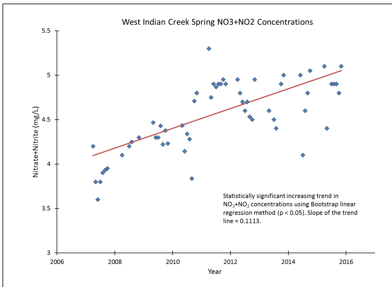
Figure 17. West Indian Creek nitrate data over time.
