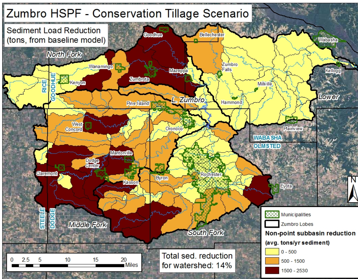
Figure 42. ZRW TSS load reduction for Conservation Tillage Management Scenario.
