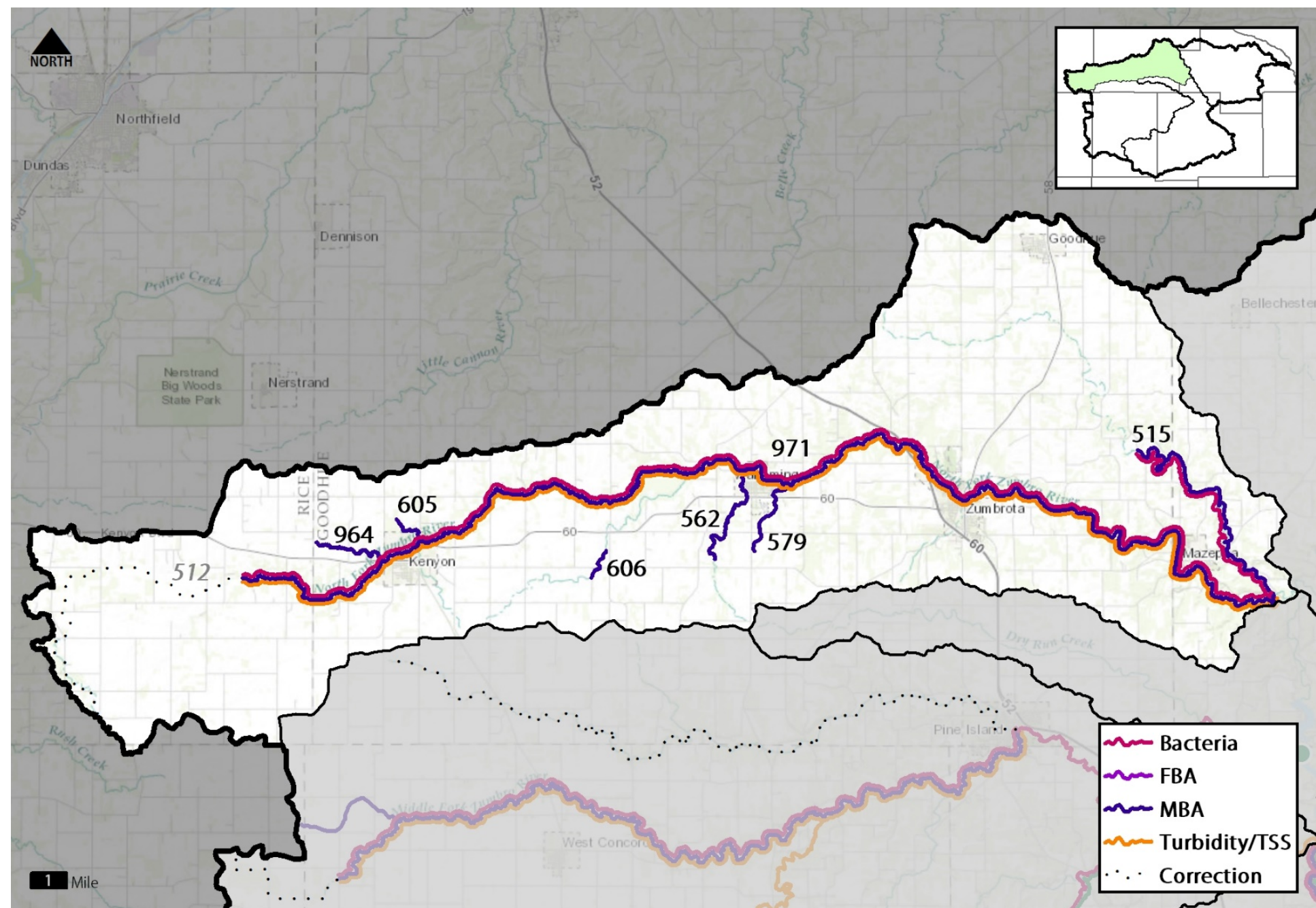
Figure 58. Map of the North Fork Watershed and macroinvertebrate impairments.
