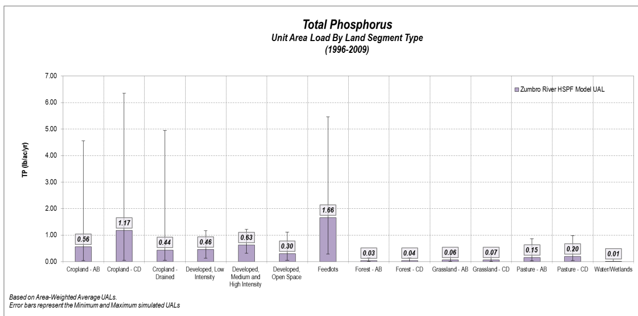
Figure 20. Total phosphorus unit area loads by land segment type for the 1996 – 2009 simulation period.
