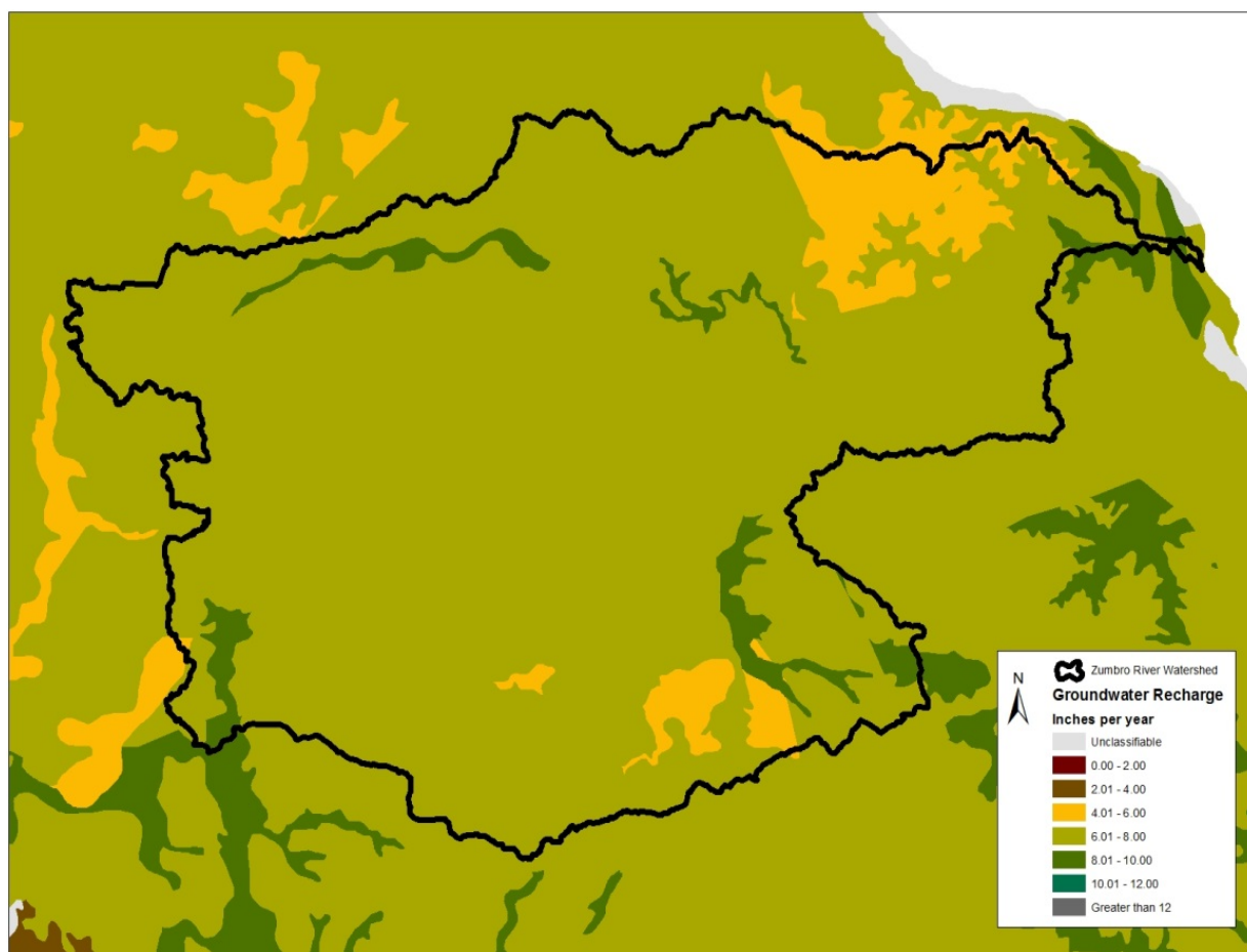
Figure 10. Average annual recharge rate to surficial materials in the ZRW (1971 – 2000).
