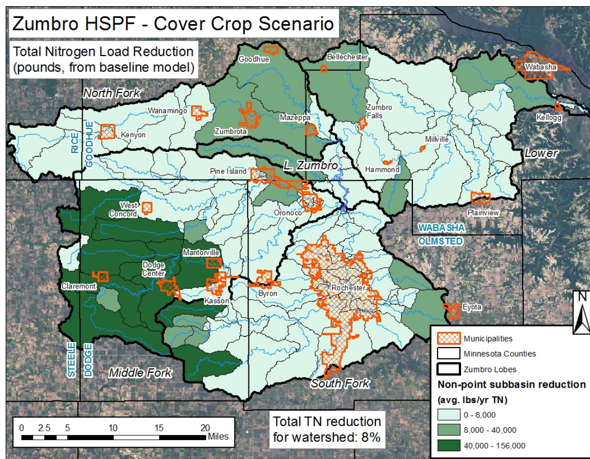
Figure 41. ZRW TN load reduction for Cover Crop Management Scenario.
