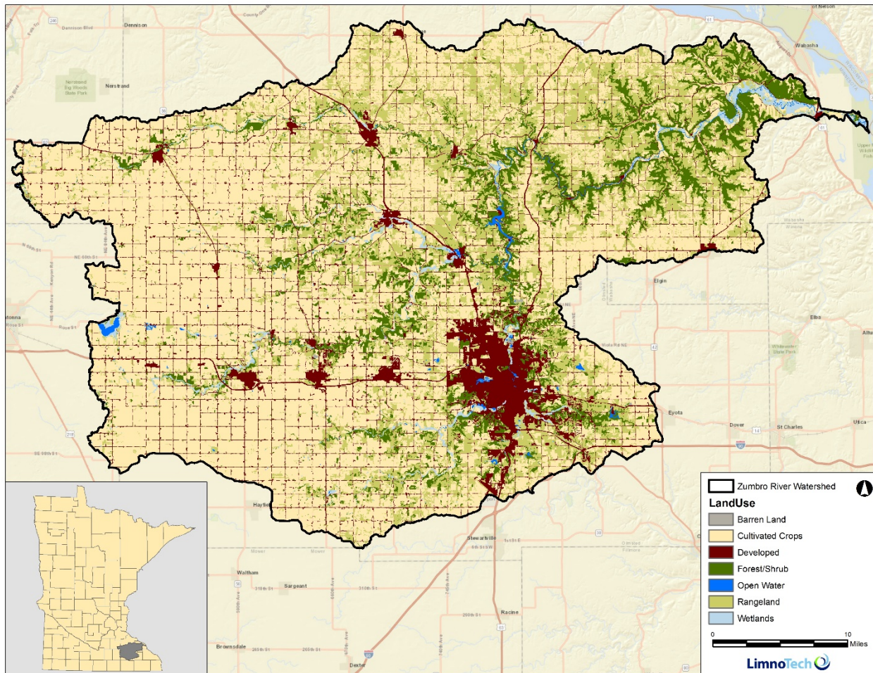
Figure 3. National Land Cover Dataset land use coverage in the ZRW (from NLCD 2011 dataset).
