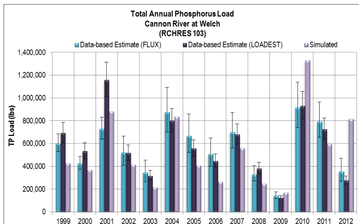
Figure 4-58. Annual Total Phosphorus Load for Cannon River at Welch (RCHRES 103).
