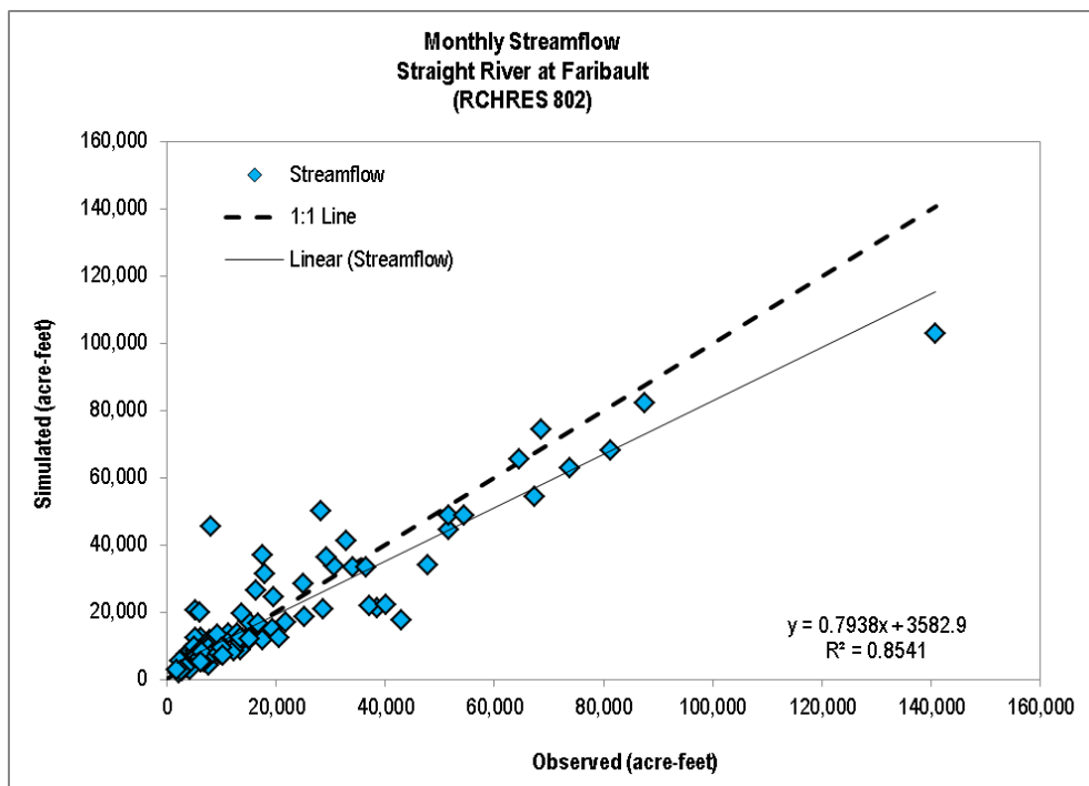
Figure 4-28. Monthly Streamflow 1:1 Plot for Straight River at Faribault, 1996-2003 (Gage #05353800)
