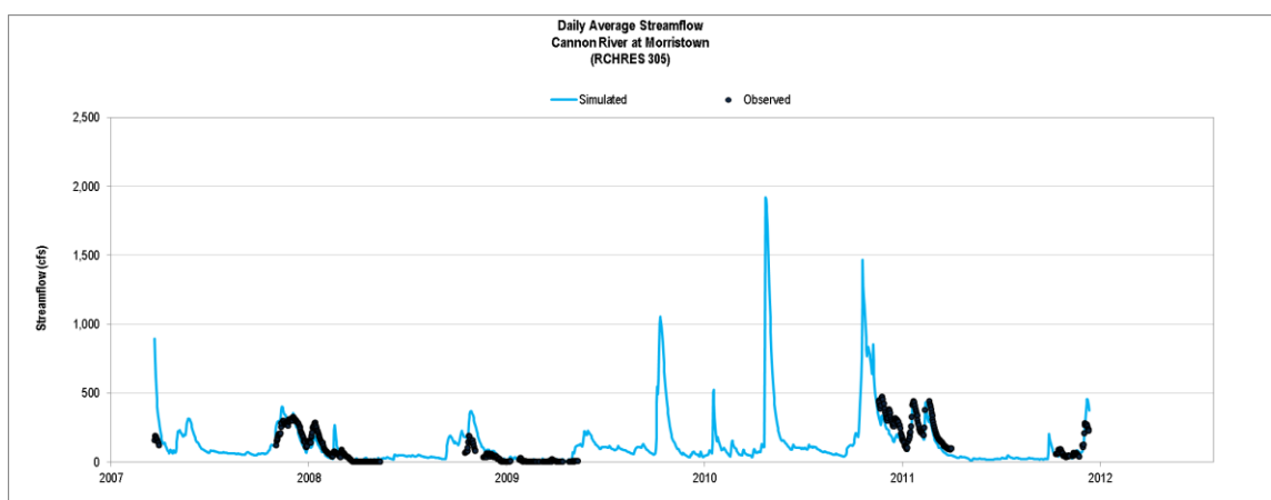
Figure A-11. Streamflow Total Daily Volume for Cannon River at Morristown (Gage #H39091001)
