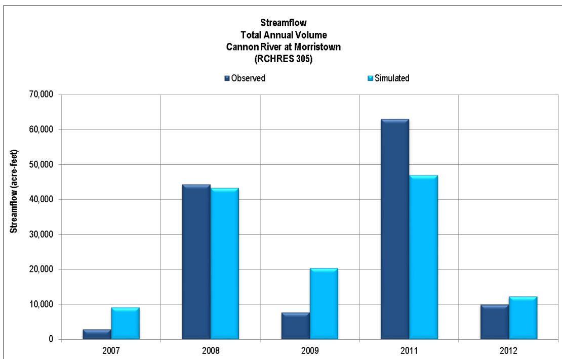
Figure A-9. Streamflow Total Annual Volume for Cannon River at Morristown (Gage #H39091001)
