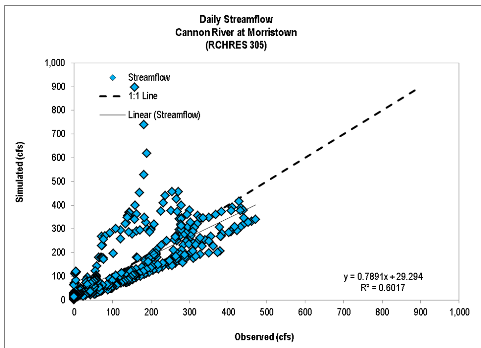
Figure A-8. Daily Streamflow 1:1 Plot for Cannon River at Morristown (Gage #H39091001)
