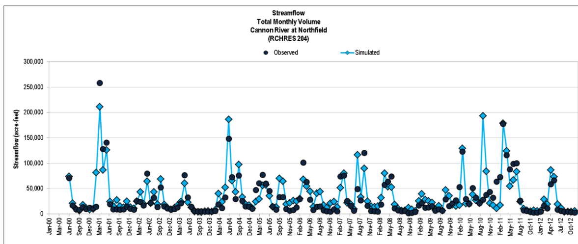
Figure A-16. Streamflow Total Monthly Volume for Cannon River at Northfield (Gage #H39069001)
