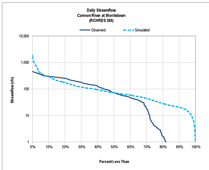
Figure A-12. Daily Streamflow Cumulative Frequency Distribution for Cannon River at Morristown (Gage #H39091001)
