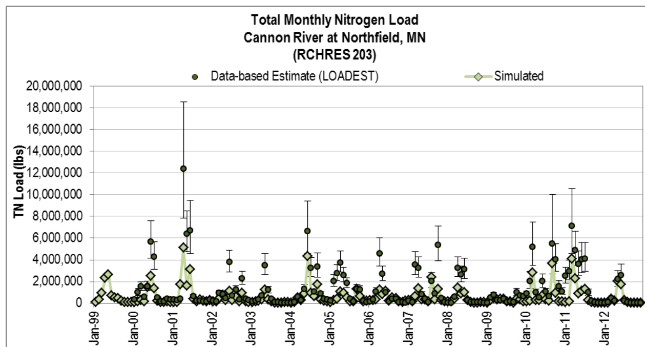
Figure 4-74. Monthly Total Nitrogen Load at Cannon River at Northfield (RCHRES 203).
