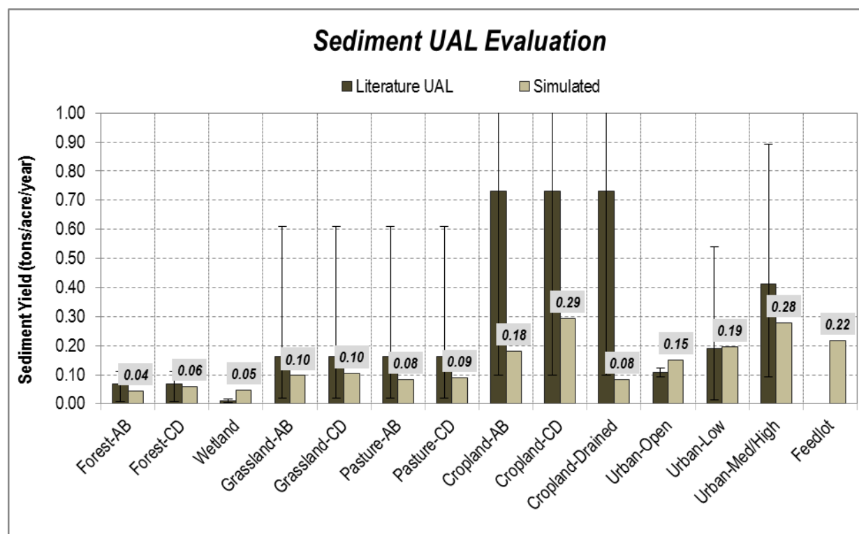
Figure 4-45. Area-weighted UALs for the Cannon River Watershed HSPF Model by Land Use Type Compared to Literature Averages (error bars represent minimum and maximum) (1996-2012).
