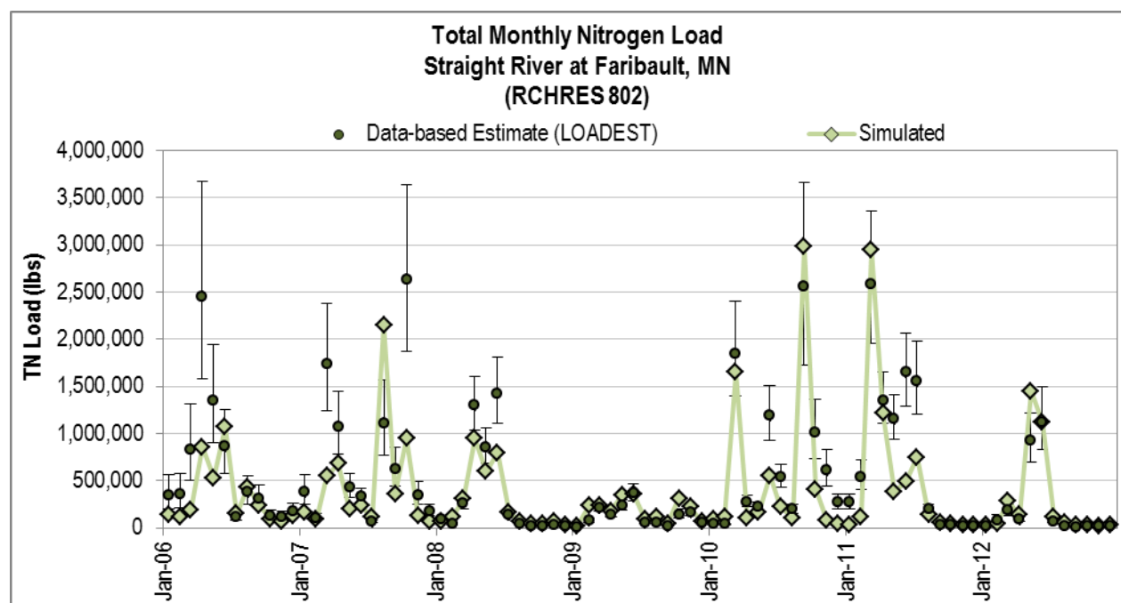
Figure 4-73. Monthly Total Nitrogen Load at Straight River at Faribault (RCHRES 802).
