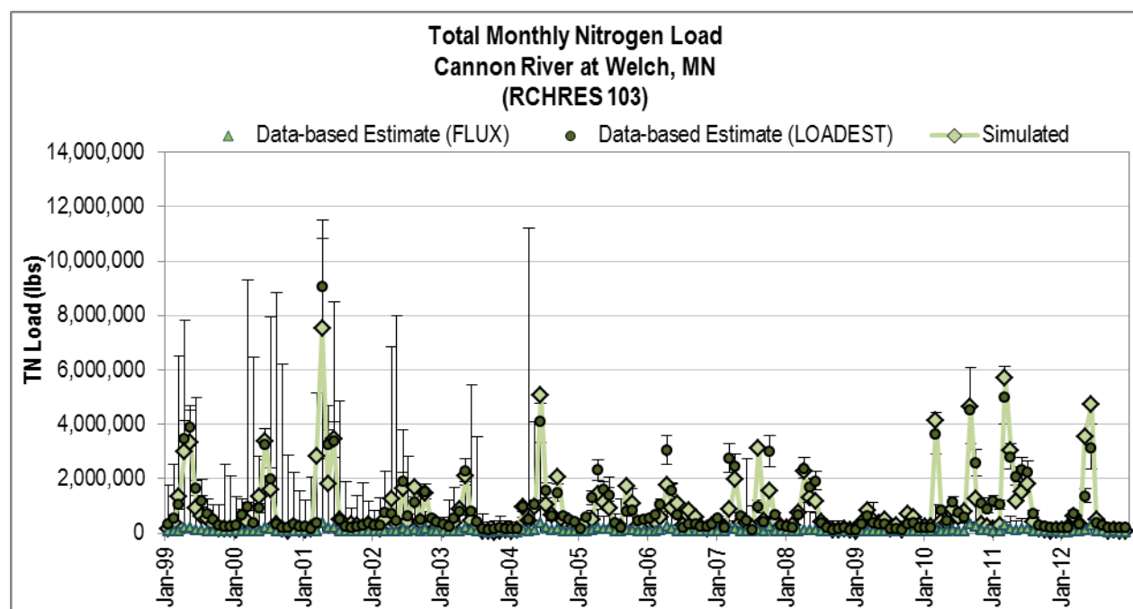
Figure 4-70. Monthly Total Nitrogen Load at Cannon River at Welch (RCHRES 103).
