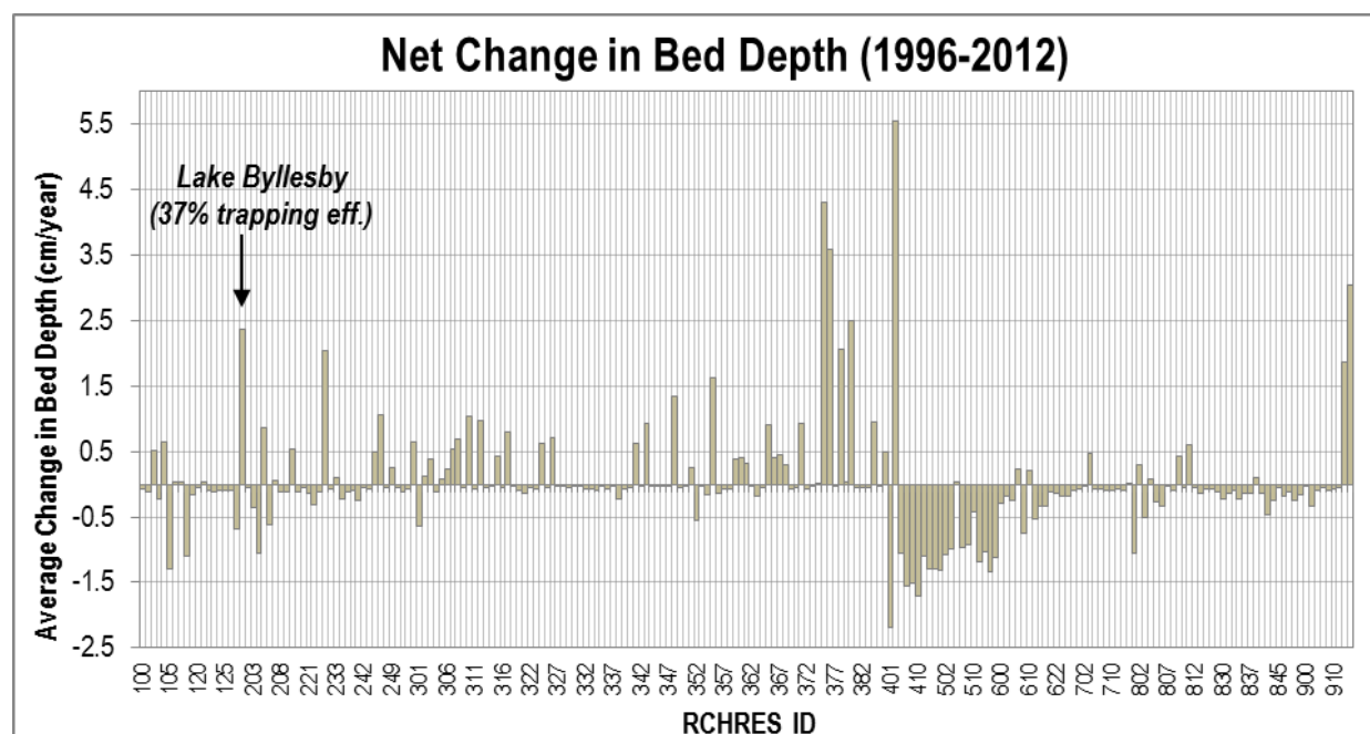
Figure 4-49. Average Annual Change in Bed Depth for All Reaches in the Cannon River Watershed HSPF Model (1996-2012).
