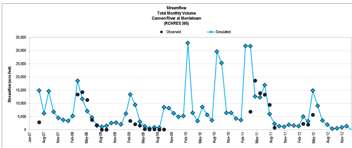
Figure A-10. Streamflow Total Monthly Volume for Cannon River at Morristown (Gage #H39091001)
