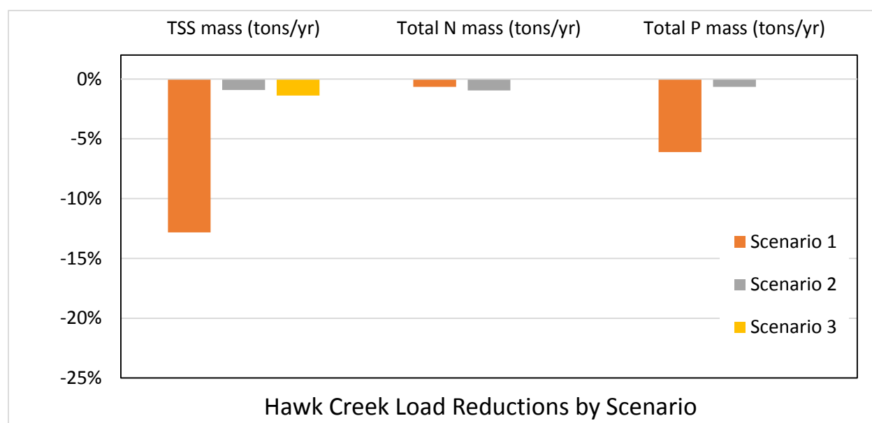
Figure 3. Changes in pollutant loading at mouth of Hawk Creek by scenario
