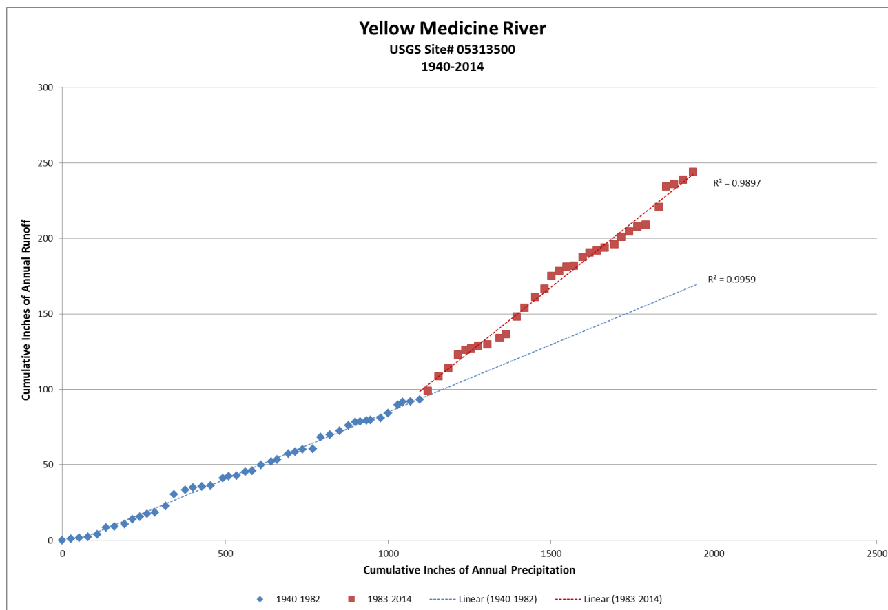
Figure 6 – Double mass curve for Yellow Medicine near Granite Falls
