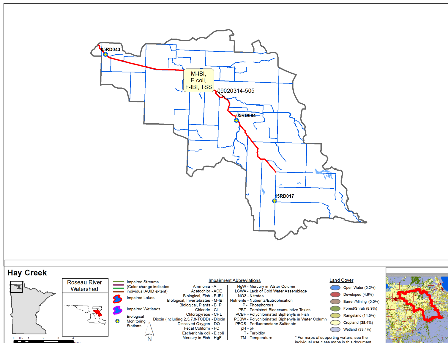
Figure 23. Currently listed impaired waters by parameter and land use characteristics in the Hay Creek Subwatershed.
