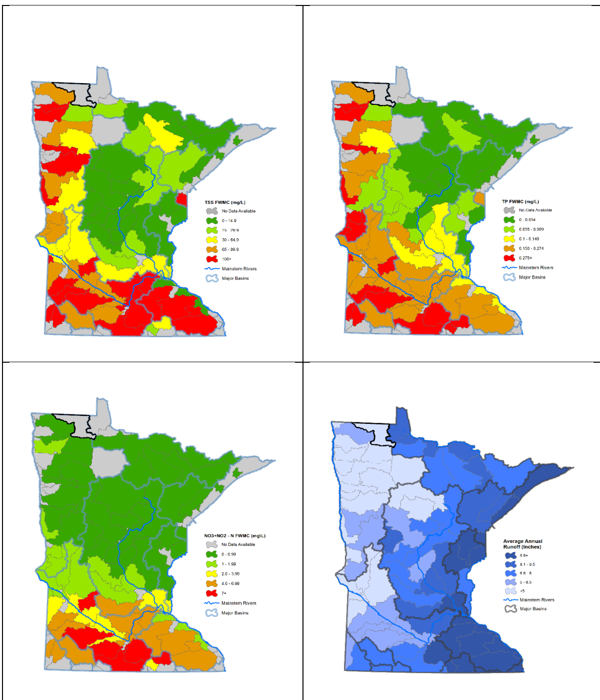
Figure 27. 2007-2015 average annual TSS, TP, and NO3-NO2-N flow weighted mean concentrations and runoff by major watershed.
