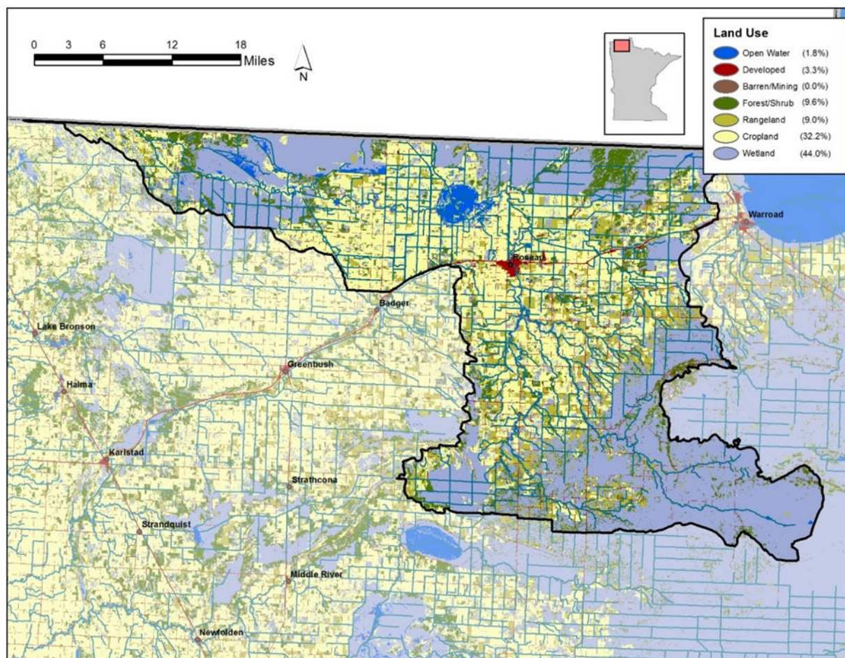
Figure 5. Land use in the Roseau River Watershed.
