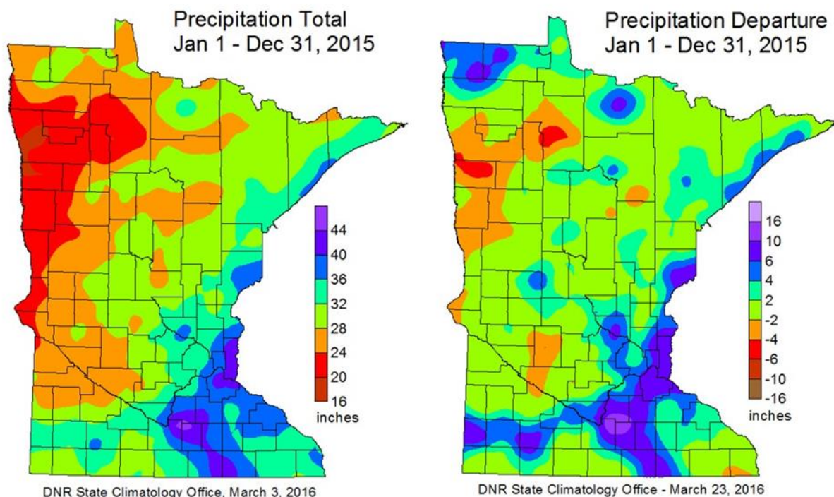
Figure 7. Statewide precipitation total (left) and precipitation departure (right) during 2015 (Source: DNR 2016a).
