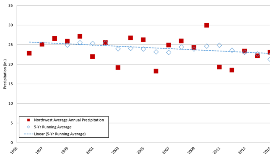
Figure 8. Precipitation trends in Northwest Minnesota (1996-2015) with five-year running average (Source: WRCC 2017).
