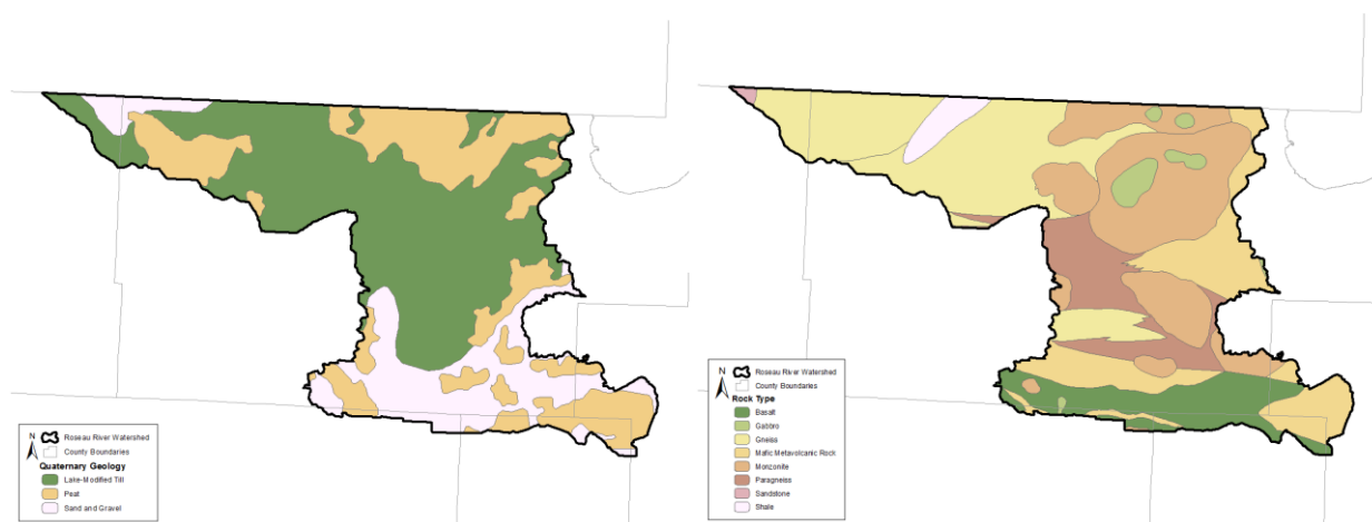
Figure 10. Quaternary geology (left) and bedrock geology rock types (right) within the Roseau River Watershed.
