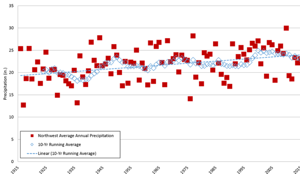
Figure 9. Precipitation trends in Northwest Minnesota (1915-2015) with 10-year running average (Source: WRCC 2017).
