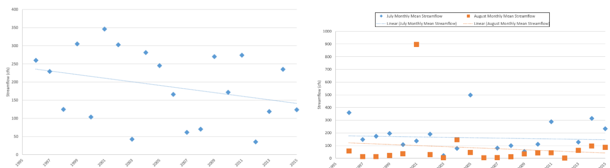
Figure 30. Annual mean (left) and monthly mean (right) streamflow for Roseau River near Malung (1996-2015) (Source: USGS 2018b)
