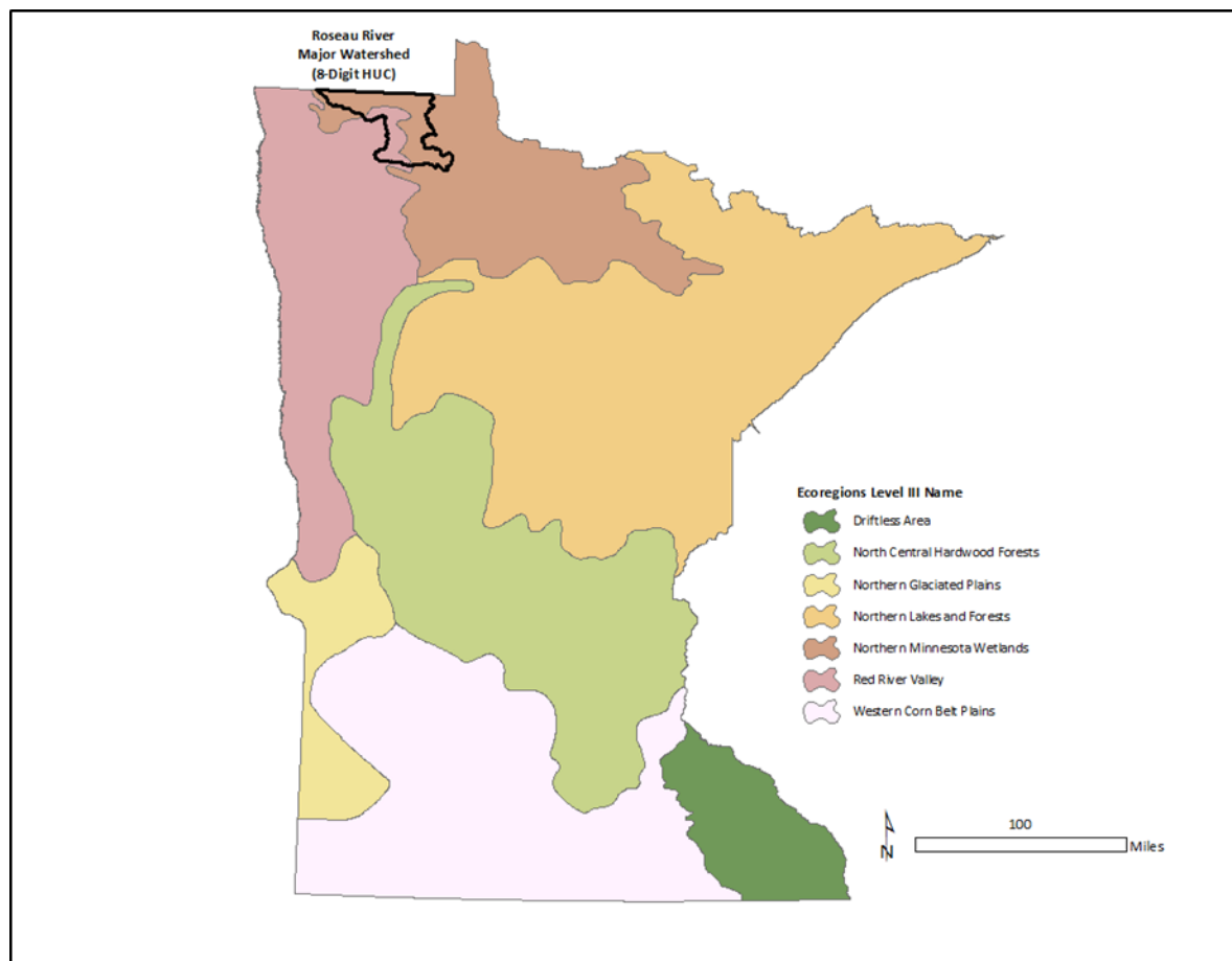
Figure 4. The Roseau River Watershed within the Northern Minnesota Wetlands and Red River Valley ecoregions of Northwest Minnesota.
