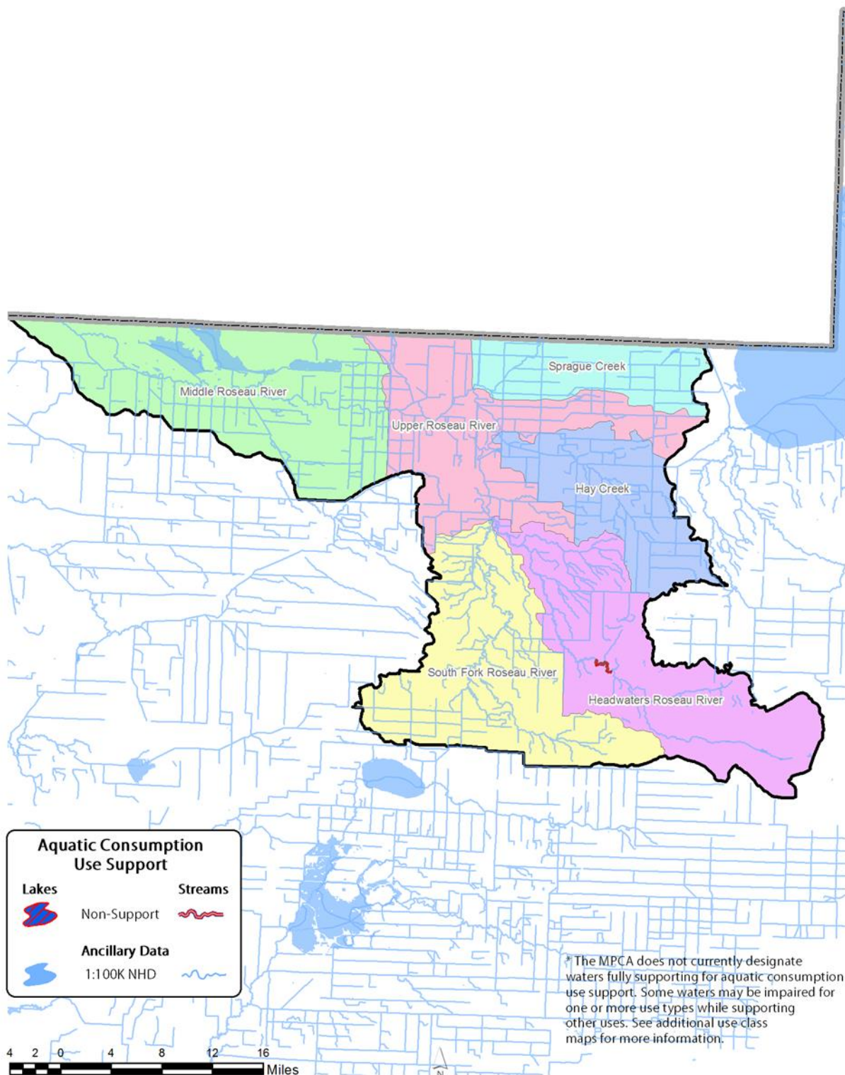
Figure 34. Aquatic consumption use support in the Roseau River Watershed.
