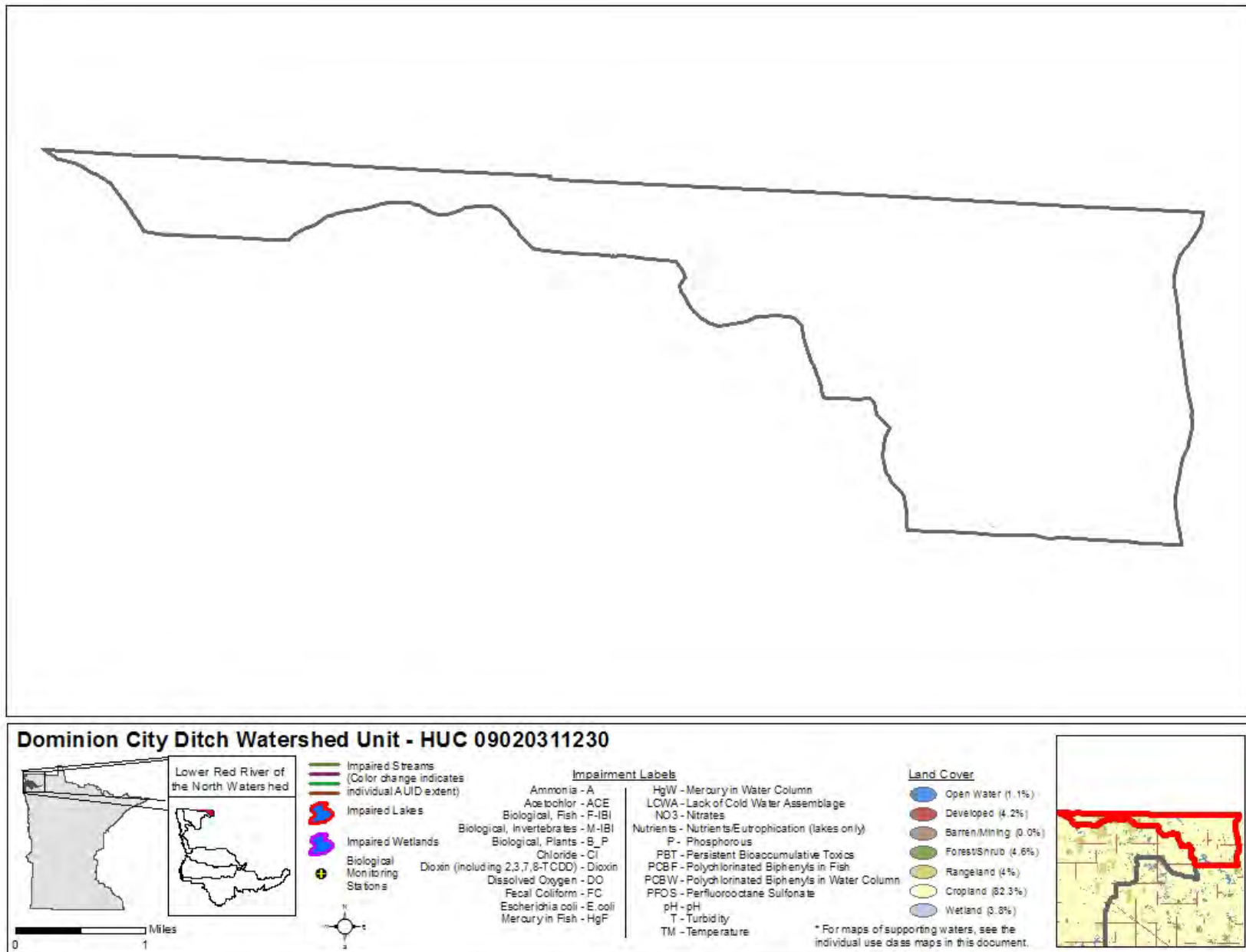
Figure 17. Currently listed impaired waters by parameters and land use characteristics in the Dominion City Ditch Watershed Unit
