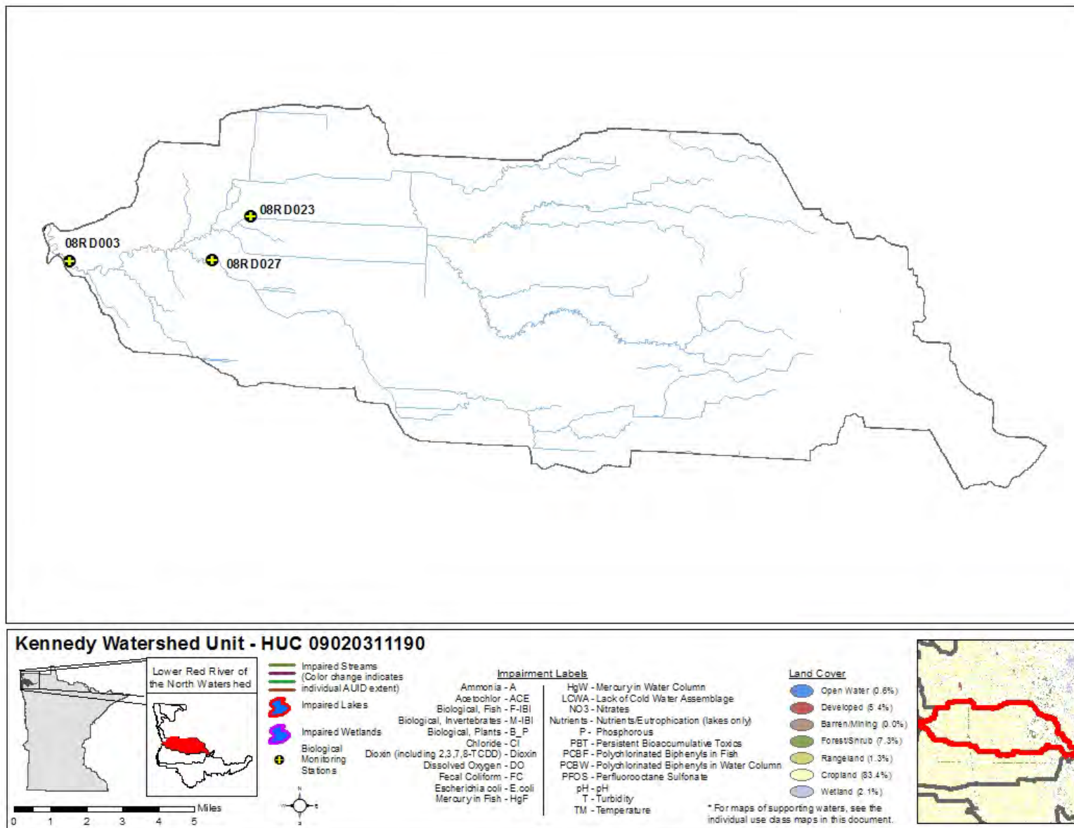
Figure 13. Currently listed impaired waters by parameters and land use characteristics in the Kennedy Watershed Unit
