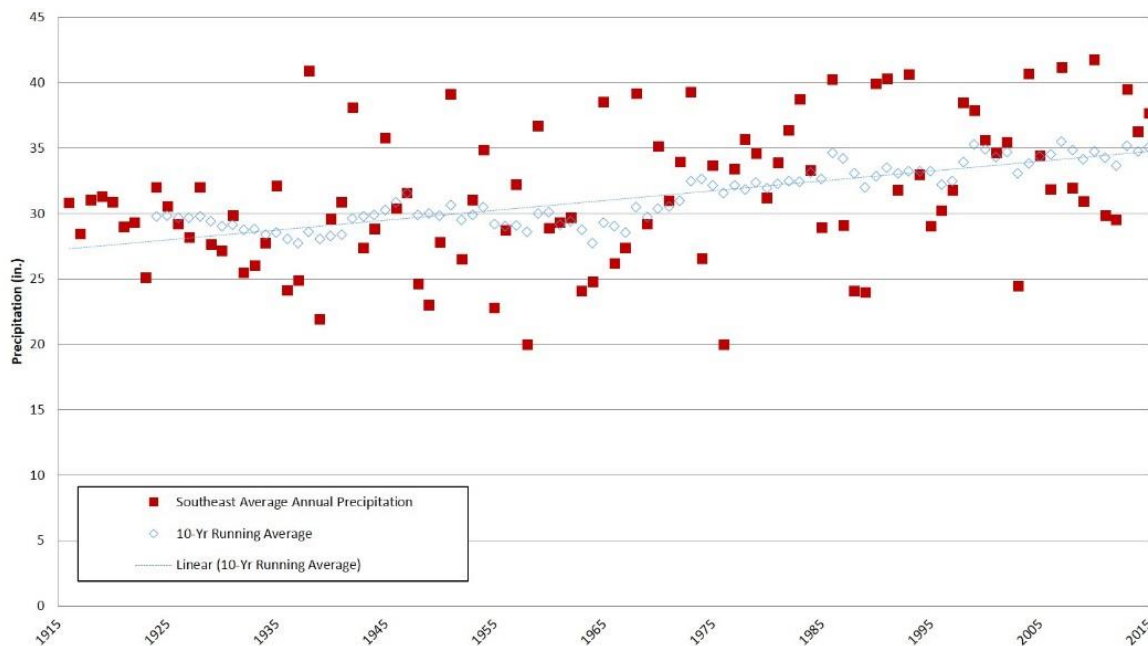
Figure 21. Precipitation trends in southeast Minnesota (1916-2015) with ten-year running average (WRCC, 2017)
