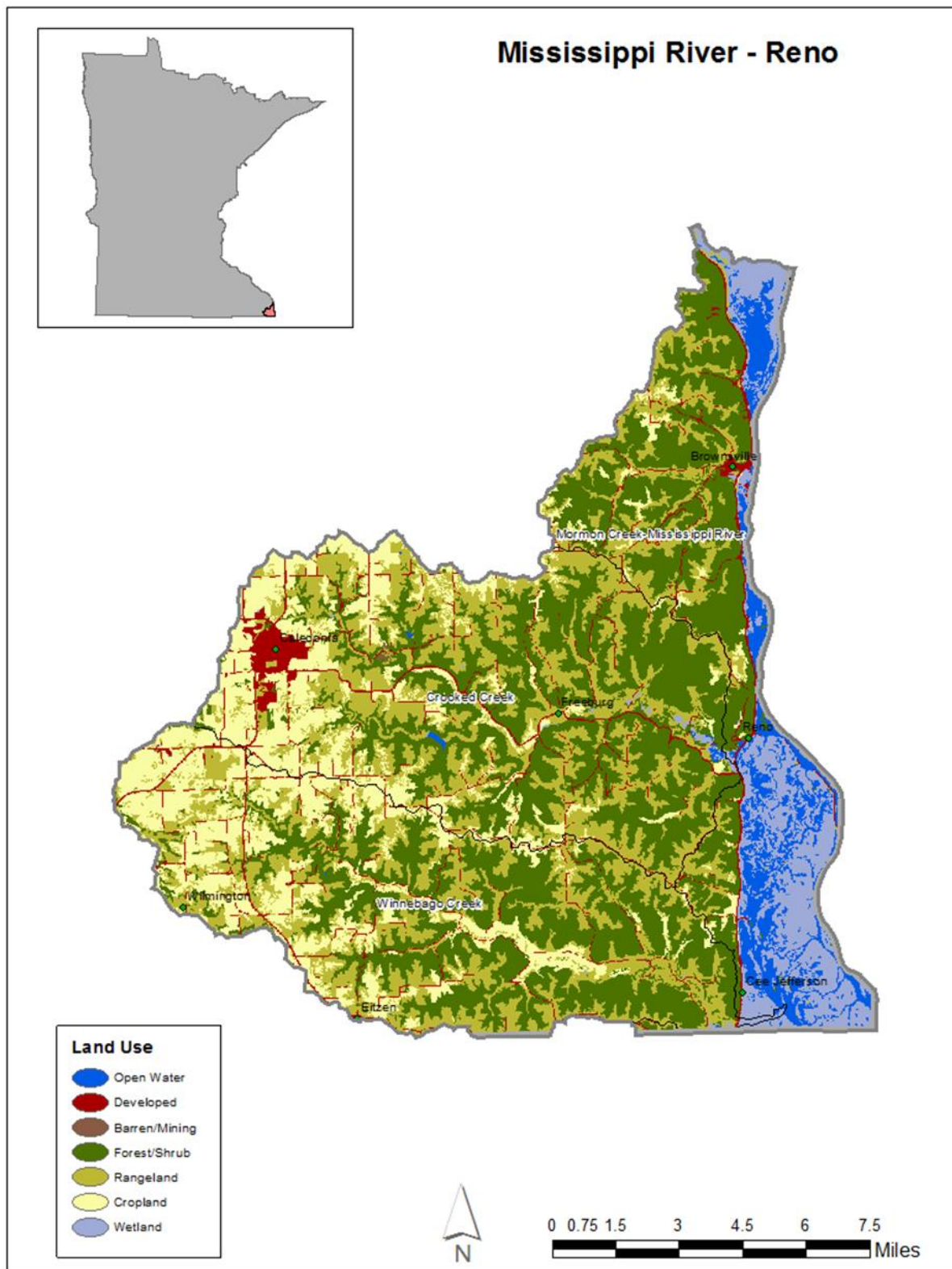
Figure 13. Land use in the Mississippi River-Reno watershed.
