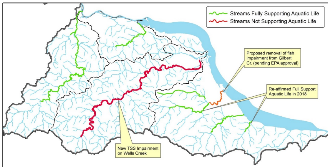
Figure 2. Summary of stream aquatic life assessments, including full support streams from 2011 assessment
