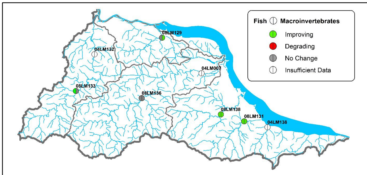
Figure 3. Biological condition comparison for each community type between 2008 and 2018.
