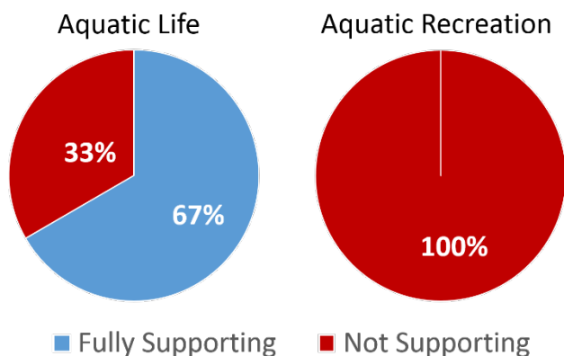
Figure 1. 2020 watershed assessment results for stream aquatic life and recreation.
