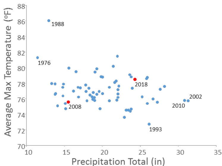
Figure 4. Characterization of air temperature and rainfall conditions for May-September period across the historical record of climate data for the MRLP watershed. Biological monitoring years highlighted in red.
