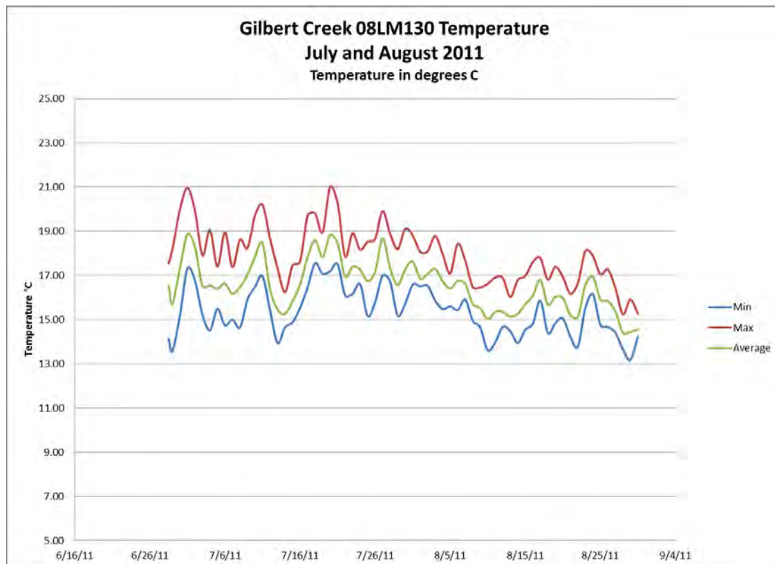
Figure 16: Temperature data collected for Gilbert Creek, July and August 2011
