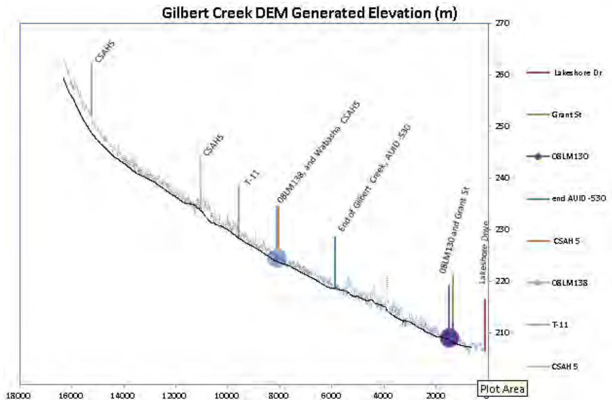
Figure 10: Elevation Profile of Gilbert Creek Watershed
