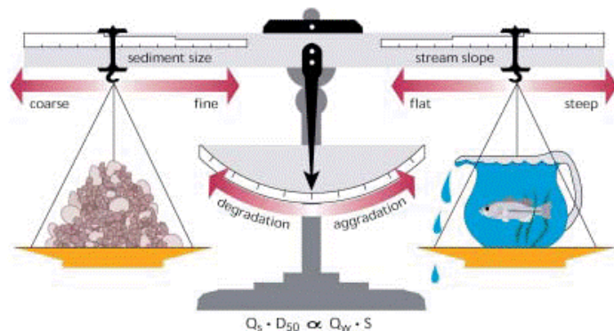
Figure 11: Generalized relationship of stream stability (Rosgen)
