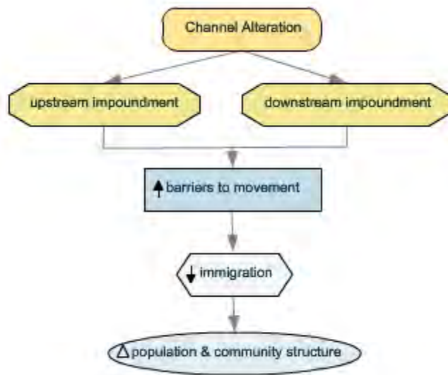
Figure 20: Conceptual Model for Connectivity
