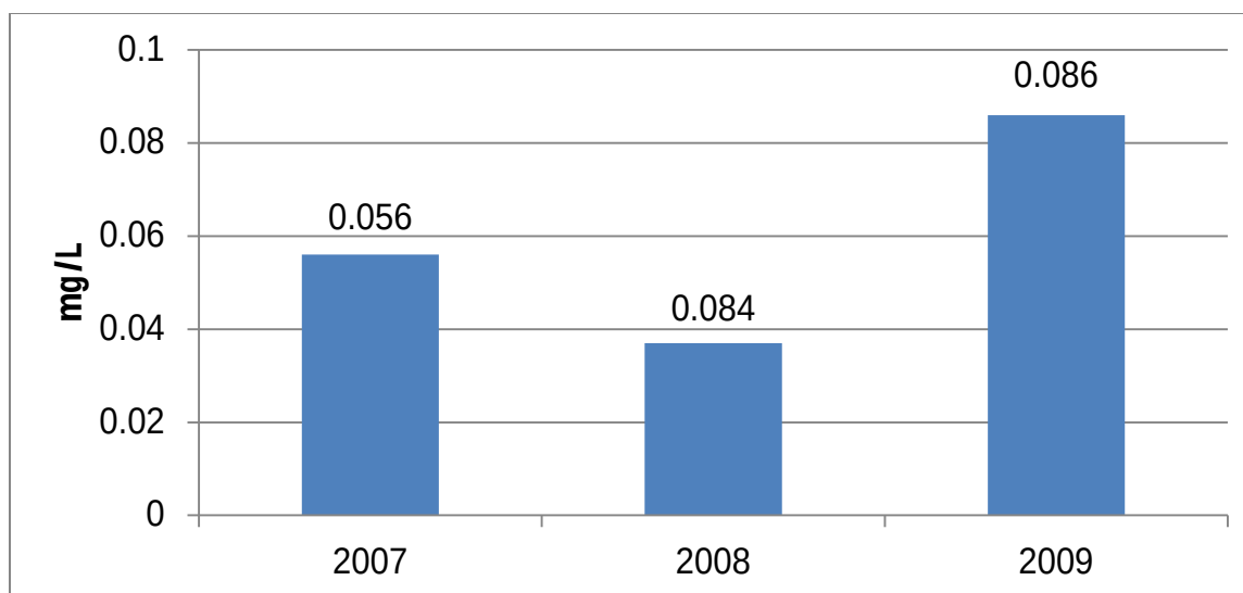
Figure 35. Dissolved Orthophosphate (DOP) Flow Weighted Mean Concentrations for the Chippewa River
