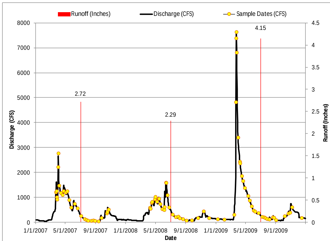
Figure 37. 2007-2009 Hydrograph, Sampling Regime and Annual Run-off for the Chippewa River near Milan, Minnesota
