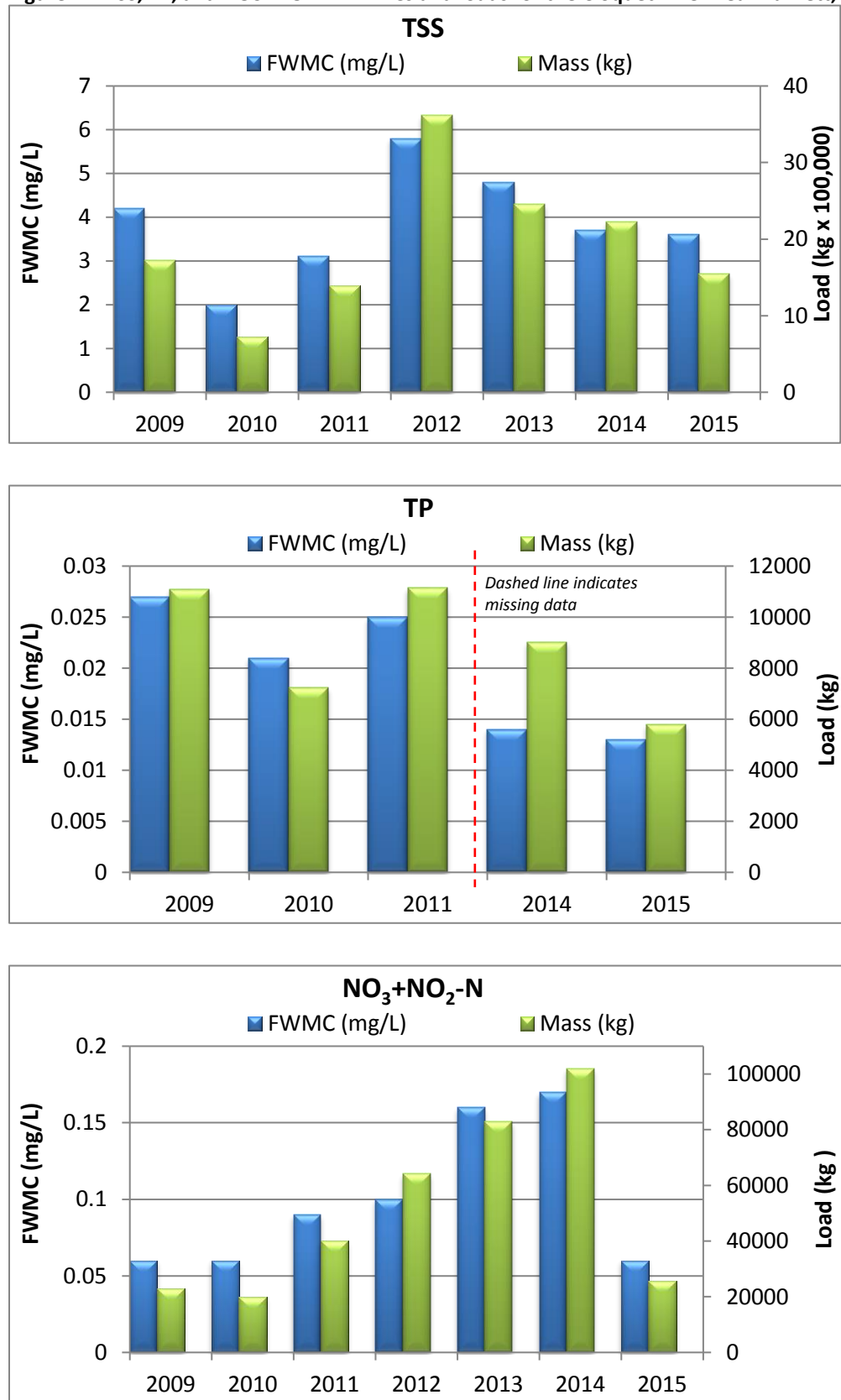
Figure 42. TSS, TP, and NO 3 +NO 2 -N FWMCs and loads for the Cloquet River near Burnett, MN.
