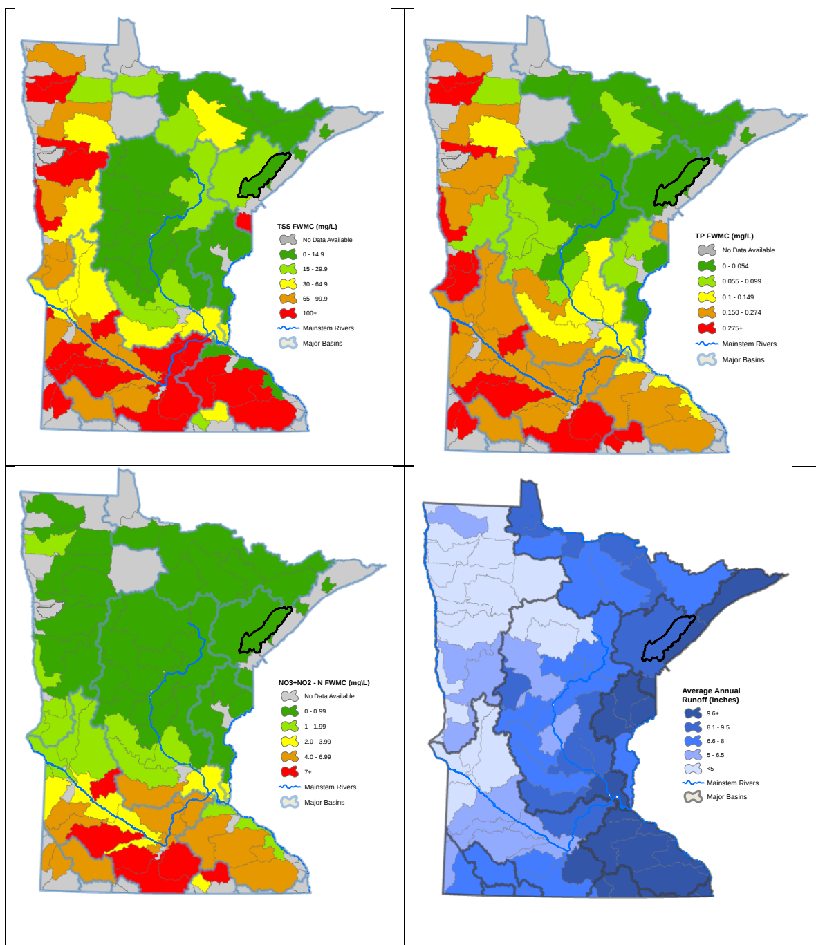
Figure 41. 2007-2015 Average annual TSS, TP, and NO 3 -NO 2 -N FVMCs, and runoff by major watershed.
