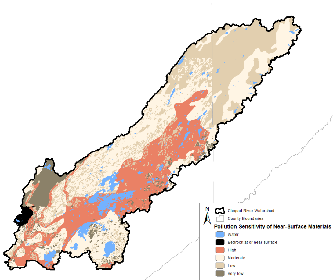
Figure 15. Pollution Sensitivity of Near-Surface Materials for the Cloquet River Watershed (GIS Source: DNR, 2016).
