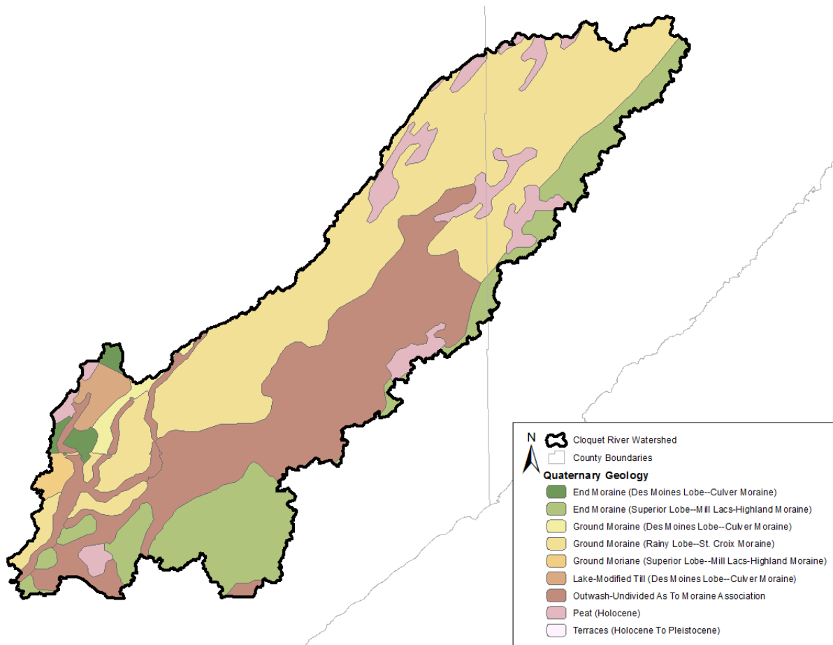
Figure 13. Quarternary geology within the Cloquet River Watershed (GIS Source: Hobbs & Goebel, 1982; Morey & Meints, 2000).
