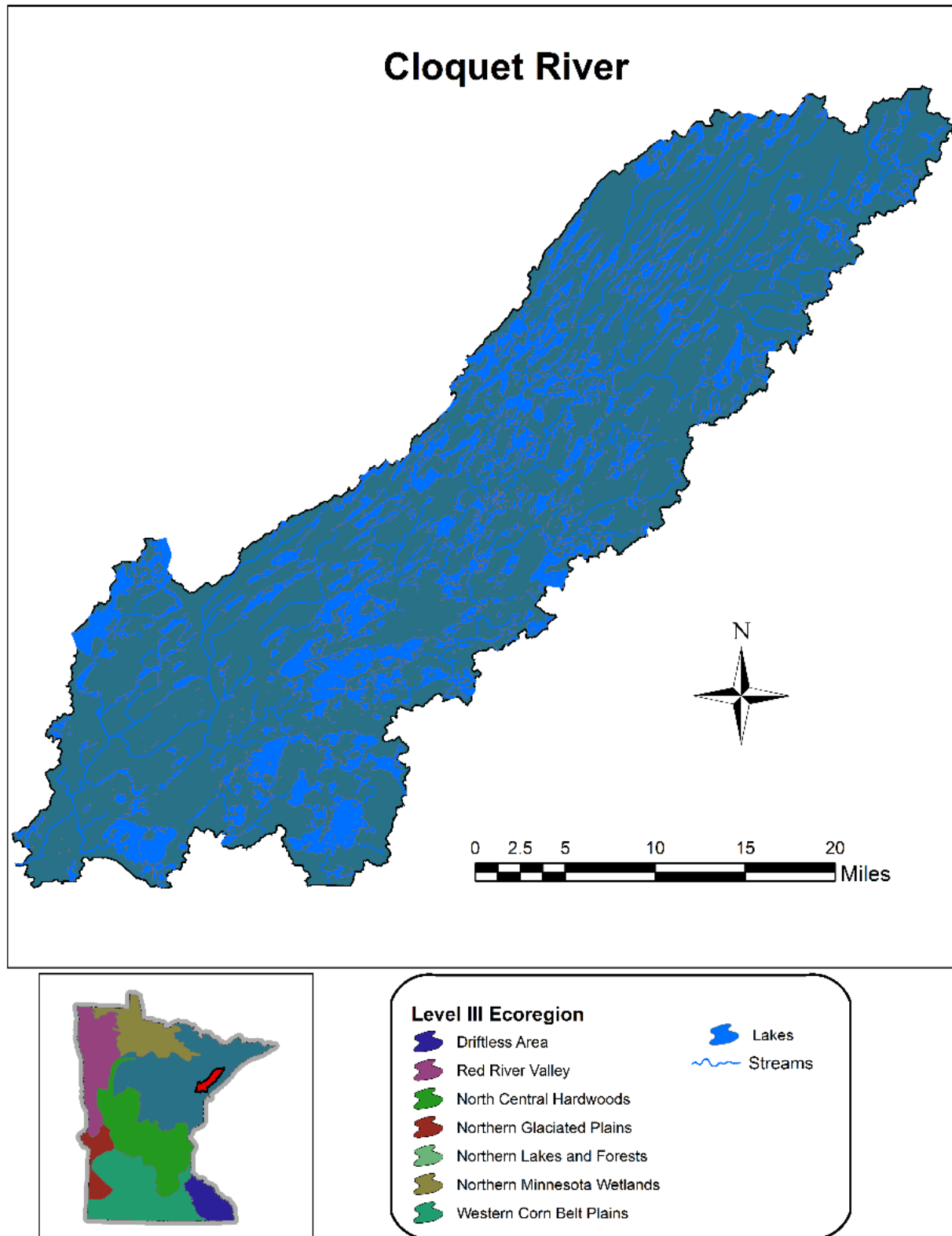
Figure 5. The Cloquet River Watershed within the Northern Lakes and Forest ecoregion of NE Minnesota.
