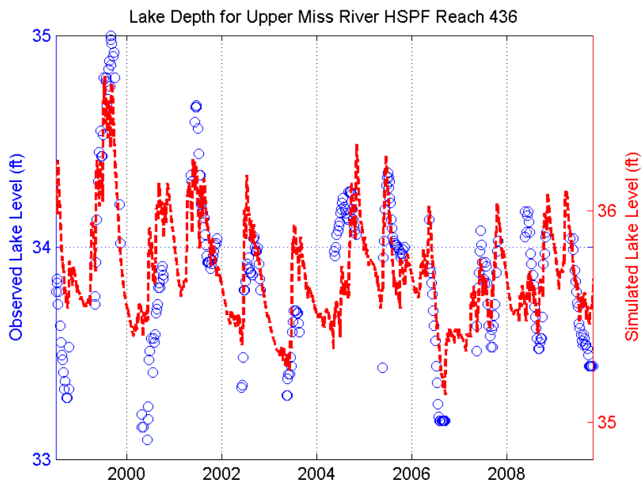
Figure A-18. Big Lake Level Time Series.
