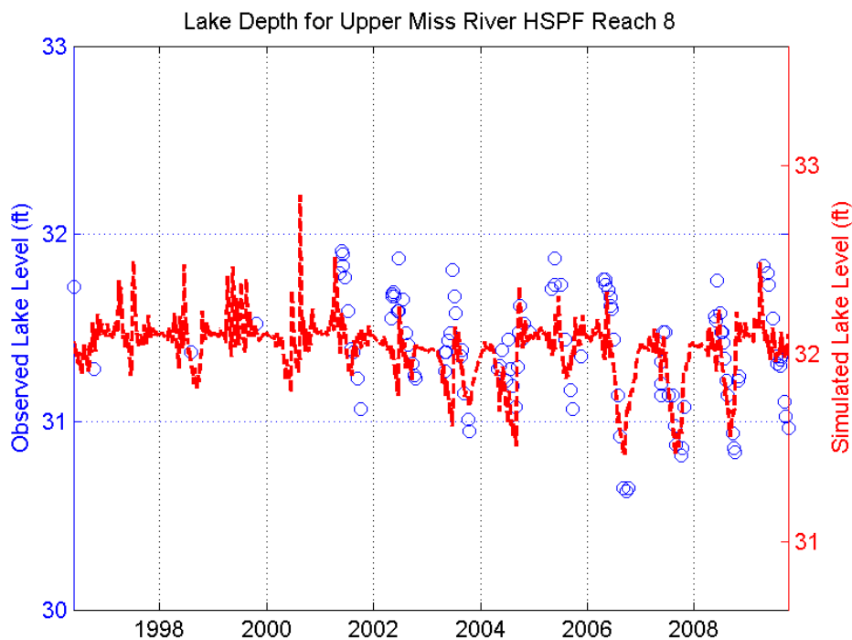
Figure B-1. Garfield Lake Level Time Series.
