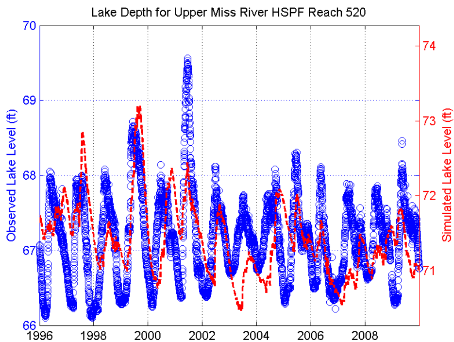
Figure A-24. Lake Winnibigoshish Level Time Series.
