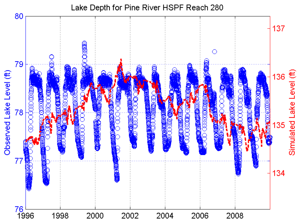
Figure C-8. Cross Lake Level Time Series.
