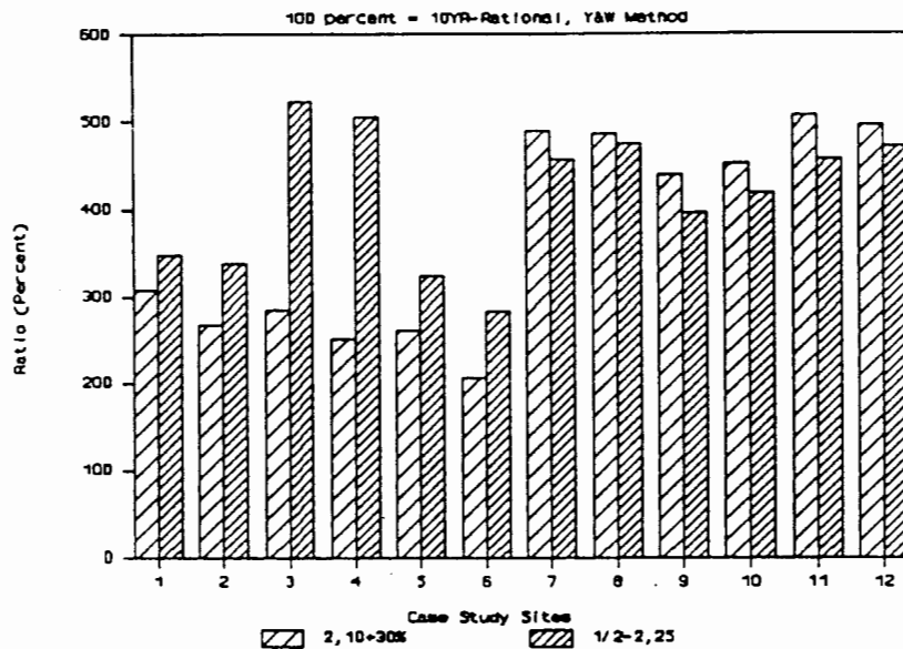
Figure AIII-4.7 - Comparison of detention volume for 2 and 10-year events plus 30 percent, and 1/2-2,25-year events
