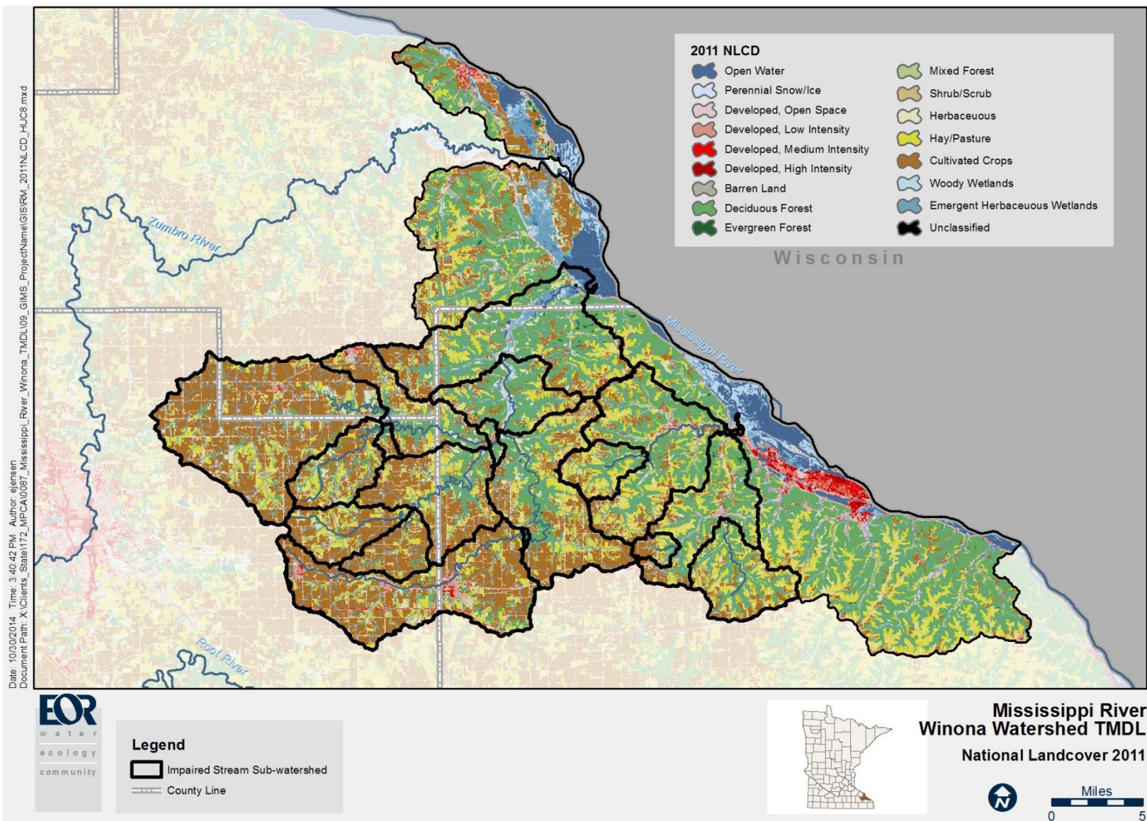
Figure 5. Mississippi River – Winona Watershed Land Cover (2011 NLCD)
