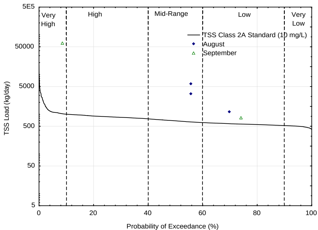
Figure 38. Total suspended solids load duration curve for Whitewater River, North Fork (07040003-523)
