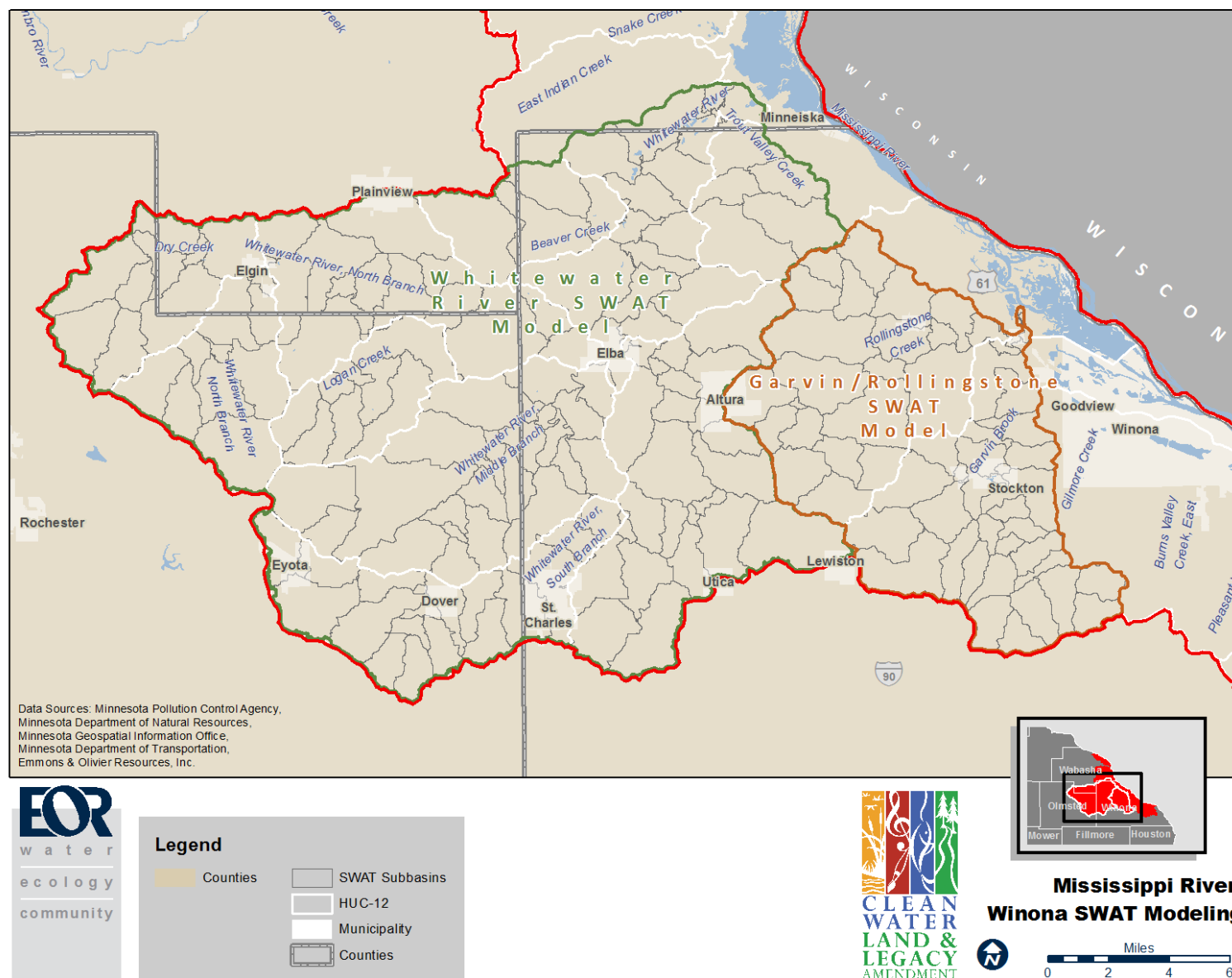
Figure 20. Whitewater River and Garvin/Rollingstone SWAT Model boundaries within the Mississippi River-Winona Watershed
