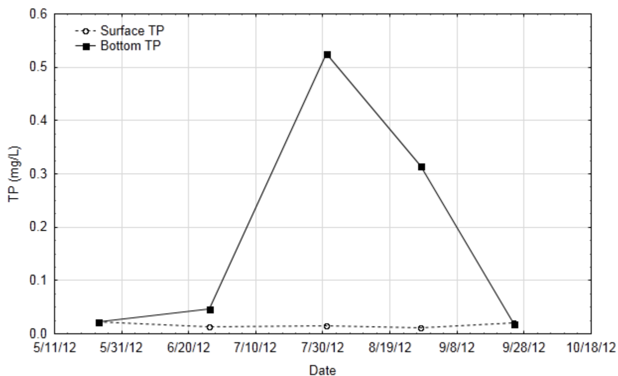
Figure 38. Bottom and surface TP concentrations, Latimer Lake, 2012
