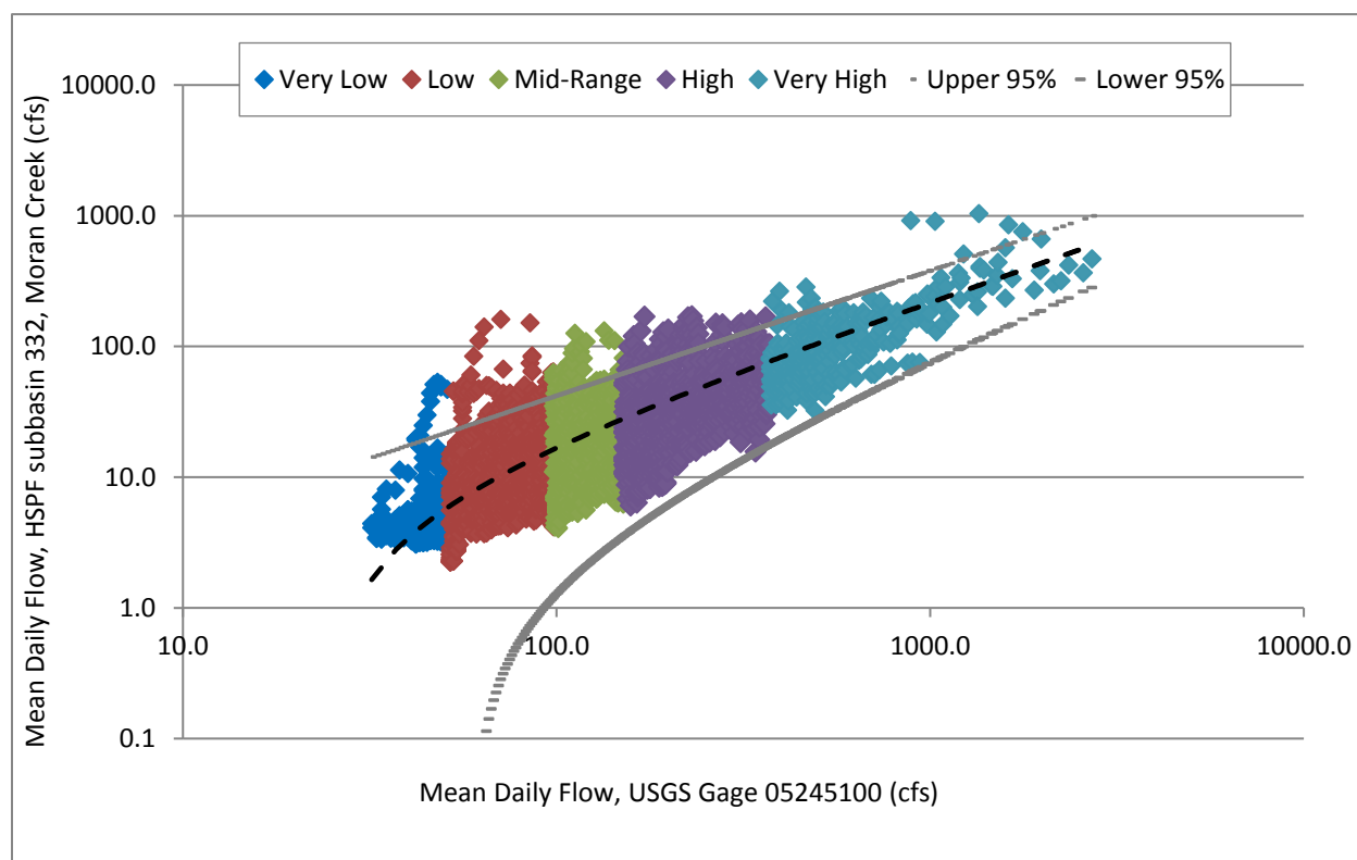
Figure 49. Moran Creek HSPF flows vs. USGS gaged flow for the Long Prairie River near Long Prairie at CSAH 11, 2000 to 2009. Note that flows are plotted on a log-log scale.
