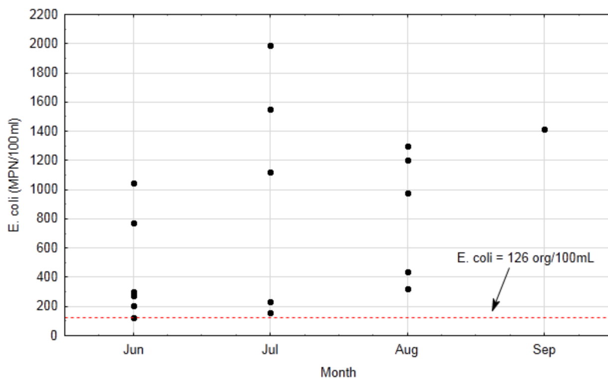
Figure 12. E. coli (MPN/100mL) by month in Unnamed Creek at monitoring station S001-780, 2004 to 2013
