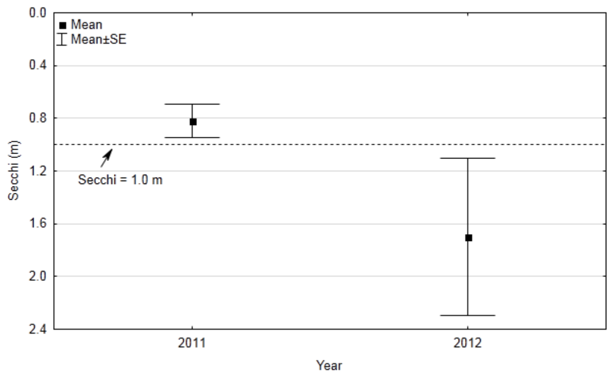
Figure 48. Growing Season Means \pm SE of Secchi transparency for Twin Lake by Year
