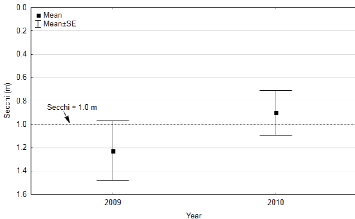
Figure 27. Growing Season Means \pm SE of Secchi transparency for Fish Lake by Year
