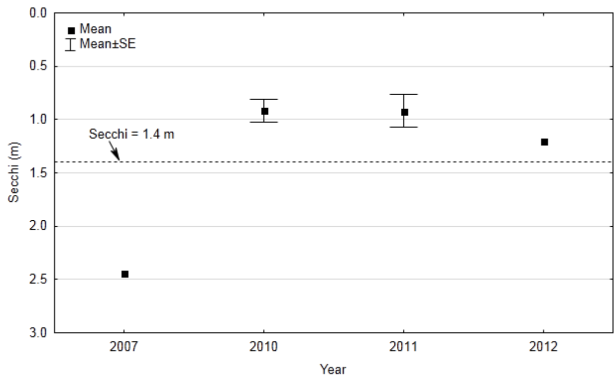
Figure 17. Growing Season Means \pm SE of Secchi transparency for Crooked (East) Lake by Year
