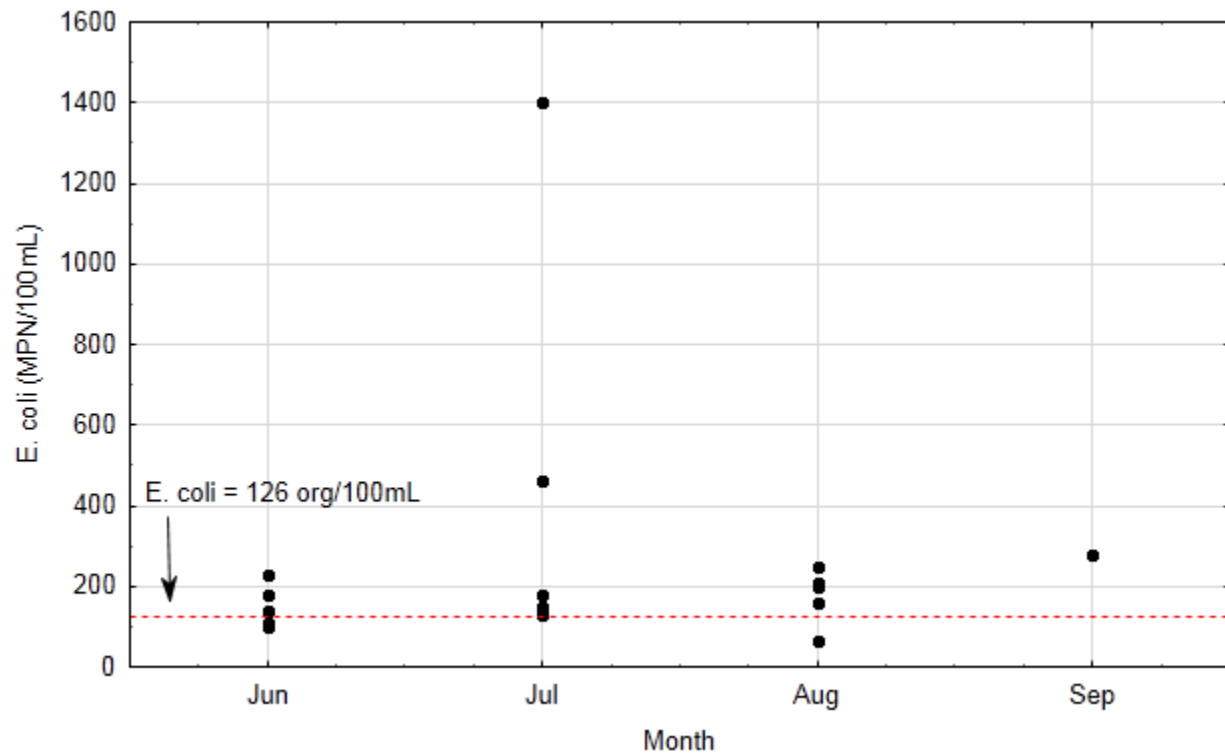
Figure 11. E. coli (MPN/100mL) by month in Moran Creek at monitoring station S002-903, 2004 to 2013
