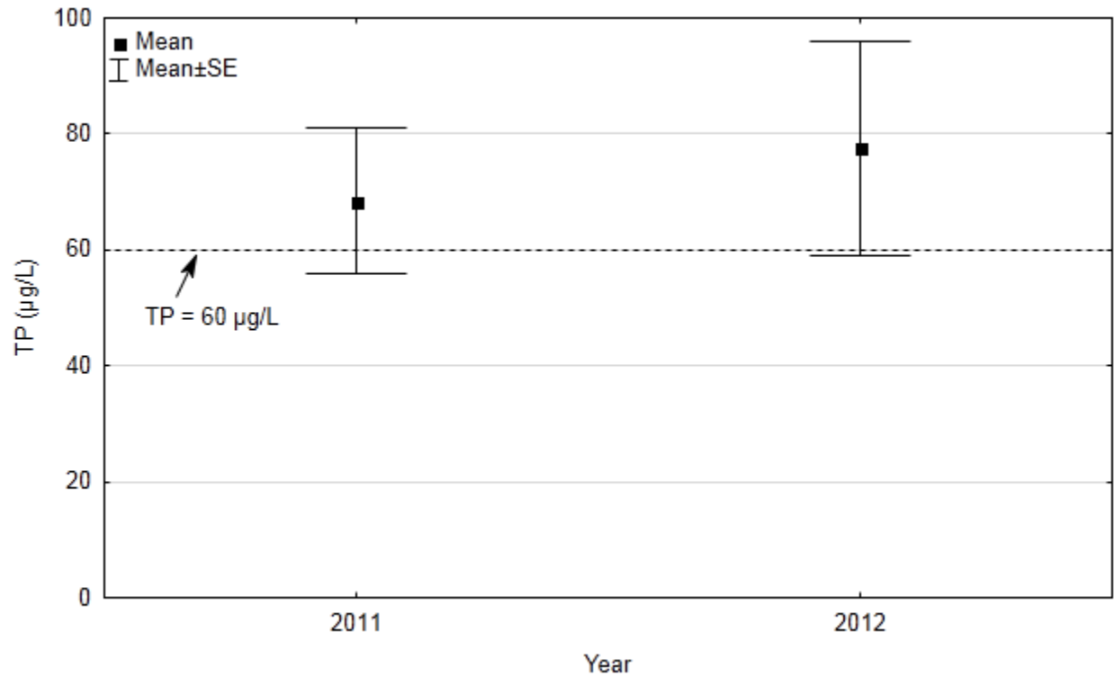
Figure 42. Growing Season Means \pm SE of Total Phosphorus for Nelson Lake by Year.
