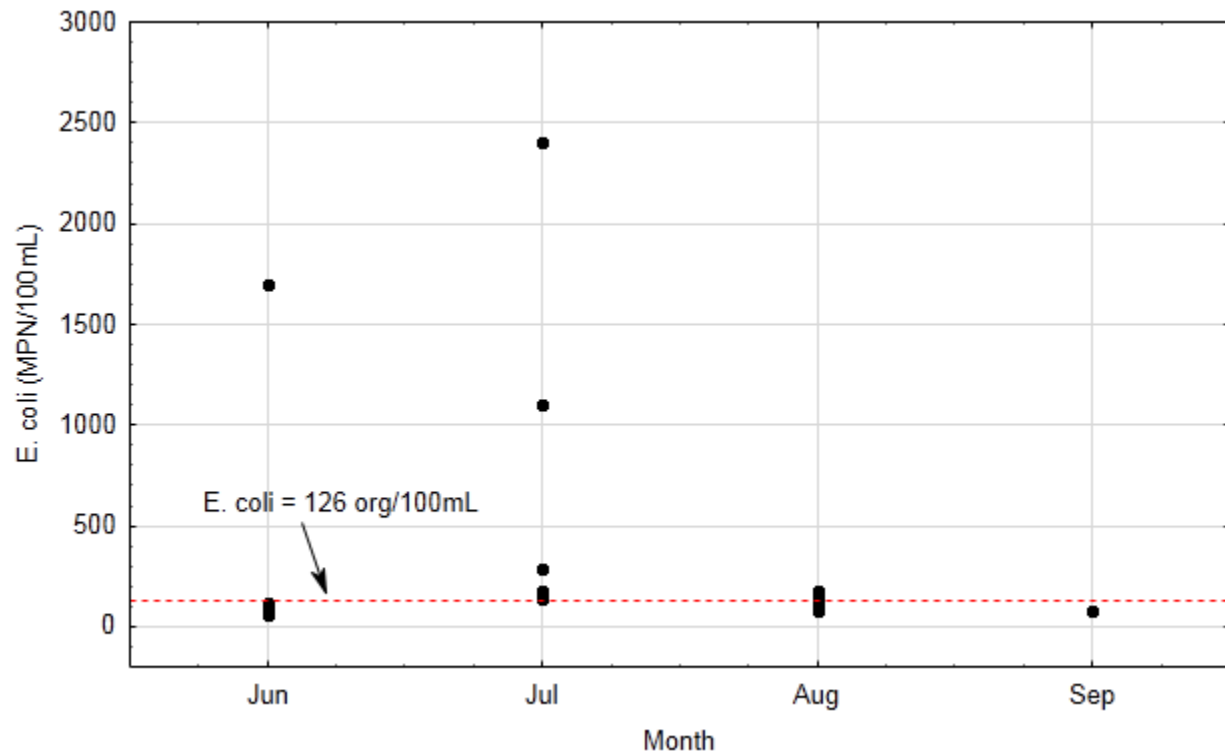
Figure 10. E. coli (MPN/100mL) by month in Eagle Creek at monitoring station S000-723, 2004 to 2013
