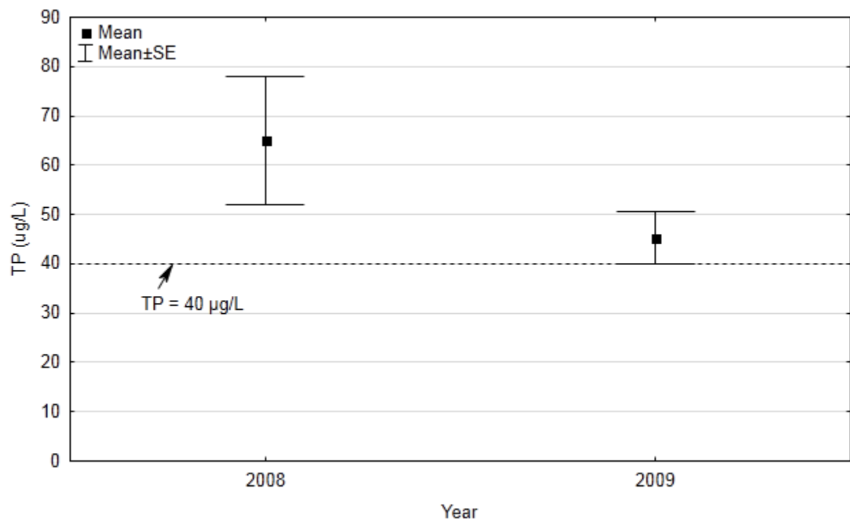
Figure 30. Growing Season Means \pm SE of Total Phosphorus for Jessie Lake by Year.
