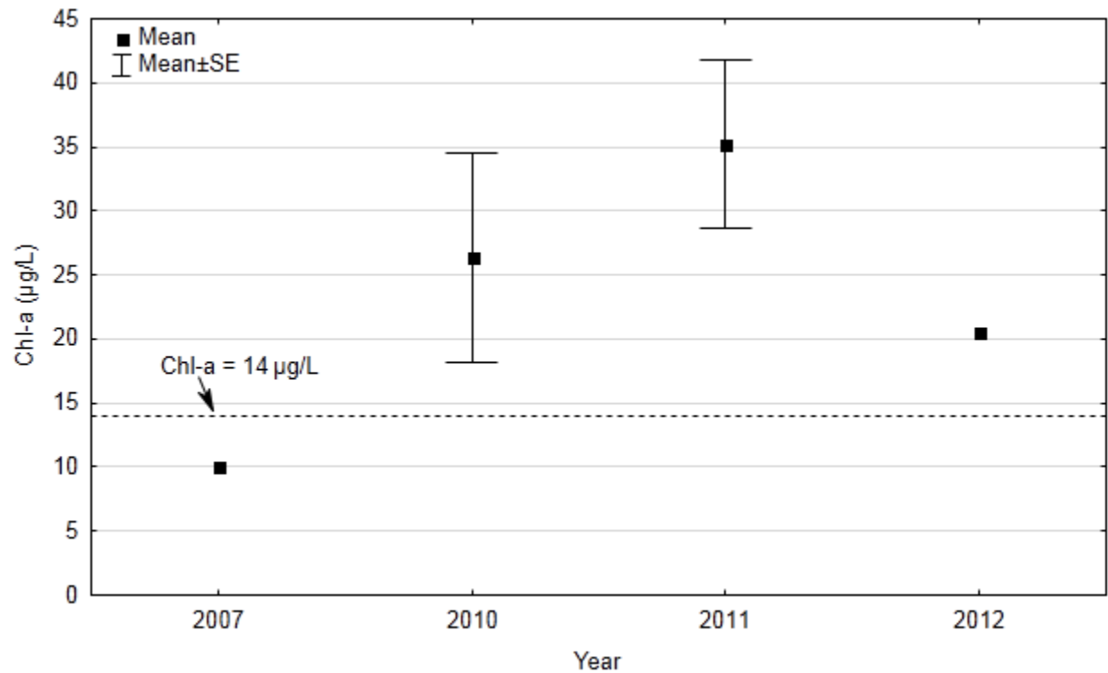
Figure 16. Growing Season Means \pm SE of Chl-a for Crooked (East) Lake by Year.
