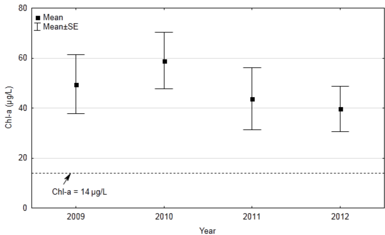
Figure 36. Growing Season Means ± SE of Chl- a for Latimer Lake by Year.
