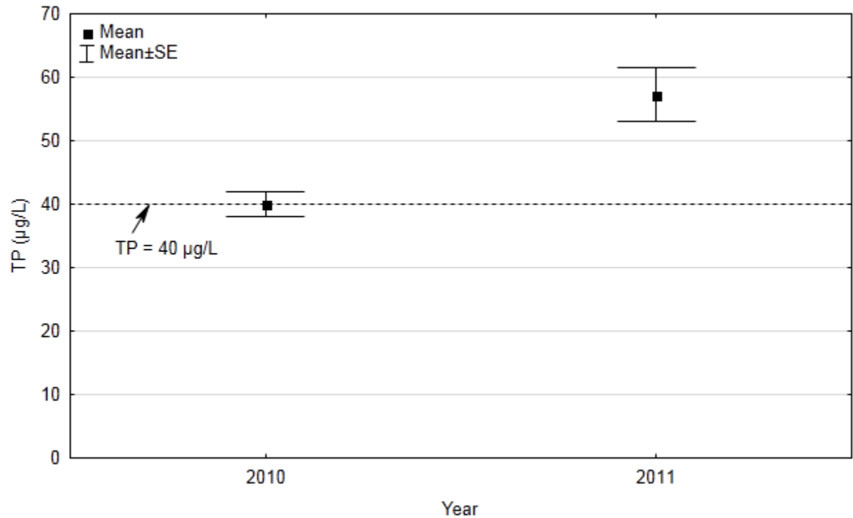
Figure 20. Growing Season Means \pm SE of Total Phosphorus for Echo Lake by Year.
