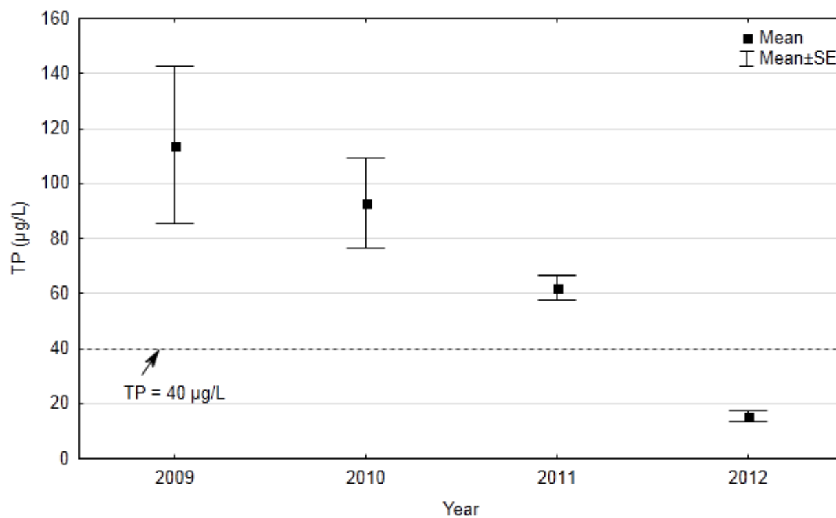
Figure 35. Growing Season Means \pm SE of Total Phosphorus for Latimer Lake by Year.
