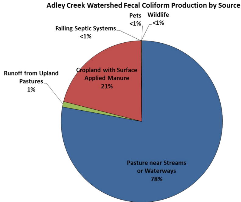
Figure 2.16. Fecal coliform available (by source) for delivery in the Adley Creek impaired reach watershed.
