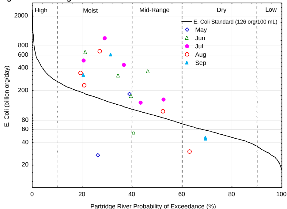
Figure 17. Partridge River E. coli Load Duration Curve
