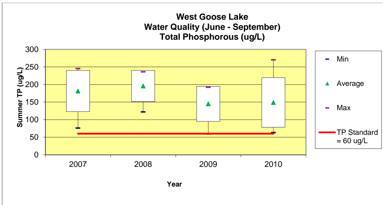
Figure 3.10. West Goose Lake Total Phosphorus Concentrations (June – September).
