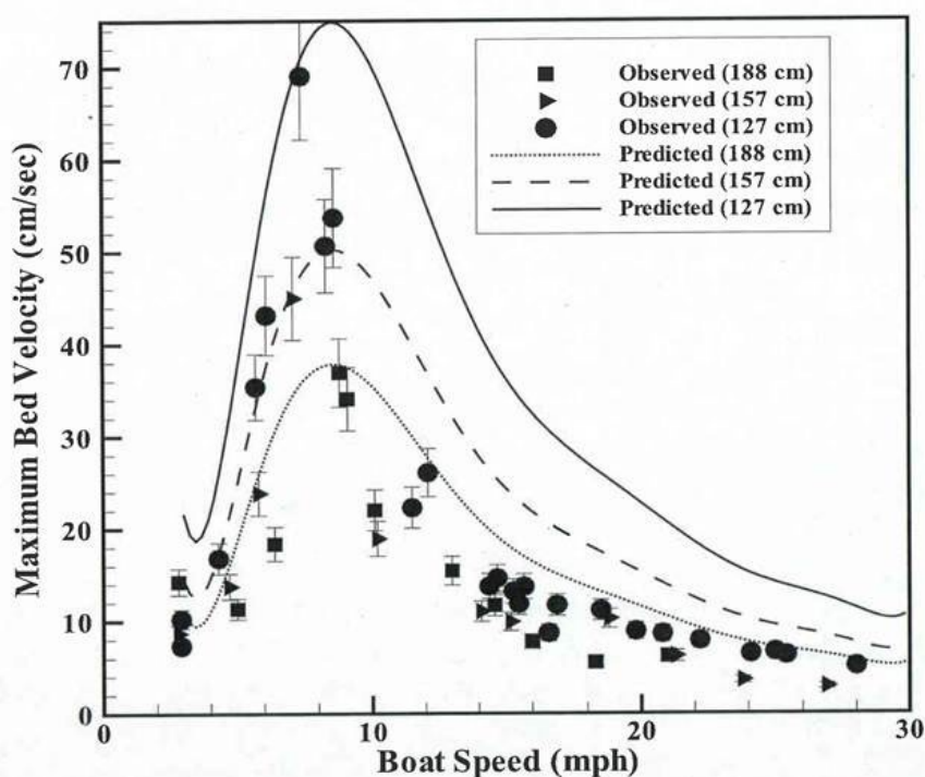
Figure 4.1. Sediment Bed Velocity and Boat Speed. (Source: Beachler and Hill 2003)
