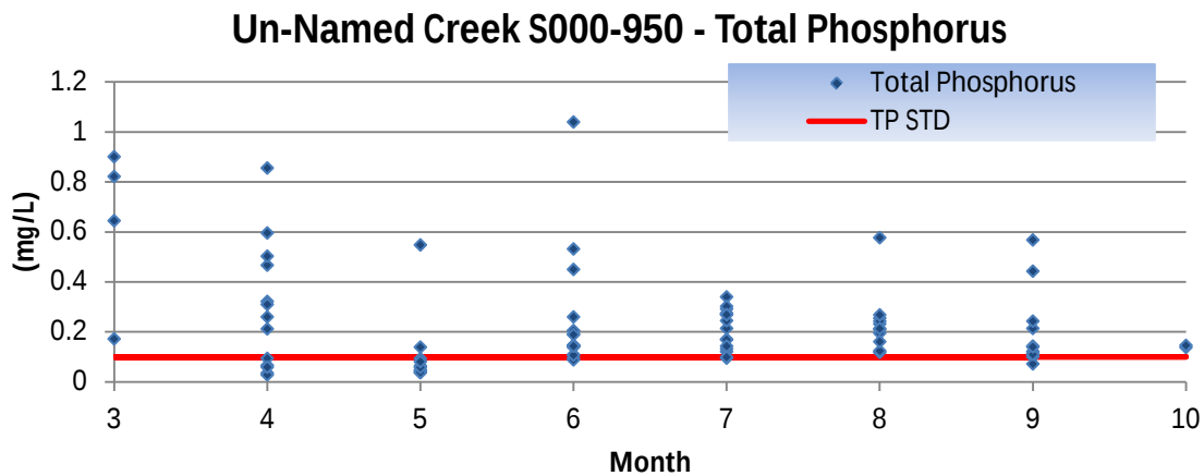
Figure 69: TP values composited by month from Un-named Creek EQuIS sites (2000-2010).
