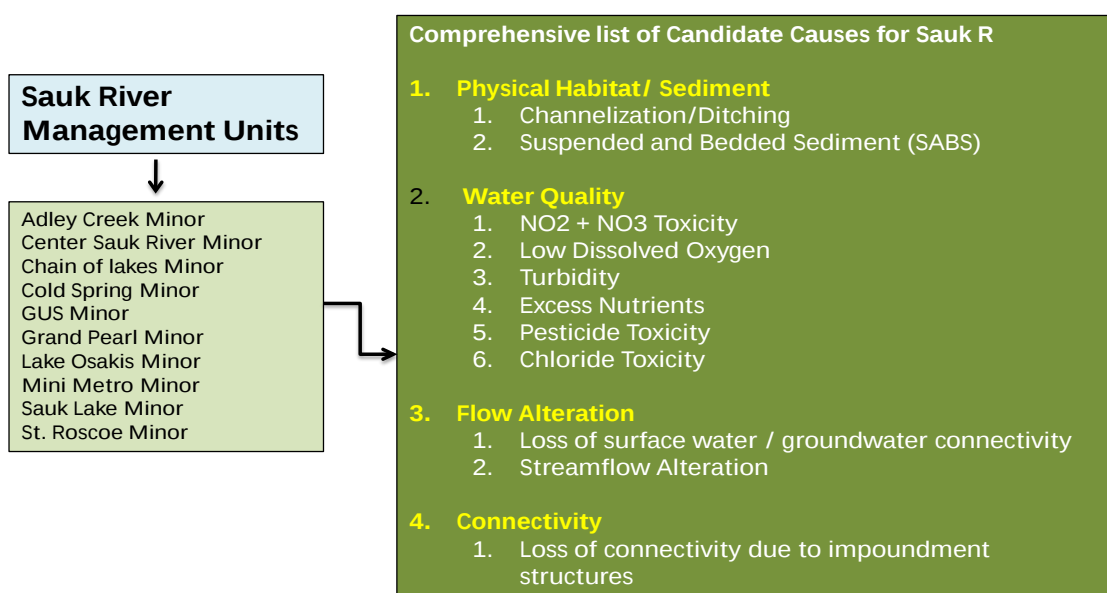
Figure 6: List of candidate causes for biological impairment in the Sauk River watershed
