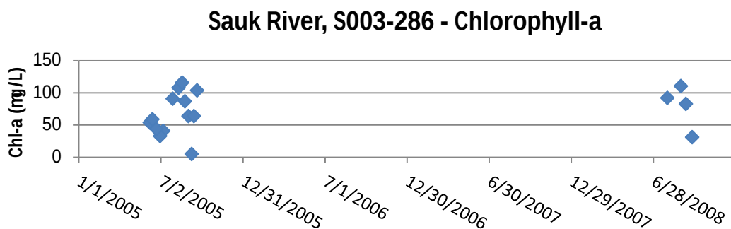
Figure 95: Chlorophyll-a data from EQuIS site S003-286
