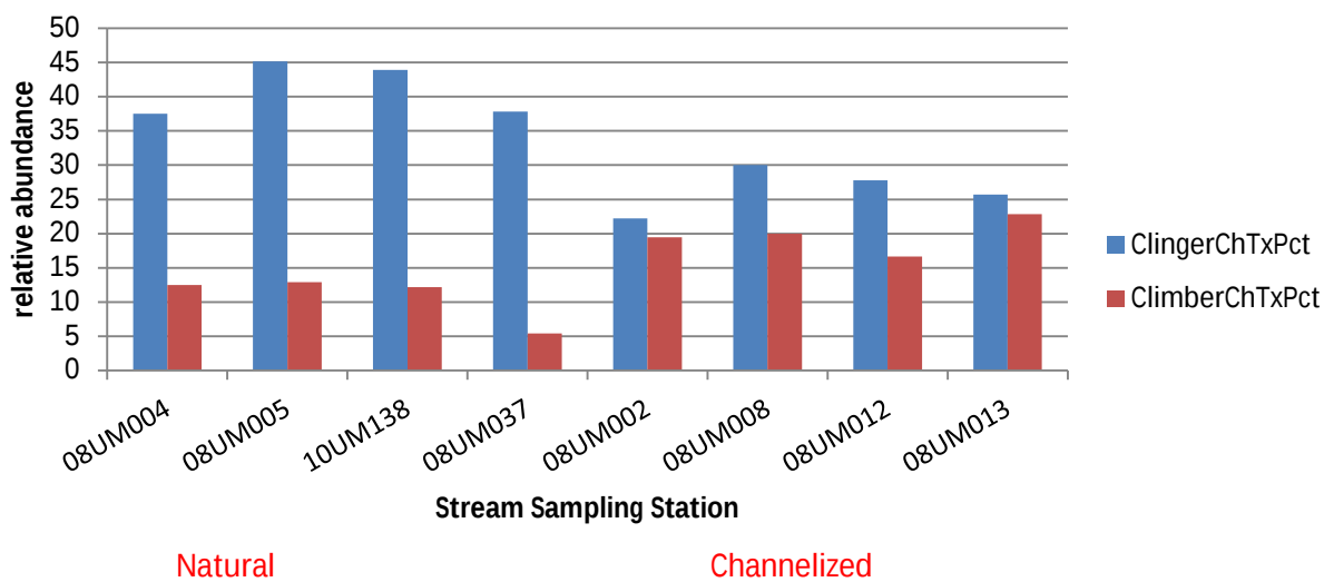
Figure 15: Macroinvertebrate taxa percent of the functional groups clingers and climbers and their relative abundance for natural versus channelized streams
