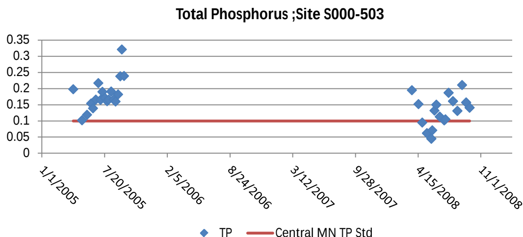
Figure 111: Sauk River downstream of CSAH-4 in St Cloud; TP concentrations
