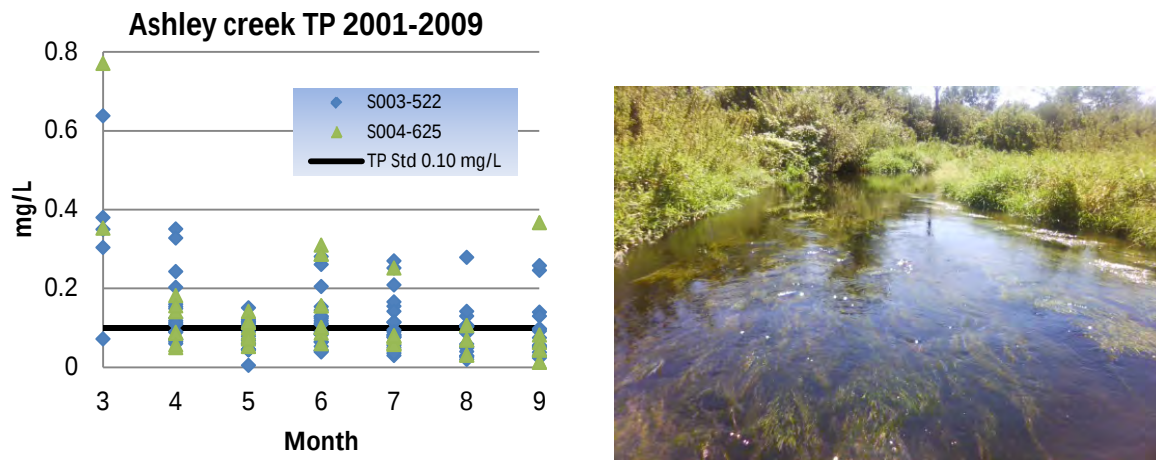
Figure 40: TP values over time collected from Ashley Creek STORET sites, excessive plant growth.
