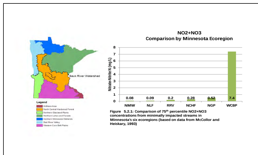
Figure 27: Comparison of 75th percentile NO 2 +NO 3 concentrations from minimally impacted streams in Minnesota's six ecoregions (based on McCollor and Heiskary, 1993).
