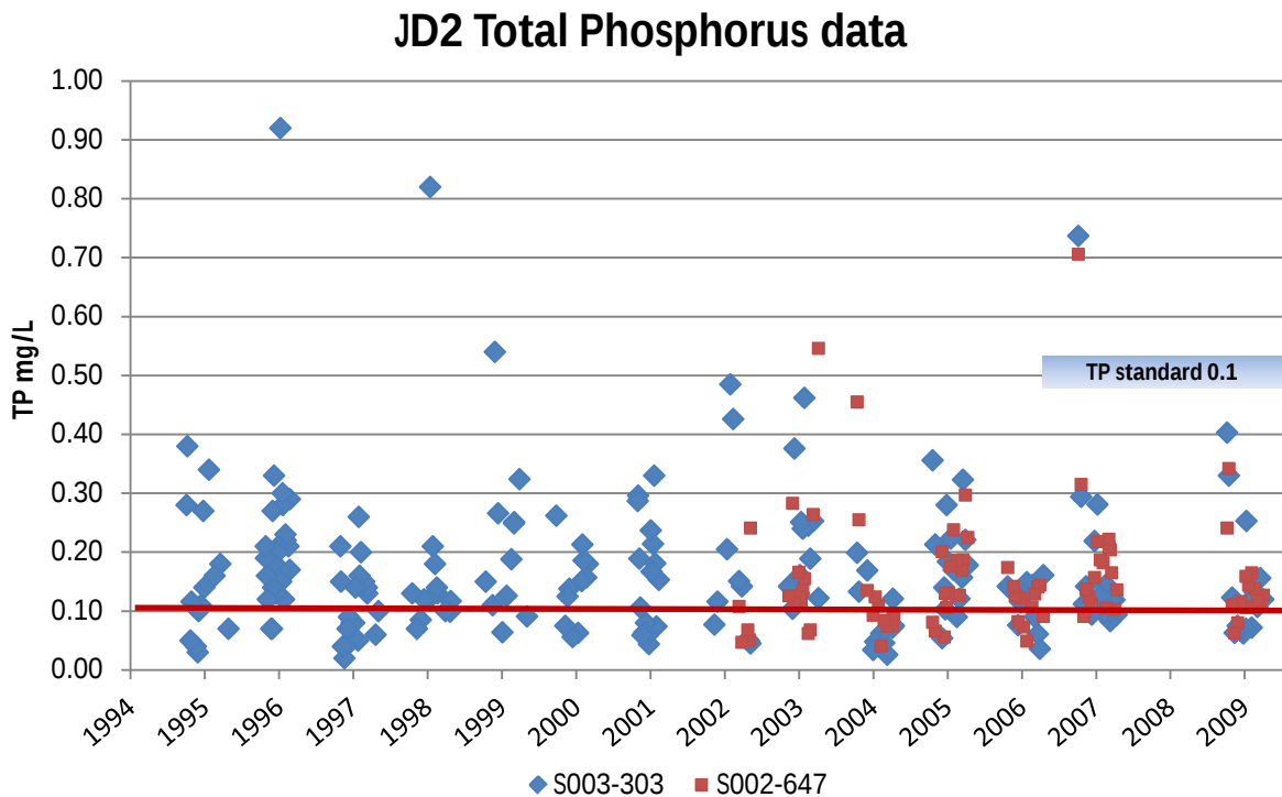
Figure 33: TP values over time collected from Crooked Lake Ditch (JD2)
