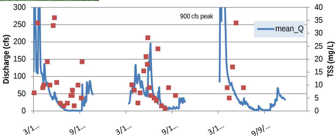
Figure 49: Ashley Creek at CR11; Flow versus TSS
