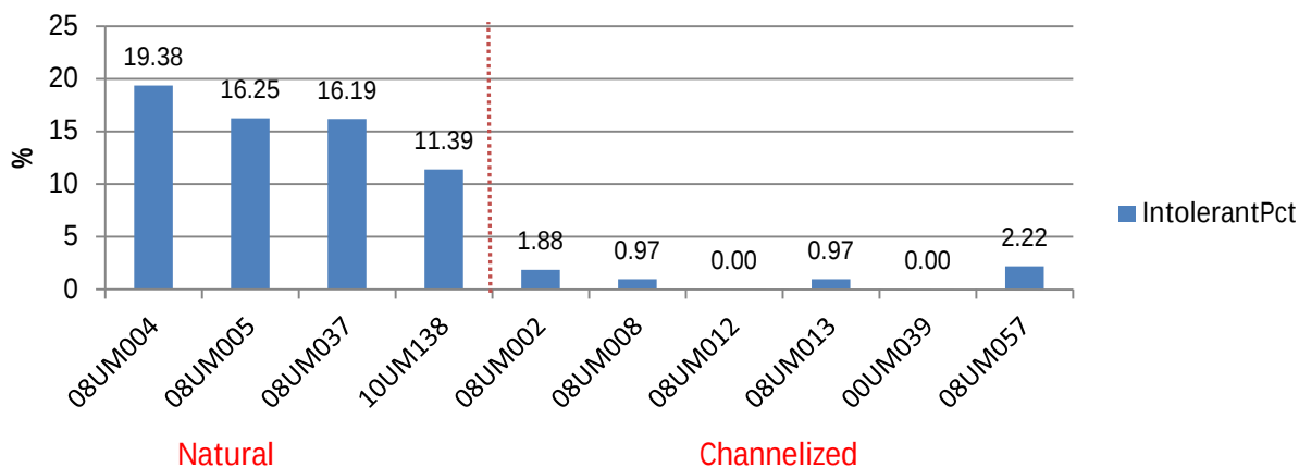
Figure 16: Macroinvertebrate percentage of intolerant taxa found in each stream sampling site.
