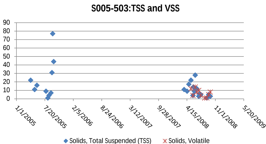
Figure 112: TSS and VSS concentrations for the Sauk River in St Cloud at CSAH4.
