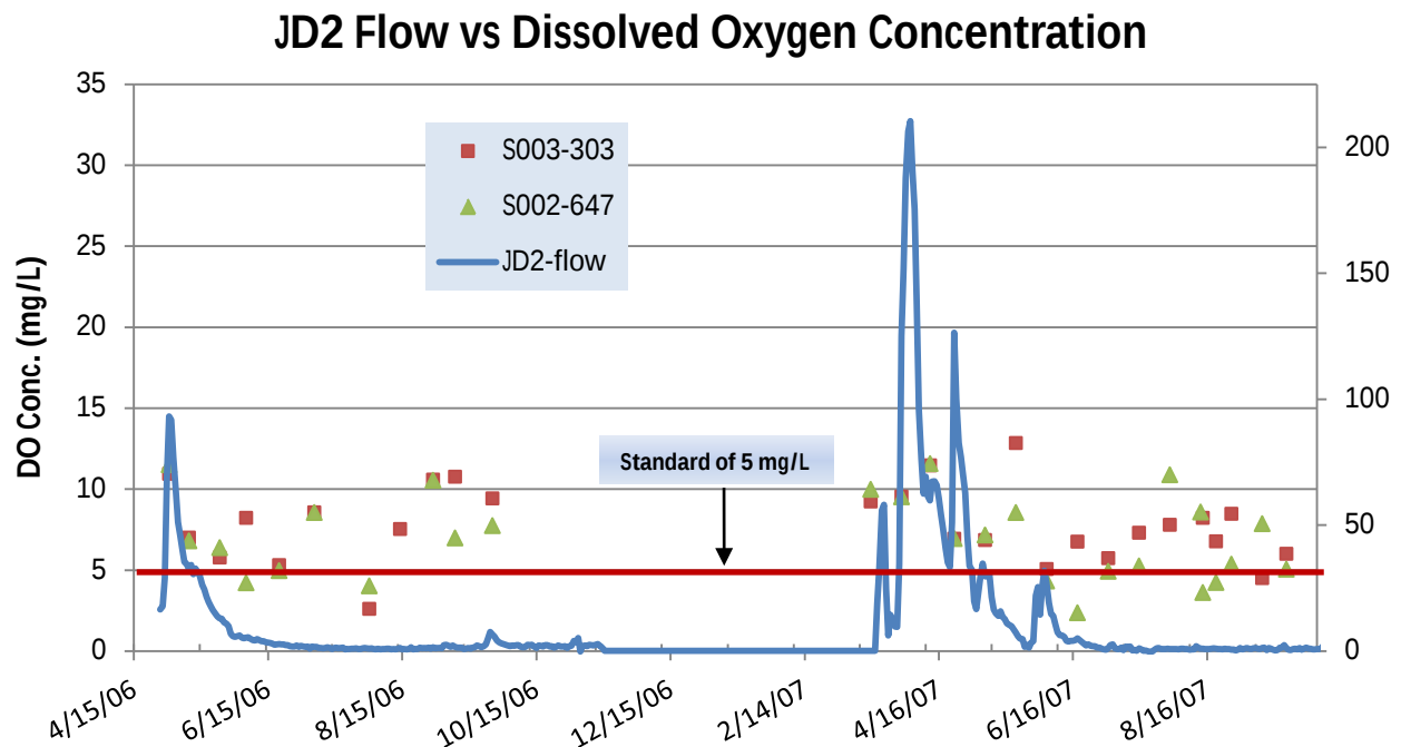
Figure 37: Dissolved Oxygen data versus discharge data for JD2 from 2006-2007.
