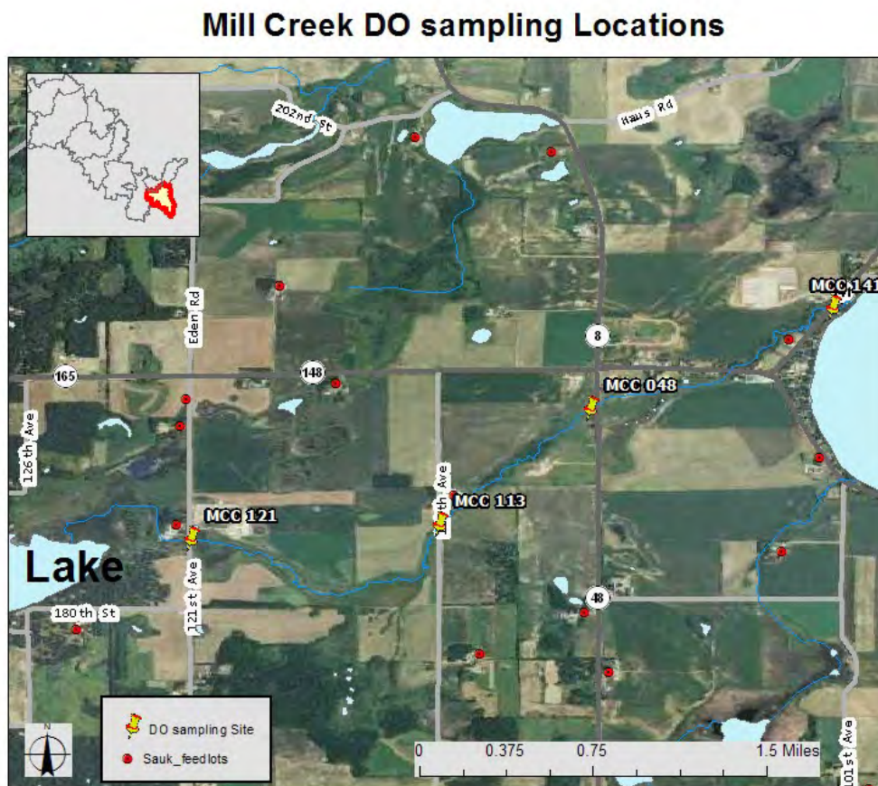
Figure 107: 2010 early morning DO sampling sites for Mill Creek above Pearl Lake
