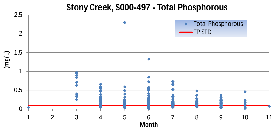
Figure 67: TP values composited by month from Stoney Creek EQuIS sites (1980;1995-2009).
