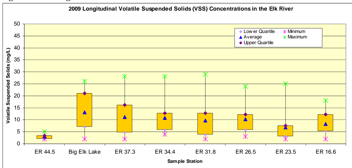
Figure 3.15: Longitudinal VSS concentrations in the Elk River
