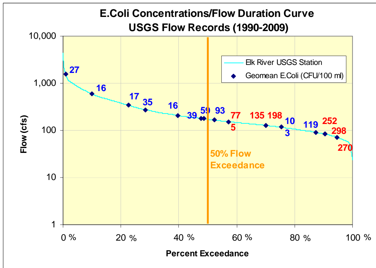
Figure 3.24: Flow duration curve with bacteria concentrations
