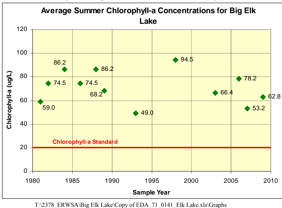
Figure 3.9: Summer average chlorophyll-a concentrations for Big Elk Lake
