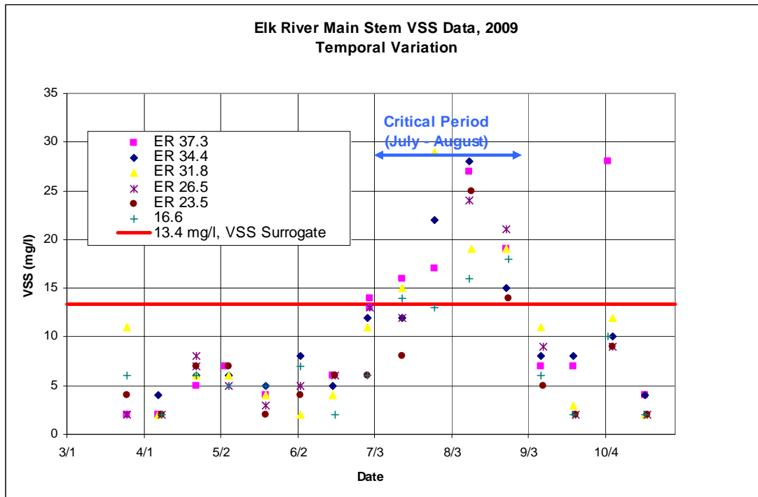
Figure 3.29: Temporal variation in 2009 VSS data
