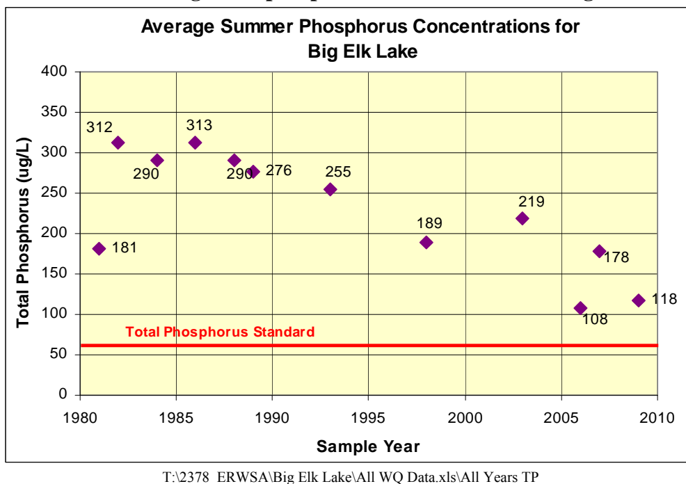
Figure 3.8: Summer average total phosphorus concentrations for Big Elk Lake
