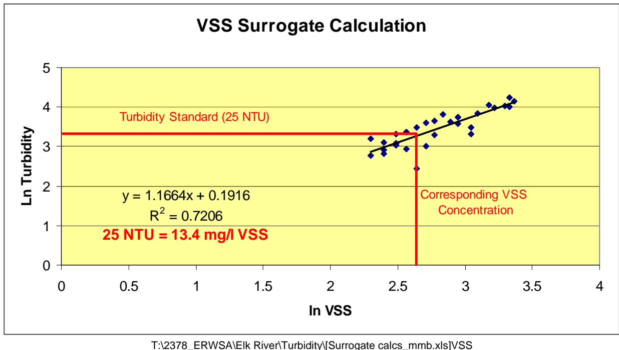
Figure 3.31: VSS surrogate calculation
