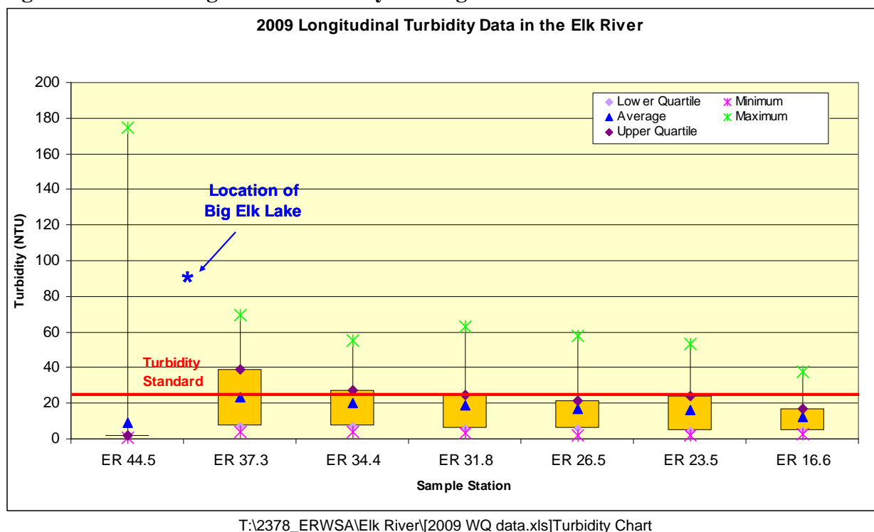
Figure 3.14: 2009 longitudinal turbidity readings in the Elk River
