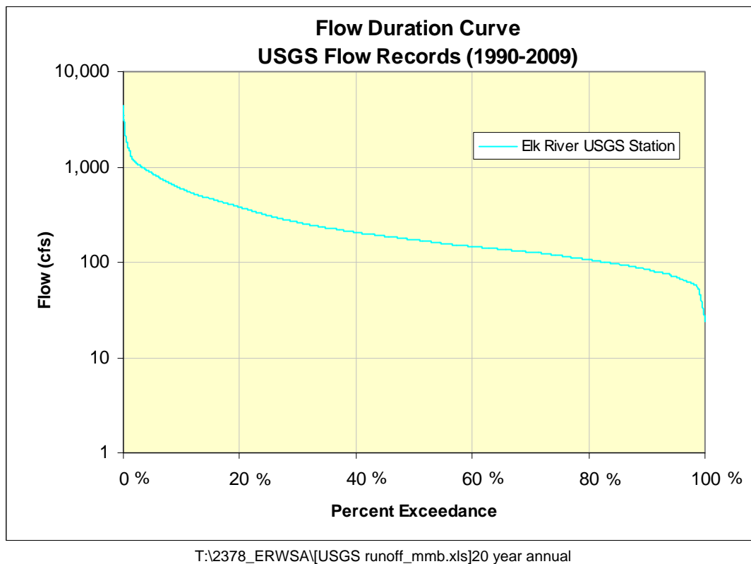
Figure 3.25: Flow duration curve
