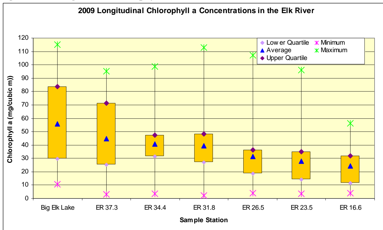
Figure 3.16: Longitudinal chlorophyll-a concentrations in the Elk River
