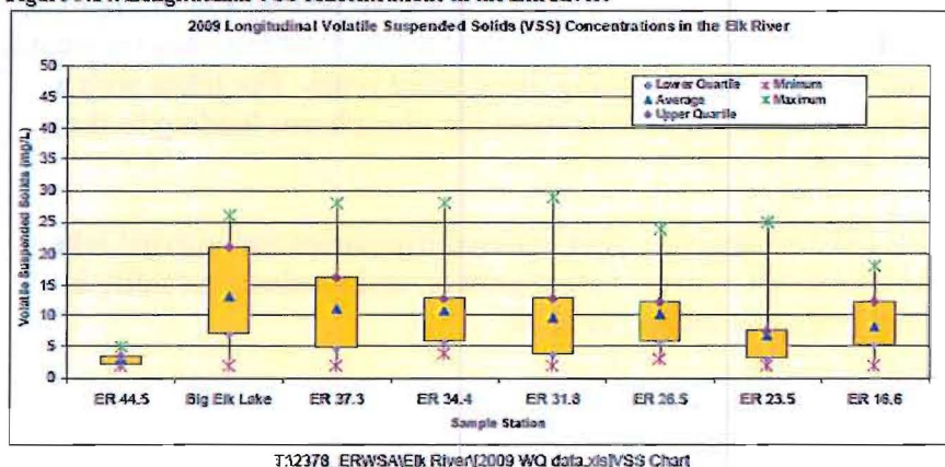
Figure 3.14. Longitudinal VSS concentrations in the Elk River.
