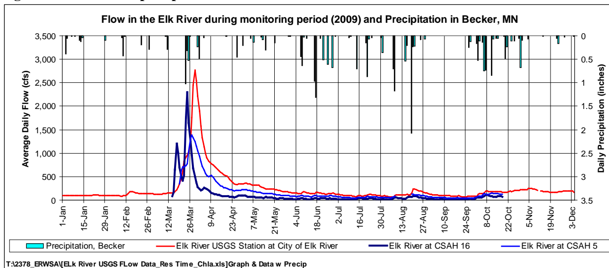
Figure 3.27. Flow and precipitation in the watershed in 2009.
