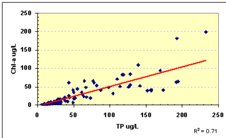
Figure 2.1. Relationships among phosphorus, chlorophyll-a and Secchi Depth in Minnesota lakes (Source: MPCA web site http://www.pca.state.mn.us/index.php/water/water-types-and-programs/surface-water/lakes/lake-water-quality/assessment-definitions-andnotes.html?menuid=&missing=0&redirect=1 )
