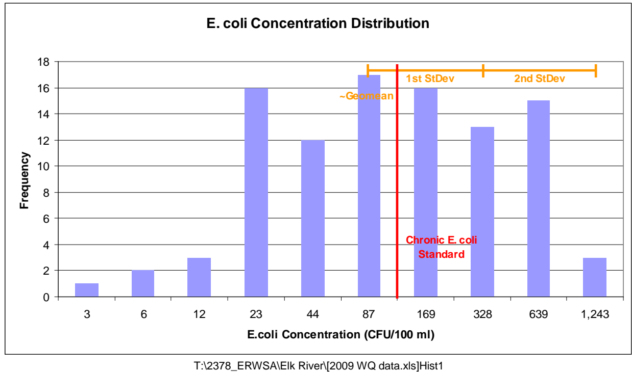
Figure 6.3. Distribution of 2009 E. coli concentrations.
