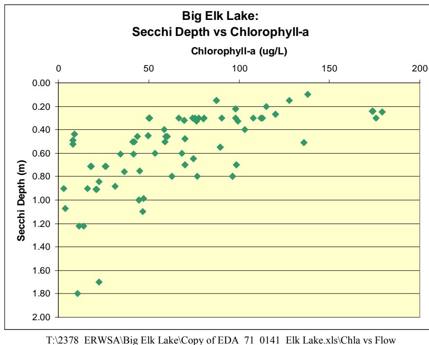
Figure 3.11. Discrete chlorophyll-a concentrations versus discrete Secchi depth readings for Big Elk Lake.
