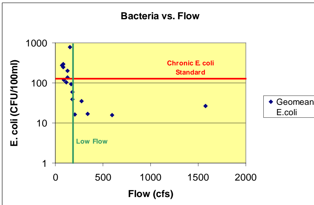
Figure 3.23: Bacteria concentrations vs. flow for Elk River impaired reach.
