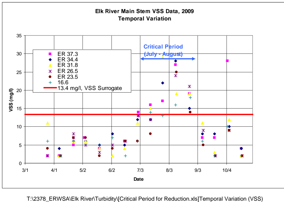
Figure 5.6. Temporal variation in 2009 VSS data.
