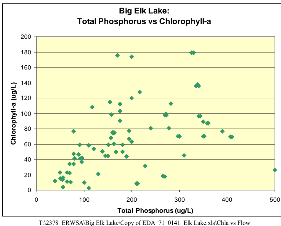
Figure 3.10. Discrete chlorophyll- a concentrations versus discrete total phosphorus concentrations for Big Elk Lake.
