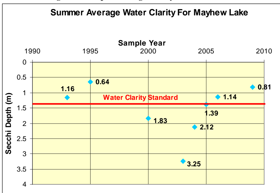
Figure 3.4. Summer average Secchi depth readings in Mayhew Lake.
