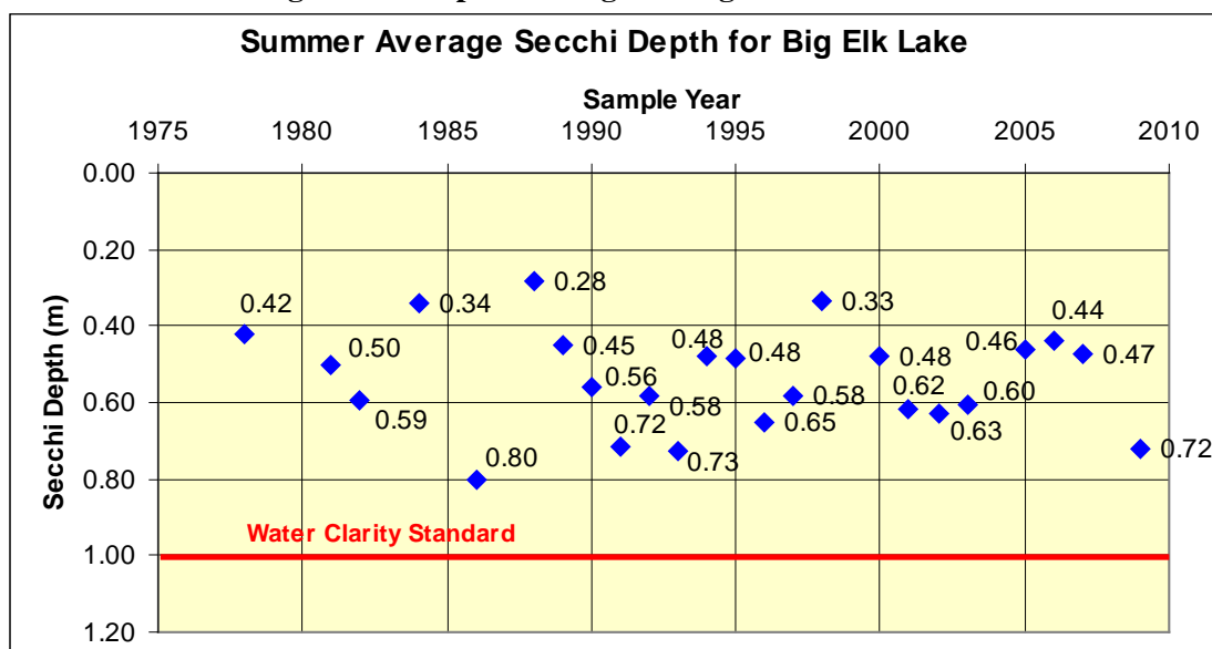
Figure 3.7. Summer average Secchi depth readings for Big Elk Lake.
