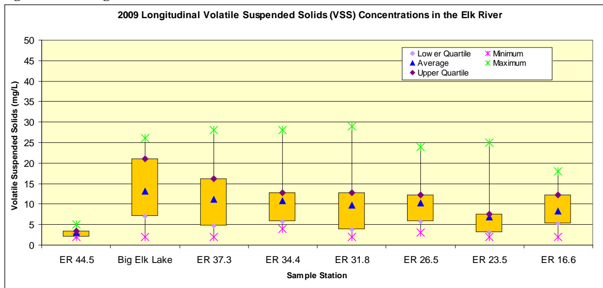
Figure 3.14. Longitudinal VSS concentrations in the Elk River.
