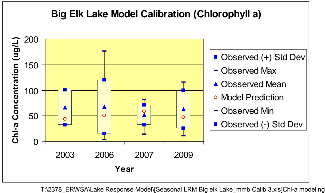
Figure 5.4. Mayhew Lake model calibration (chlorophyll-a).
