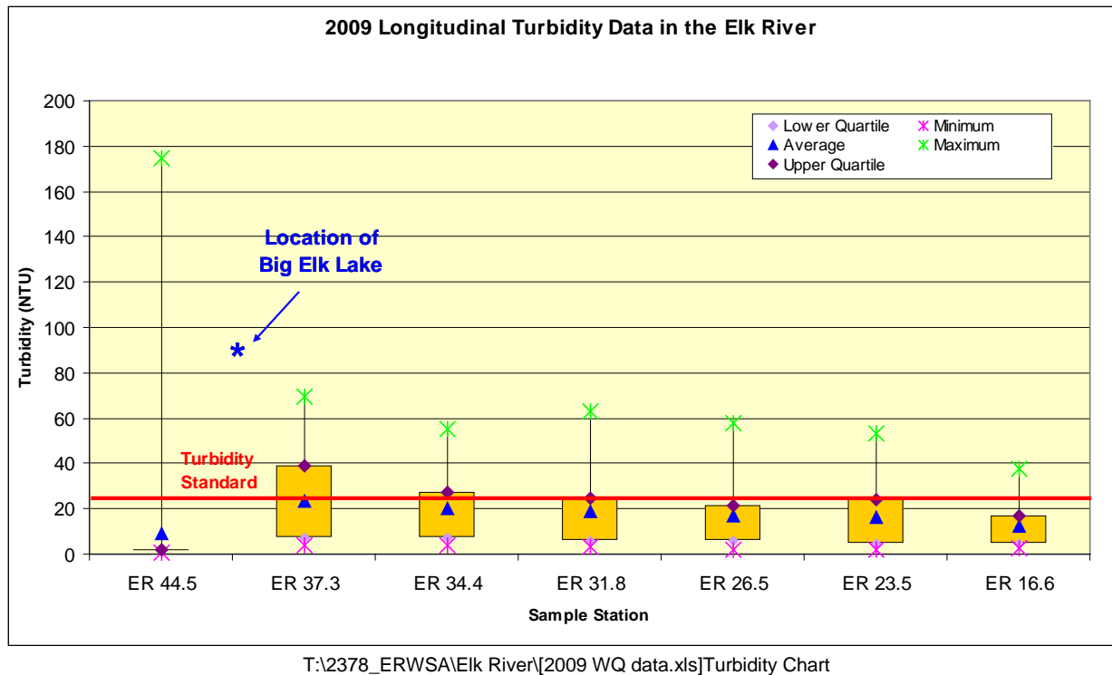
Figure 3.13. 2009 longitudinal turbidity readings in the Elk River.
