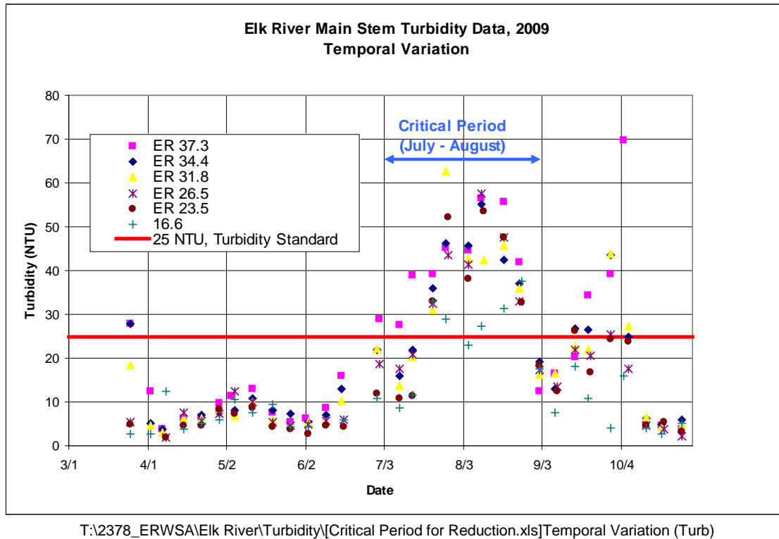
Figure 5.5. Temporal variation in 2009 turbidity data.
