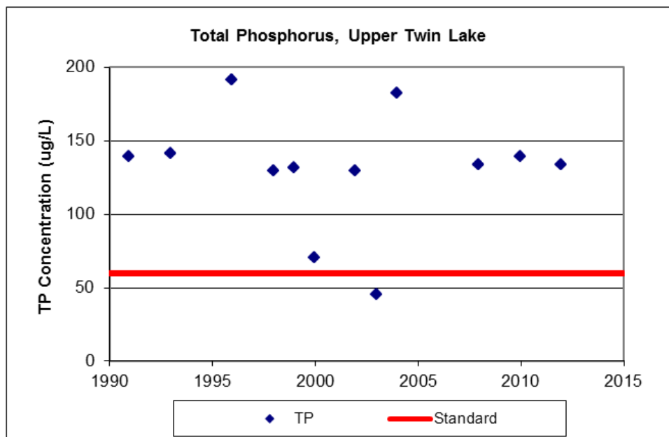
Figure 3.1. Upper Twin Lake summer average total phosphorus data.
