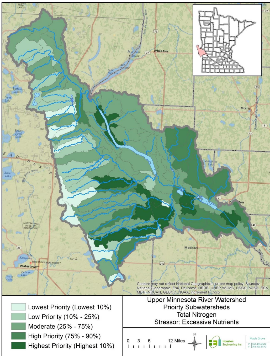
Figure 13: Watershed scale subwatershed priority for implementation for the stressor excessive nutrients, using average (1995-2012) total nitrogen yields.
