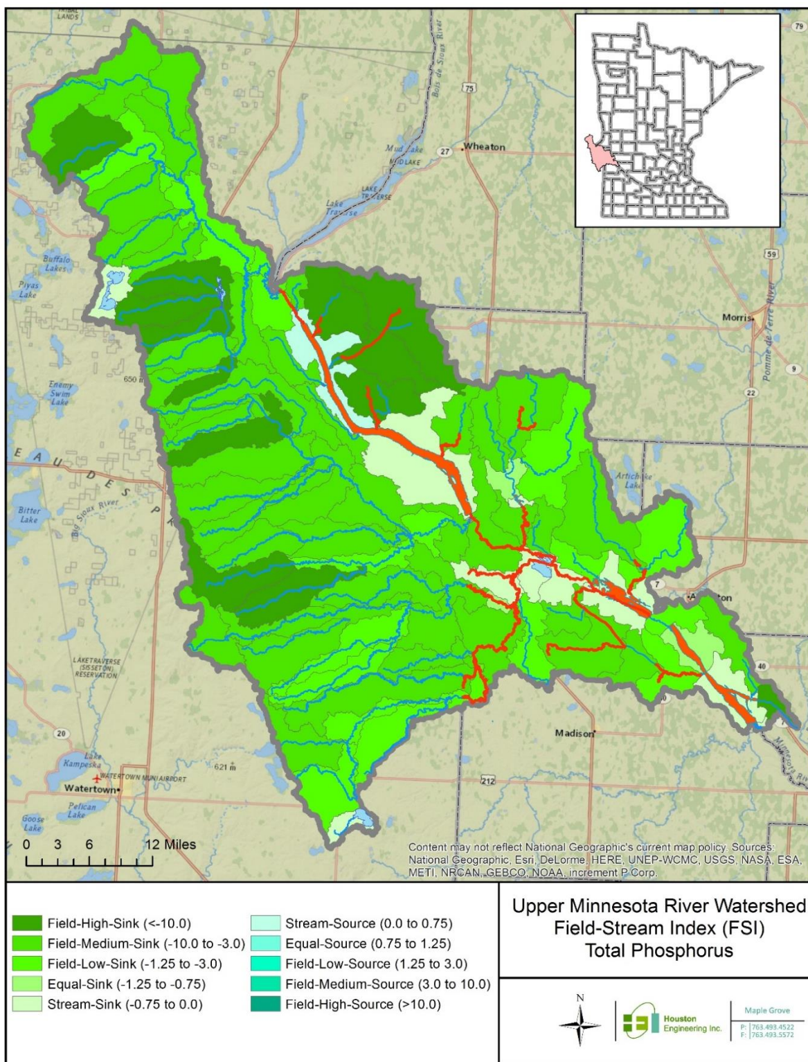
Figure 10: Watershed scale subwatershed priority for implementation of field and stream practices (Field Stream Index) for the stressor excess nutrients using total phosphorus (1996-2009) annual average load.
