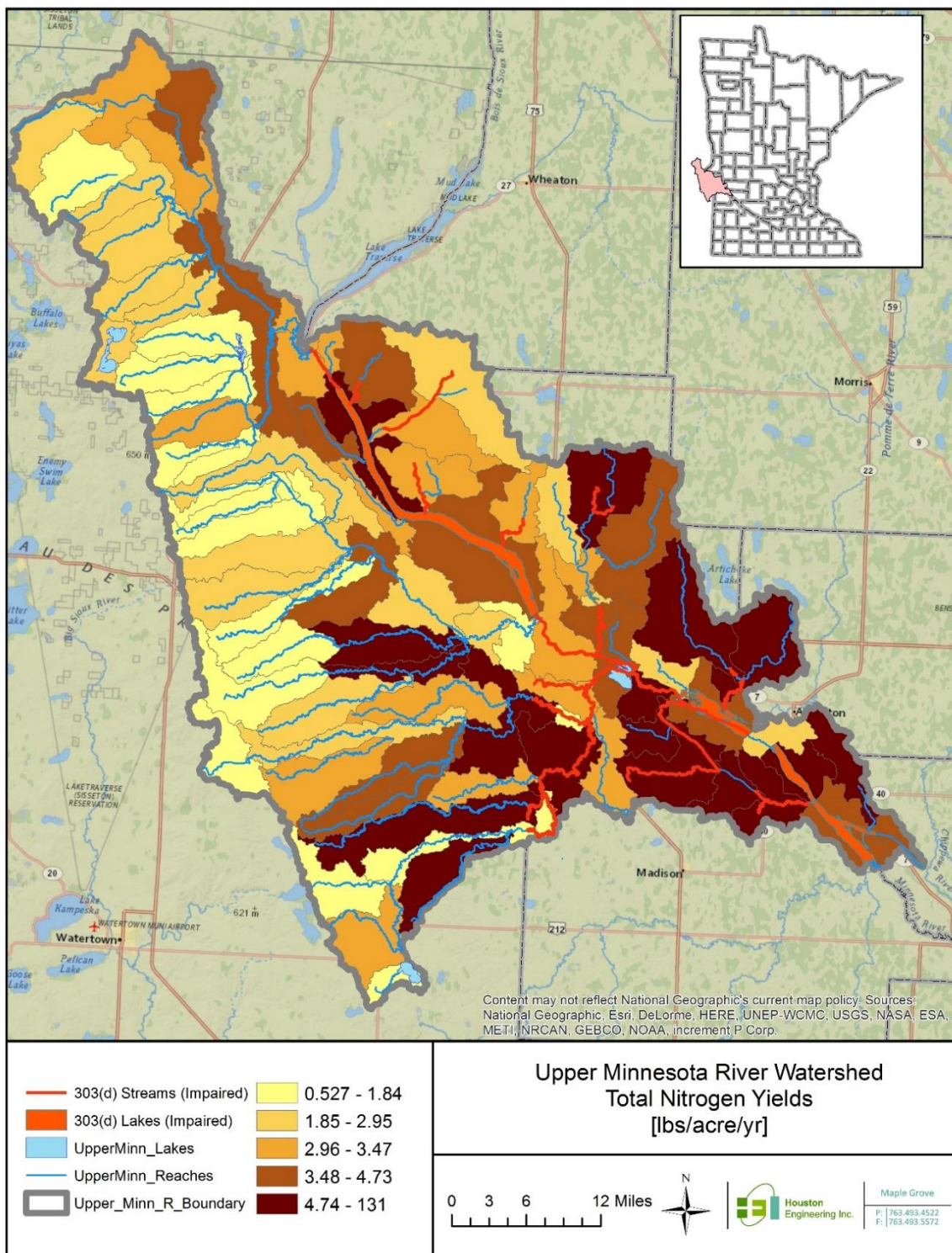
Figure 12. Average (1995-2012) total nitrogen yield (lbs/acre/yr) delivered to the channel from the HSPF model by subwatershed.
