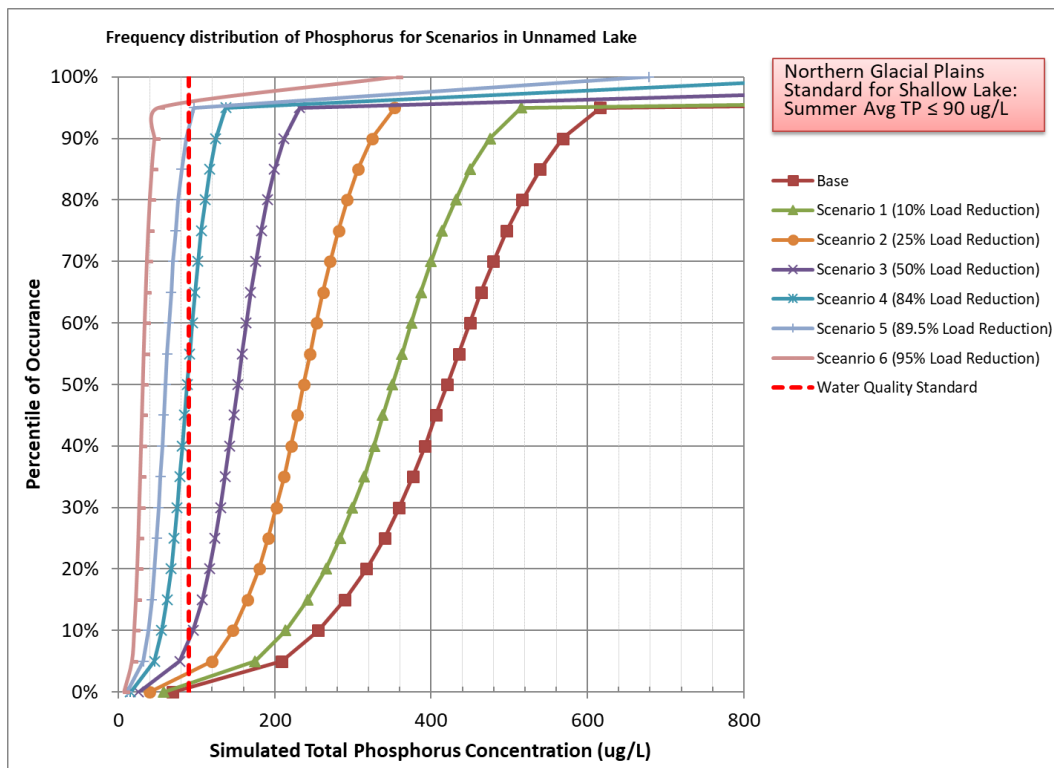
Figure 10. Frequency distribution of phosphorus concentrations in Unnamed Lake by load reduction scenario.
