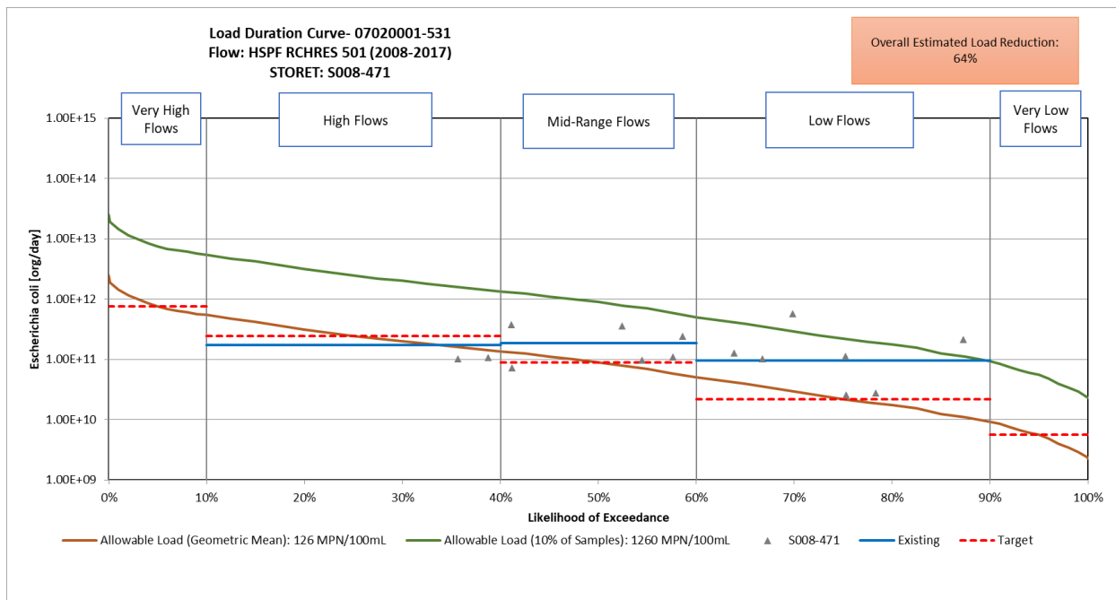
Figure 20. Stony Run Creek, Unnamed cr to Minnesota R (07020001-531) E. coli LDC.
