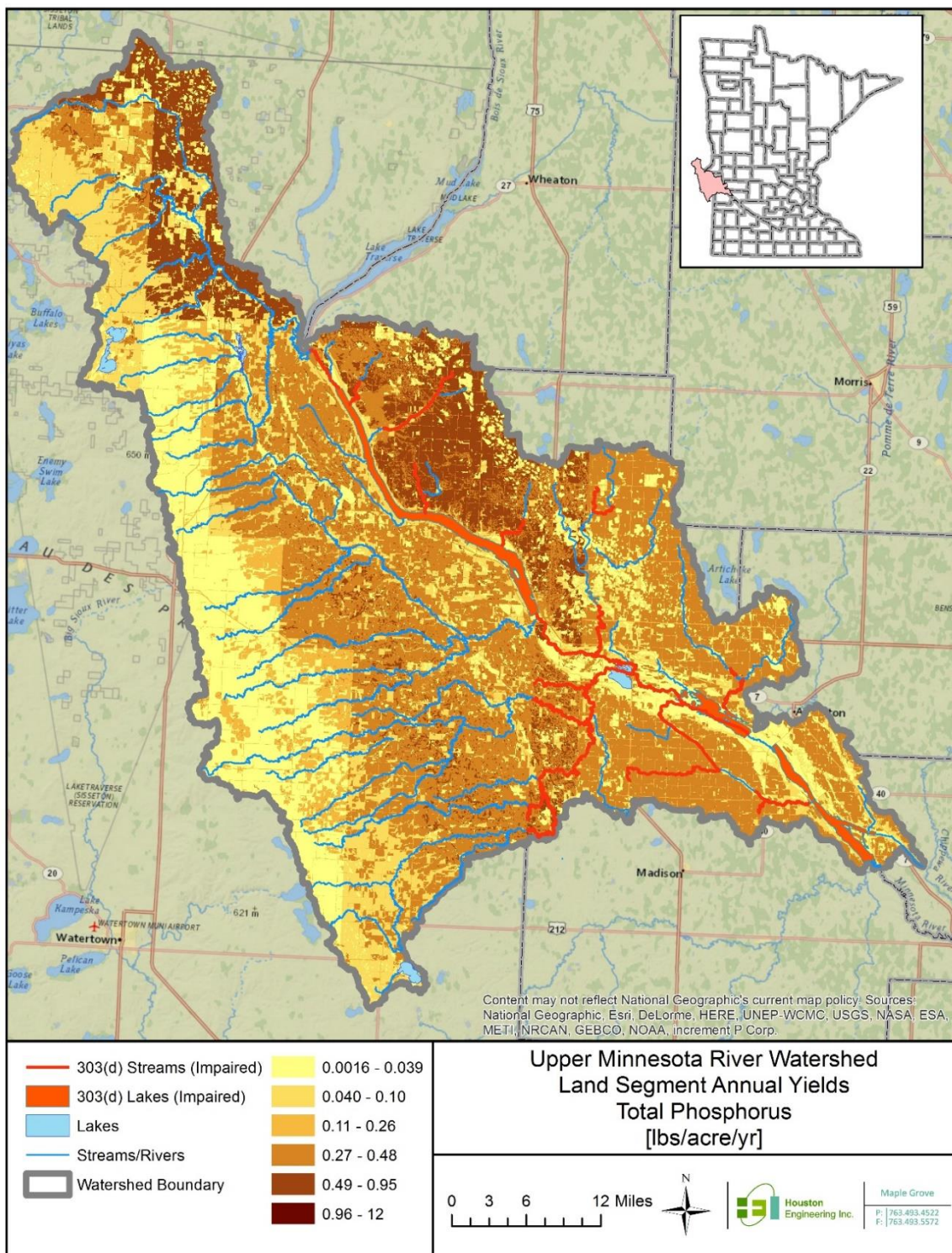
Figure 7. Average (1995-2012) total phosphorus yield (lbs/acre/yr) delivered to the channel from the HSPF model by land segment.
