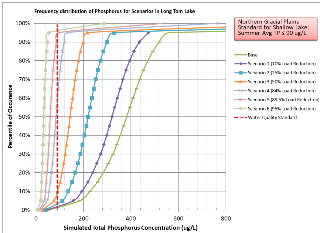
Figure 16. Frequency distribution of phosphorus concentrations in Long Tom Lake by load reduction scenario.
