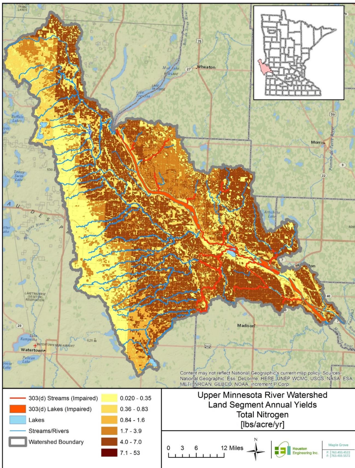
Figure 11. Average (1995-2012) total nitrogen yield (lbs/acre/yr) delivered to the channel from HSPF model by HRU.
