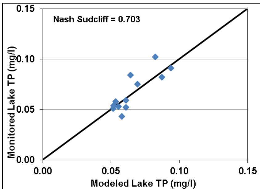
Figure A.3 Lotus Lake comparison between modeled volumetric average TP concentration and measured concentrations for the 2015 water year.
