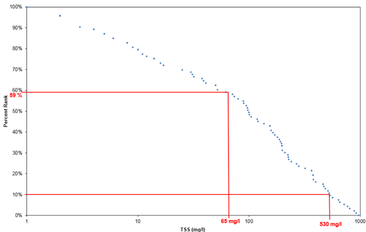
Figure 3.15 Riley Creek TSS concentration cumulative frequency curve, 2006-2015
