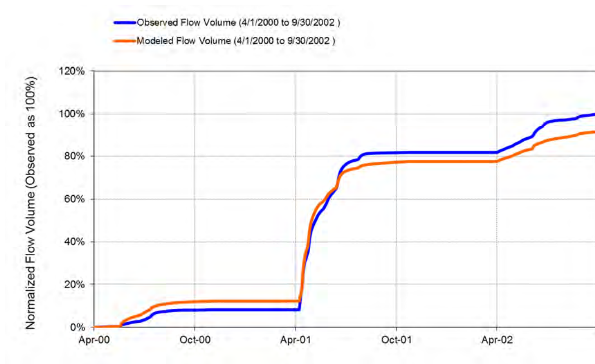
Figure 25. Flow accumulation at MN 31040001 Watonwan River near La Salle, CSAH16
