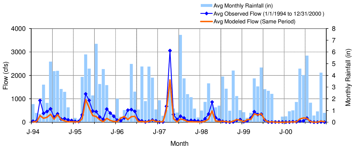
Figure 45. Mean monthly flow: Model DSN 100 vs. USGS 05313500 Yellow Medicine River near Granite Falls, MN, 1994-2000
