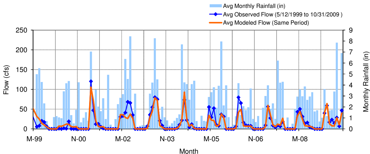
Figure 9. Mean monthly flow: Model DSN 700 vs. Hawk Creek - Priam (S002-140)
