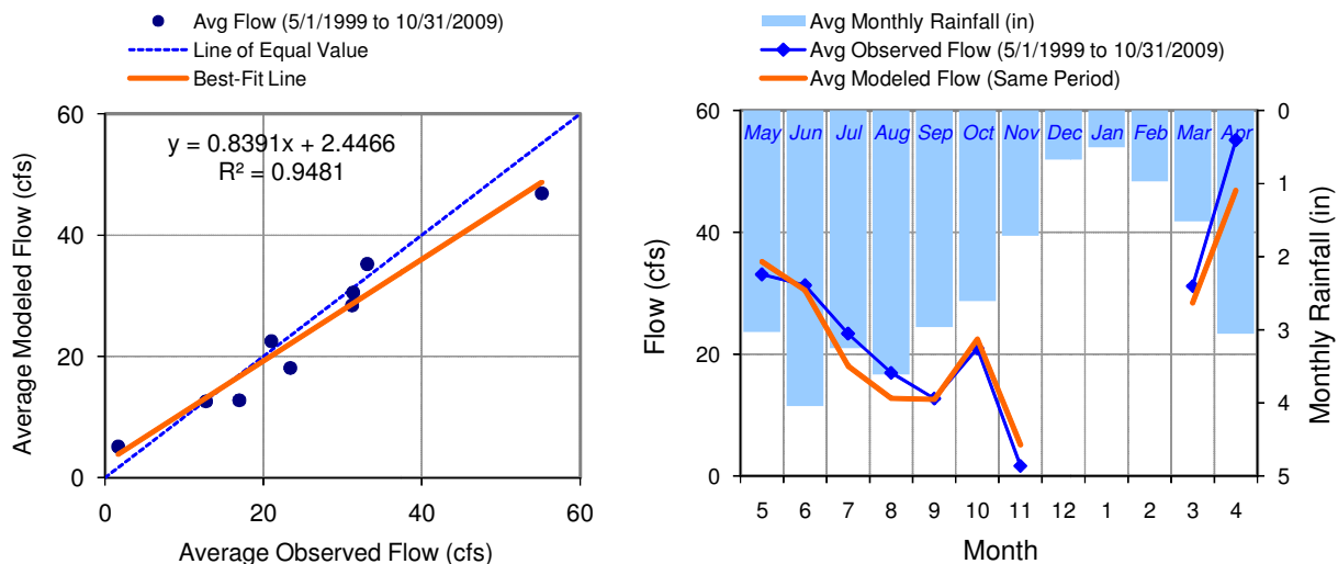
Figure 11. Seasonal regression and temporal aggregate: Model DSN 700 vs. Hawk Creek - Priam (S002-140)
