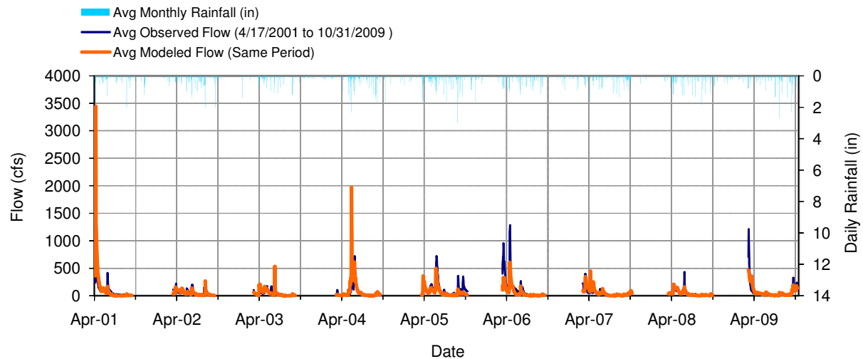
Figure 38. Mean daily flow: Model DSN 400 vs. Beaver Falls (S000-666)
