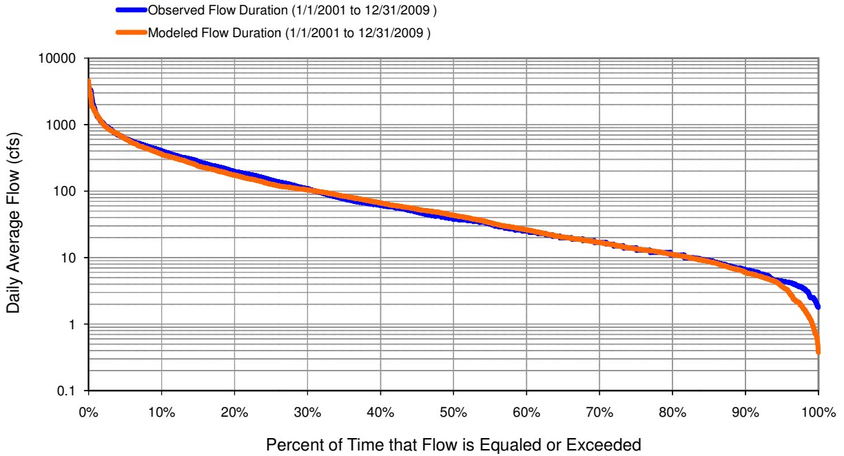
Figure 6. Flow exceedence: Model DSN 100 vs. USGS 05313500 Yellow Medicine River near Granite Falls, MN
