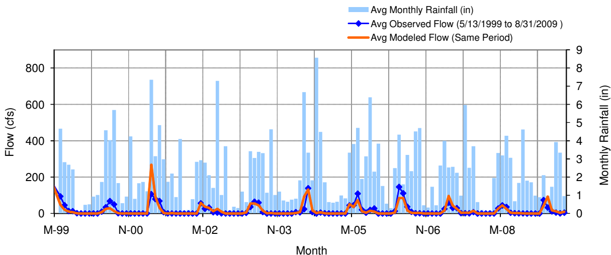
Figure 33. Mean monthly flow: Model DSN 300 vs. West Fork Beaver Creek (S000-405)
