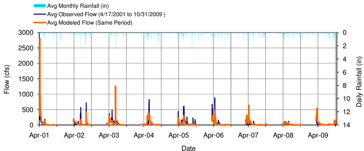
Figure 20. Mean daily flow: Model DSN 900 vs. Chetomba Creek (S002-152)
