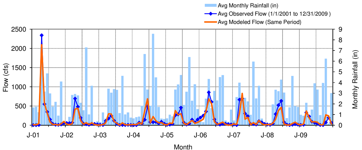
Figure 2. Mean monthly flow: Model DSN 100 vs. USGS 05313500 Yellow Medicine River near Granite Falls, MN
