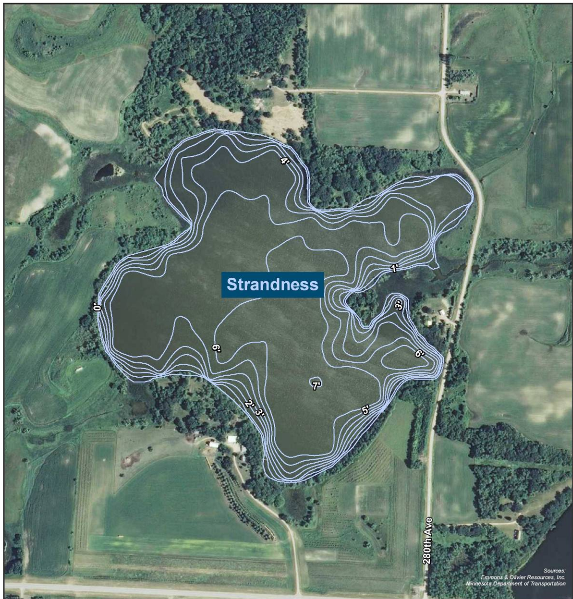
Figure 85. Strandness Lake Bathymetry
