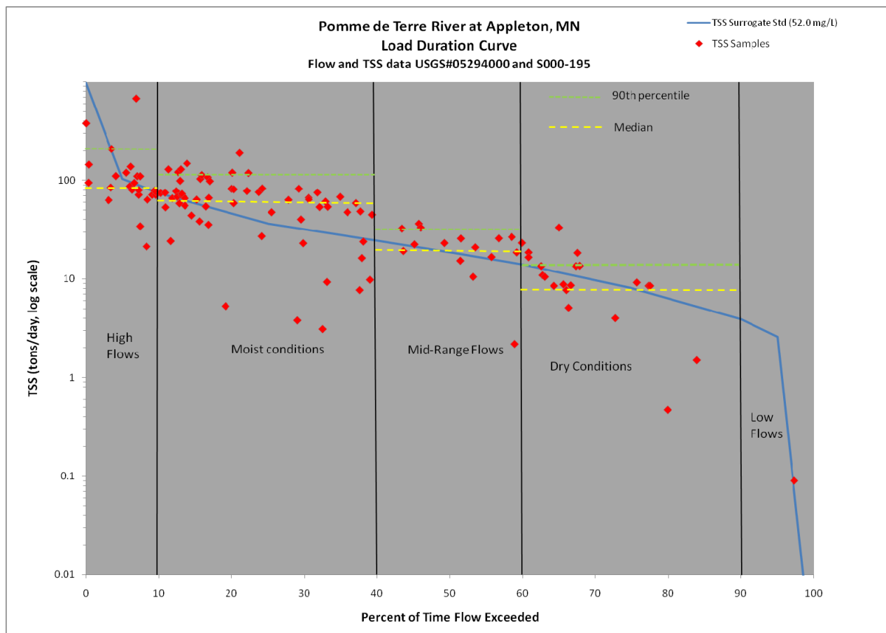
Figure 6.1: Loading Duration Curve for PdT River
