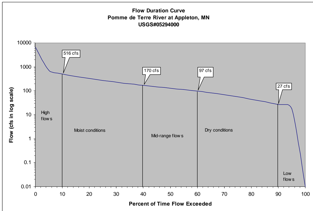
Figure 5.1: Flow Duration Curve for the PdT at Appleton, MN
