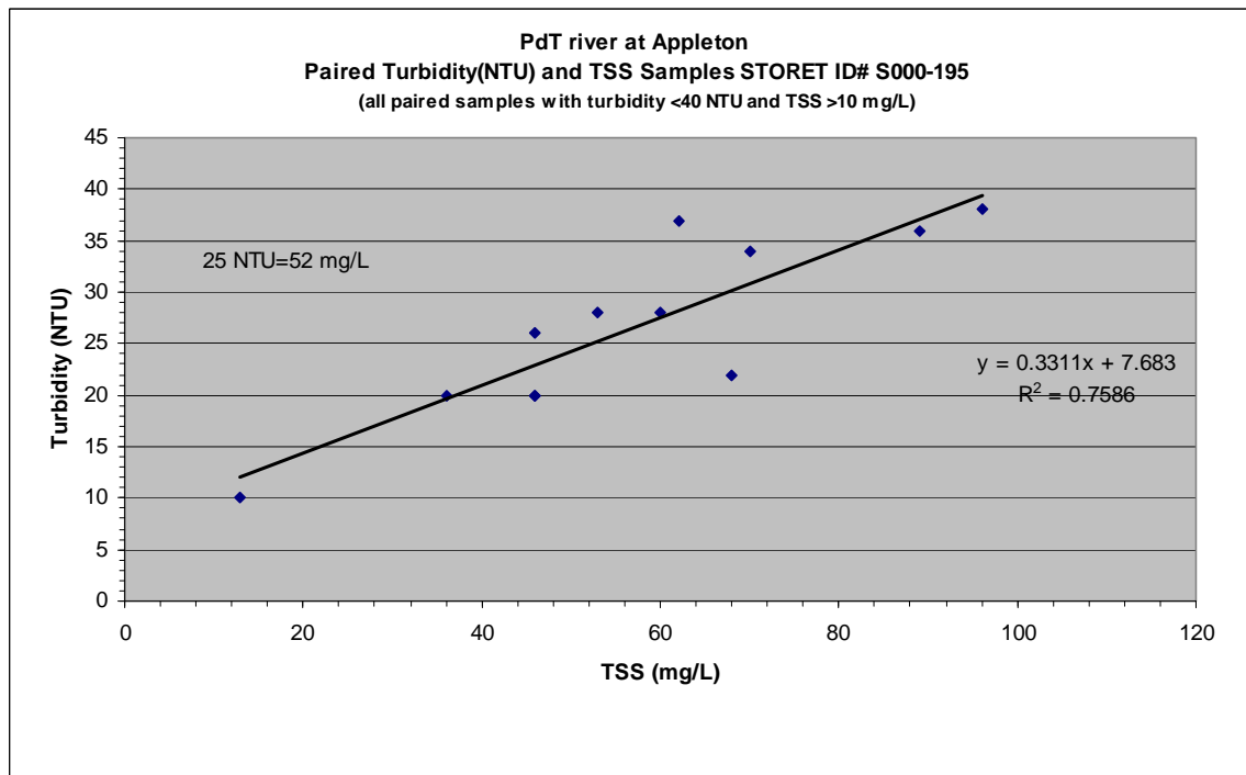
Figure 5.3: Paired Turbidity (NTU)/TSS samples
