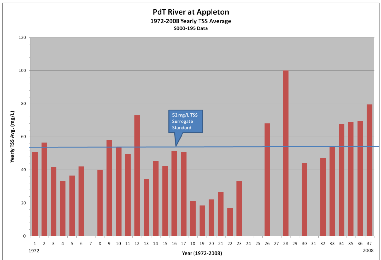
Figure 4.1: 1972-2008 Yearly Average TSS concentrations (the corresponding TSS surrogate value for the 25 NTU standard is shown.)
