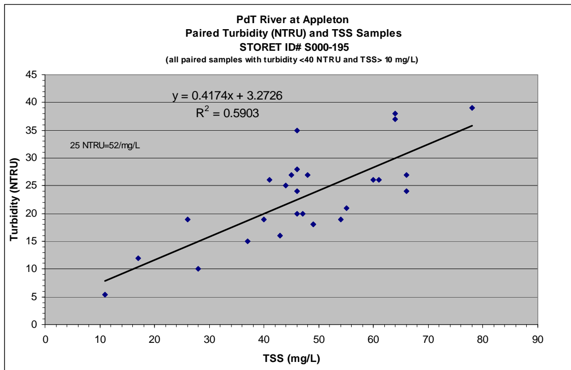
Figure 5.2: Paired Turbidity (NTRU)/TSS samples
