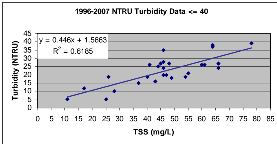
Figure 5: Regression analysis for TSS and NTRU Turbidity units
