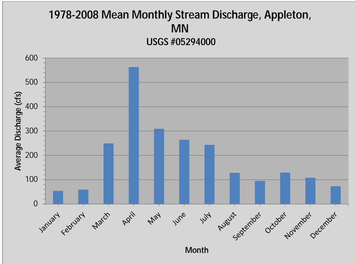
Figure 6.4: Average Monthly flow
