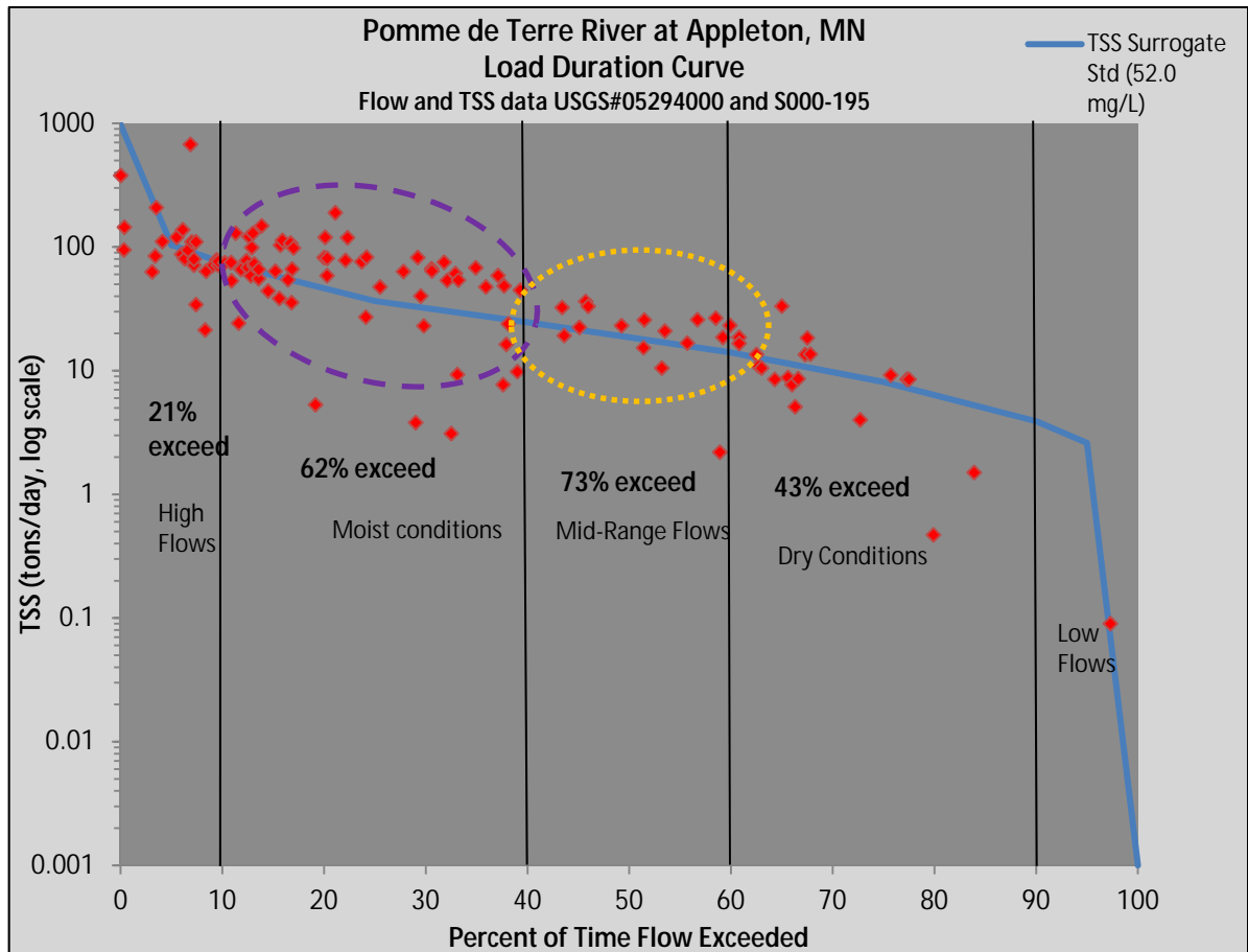
Figure 6.3: Using the Load Duration Curve to Discuss Contributing Erosion Zones
