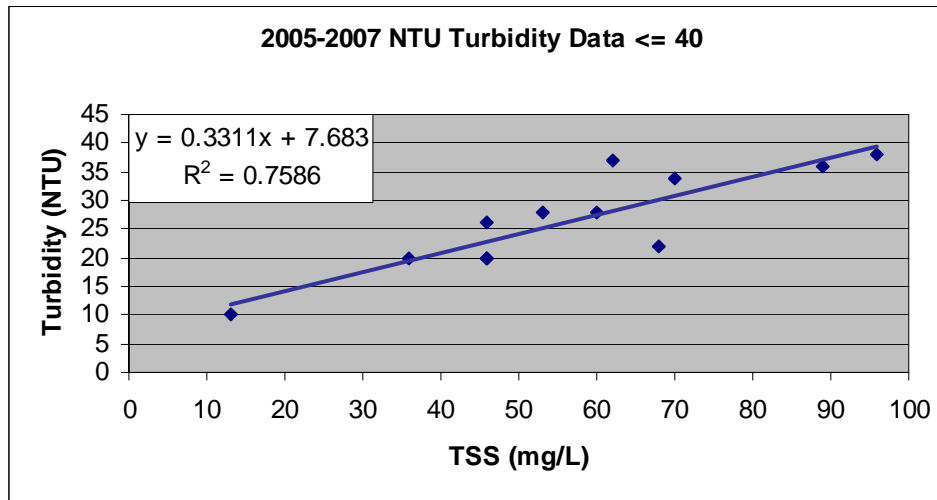
Figure 4: Regression analysis for TSS and NTU Turbidity units
