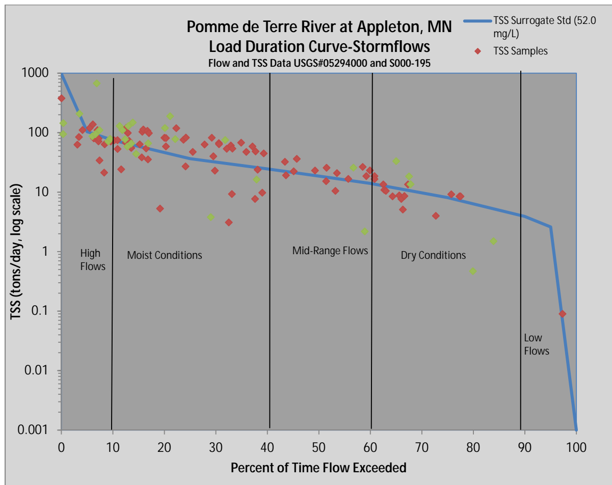
Figure 6.2: Load Duration Curve with Stormflow Samples
