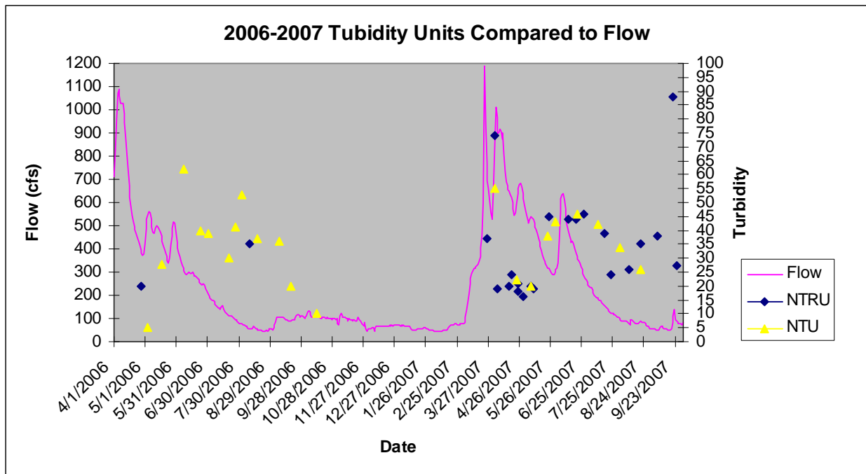
Figure 3: NTU and NTRU Turbidity units compared by date and correlated to flow
