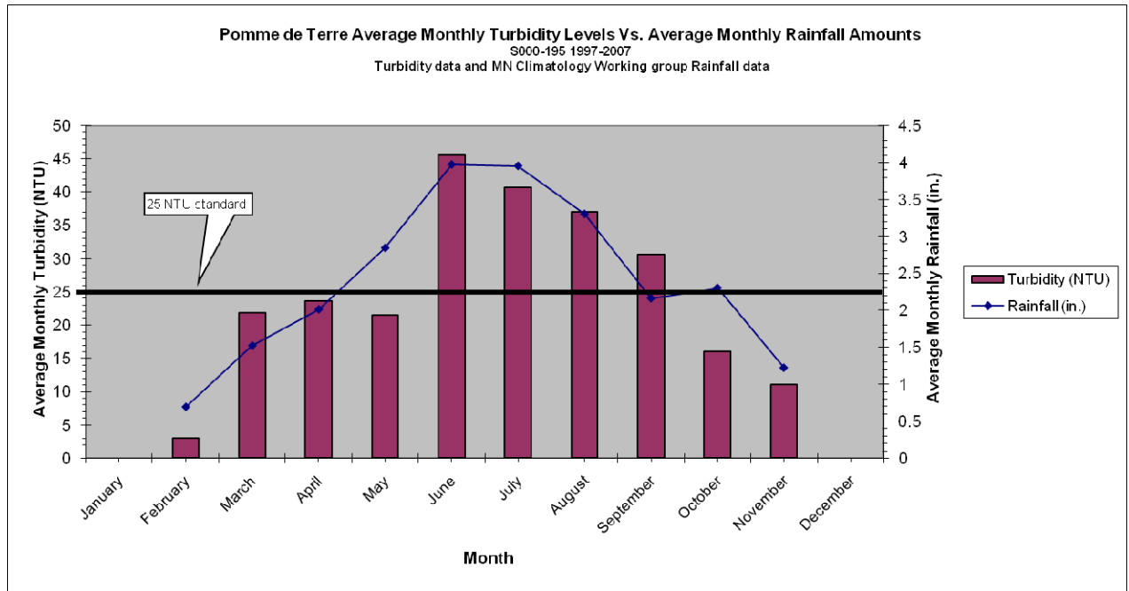
Figure 6.5: Monthly Turbidity and Rainfall Averages
