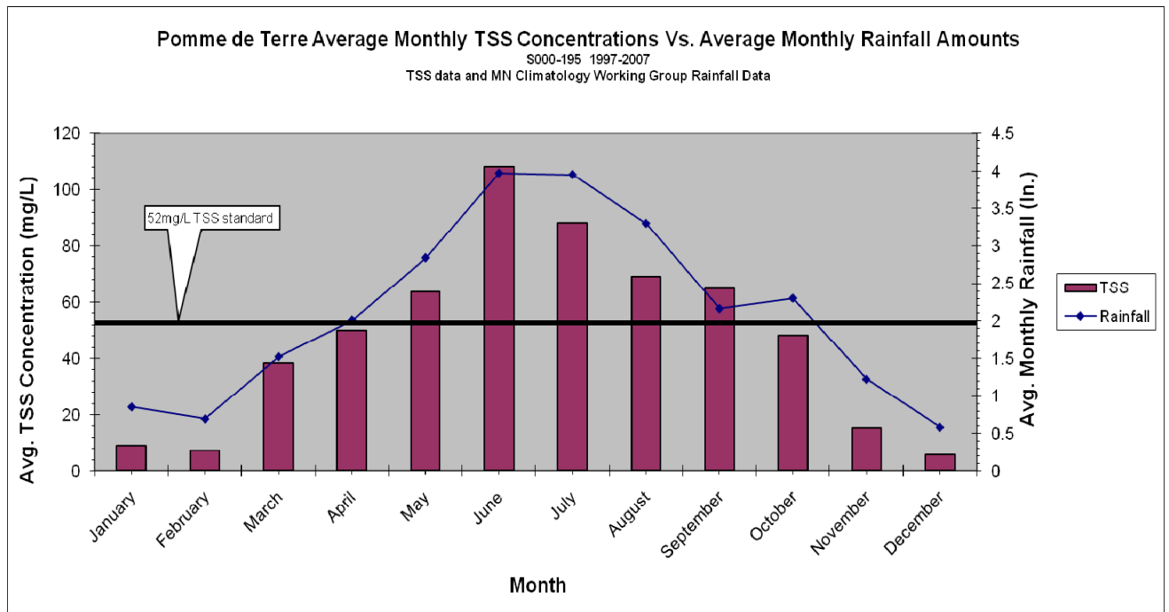
Figure 6.6: Monthly TSS and Rainfall Averages
