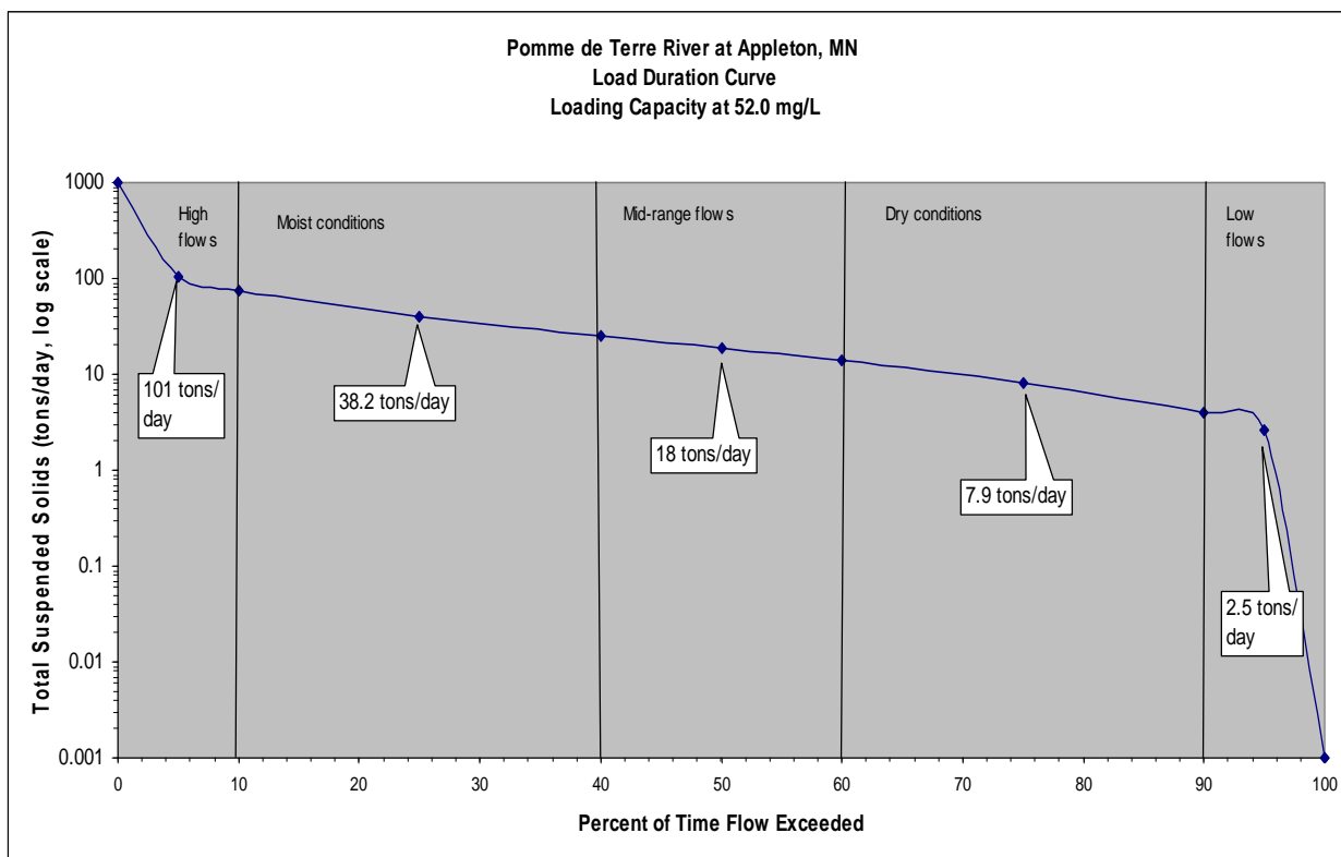
Figure 5.4: TDLC by Flow Regime
