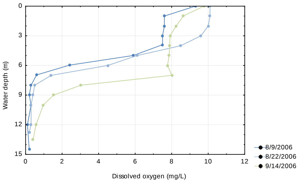
Figure 31: Dissolved oxygen profiles for Goose Lake (South), 2006
