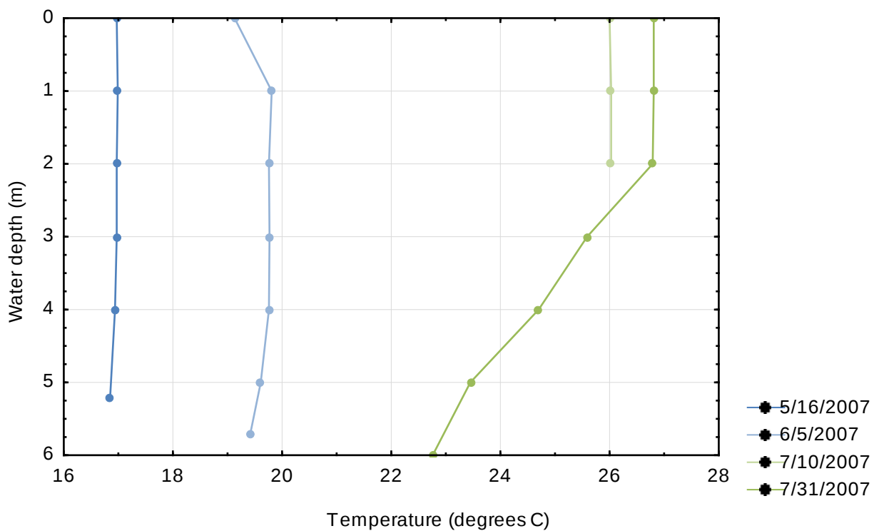
Figure 64: Temperature profiles for Rush Lake (East), 2007
