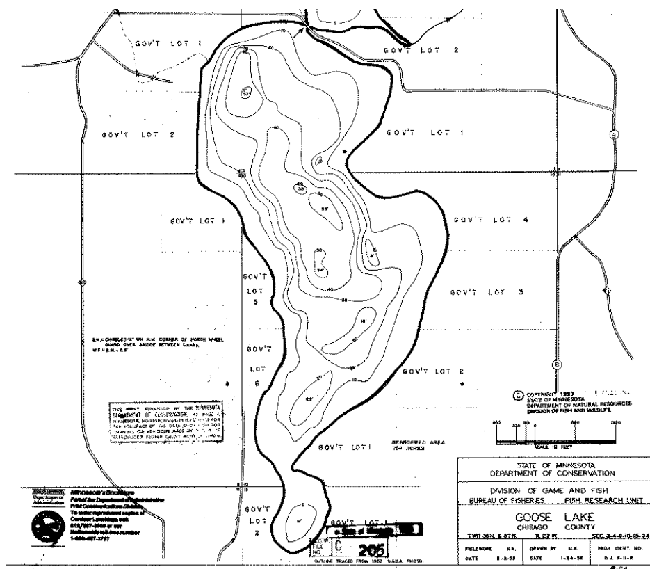
Figure 24. Goose Lake (South Bay) Bathymetry (DNR)
