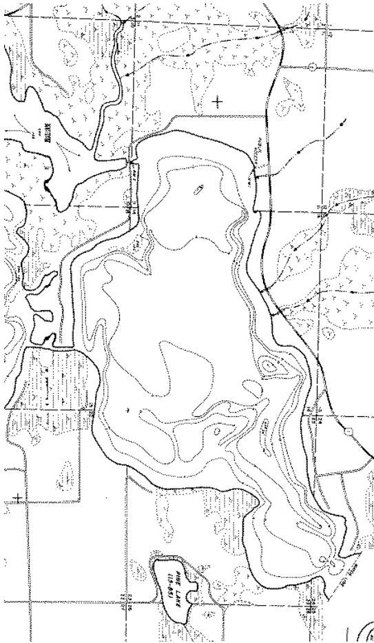
Figure 58. Rush Lake (East) bathymetry (DNR)
