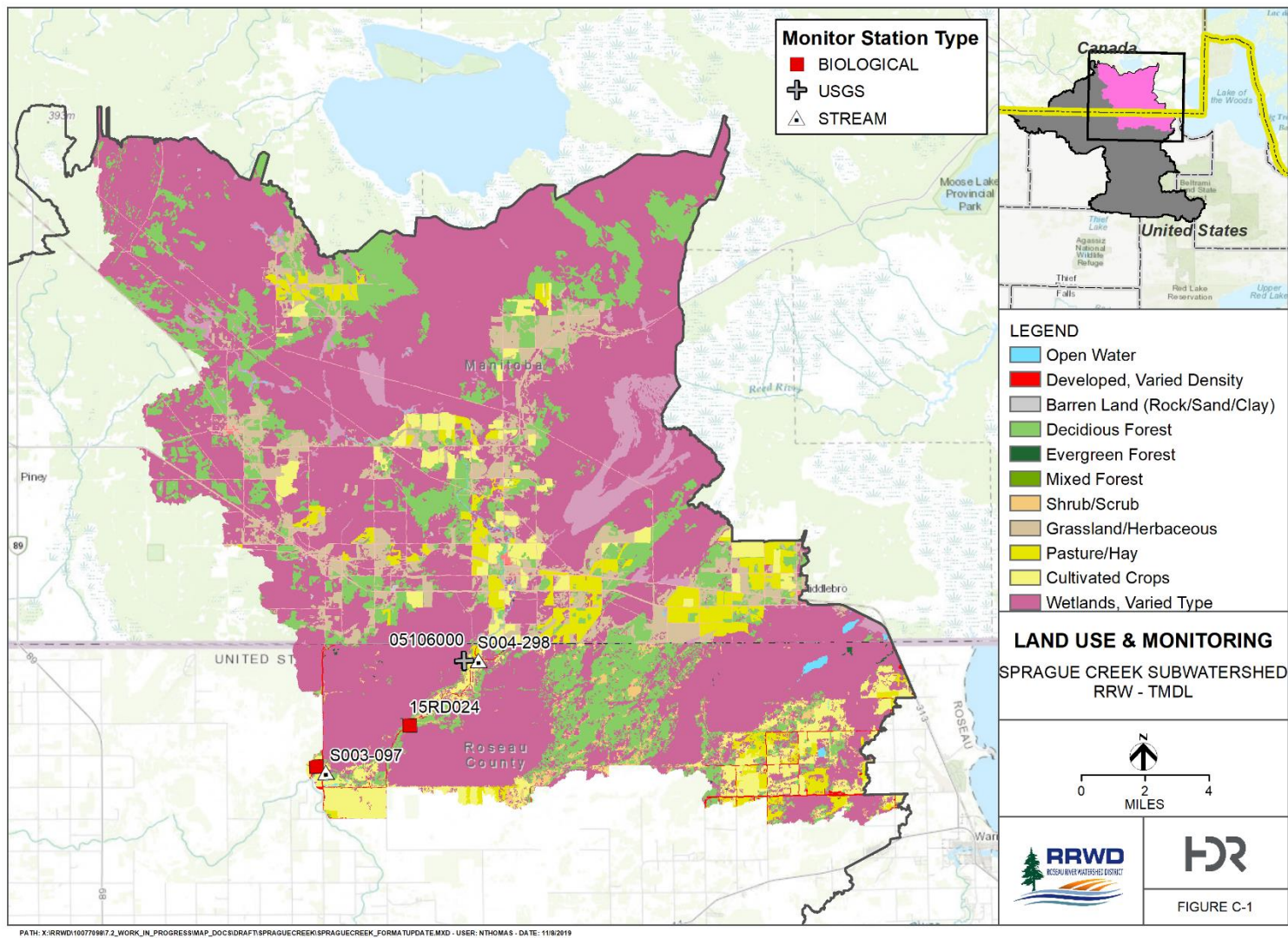
Figure C-1: Sprague Creek land use and monitoring locations
