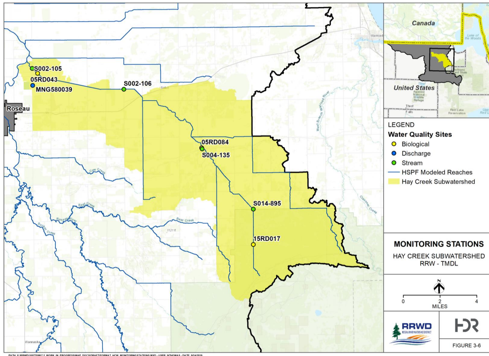
Figure 3-6: Water quality monitoring stations in Hay Creek Subwatershed
