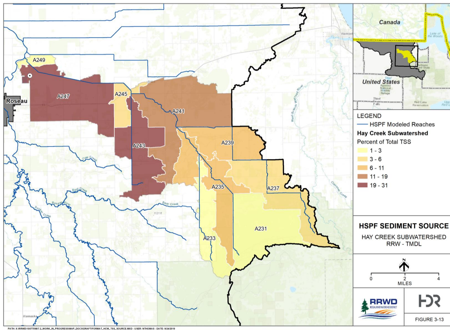
Figure 3-13: Hay Creek Subwatershed sediment source loading summary map. The figure is colored by the percent of total load each sub-basin contributes to the end of the impaired reach (Hay Creek). Darker color denotes higher contribution. HSPF modeling results over the analysis period (2005 to 2014)
