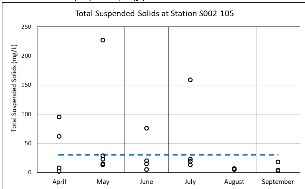
Figure 3-8: TSS sampling aggregated by month on Hay Creek at the monitoring station S002-105. The dashed line denotes the stream water quality standard (30 mg/L).
