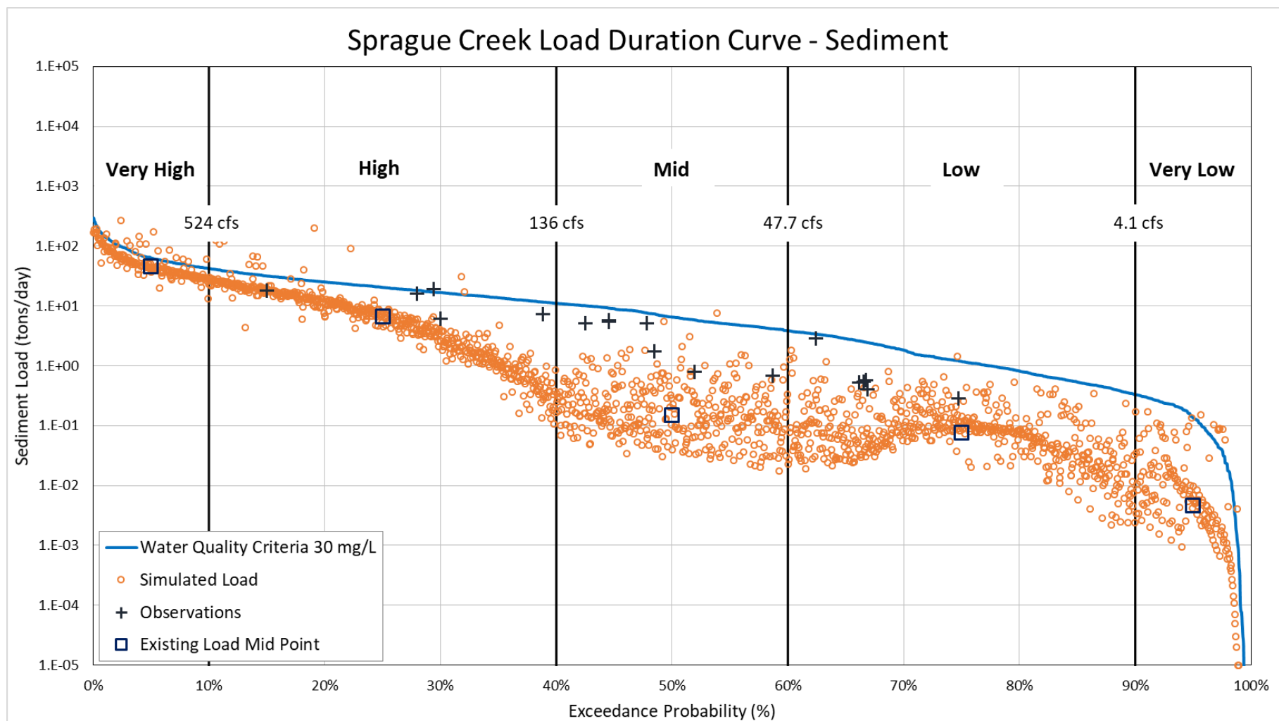
Figure C-2: Sprague Creek (AUID - 508) TSS load duration curve
