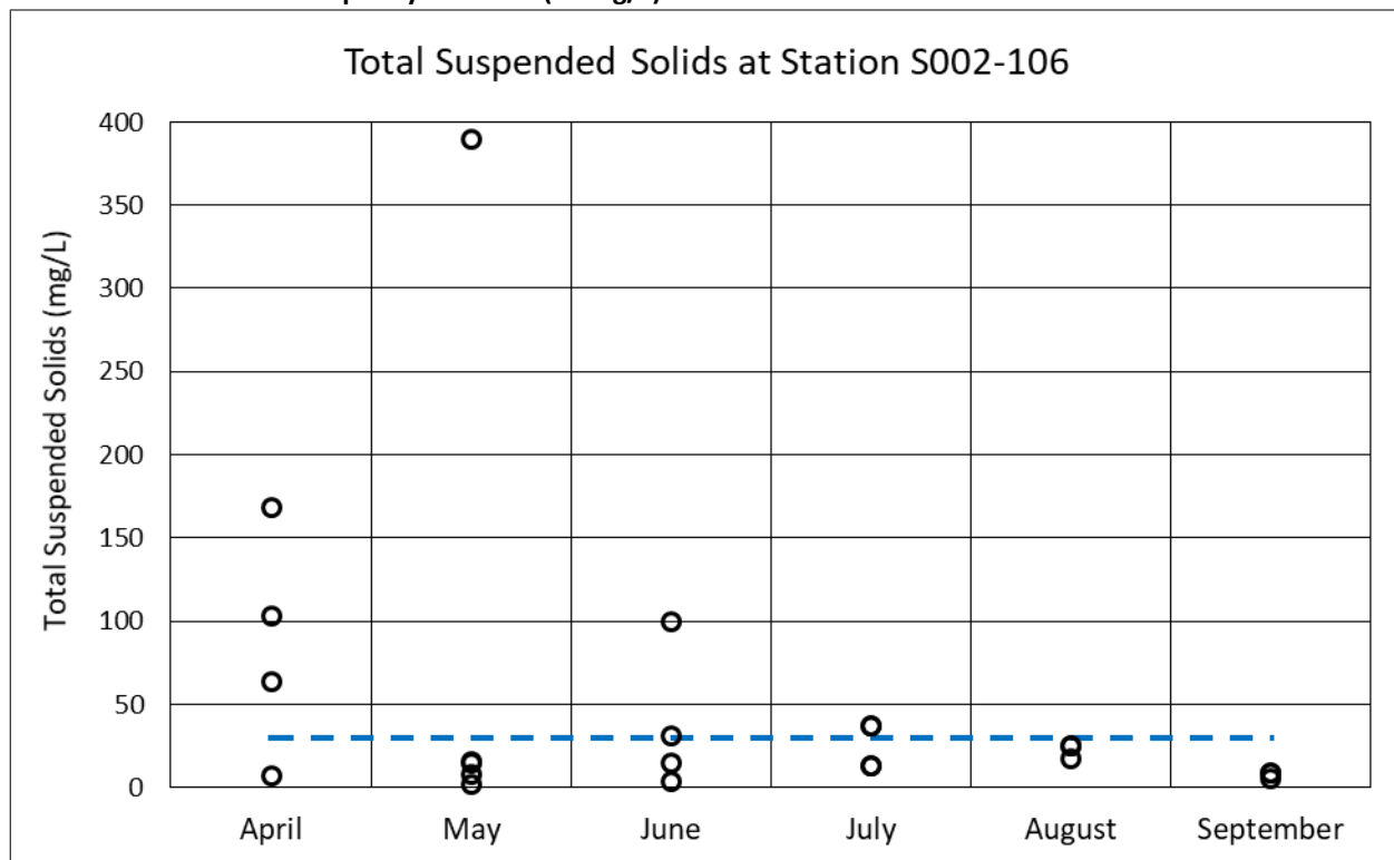
Figure 3-9: TSS sampling aggregated by month on Hay Creek at the monitoring station S002-106. The dashed line denotes the stream water quality standard (30 mg/L).
