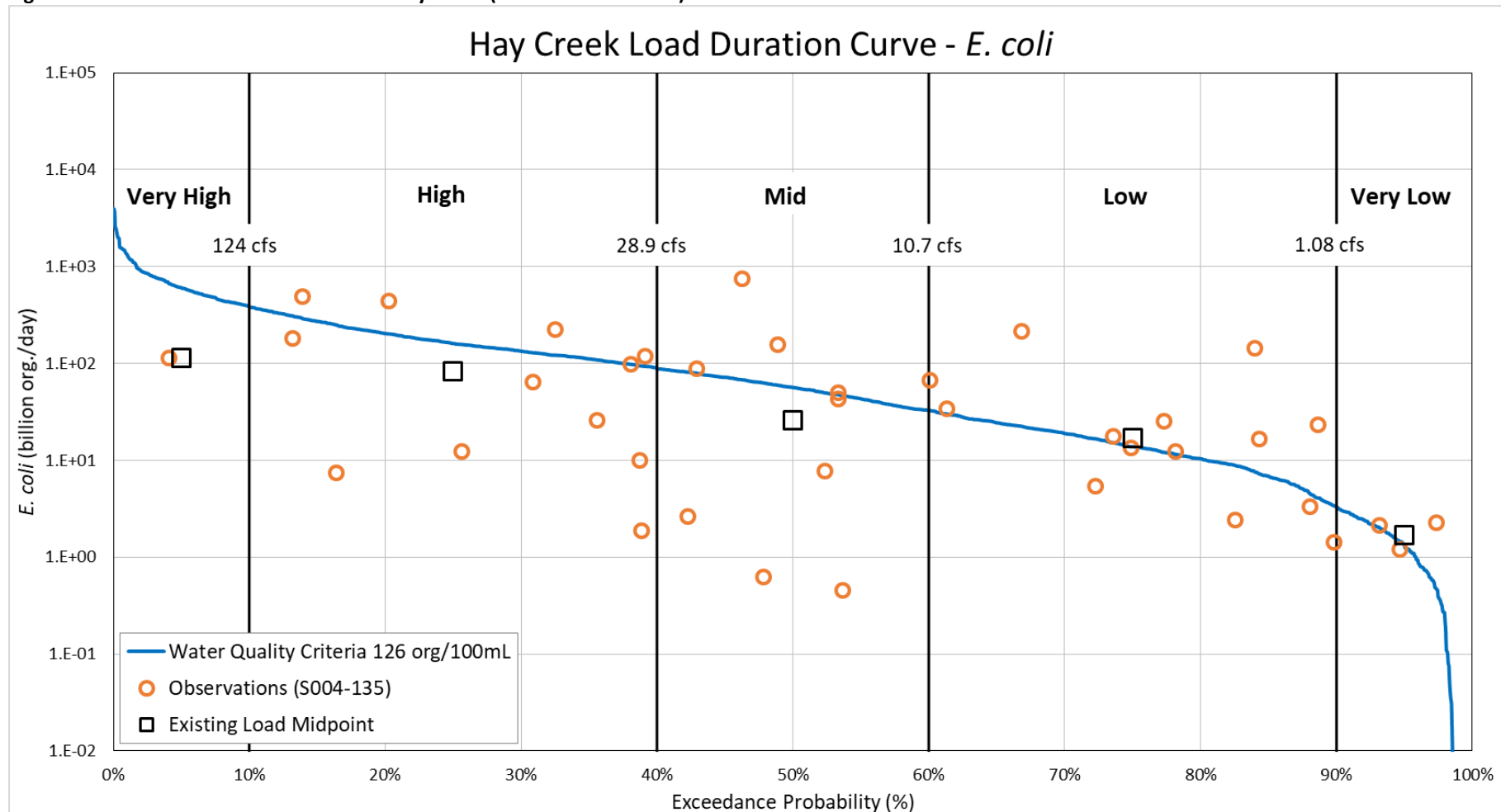
Figure 4-2: E. coli Load Duration Curve for Hay Creek (AUID 09020314-505)
