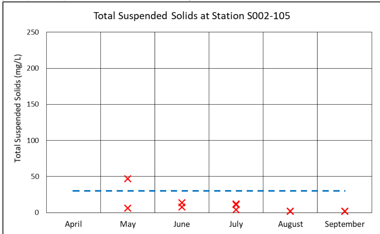
Figure B-1: TSS sampling aggregated by month on Hay Creek at the monitoring station S002-105. The dashed line denotes the stream water quality standard (30 mg/L). Data originates from intensive watershed monitoring period (2015-2016). Data not included in the TMDL analysis.
