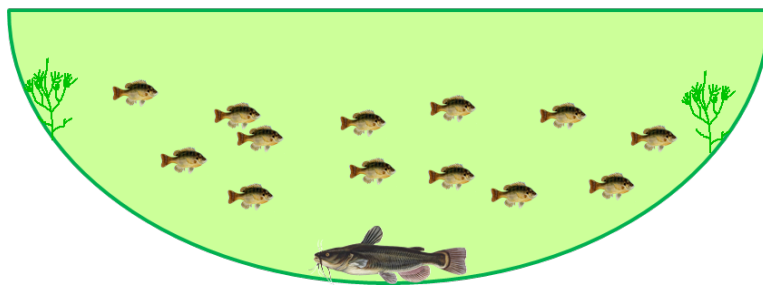
Figure 1. Alternative stable states in shallow lakes
