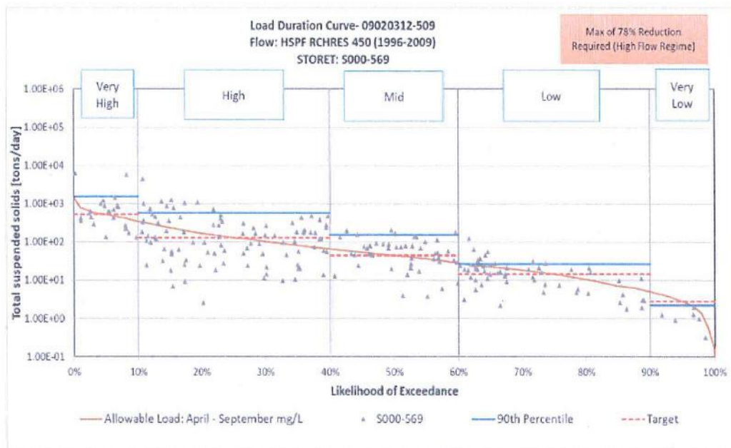
Figure 9. Two Rivers, North Branch Two Rivers to Red River (AUID 09020312-509) TSS LDC.
