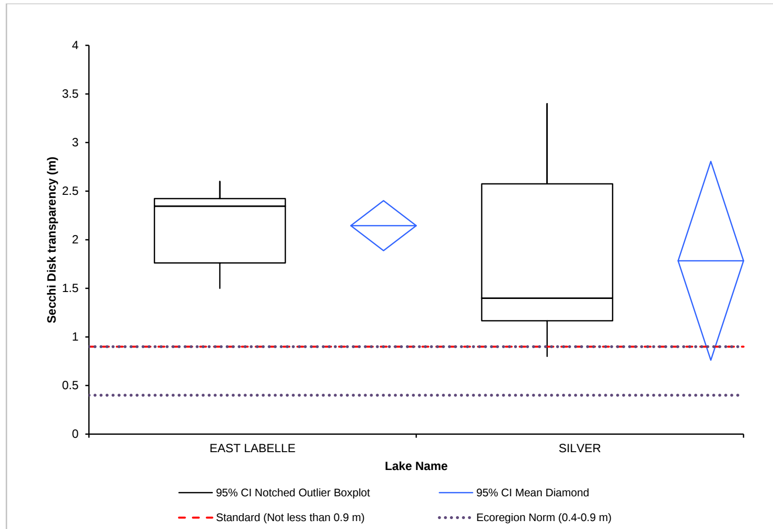
Figure 19. Secchi disk transparency depth (m) summary for deep lakes in the Lake Agassiz Ecoregion relative to the Class 2B numeric criteria and Ecoregion norms.
