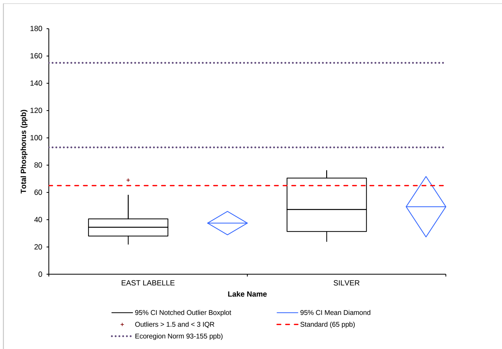
Figure 20. Total phosphorus concentration (ppb) summary for deep lakes in the Lake Agassiz Ecoregion relative to the Class 2B numeric criteria and Ecoregion norms.
