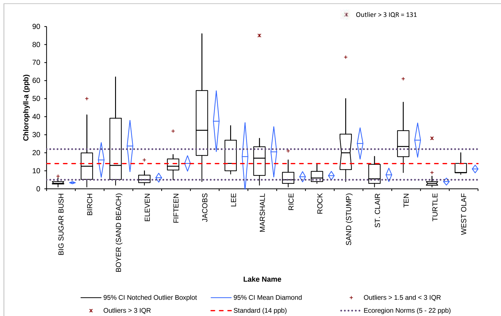
Figure 9. Chlorophyll-a concentrations (ppb) summary for deep lakes in the North Central Hardwood Forest Ecoregion relative to the Class 2B numeric criteria and Ecoregion norms.
