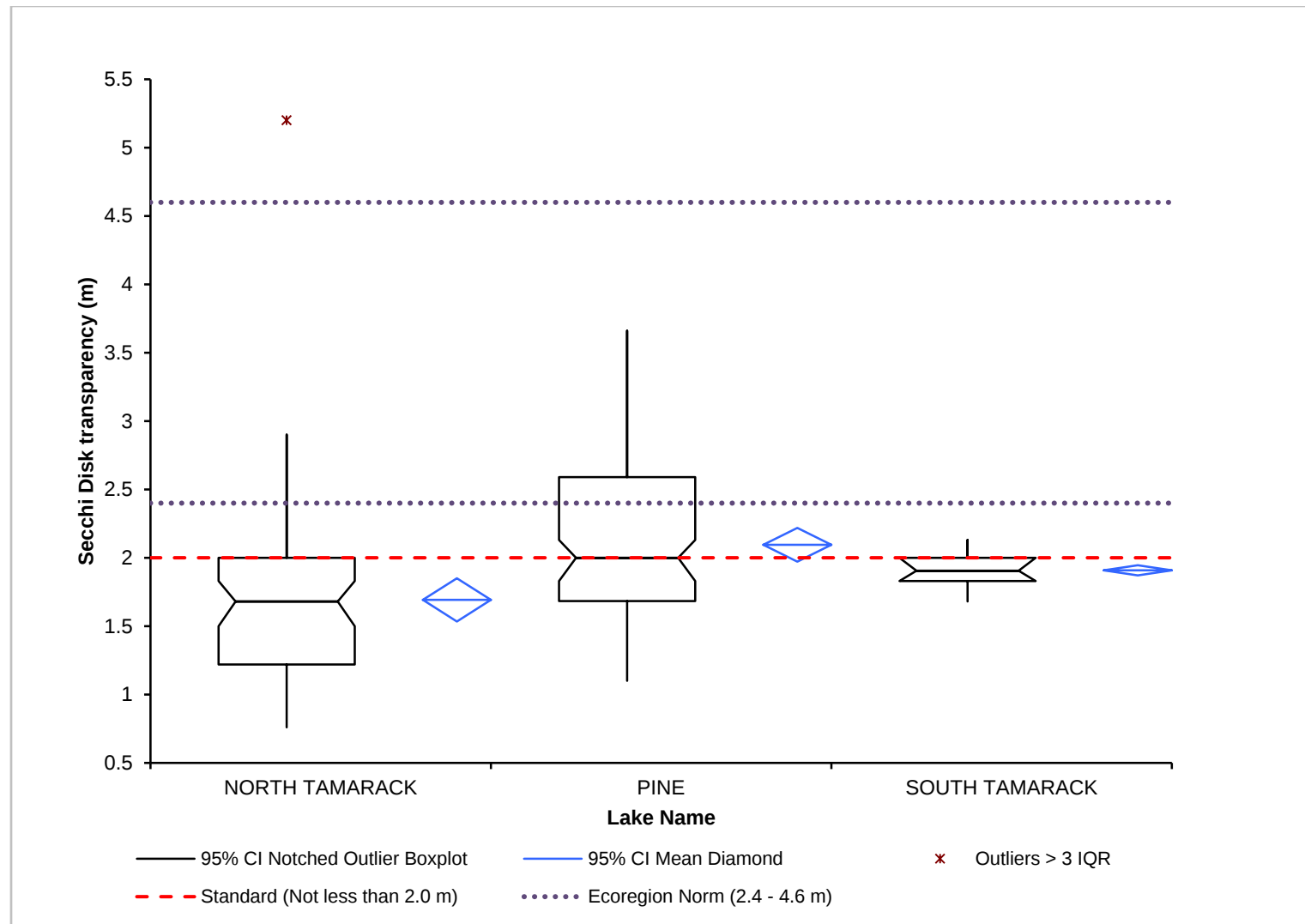
Figure 16. Secchi disk transparency depth (m) summary for lakes in the Northern Lakes and Forest Ecoregion relative to the Class 2B numeric criteria and Ecoregion norms.
