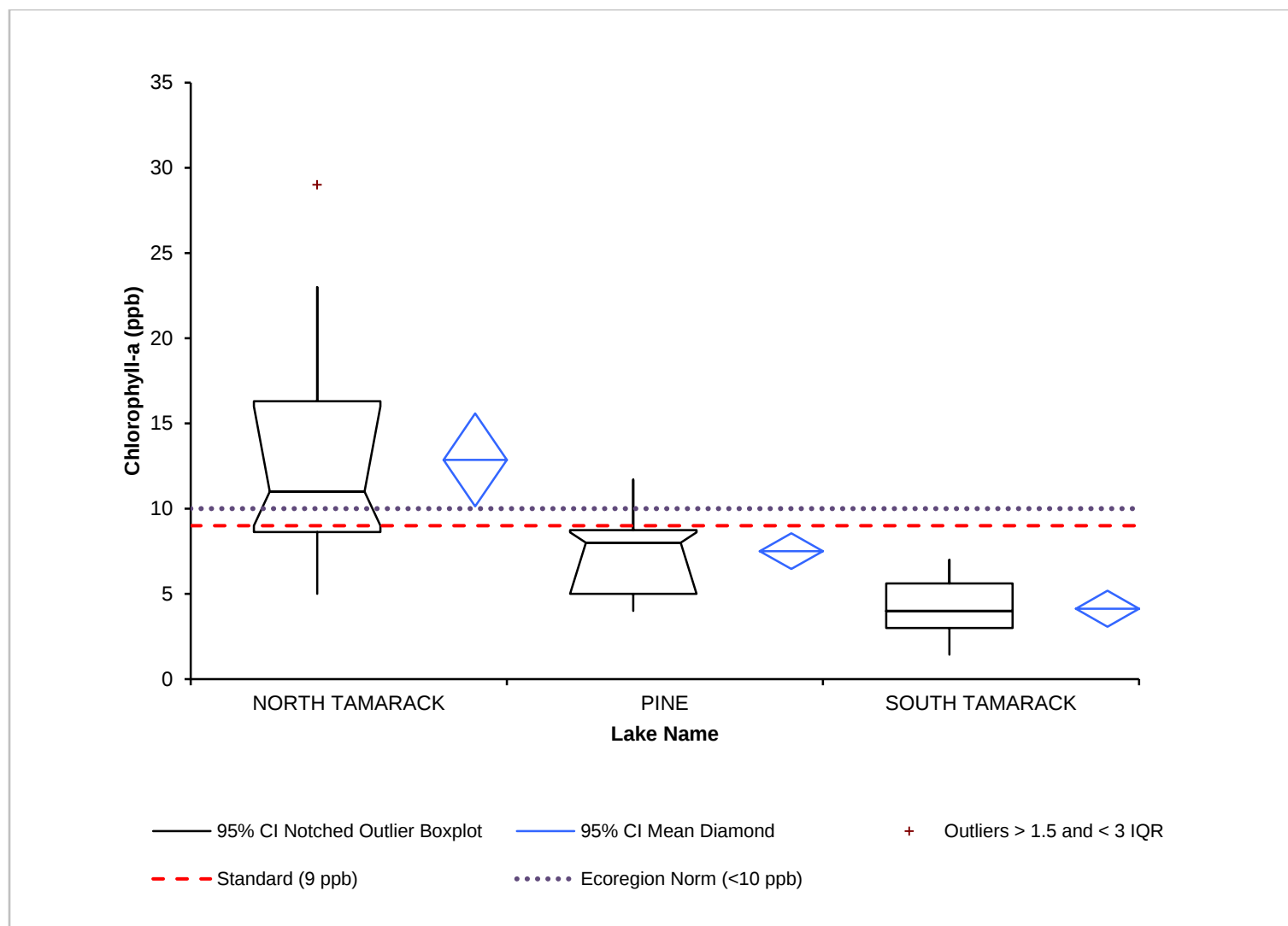
Figure 15. Chlorophyll-a concentration (ppb) summary for lakes in the Northern Lakes and Forest Ecoregion relative to the Class 2B numeric criteria and Ecoregion norms.
