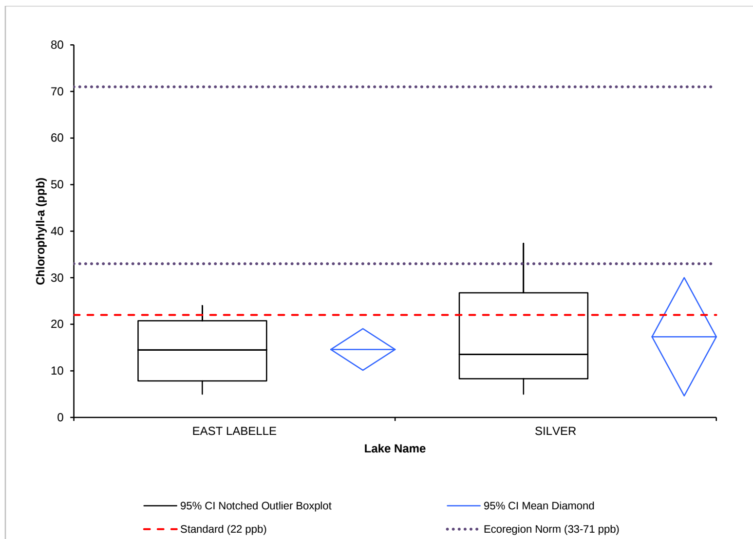
Figure 18. Chlorophyll-a concentrations (ppb) summary for deep lakes in the Lake Agassiz Ecoregion relative to the Class 2B numeric criteria and Ecoregion norms.
