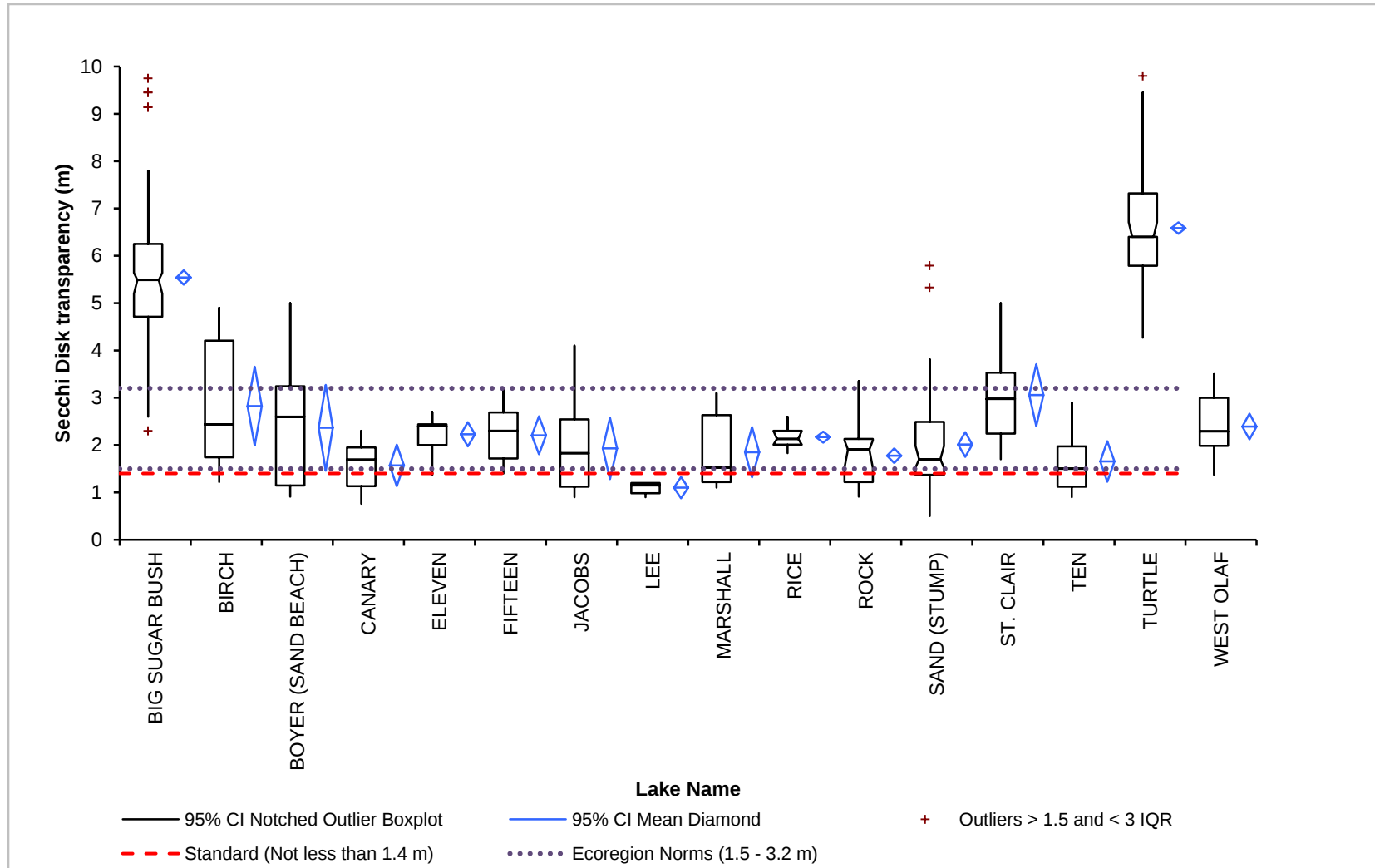
Figure 10. Secchi disk transparency depth (m) summary for deep lakes in the North Central Hardwood Forest Ecoregion relative to the Class 2B numeric criteria and Ecoregion norms.
