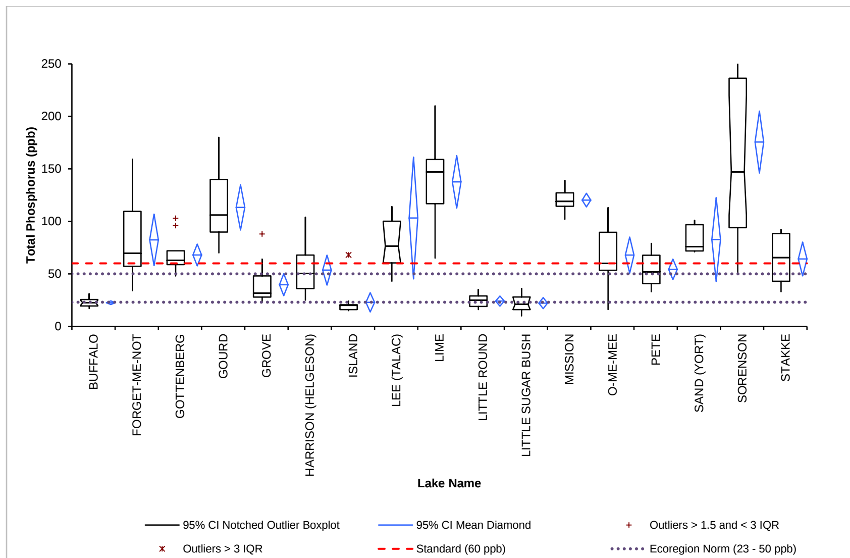
Figure 14. Total phosphorus concentration (ppb) summary for shallow lakes in the North Central Hardwood Forest Ecoregion relative to the Class 2B numeric criteria and Ecoregion norms.
