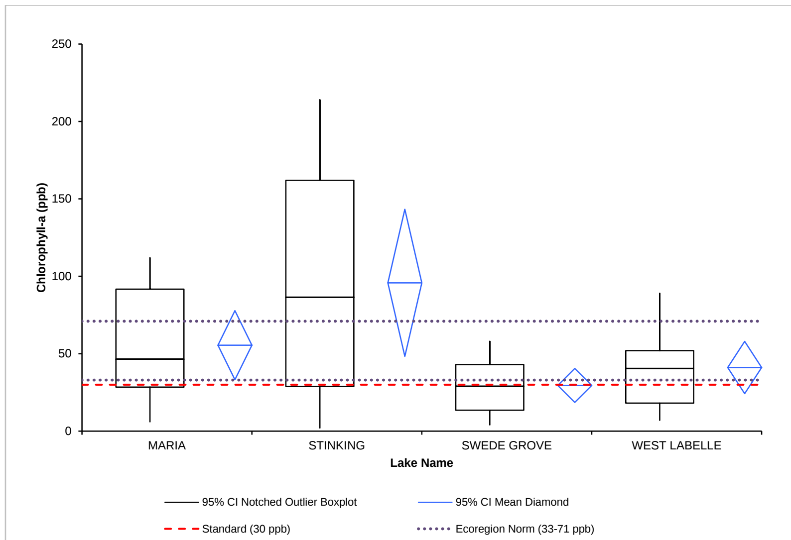
Figure 21. Chlorophyll-a concentration (ppb) summary for shallow lakes in the Lake Agassiz Ecoregion relative to the Class 2B numeric criteria and Ecoregion norms.
