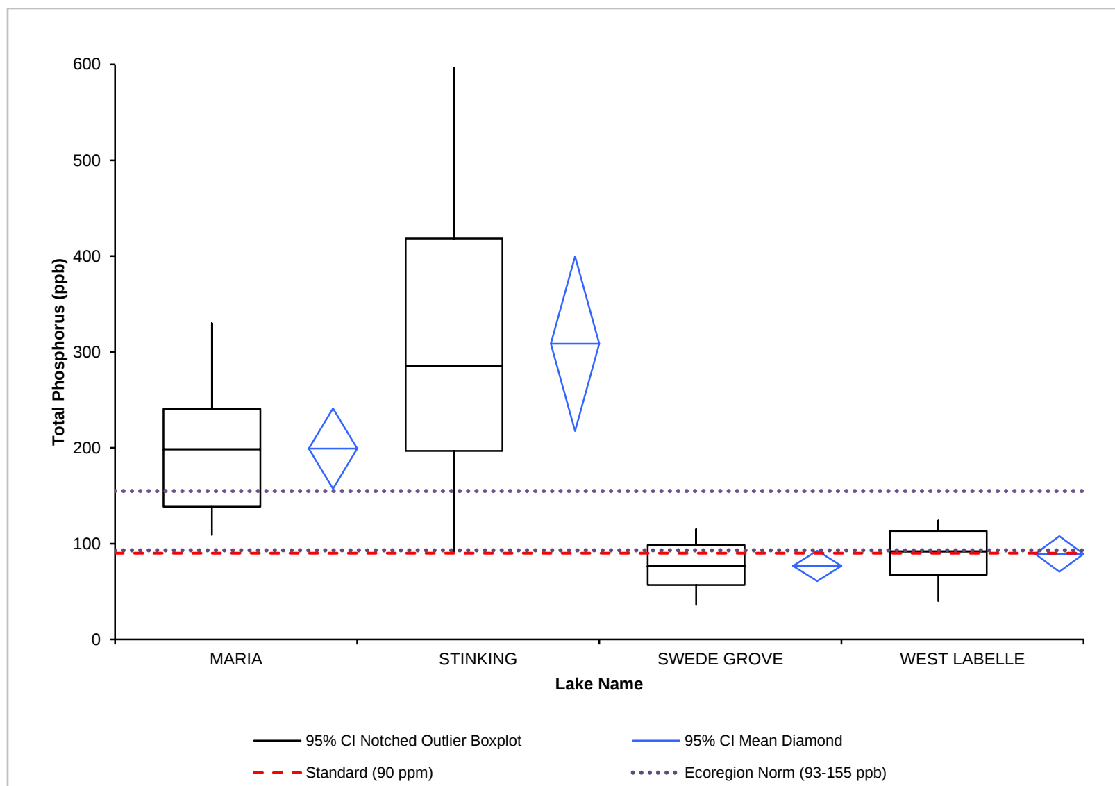
Figure 23. Total phosphorus concentration (ppb) summary for shallow lakes in the Lake Agassiz Ecoregion relative to the Class 2B numeric criteria and Ecoregion norms.
