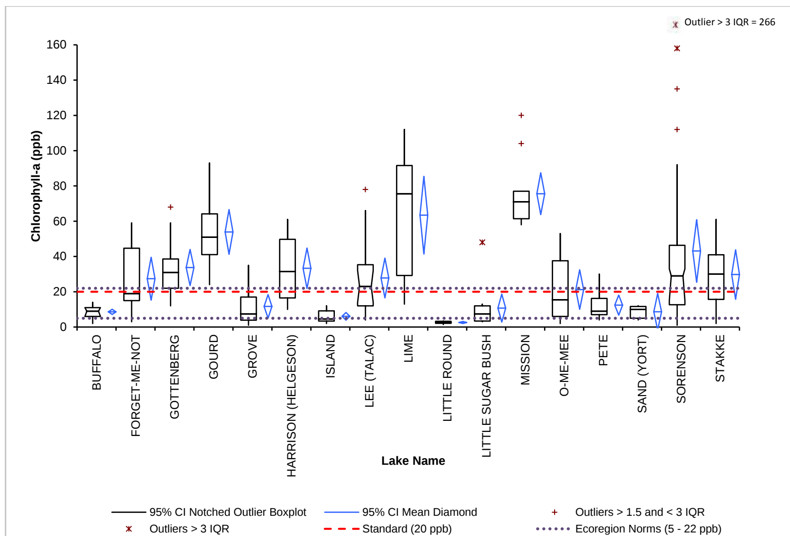
Figure 12. Chlorophyll-a concentration (ppb) summary for shallow lakes in the North Central Hardwood Forest Ecoregion relative to the Class 2B numeric criteria and Ecoregion norms.
