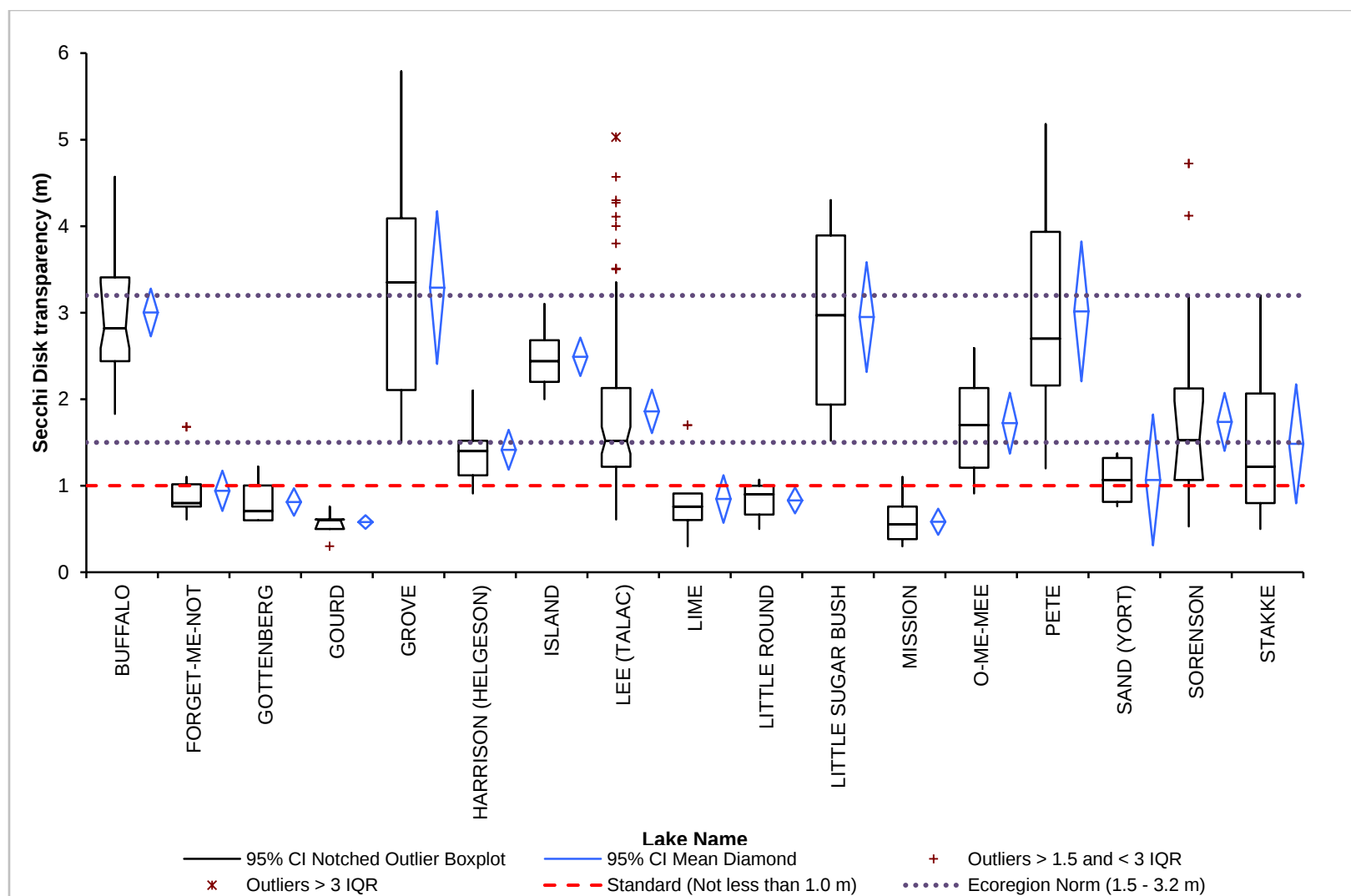
Figure 13. Secchi disk transparency (m) summary for shallow lakes in the North Central Hardwood Forest Ecoregion relative to the Class 2B numeric criteria and Ecoregion norms.
