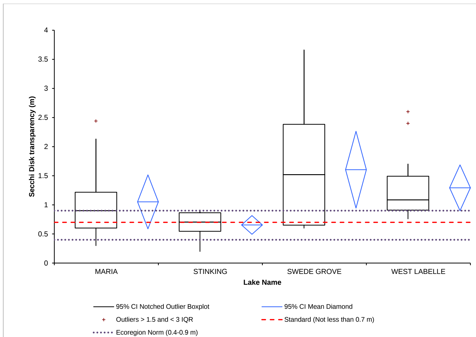
Figure 22. Secchi disk transparency depth (m) summary for shallow lakes in the Lake Agassiz Ecoregion relative to the Class 2B numeric criteria and Ecoregion norms.
