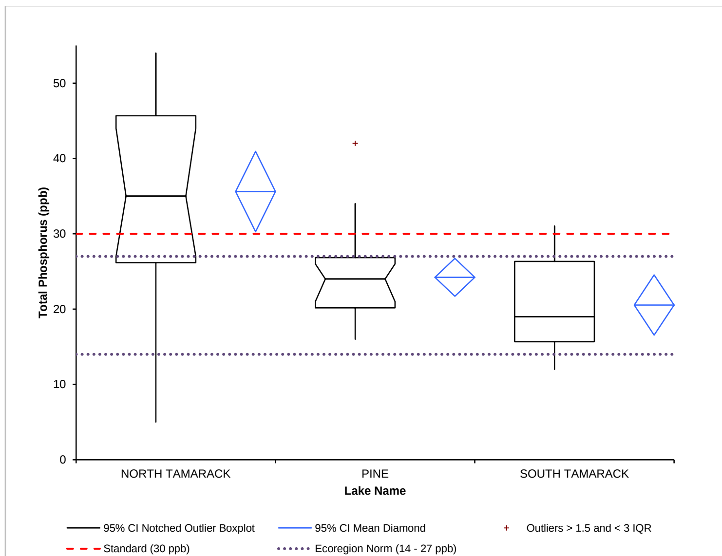
Figure 17. Total phosphorus concentration (ppb) summary for lakes in the Northern Lakes and Forest Ecoregion relative to the Class 2B numeric criteria and Ecoregion norms.
