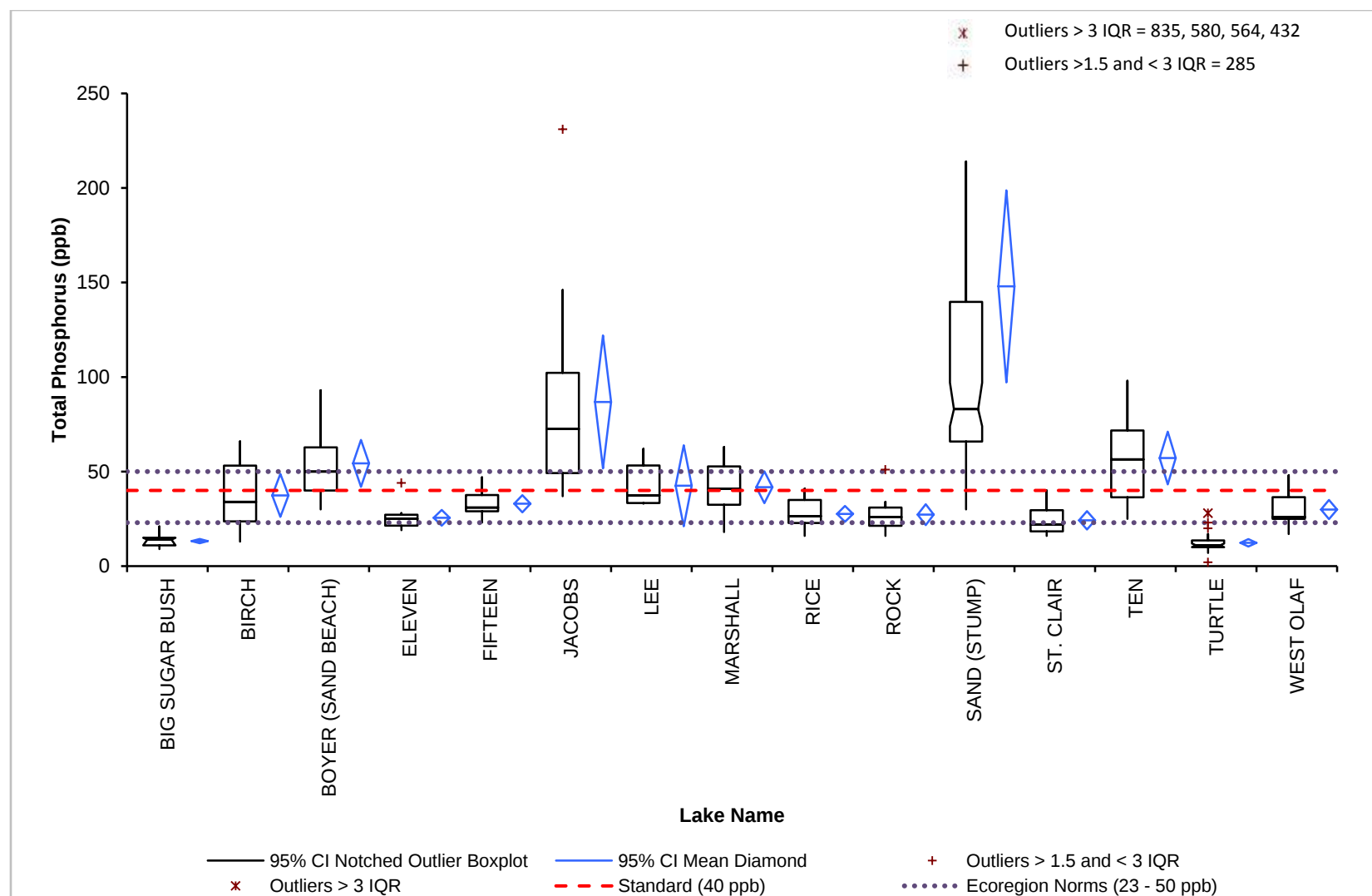
Figure 11. Total phosphorus concentration (ppb) summary for deep lakes in the North Central Hardwood Forest Ecoregion relative to the Class 2B numeric criteria and Ecoregion norms.
