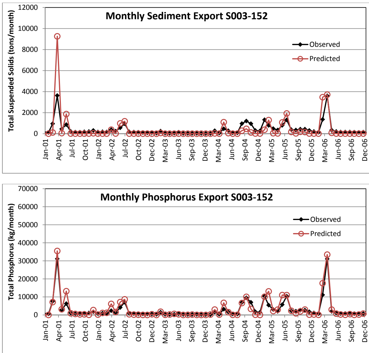
Figure 8. “Observed” and predicted monthly loads of sediment and phosphorus for monitoring point S003-152 (Buffalo River Mainstem) for the model calibration period from 2001-2006.
