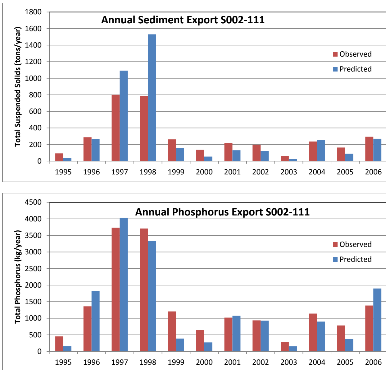
Figure 11. "Observed" and predicted annual loads of sediment and phosphorus at monitoring point S002-111 for the simulation period from 1995-2006 (water quality data were sparse or non-existent before 2001).
