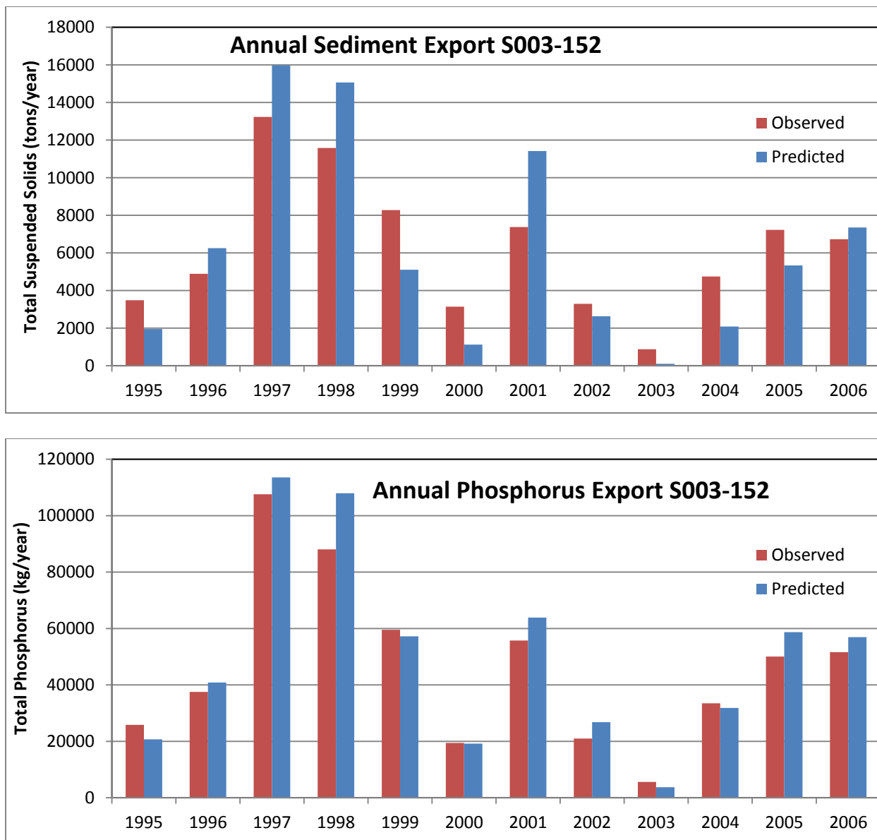
Figure 9. “Observed” and predicted annual loads of sediment and phosphorus at monitoring point S003-152 for the simulation period from 1995-2006 (water quality data were sparse or non-existent before 2001).
