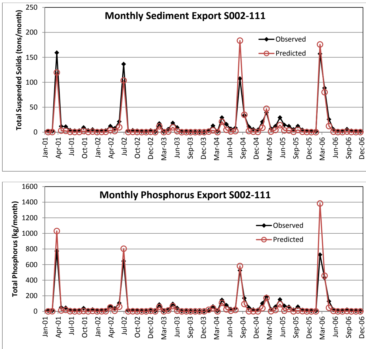
Figure 10. “Observed” and predicted monthly loads of sediment and phosphorus for monitoring point S002-111 (Buffalo River South Branch Model) for the model calibration period from 2001-2006.
