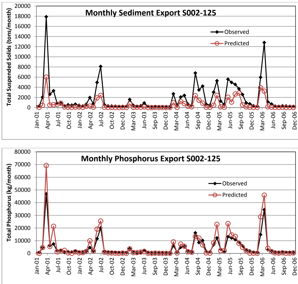
Figure 16 . “Observed” and predicted monthly loads of sediment and phosphorus for monitoring point S002-125 (Buffalo River South Branch Model) for the model calibration period from 2001-2006.
