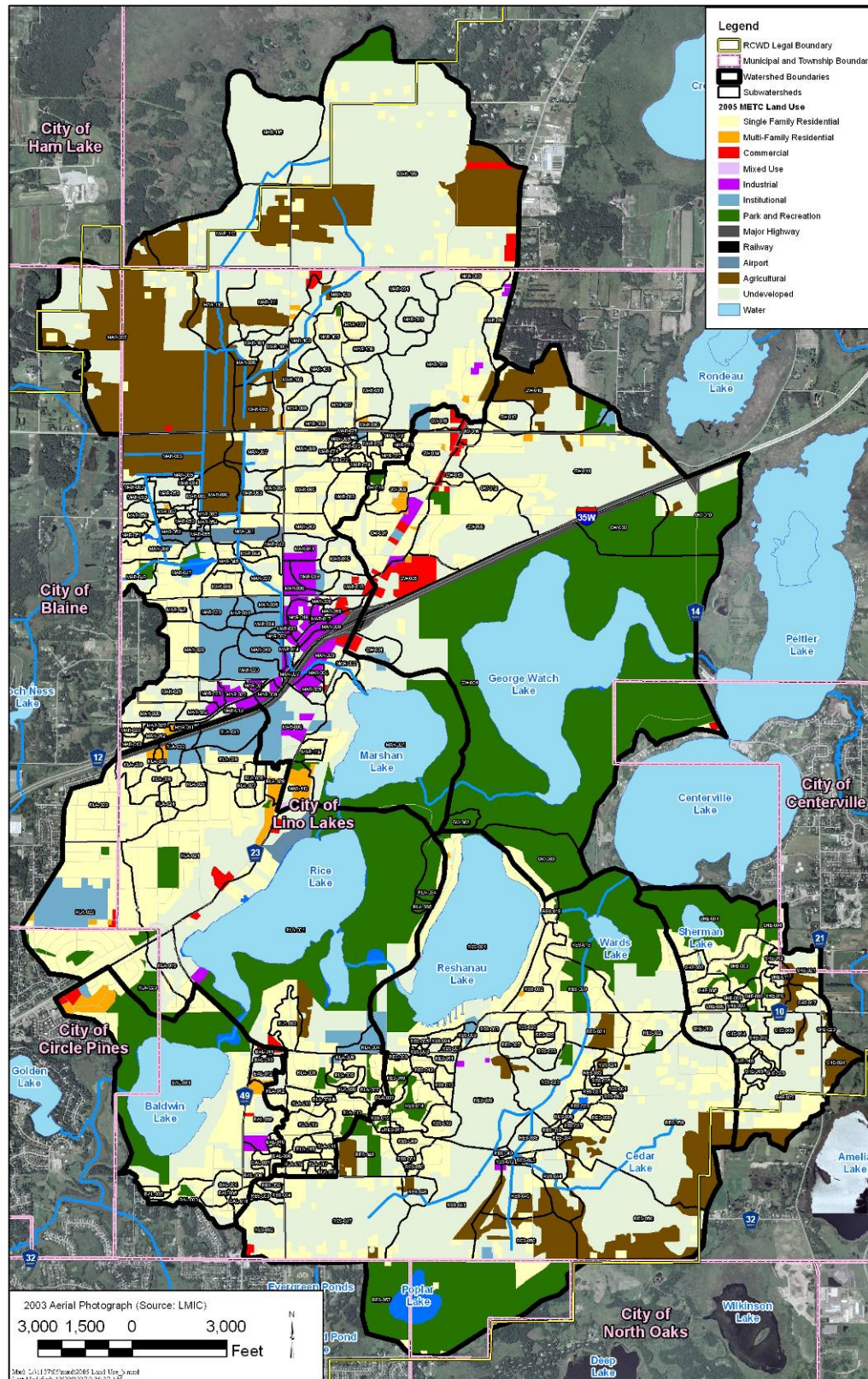
Figure 3-3. 2005 land use.
