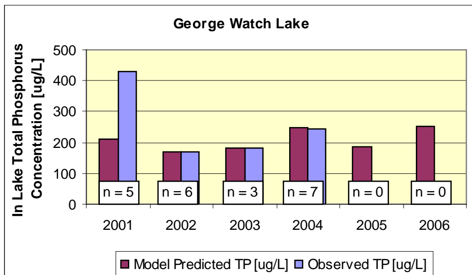
Figure 4-4. Calibrated model results for George Watch Lake, 2001-2006.
