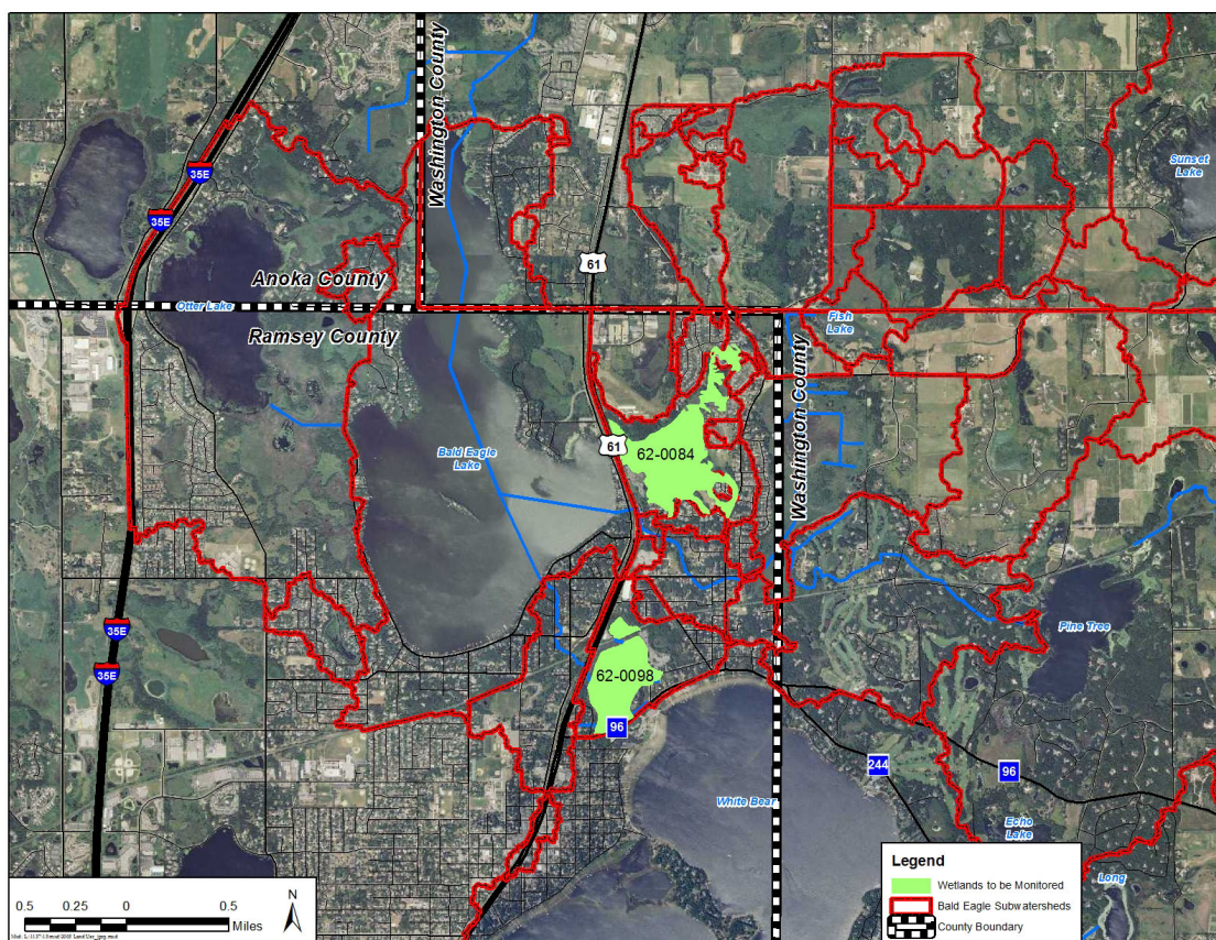
Figure 4.6. Recommended wetland outlet monitoring.
