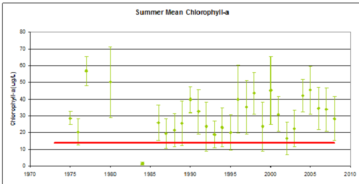
Figure 2.2. Summer (June 1 –September 30) mean chlorophyll-a concentrations for Bald Eagle Lake. Note: the red line indicates the current State standard for the North Central Hardwood Forest ecoregion.
