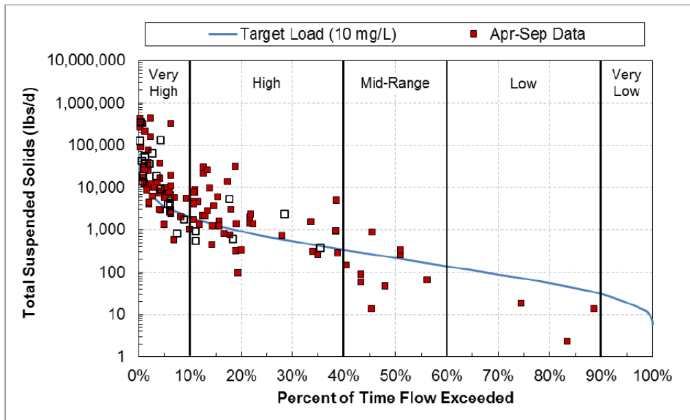
Figure 70. TSS load duration curve, Amity Creek (04010102-511).
