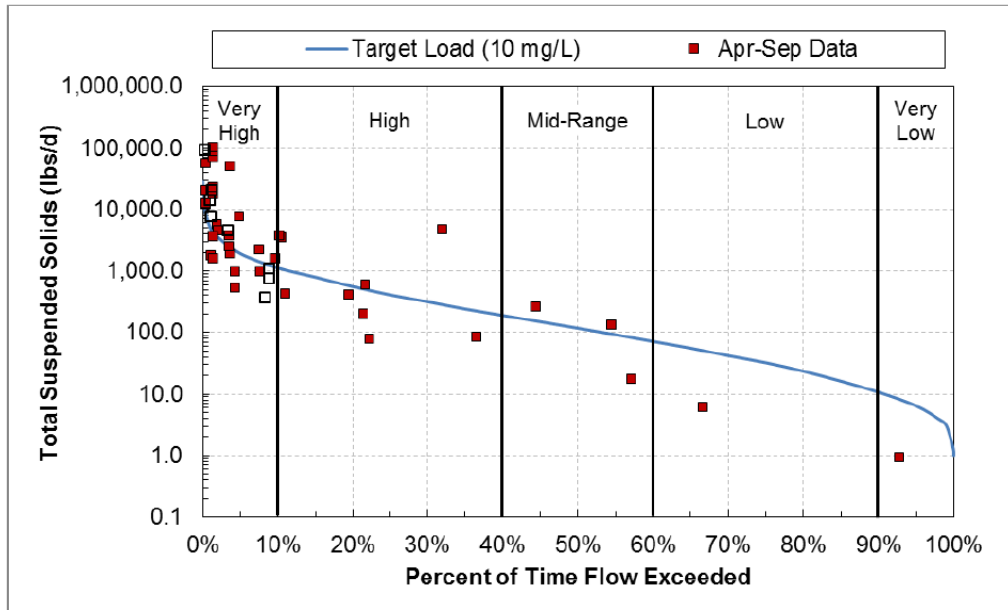
Figure 69. TSS load duration curve, Kingsbury Creek (04010201-626).
