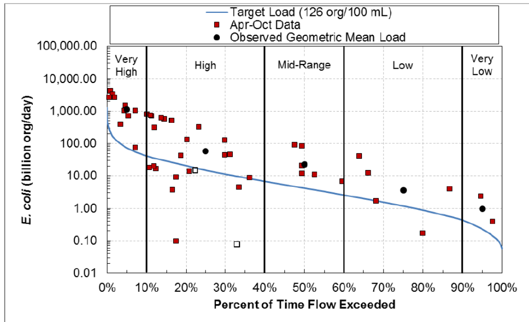
Figure 73. E. coli load duration curve, Keene Creek (04010201-627).
