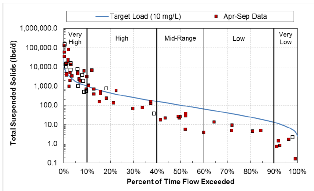
Figure 71. TSS load duration curve, Amity Creek, East Branch (04010102-540).
