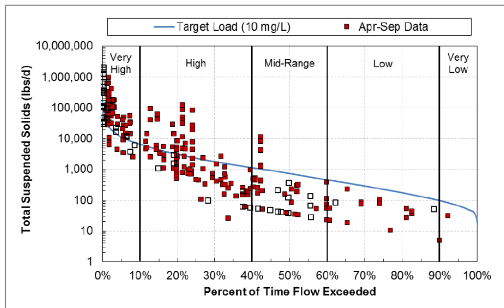
Figure 72. TSS load duration curve, Lester River (04010102-549).
