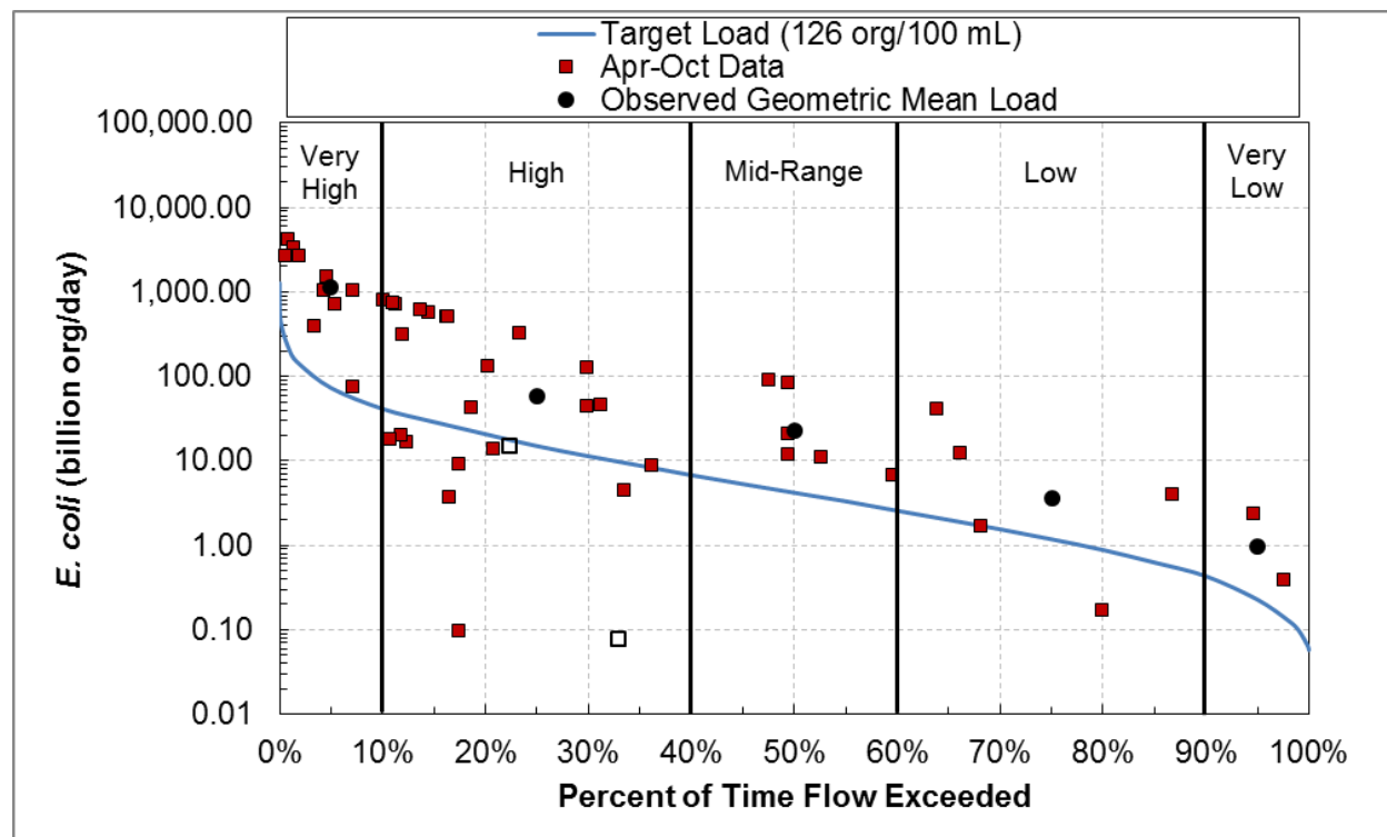
Figure 73. E. coli load duration curve, Keene Creek (04010201-627).
