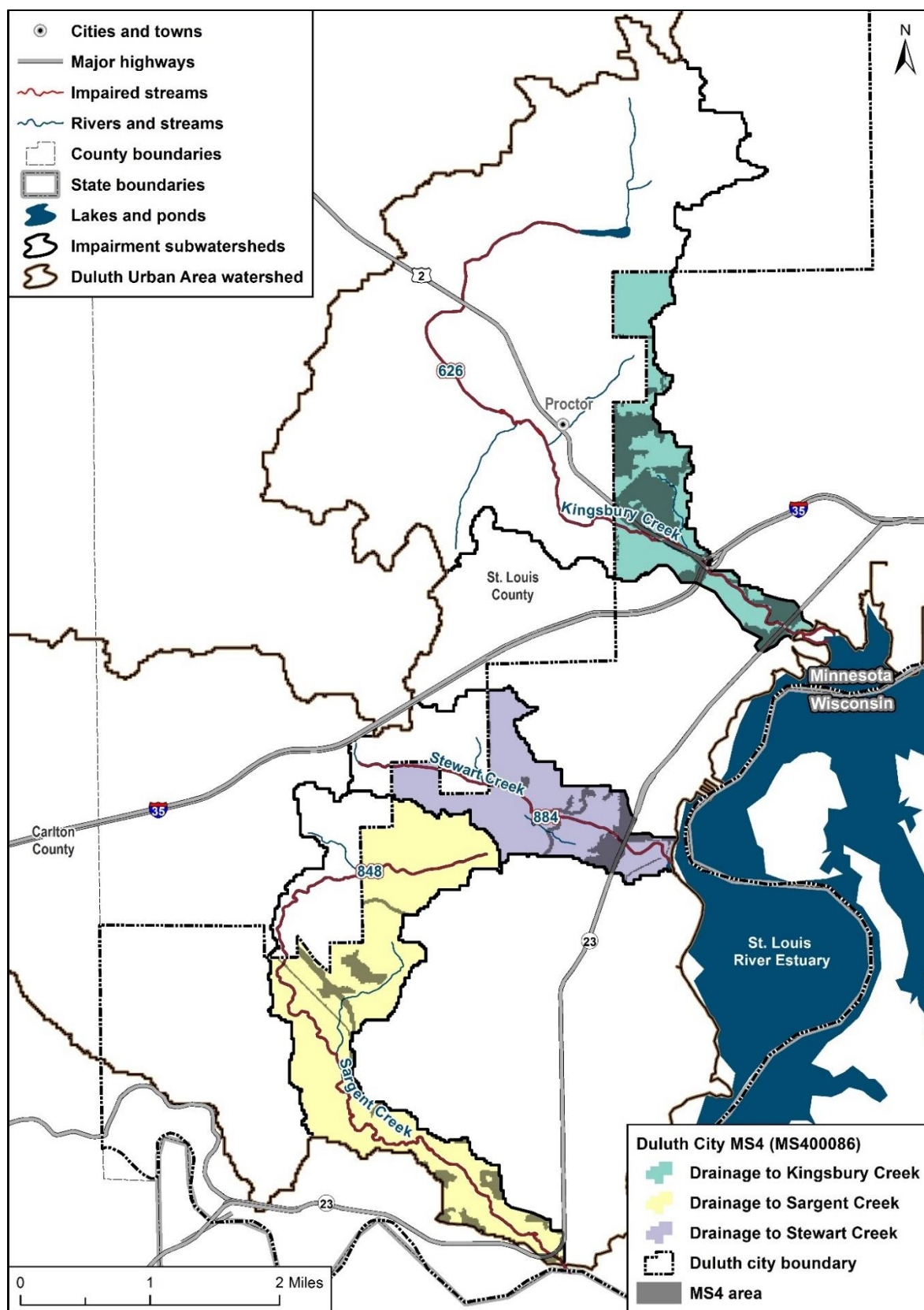
Figure 89. Duluth MS4 (southern).
