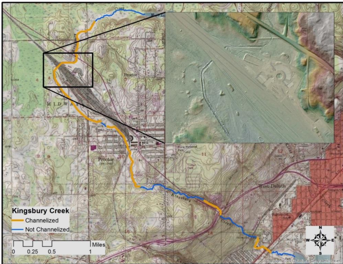
Figure 26. Channelized and straightened reaches of Kingsbury Creek (MPCA 2016).
