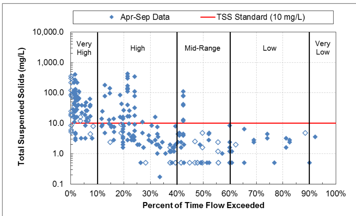
Figure 17. TSS water quality duration plot, Lester River.
