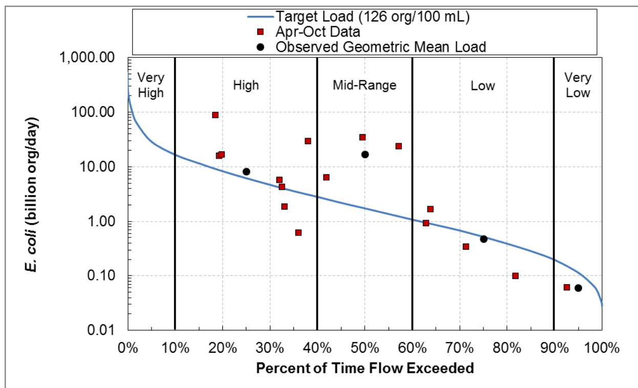
Figure 75. E. coli load duration curve, Sargent Creek (04010201-848).
