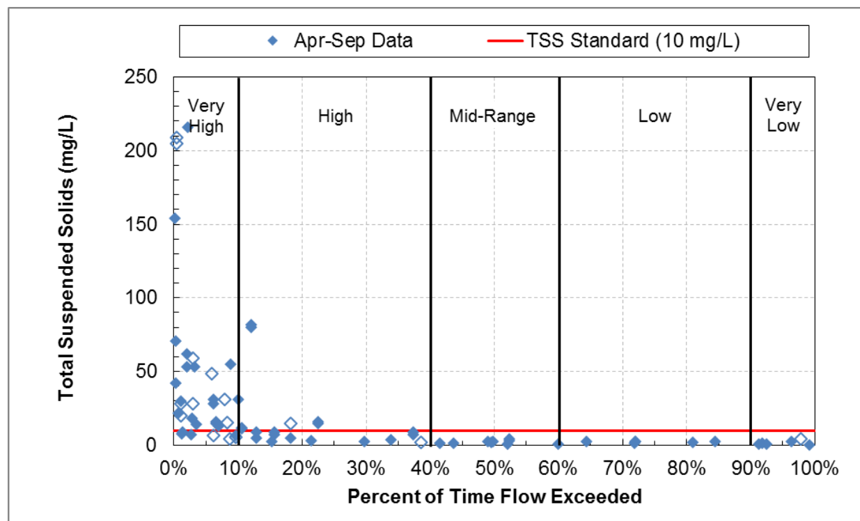
Figure 16. TSS water quality duration plot, Amity Creek, East Branch.
