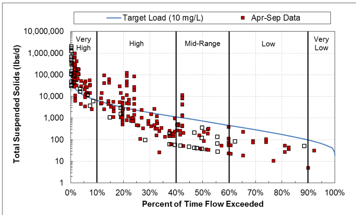
Figure 72. TSS load duration curve, Lester River (04010102-549).
