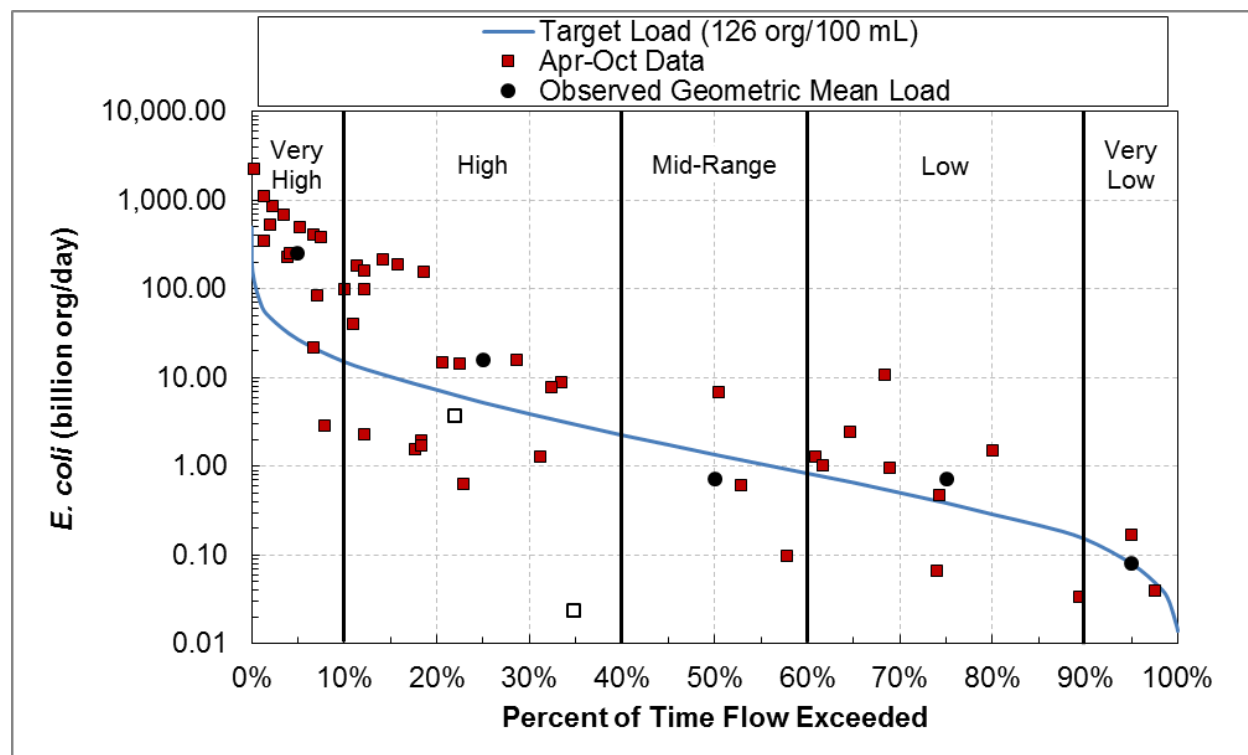
Figure 77. E. coli load duration curve, Unnamed Creek (Merritt Creek; 04010201-987).
