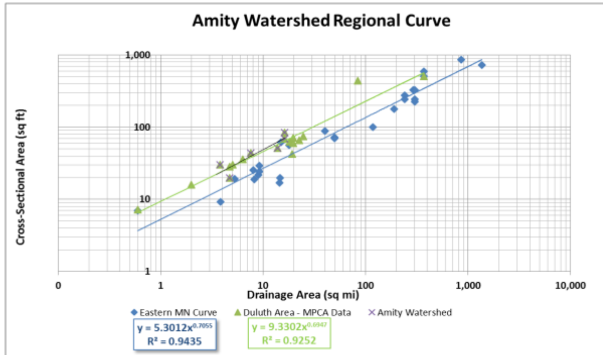
Figure 7. Bankfull Cross-Section Areas from Table 3 Plotted on Regional Curve Relationships for Eastern Minnesota and Duluth Area.
