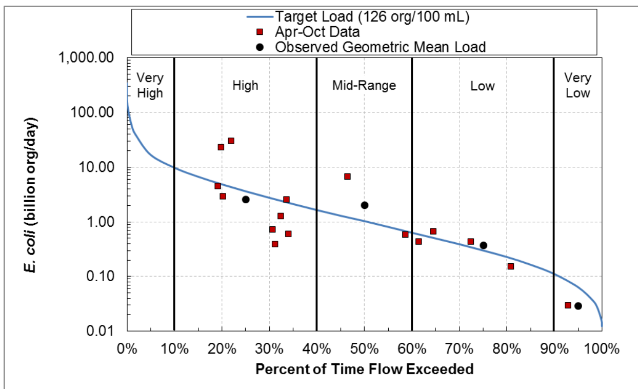
Figure 76. E. coli load duration curve, Stewart Creek (04010201-884).
