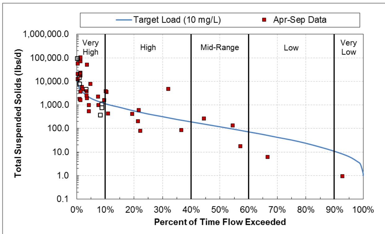
Figure 69. TSS load duration curve, Kingsbury Creek (04010201-626).
