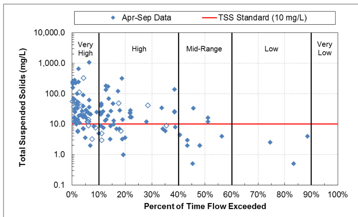
Figure 15. TSS water quality duration plot, Amity Creek.
