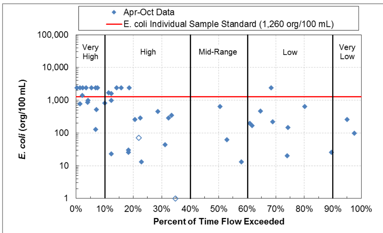
Figure 12. E. coli water quality duration plot, Unnamed Creek (Merritt Creek).
