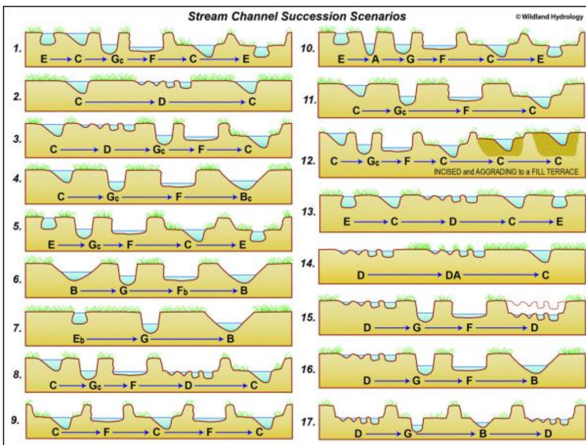
Figure 3. Stream Channel Succession Scenarios for Predicting Channel Evolution (Rosgen, 2006).
