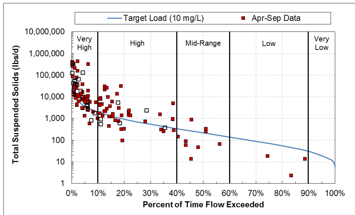
Figure 70. TSS load duration curve, Amity Creek (04010102-511).
