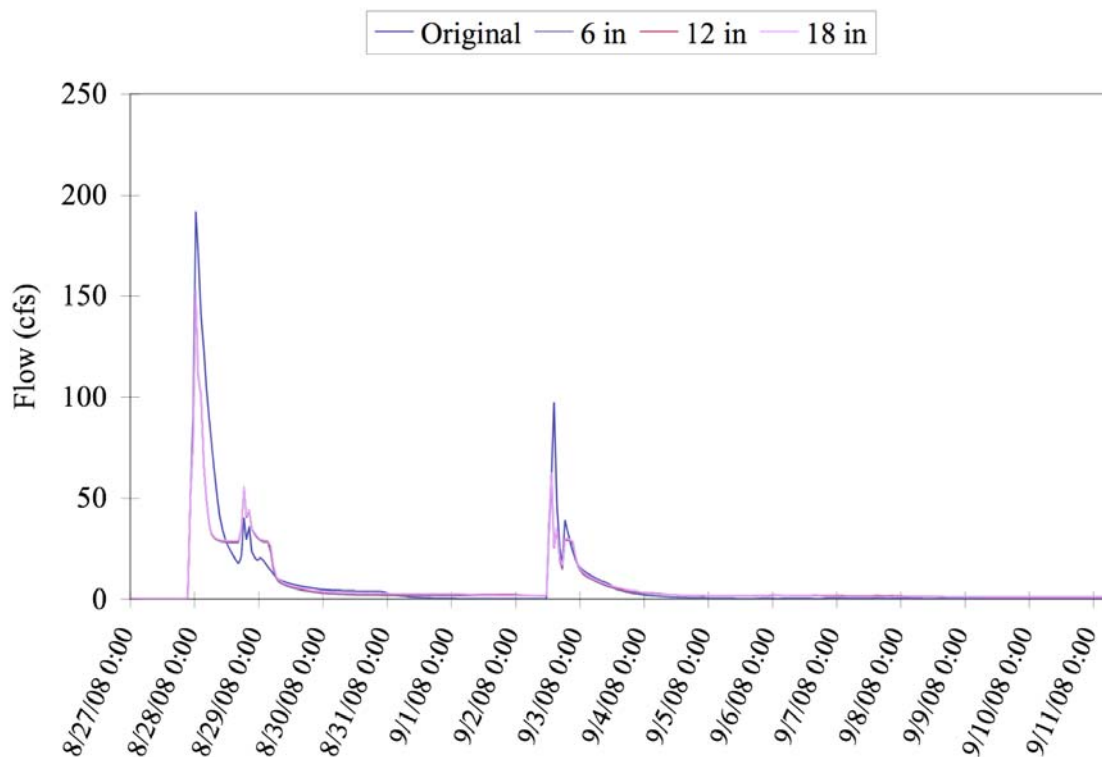
Figure 9.10 Modeled streamflows in Miller Creek at the lower gauging station when three retention ponds are added in the watershed (Figure 9.9).
