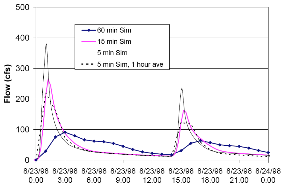
Figure 2.1 Example of time-step dependent flow from the NRRI SWMM 4 model.
