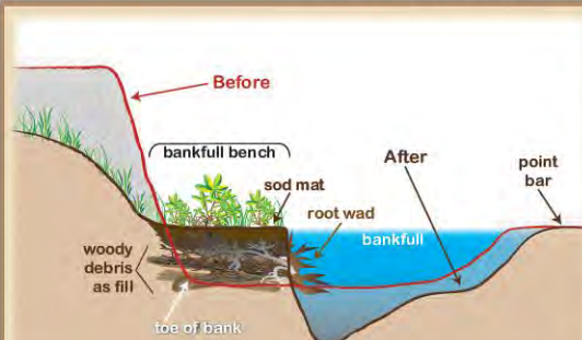
Installation of root wads using an excavator to drive tree trunks into the bankfull bench (looking upstream).
