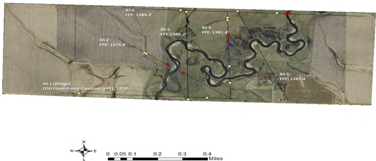
Figure 17. Aerial photo of the landowner's property on Kanaranzi Creek with Q50 FPE. Each black line is a cross section created with LiDAR data. Flood-prone elevation is labeled at each of the cross sections, as well as colored dots that show areas within that cross section that are below the FPE. All cross sections were created from right (looking downstream) to left across the stream.
