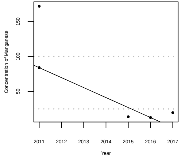
Concentration of Manganese over time for SW-543 at MW-4
