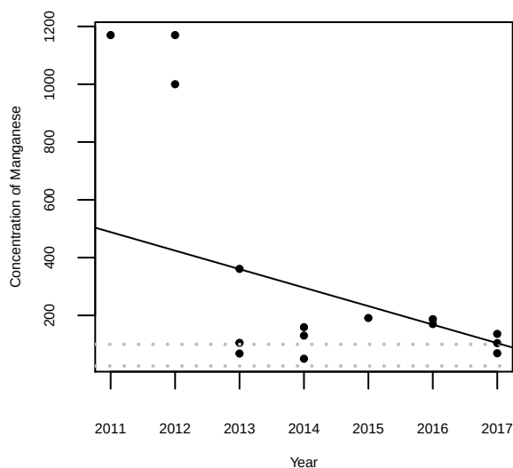
Concentration of Manganese over time for SW-590 at MW-2
