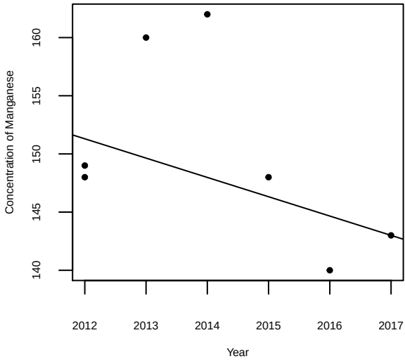
Concentration of Manganese over time for SW-464 at MW-3A
