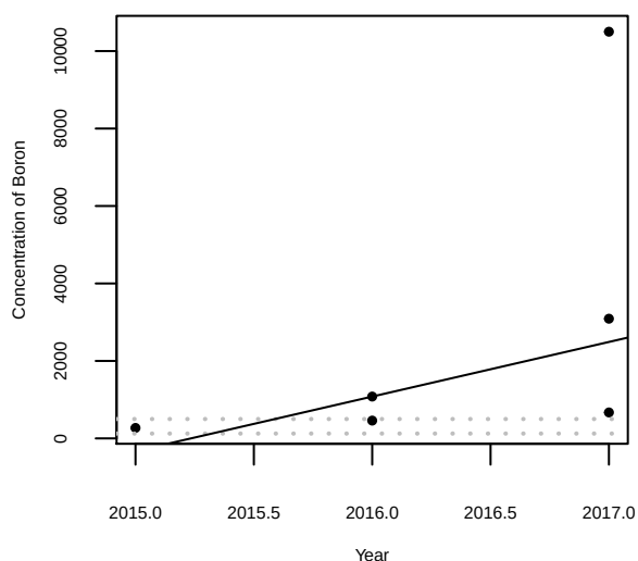
Concentration of Boron over time for SW-590 at MW-3
