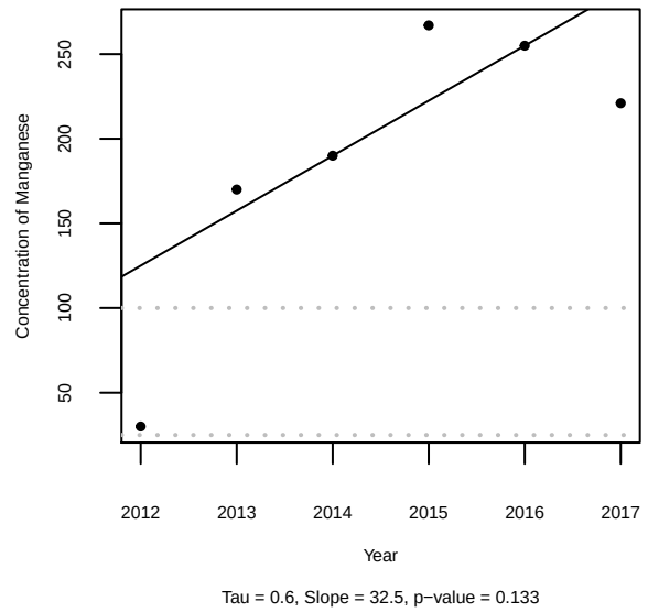
Concentration of Manganese over time for SW-464 at MW-3B
