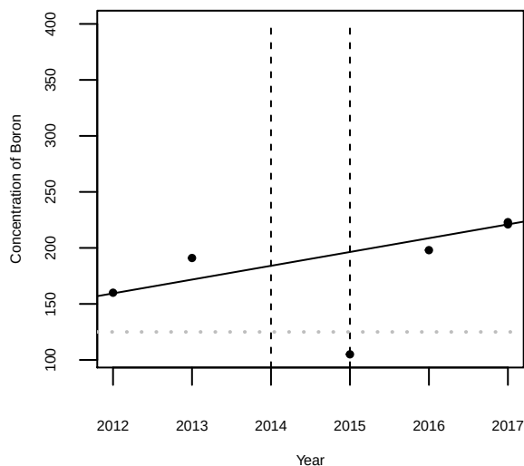
Concentration of Boron over time for SW-188 at MW-10R
