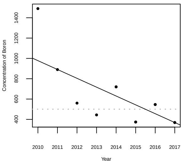
Concentration of Boron over time for SW-337 at MW-2
