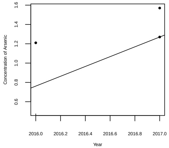
Concentration of Arsenic over time for SW-464 at MW-6A
