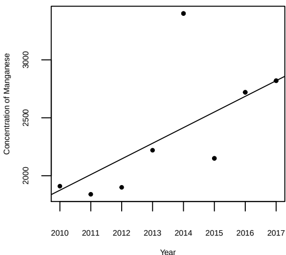
Concentration of Manganese over time for SW-337 at MW-2
