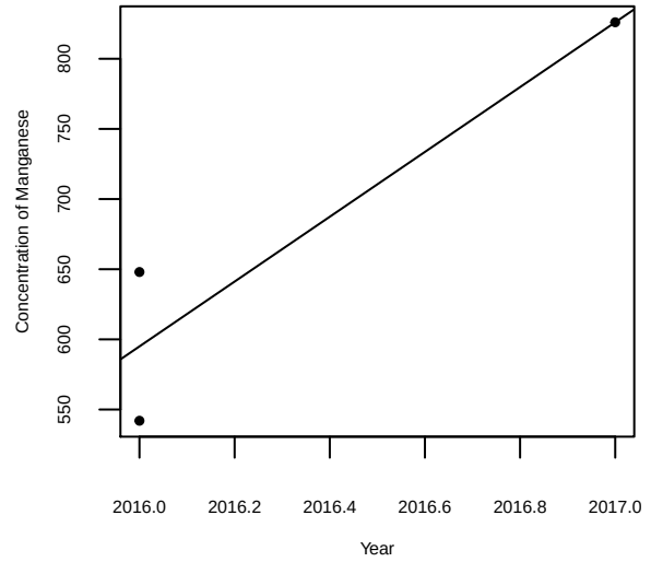
Concentration of Manganese over time for SW-306 at MW-20
