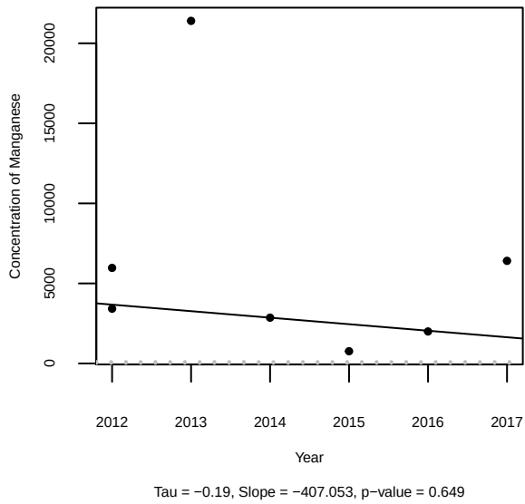
Concentration of Manganese over time for SW-464 at MW-5A
