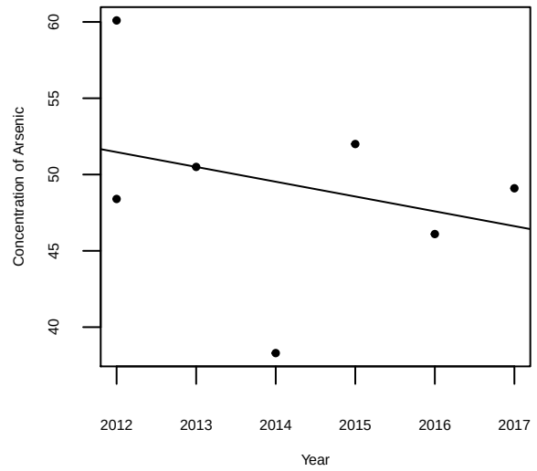
Concentration of Arsenic over time for SW-464 at MW-3A
