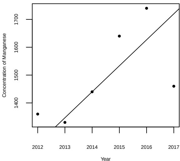
Concentration of Manganese over time for SW-188 at MW-10F
