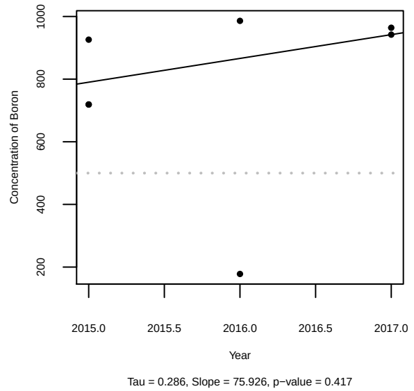
Concentration of Boron over time for SW-188 at MW-12
