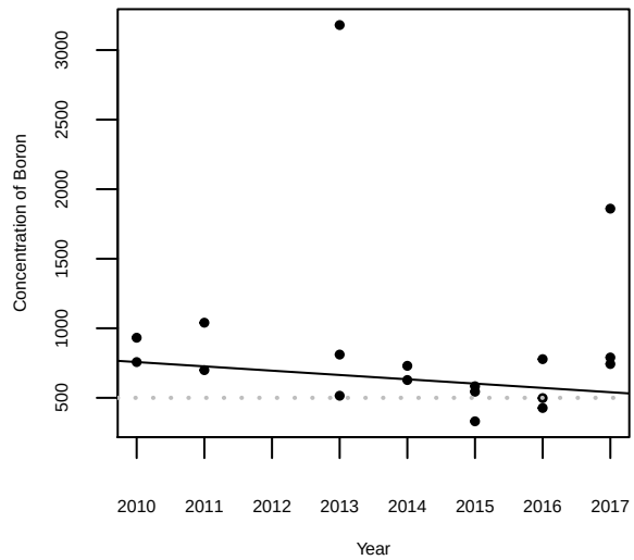
Concentration of Boron over time for SW-335 at MW-9
