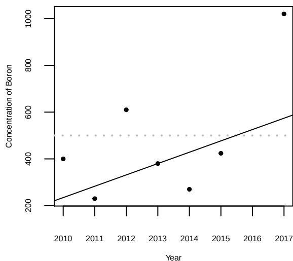
Concentration of Boron over time for SW-318 at MW-5
