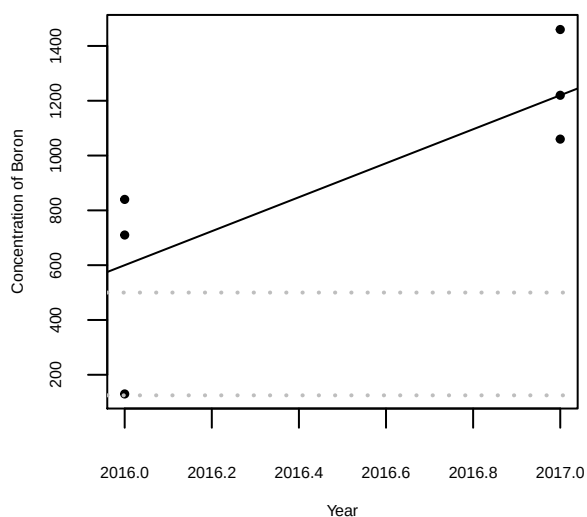
Concentration of Boron over time for SW-600 at MW-4A
