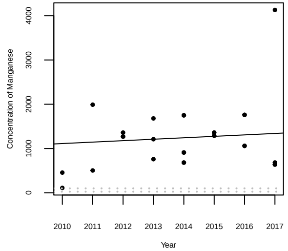
Concentration of Manganese over time for SW-432 at MW-4
