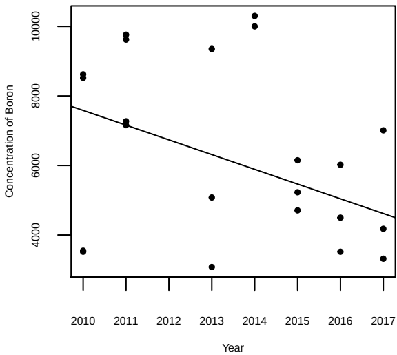
Concentration of Boron over time for SW-335 at MW-8
