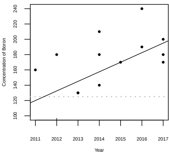
Concentration of Boron over time for SW-590 at MW-2
