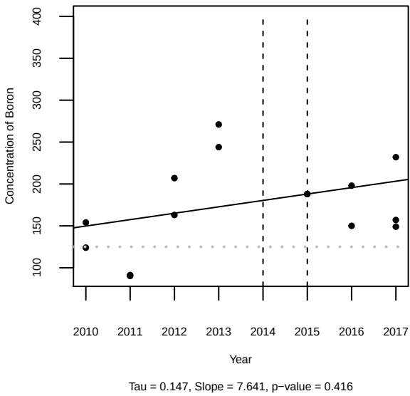
Concentration of Boron over time for SW-188 at MW-5
