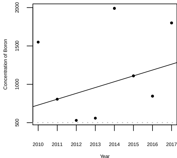
Concentration of Boron over time for SW-337 at MW-3
