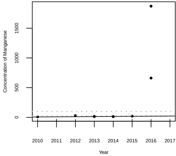
Concentration of Manganese over time for SW-306 at MW-9
