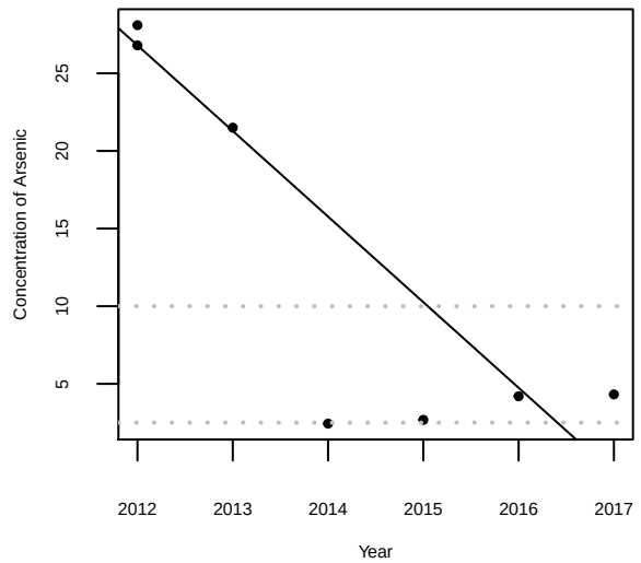
Concentration of Arsenic over time for SW-464 at MW-2A
