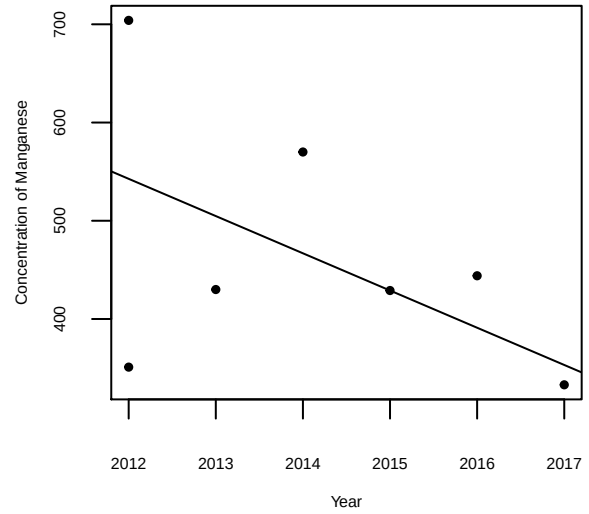
Concentration of Manganese over time for SW-464 at MW-2B
