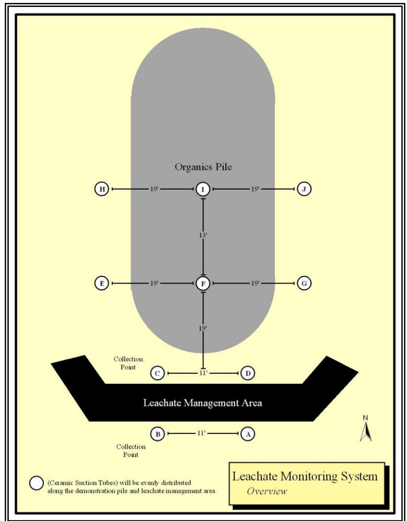
Diagram 4. Schematics of Leachate Monitoring System
