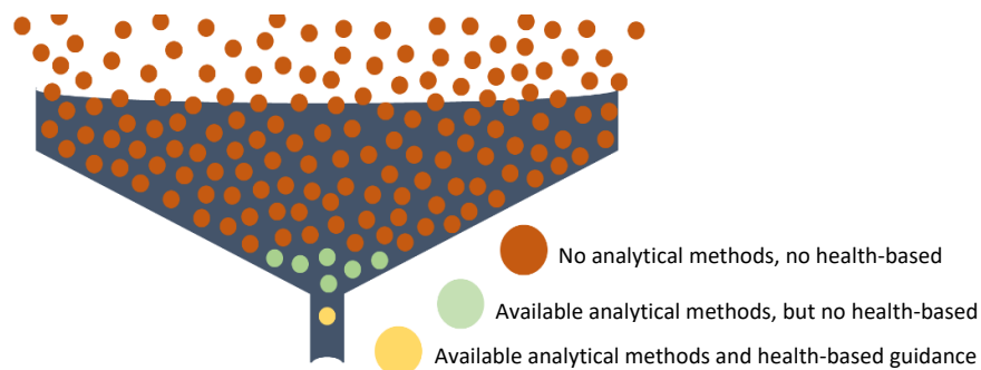
Figure 2. Schematic diagram of PFAS risk assessment and method availability.
